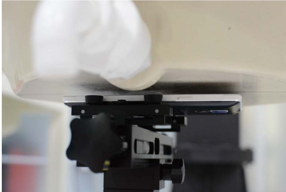
SAR Test Setup Photo 15: Front Side at 1.0 cm with Wireless Charging Cover
