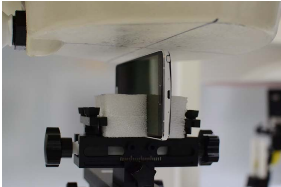
SAR Test Setup Photo 22: Right Edge at 1.0 cm with Wireless Charging Cover
