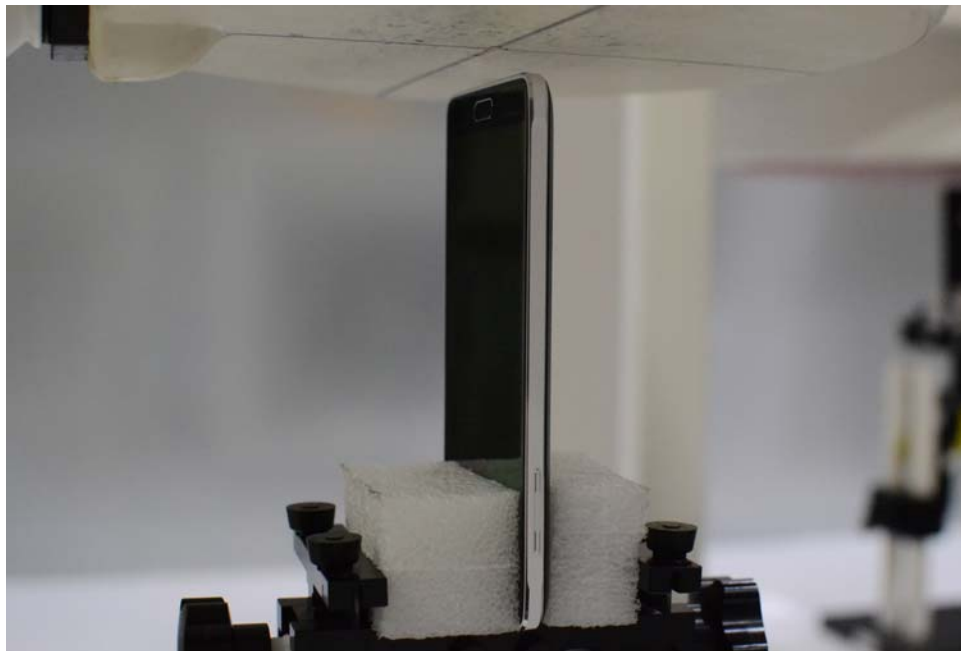
SAR Test Setup Photo 20: Bottom Edge at 1.0 cm with Wireless Charging Cover
