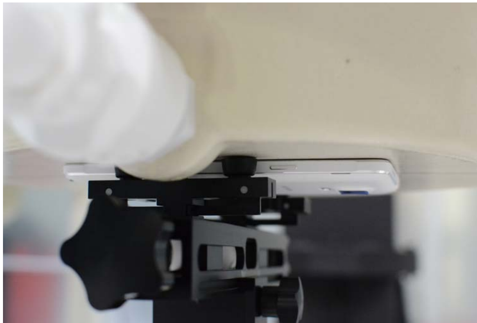
SAR Test Setup Photo 16: Front Side at 0.0 cm with Standard Cover
