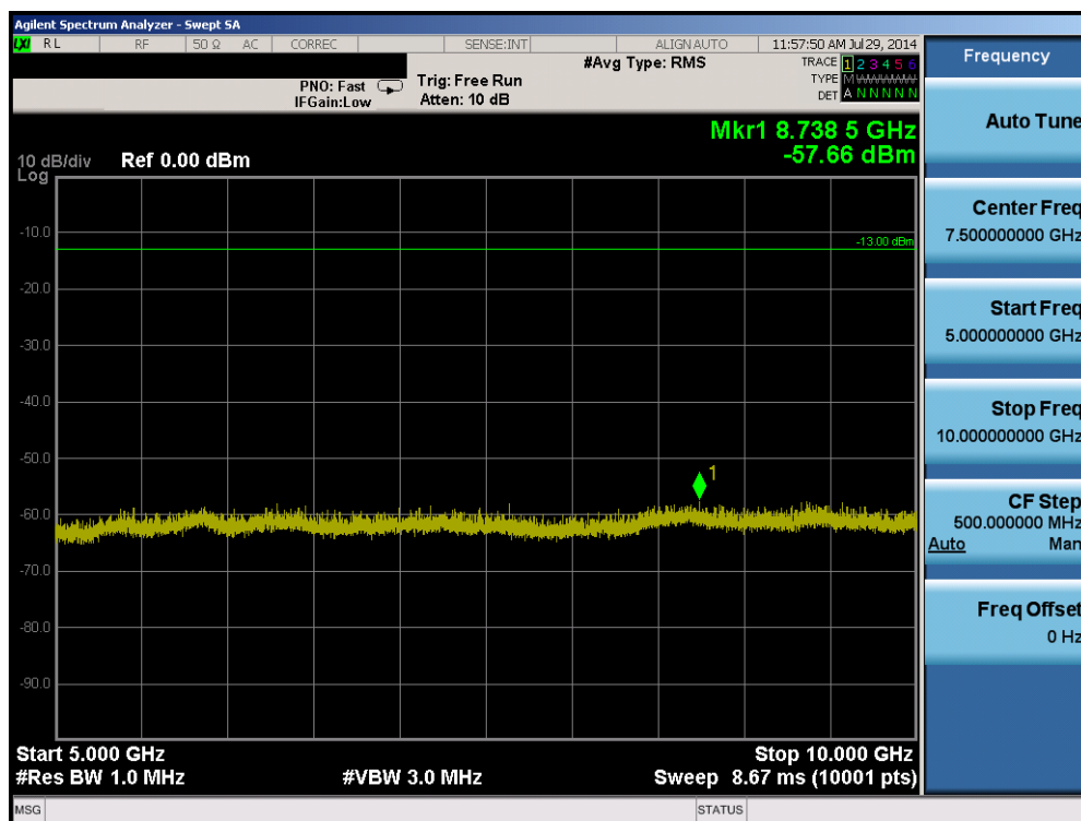
Plot 6-16. Conducted Spurious Plot (Band 17 – 5.0MHz QPSK – RB Size 1, RB Offset 0 – Mid Channel)
