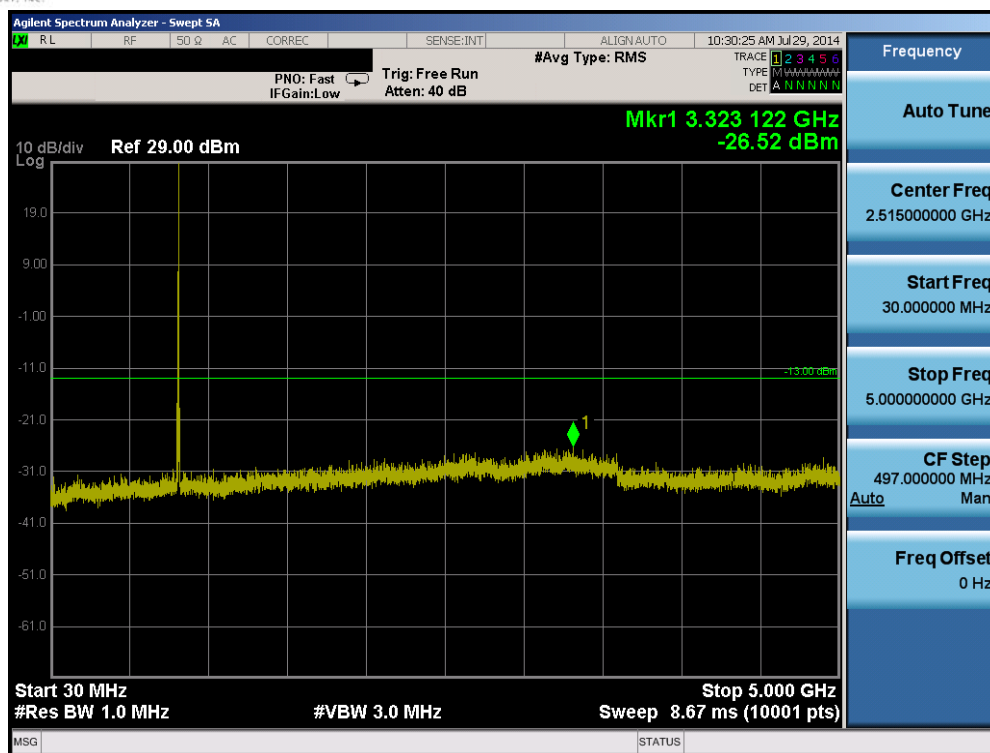
Plot 6-21. Conducted Spurious Plot (Band 5 – 5.0MHz QPSK – RB Size 1, RB Offset 0 – Mid Channel)
