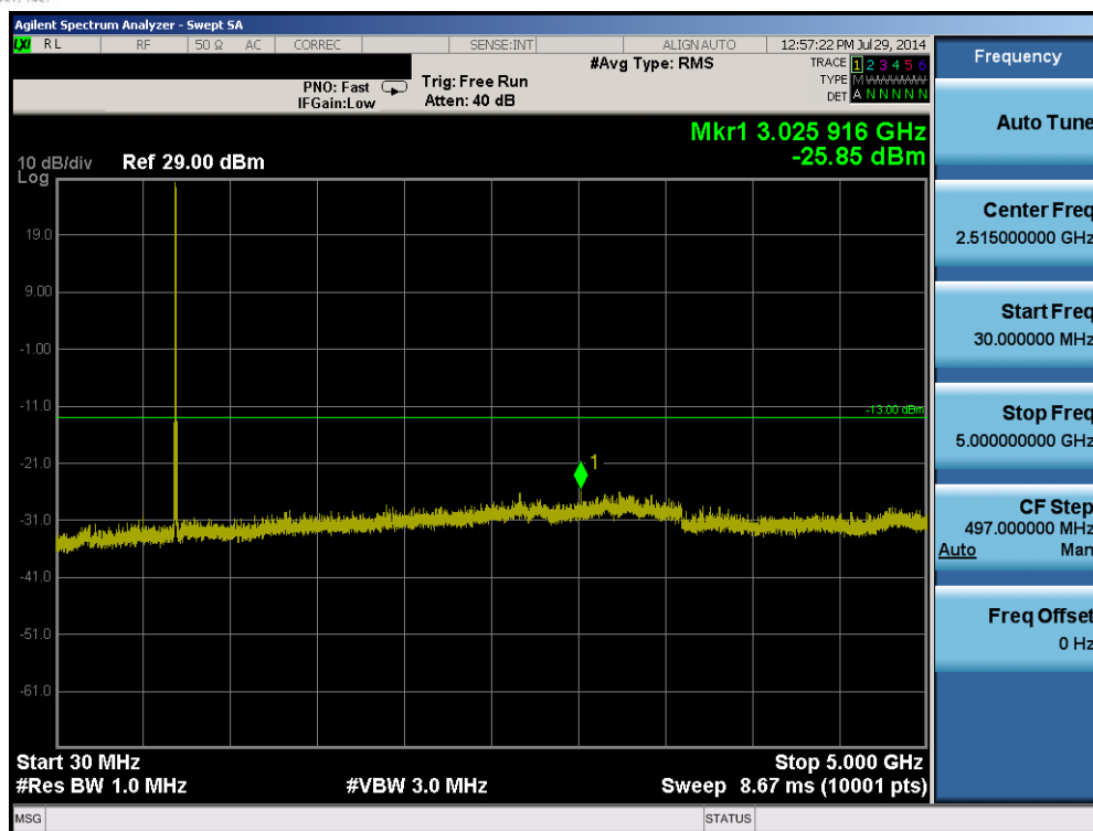
Plot 6-17. Conducted Spurious Plot (Band 17 – 5.0MHz QPSK – RB Size 1, RB Offset 0 – High Channel)
