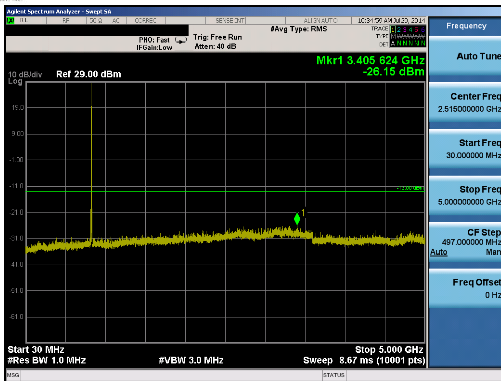
Plot 6-23. Conducted Spurious Plot (Band 5 – 5.0MHz QPSK – RB Size 1, RB Offset 0 – High Channel)
