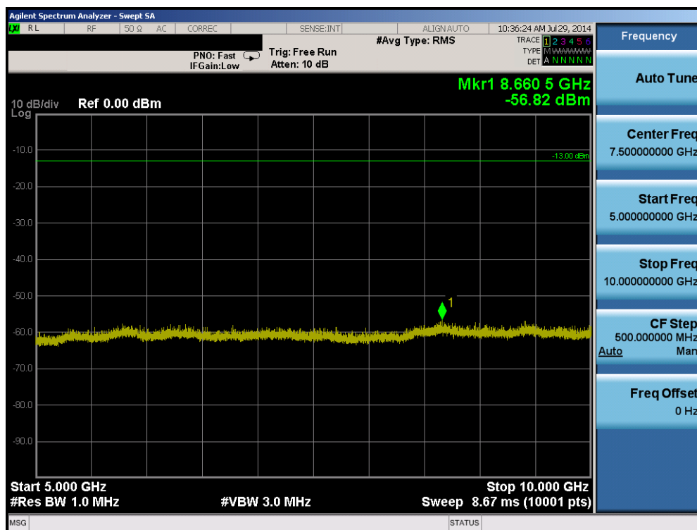
Plot 6-24. Conducted Spurious Plot (Band 5 – 5.0MHz QPSK – RB Size 1, RB Offset 0 – High Channel)
