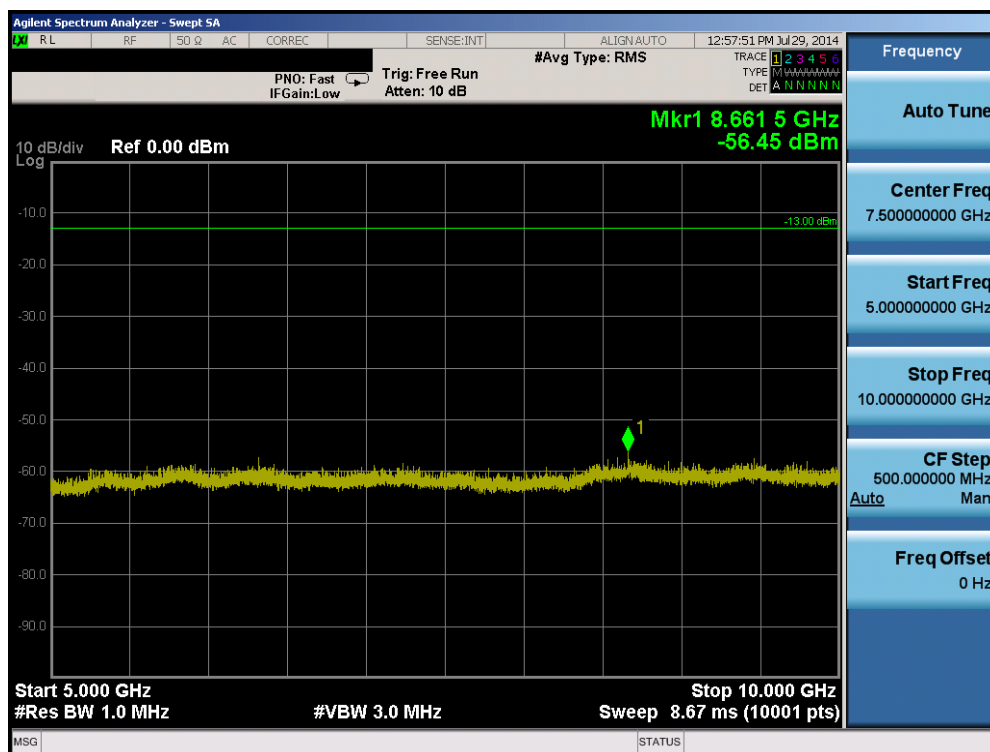
Plot 6-18. Conducted Spurious Plot (Band 17 – 5.0MHz QPSK – RB Size 1, RB Offset 0 – High Channel)
