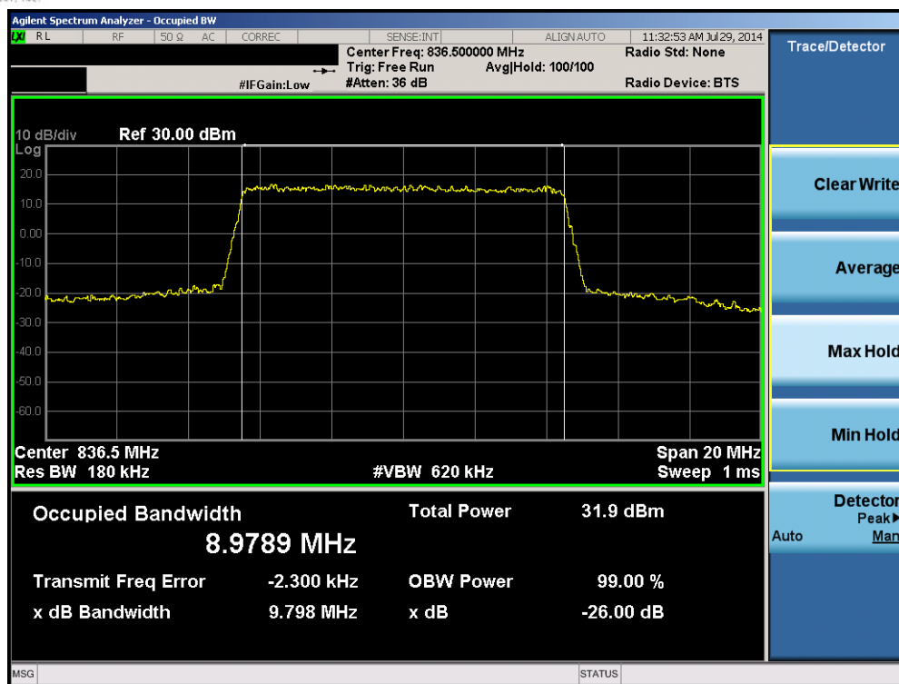
Plot 6-11. Occupied Bandwidth Plot (Band 5 – 10.0MHz QPSK – RB Size 50)
