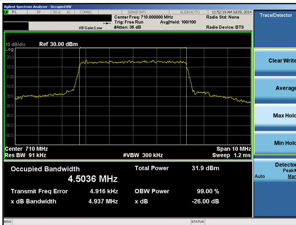
Plot 6-1. Occupied Bandwidth Plot (Band 17 – 5.0MHz QPSK – RB Size 25)
