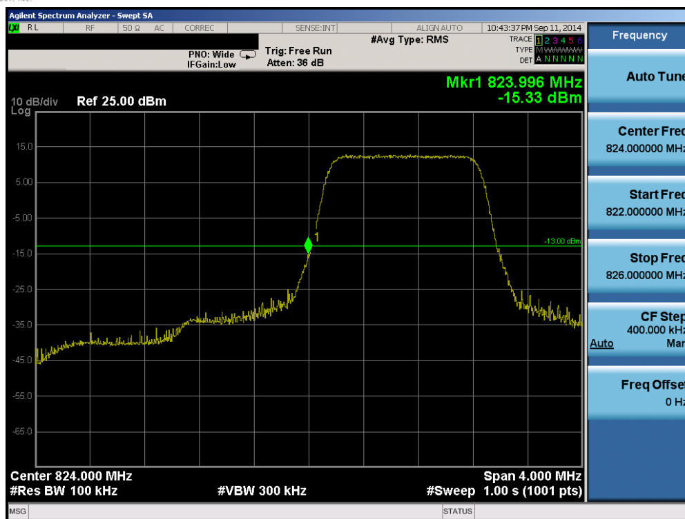
Plot 6-29. Lower Band Edge Plot (Band 5 – 1.4MHz QPSK – RB Size 6)
