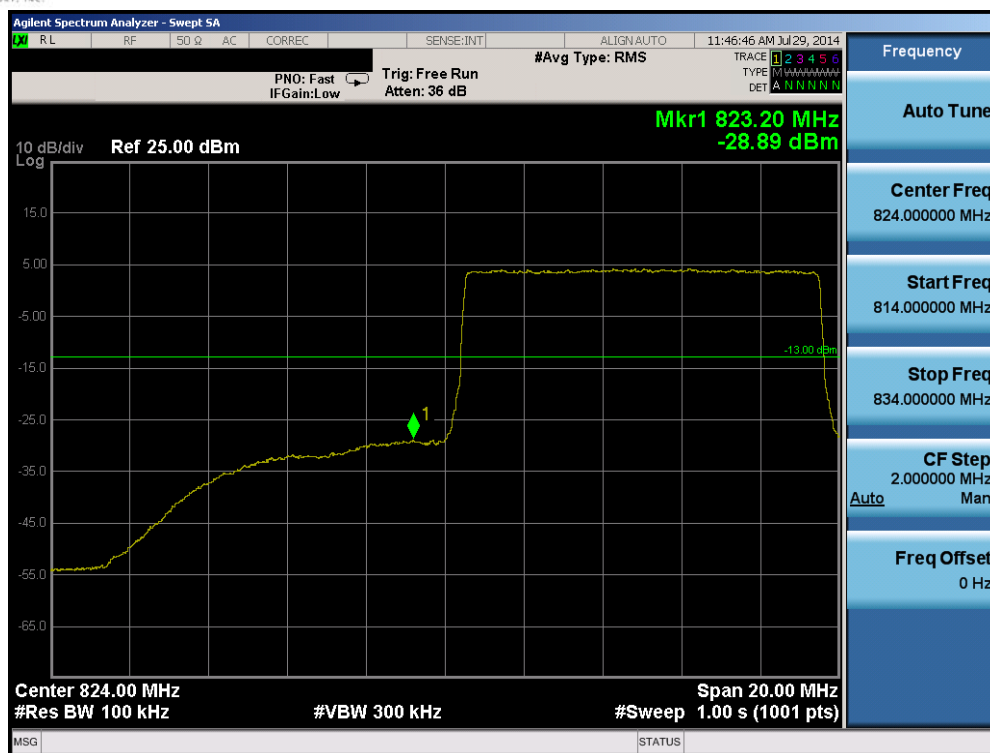
Plot 6-35. Lower Band Edge Plot (Band 5 – 10.0MHz QPSK – RB Size 50)
