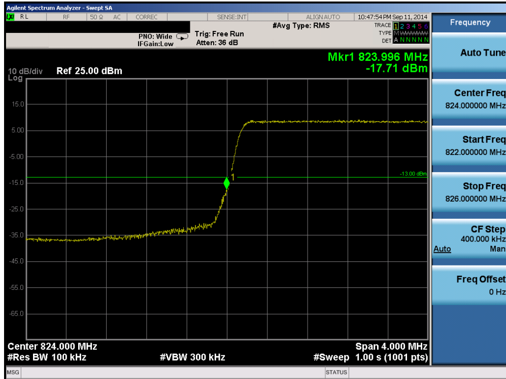
Plot 6-31. Lower Band Edge Plot (Band 5 – 3.0MHz QPSK – RB Size 15)
