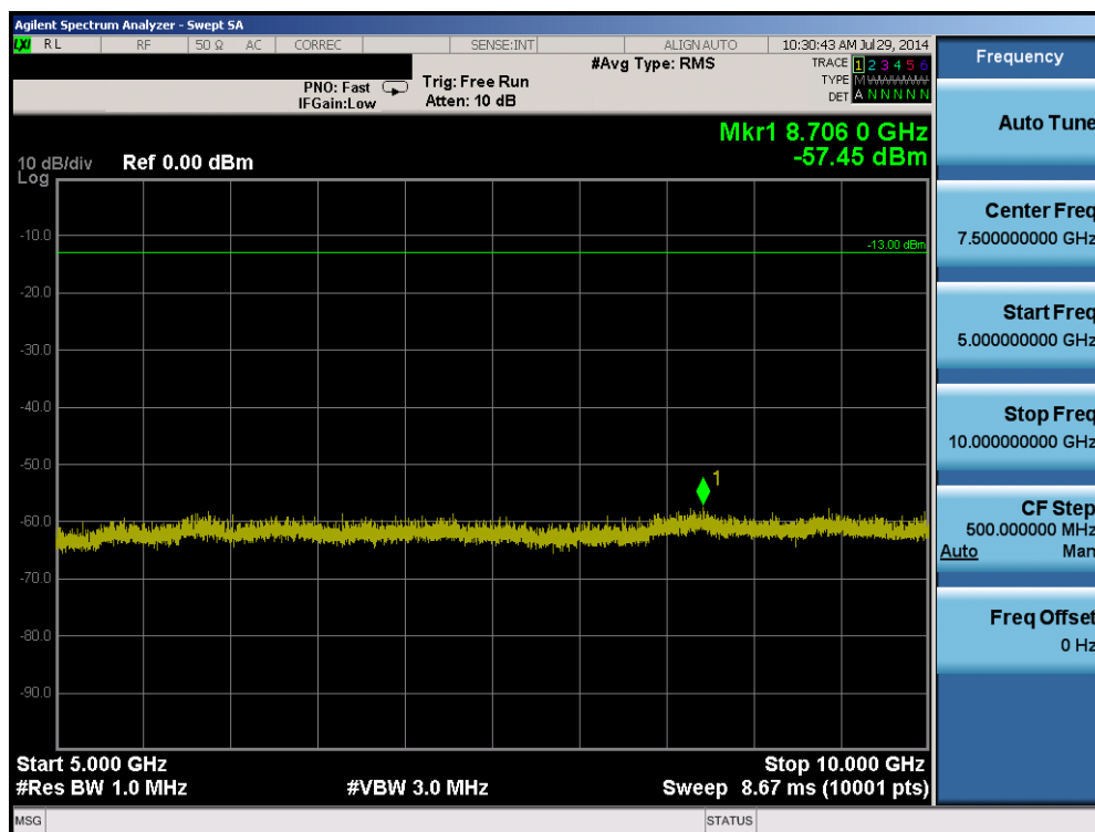
Plot 6-22. Conducted Spurious Plot (Band 5 – 5.0MHz QPSK – RB Size 1, RB Offset 0 – Mid Channel)
