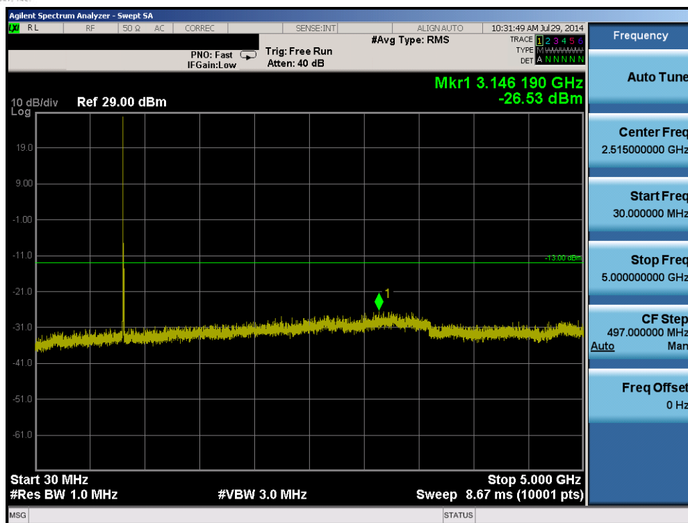
Plot 6-19. Conducted Spurious Plot (Band 5 – 5.0MHz QPSK – RB Size 1, RB Offset 0 – Low Channel)
