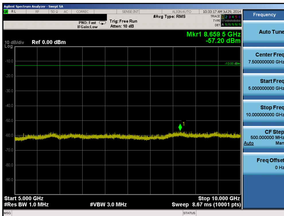
Plot 6-20. Conducted Spurious Plot (Band 5 – 5.0MHz QPSK – RB Size 1, RB Offset 0 – Low Channel)
