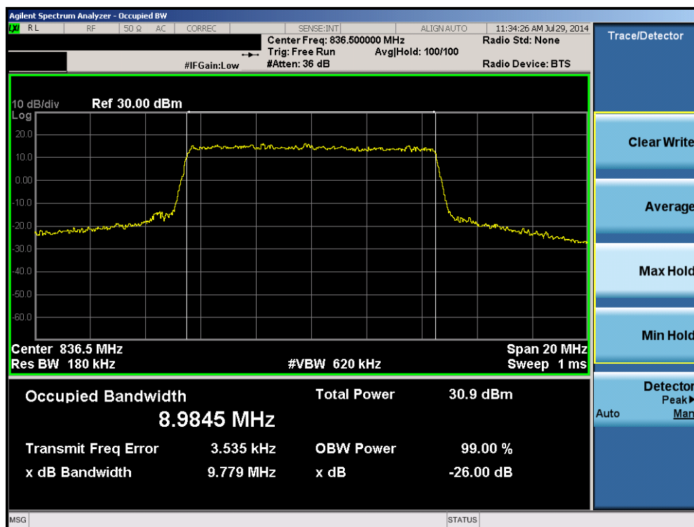
Plot 6-12. Occupied Bandwidth Plot (Band 5 – 10.0MHz 16-QAM – RB Size 50)
