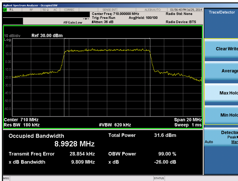
Plot 6-3. Occupied Bandwidth Plot (Band 17 – 10.0MHz QPSK – RB Size 50)
