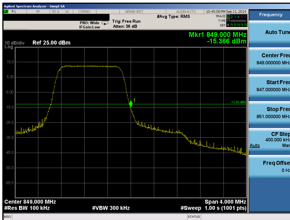
Plot 6-30. Upper Band Edge Plot (Band 5 – 1.4MHz QPSK – RB Size 6)
