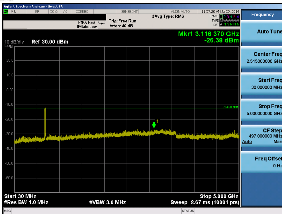
Plot 6-15. Conducted Spurious Plot (Band 17 – 5.0MHz QPSK – RB Size 1, RB Offset 0 – Mid Channel)
