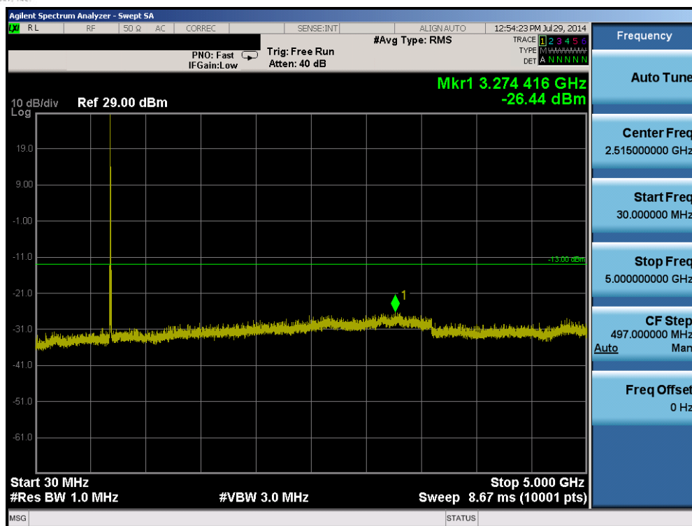
Plot 6-13. Conducted Spurious Plot (Band 17 – 5.0MHz QPSK – RB Size 1, RB Offset 0 – Low Channel)
