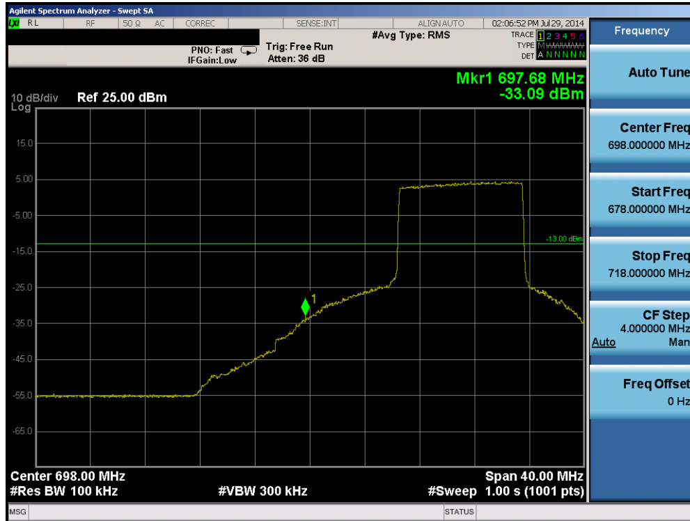
Plot 6-27. Lower Band Edge Plot (Band 17 – 10.0MHz QPSK – RB Size 50)
