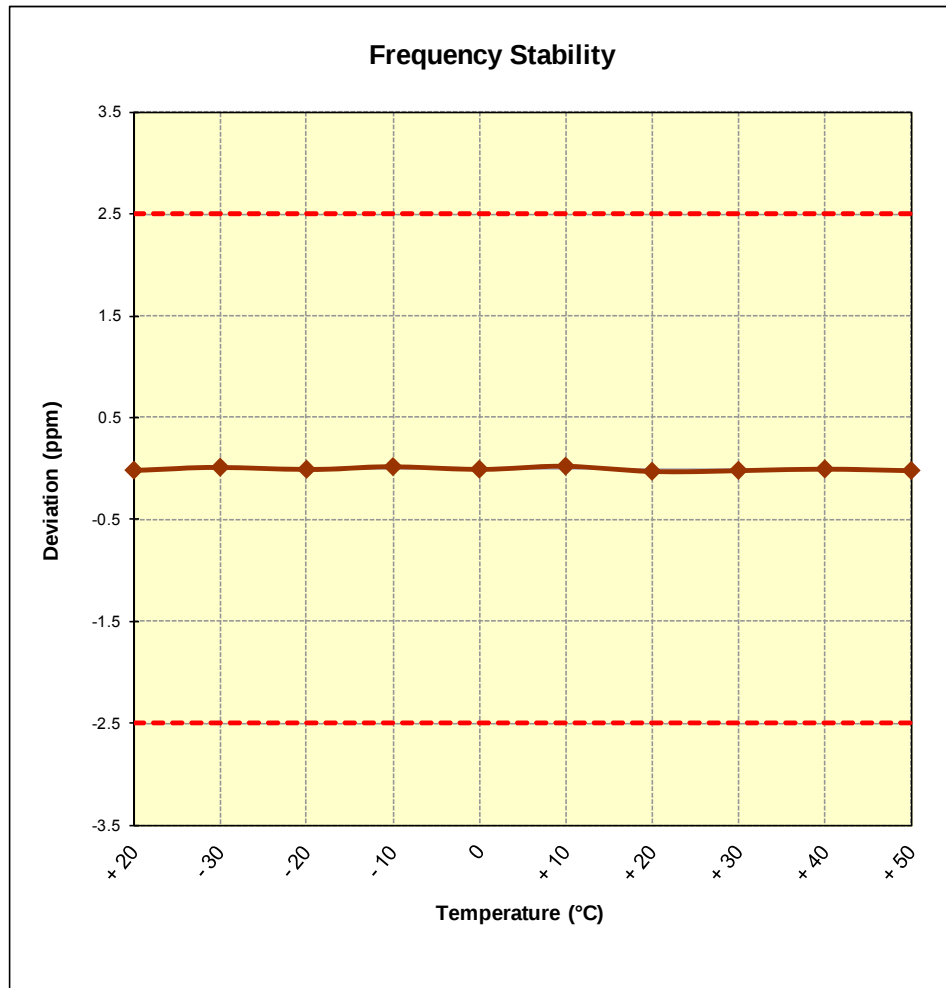
Figure 6-7. Frequency Stability Graph (Band 5)
