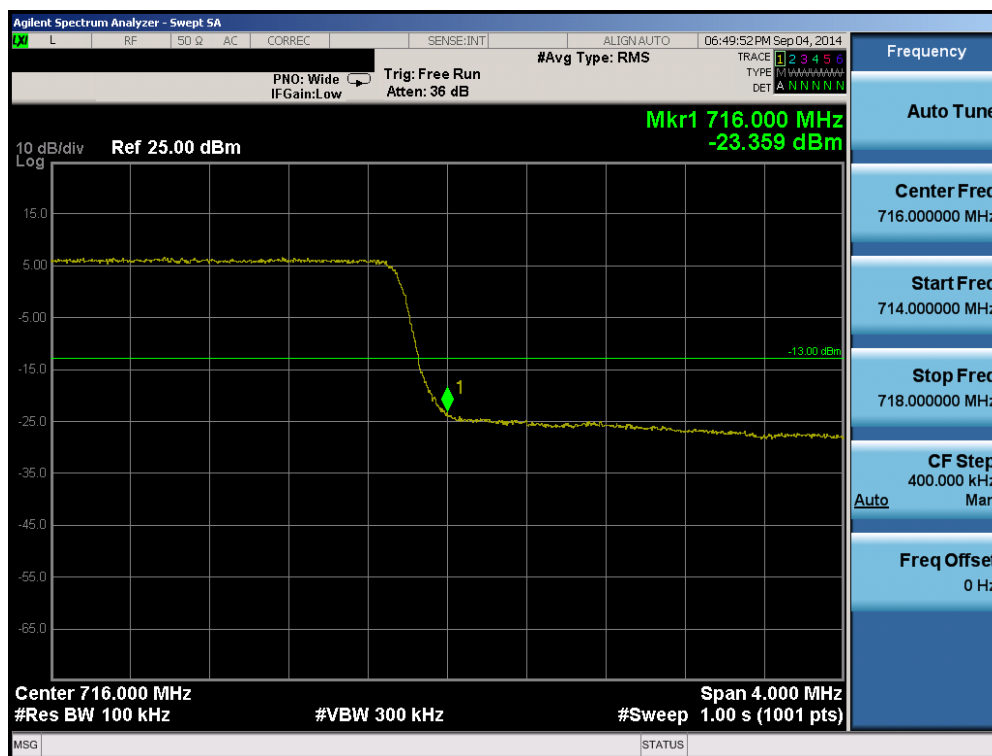
Plot 6-26. Upper Band Edge Plot (Band 17 – 5.0MHz QPSK – RB Size 25)
