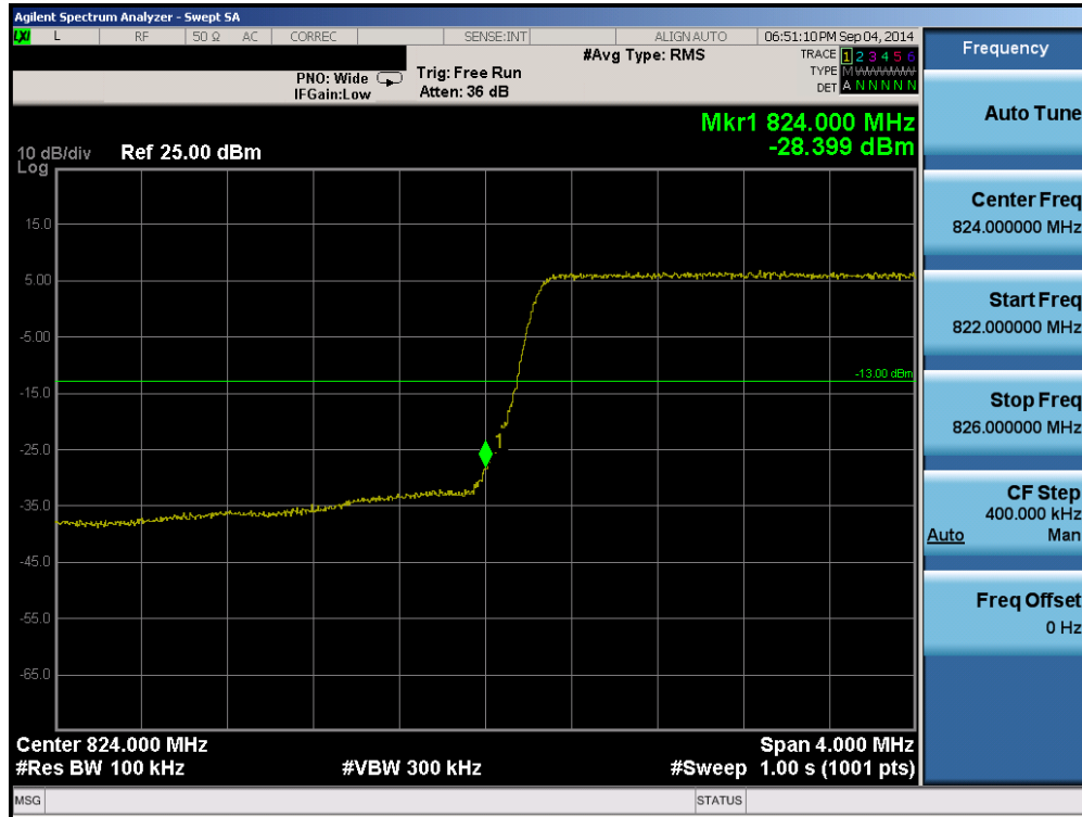
Plot 6-33. Lower Band Edge Plot (Band 5 – 5.0MHz QPSK – RB Size 25)
