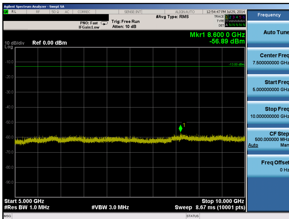
Plot 6-14. Conducted Spurious Plot (Band 17 – 5.0MHz QPSK – RB Size 1, RB Offset 0 – Low Channel)
