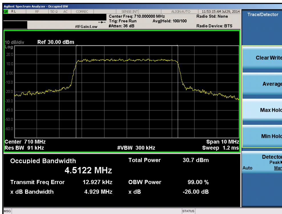
Plot 6-2. Occupied Bandwidth Plot (Band 17 – 5.0MHz 16-QAM – RB Size 25)
