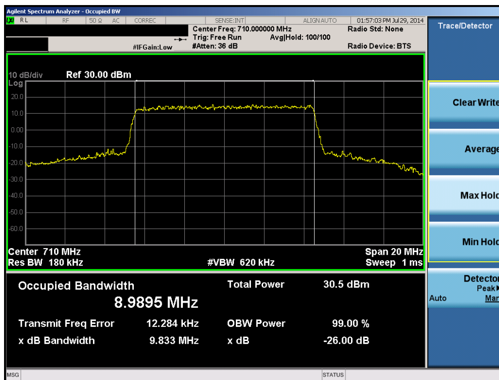
Plot 6-4. Occupied Bandwidth Plot (Band 17 – 10.0MHz 16-QAM – RB Size 50)
