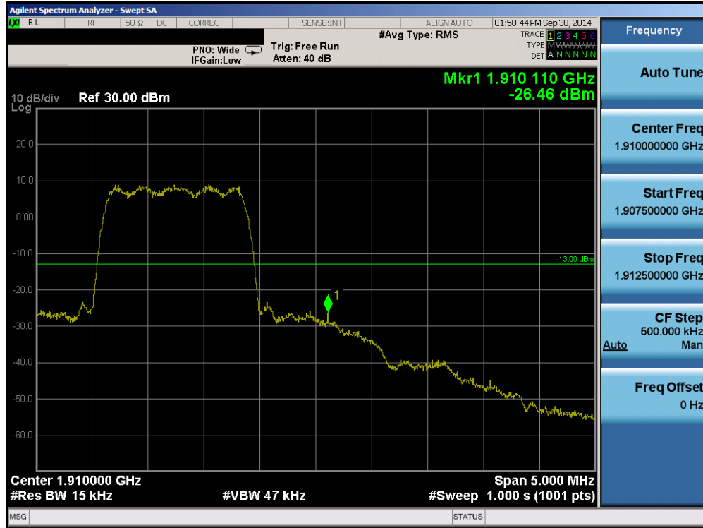
Plot 6-21. Band Edge Plot (PCS CDMA Mode – Ch. 1175)
