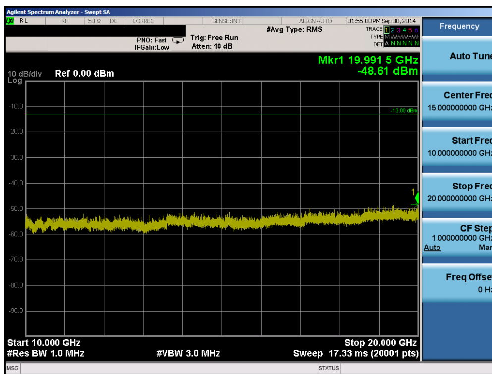
Plot 6-12. Conducted Spurious Plot (PCS CDMA Mode – Ch. 600)
