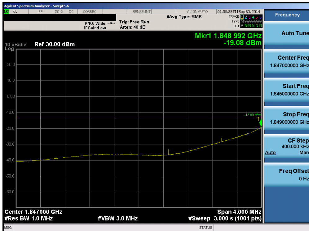
Plot 6-20. 4MHz Span Plot (PCS CDMA Mode – Ch. 25)
