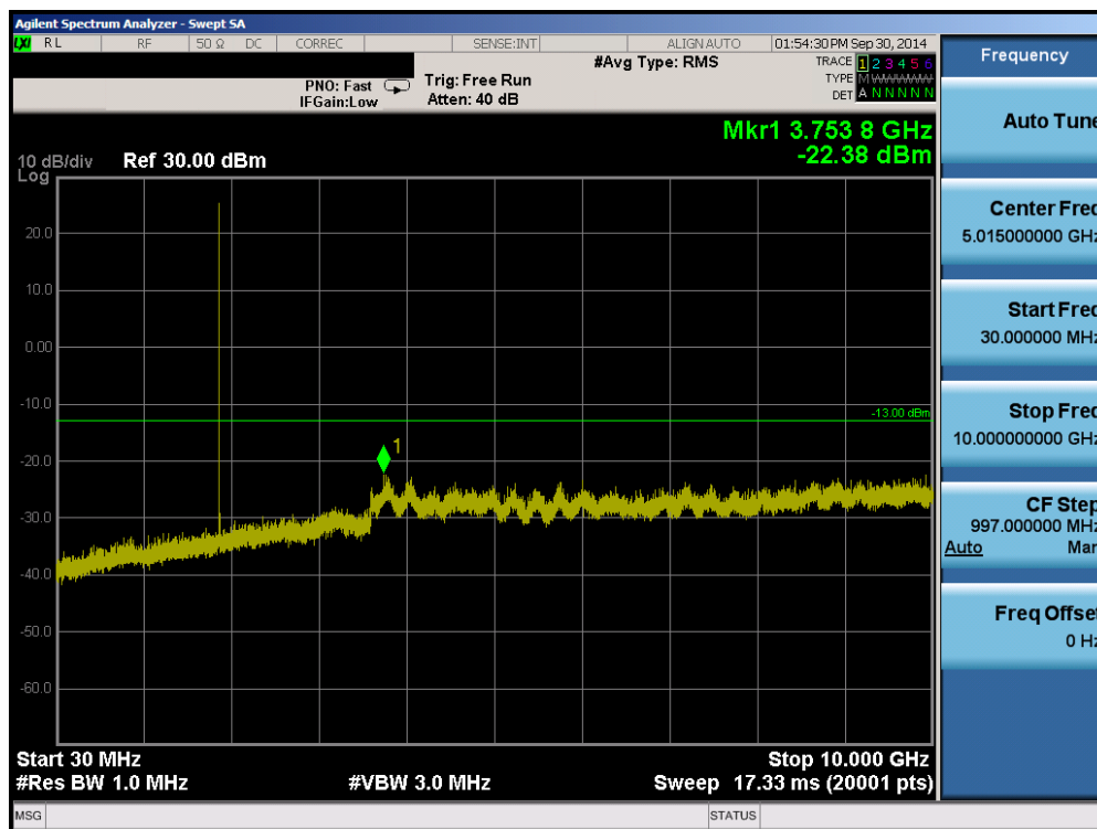
Plot 6-11. Conducted Spurious Plot (PCS CDMA Mode – Ch. 600)
