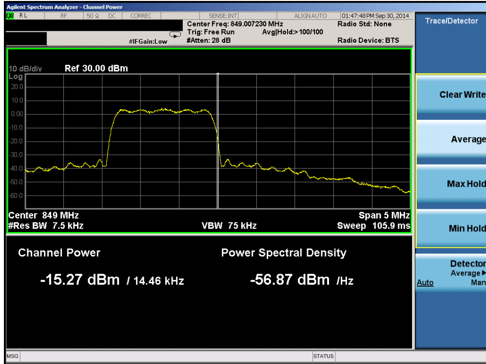
Plot 6-17. Band Edge Plot (Cellular CDMA Mode – Ch. 777)
