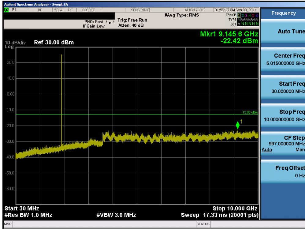
Plot 6-13. Conducted Spurious Plot (PCS CDMA Mode – Ch. 1175)
