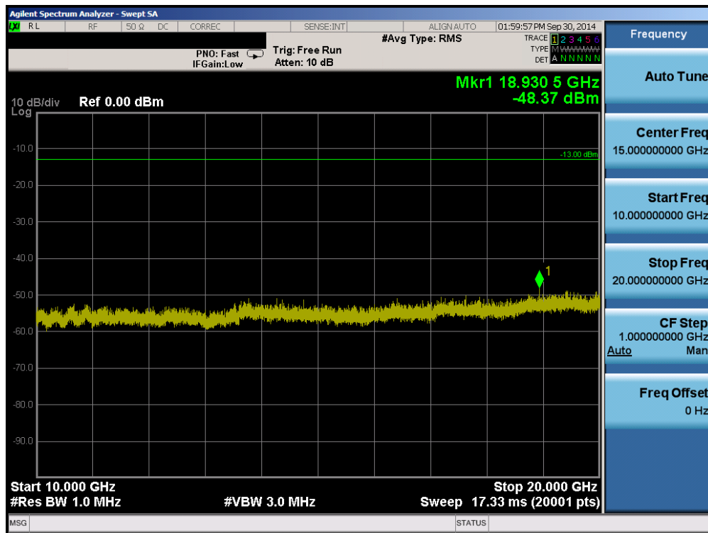
Plot 6-14. Conducted Spurious Plot (PCS CDMA Mode – Ch. 1175)
