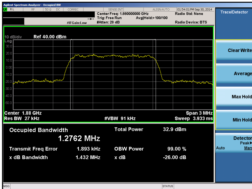
Plot 6-2. Occupied Bandwidth Plot (PCS CDMA Mode – Ch. 600)
