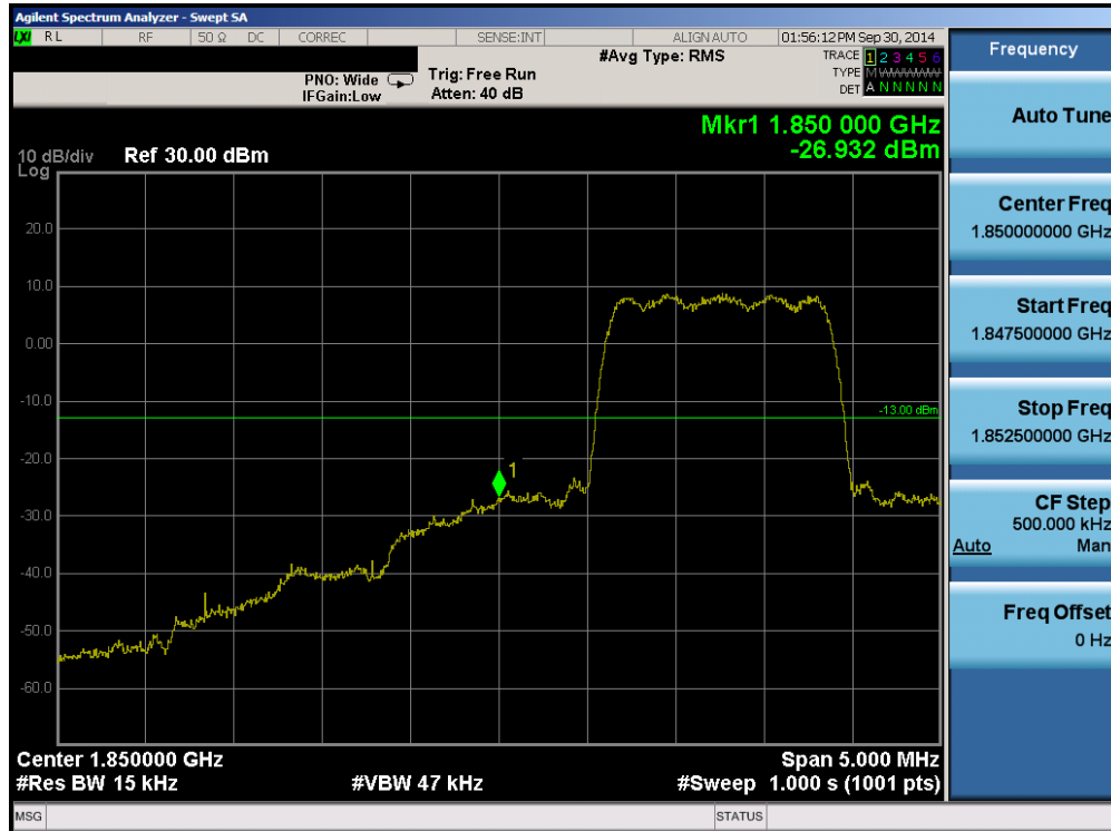
Plot 6-19. Band Edge Plot (PCS CDMA Mode – Ch. 25)
