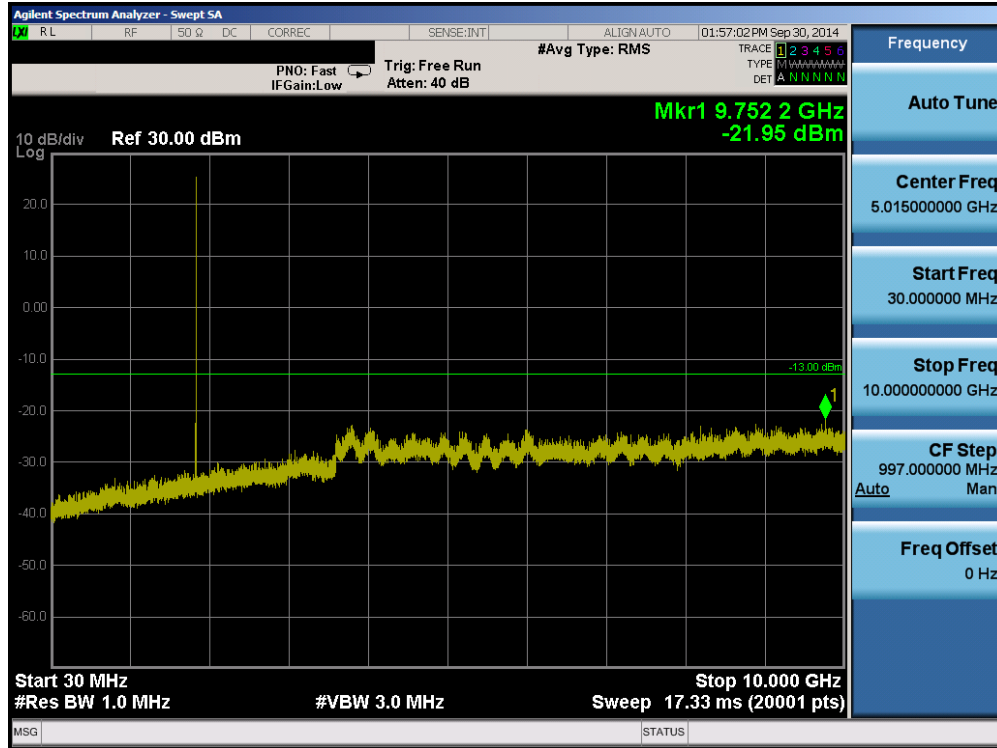
Plot 6-9. Conducted Spurious Plot (PCS CDMA Mode – Ch. 25)
