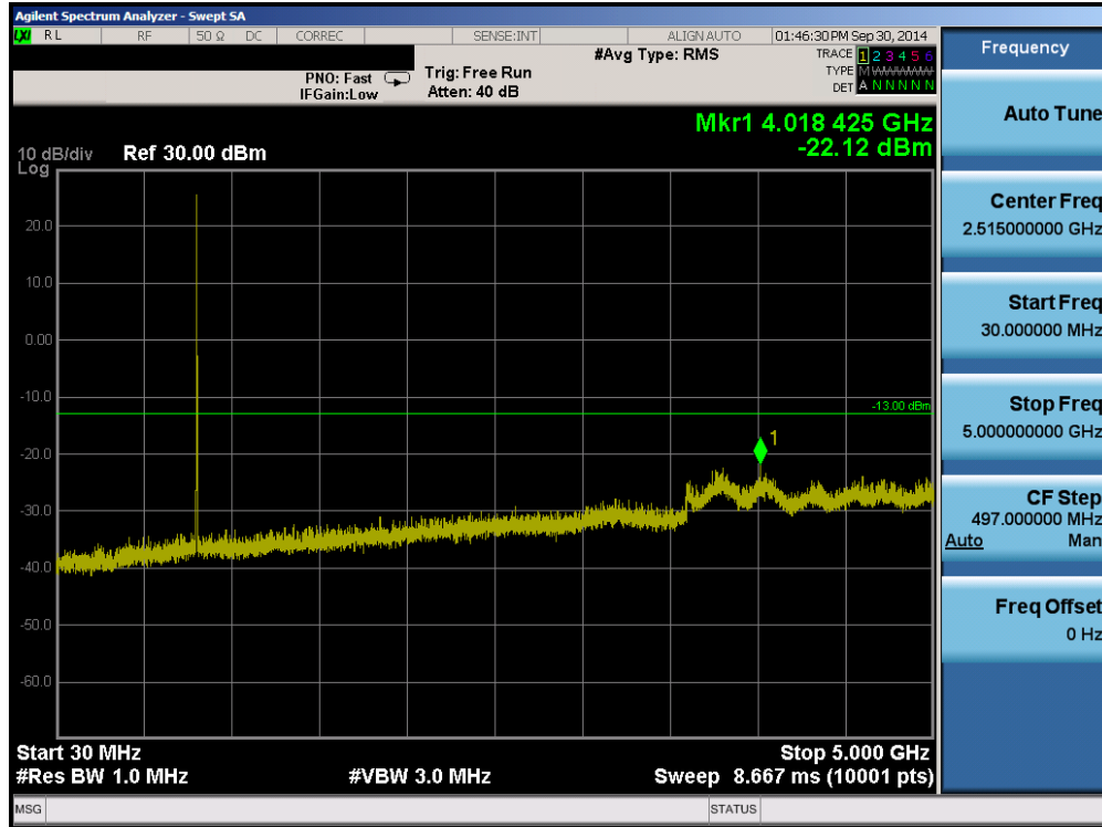
Plot 6-3. Conducted Spurious Plot (Cellular CDMA Mode – Ch. 1013)
