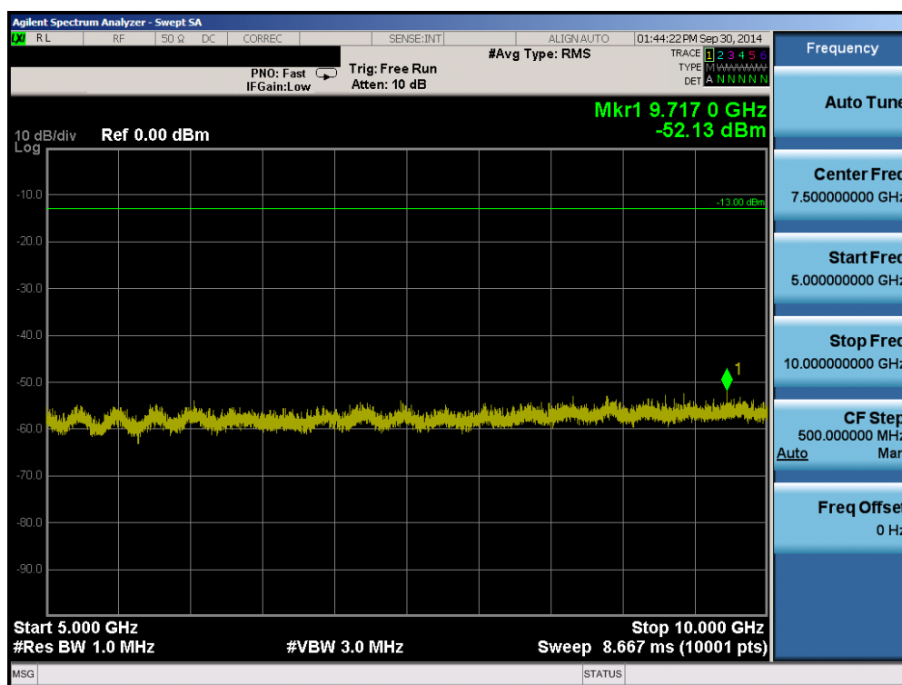
Plot 6-6. Conducted Spurious Plot (Cellular CDMA Mode – Ch. 384)
