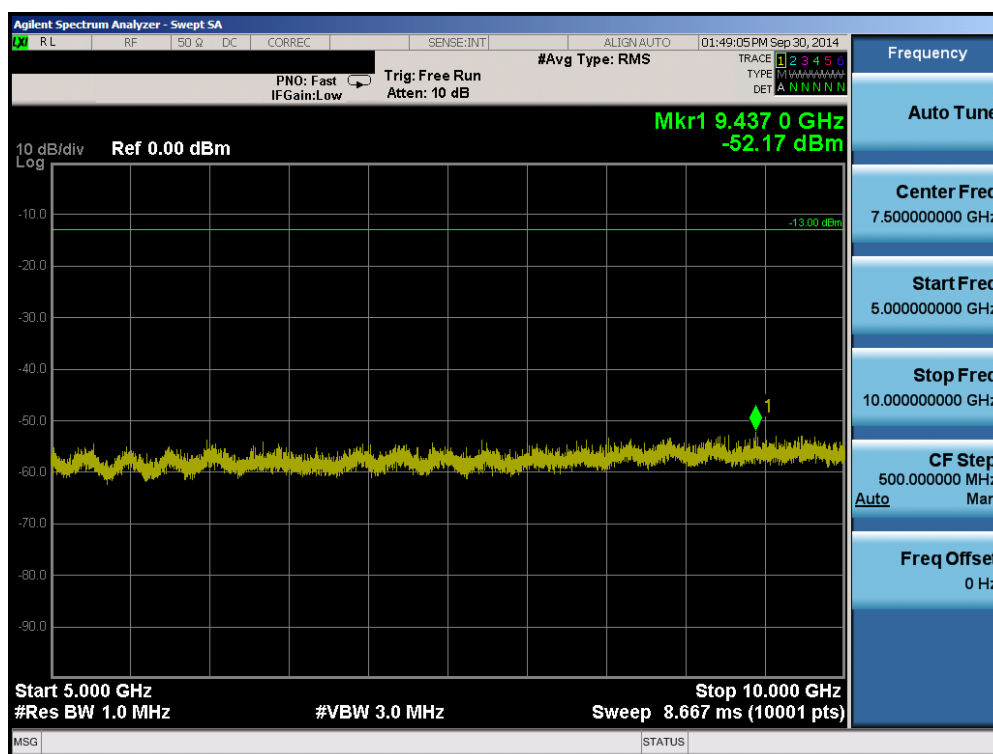
Plot 6-8. Conducted Spurious Plot (Cellular CDMA Mode – Ch. 777)
