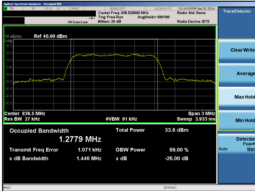
Plot 6-1. Occupied Bandwidth Plot (Cellular CDMA Mode – Ch. 384)
