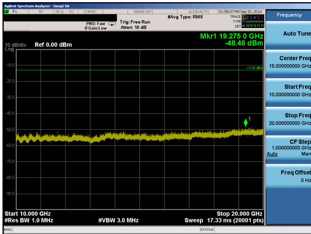
Plot 6-10. Conducted Spurious Plot (PCS CDMA Mode – Ch. 25)
