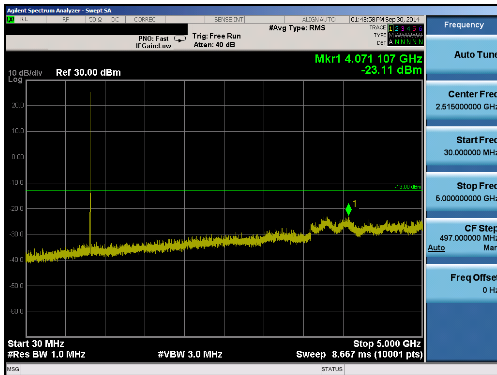
Plot 6-5. Conducted Spurious Plot (Cellular CDMA Mode – Ch. 384)
