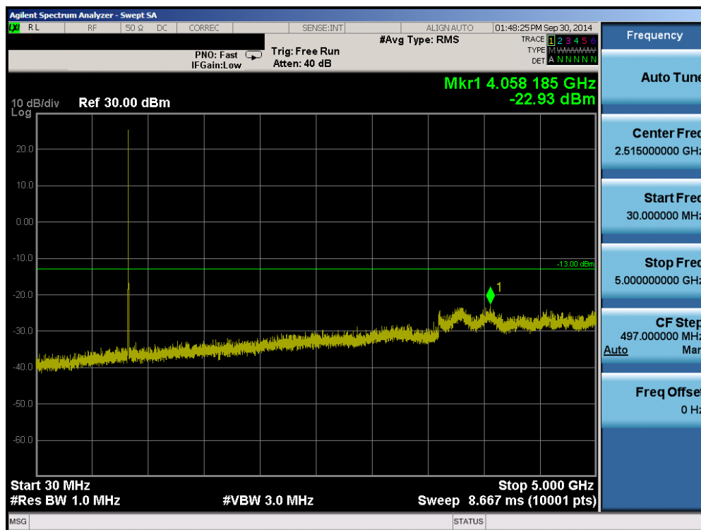
Plot 6-7. Conducted Spurious Plot (Cellular CDMA Mode – Ch. 777)
