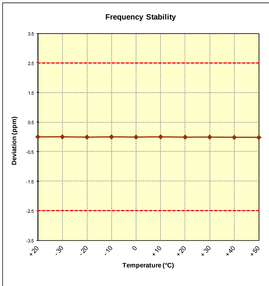
Figure 6-7. Frequency Stability Graph (Cellular CDMA Mode – Ch. 384)
