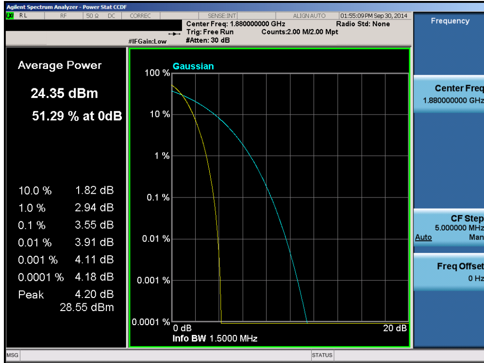
Plot 6-23. Peak-Average Ratio Plot (PCS CDMA Mode – Ch. 600)
