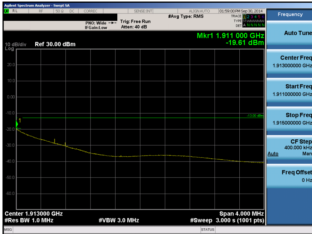
Plot 6-22. 4MHz Span Plot (PCS CDMA Mode – Ch. 1175)
