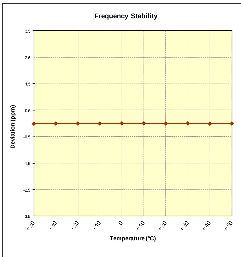
Figure 6-8. Frequency Stability Graph (PCS CDMA Mode – Ch. 600)
