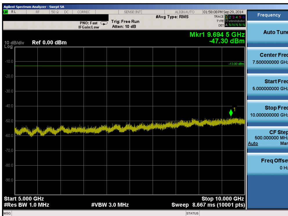
Plot 6-50. Conducted Spurious Plot (Band 5 – 10.0MHz OPSK – RB Size 1, RB Offset 0 – Mid Channel)
