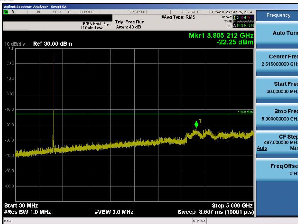
Plot 6-47. Conducted Spurious Plot (Band 5 – 10.0MHz QPSK – RB Size 1, RB Offset 0– Low Channel)
