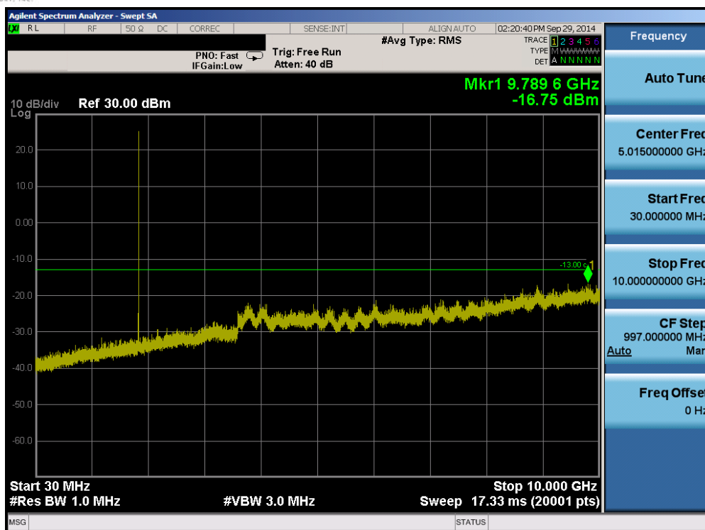
Plot 6-59. Conducted Spurious Plot (Band 2 – 5.0MHz QPSK – RB Size 1, RB Offset 0 – Low Channel)
