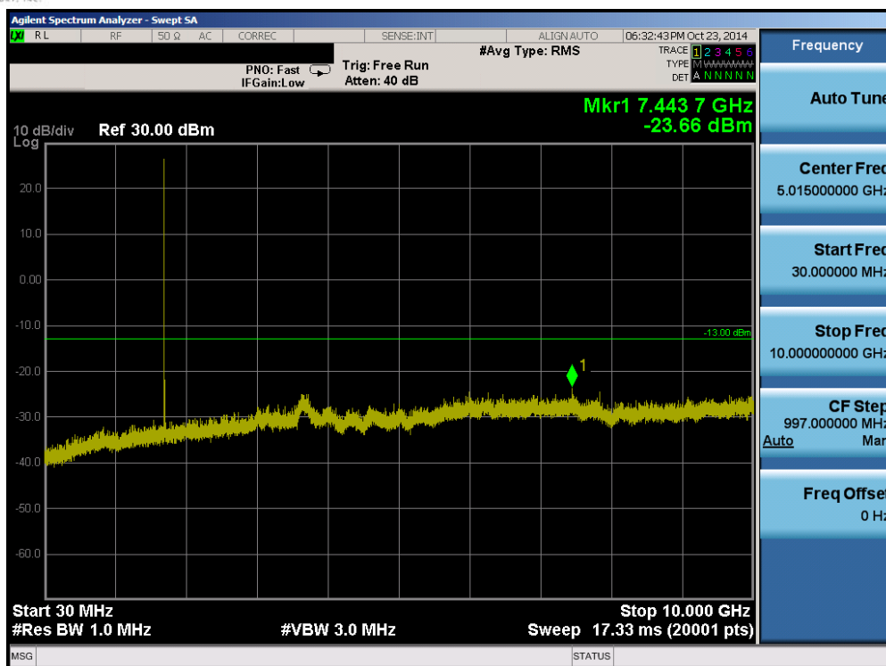
Plot 6-53. Conducted Spurious Plot (Band 4 – 3.0MHz QPSK – RB Size 1, RB Offset 0 – Low Channel)
