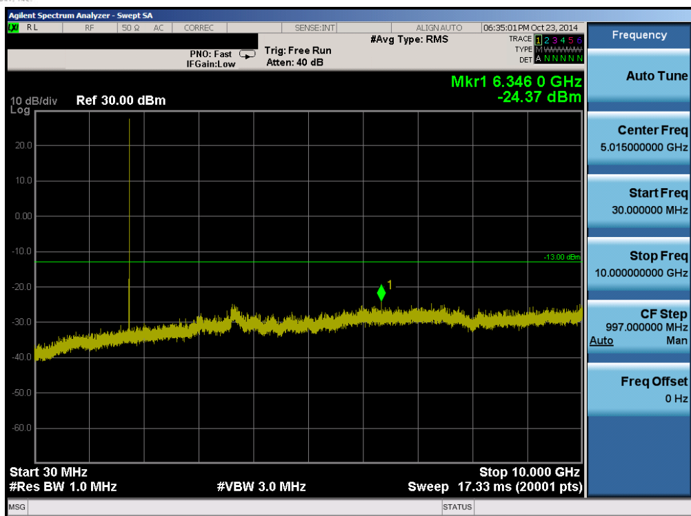
Plot 6-57. Conducted Spurious Plot (Band 4 – 3.0MHz QPSK – RB Size 1, RB Offset 0 – High Channel)
