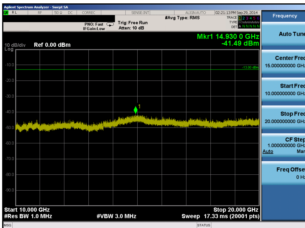
Plot 6-60. Conducted Spurious Plot (Band 2 – 5.0MHz QPSK – RB Size 1, RB Offset 0 – Low Channel)
