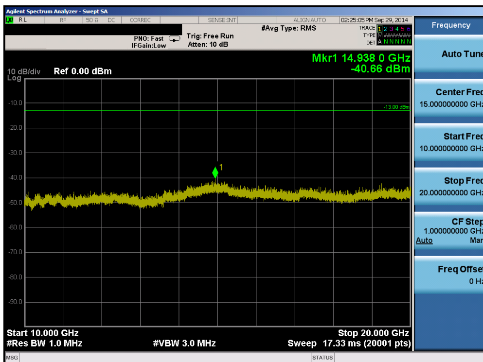
Plot 6-64. Conducted Spurious Plot (Band 2 – 5.0MHz QPSK – RB Size 1, RB Offset 0 – High Channel)
