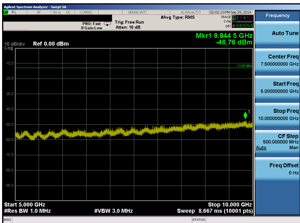
Plot 6-52. Conducted Spurious Plot (Band 5 – 10.0MHz QPSK – RB Size 1, RB Offset 0 – High Channel)
