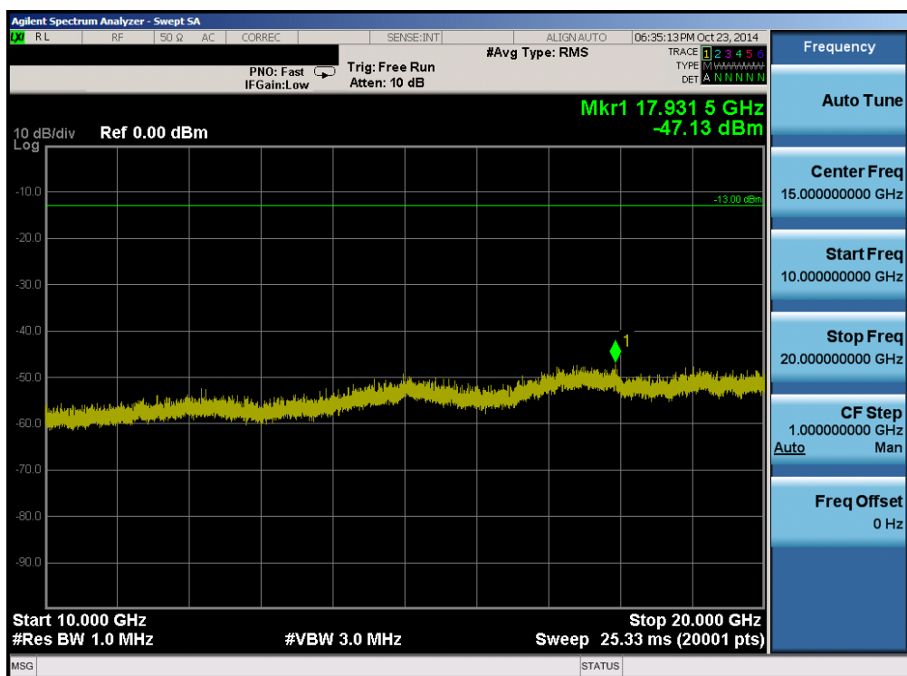
Plot 6-58. Conducted Spurious Plot (Band 4 – 3.0MHz QPSK – RB Size 1, RB Offset 0 – High Channel)
