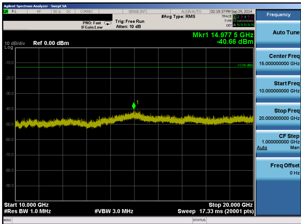
Plot 6-62. Conducted Spurious Plot (Band 2 – 5.0MHz QPSK – RB Size 1, RB Offset 0 – Mid Channel)
