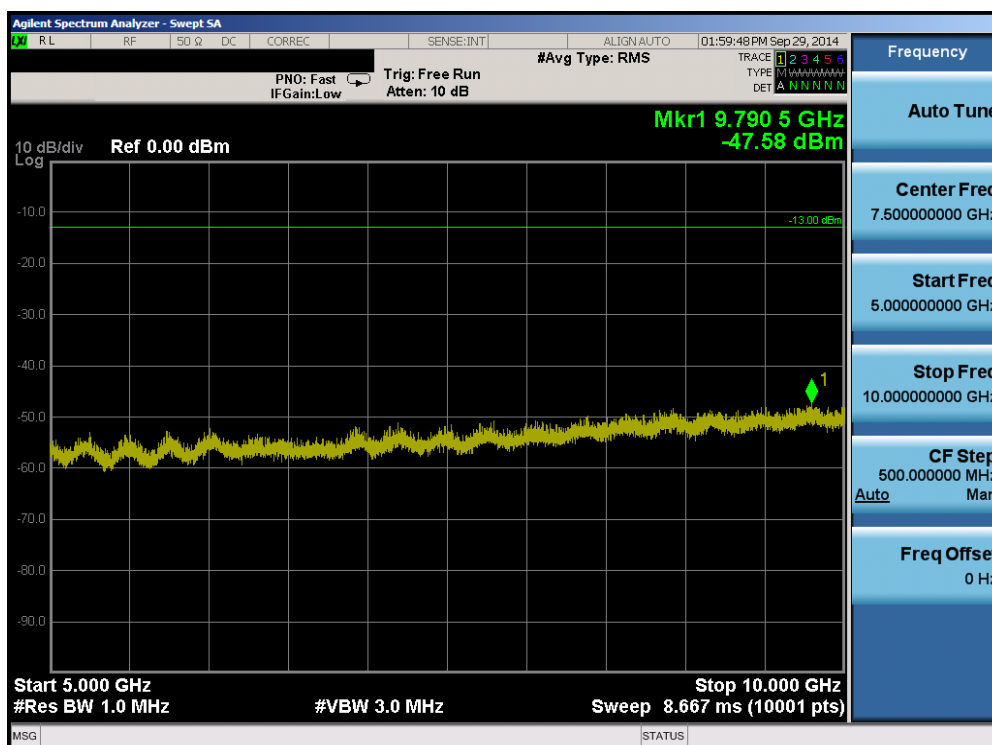
Plot 6-48. Conducted Spurious Plot (Band 5 – 10.0MHz QPSK – RB Size 1, RB Offset 0 – Low Channel)
