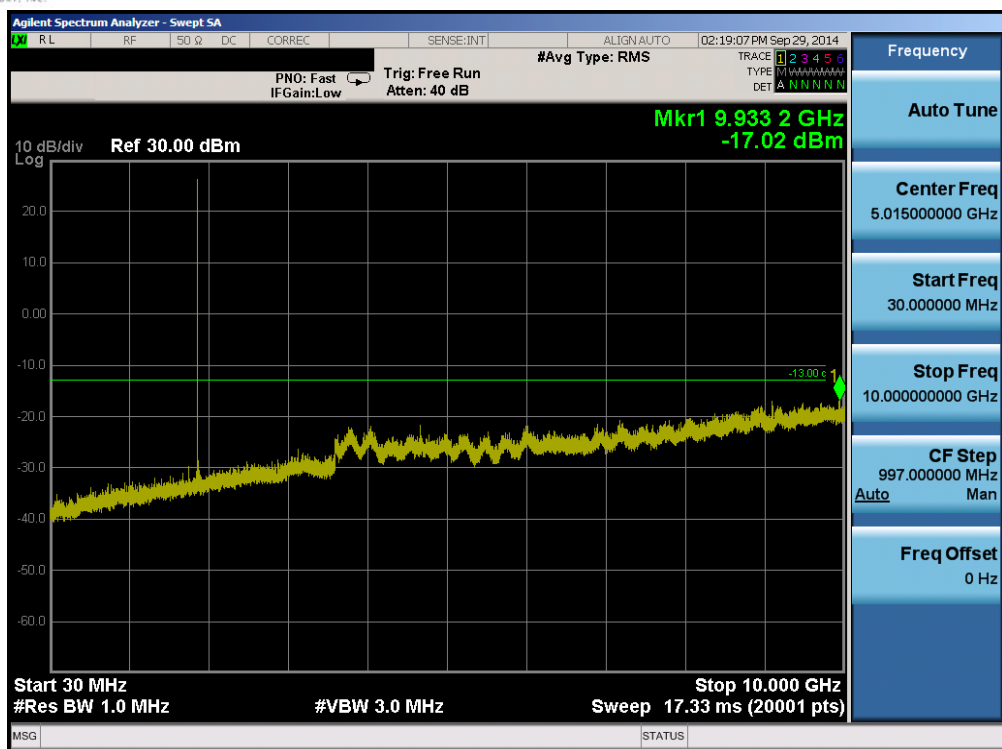
Plot 6-61. Conducted Spurious Plot (Band 2 – 5.0MHz QPSK – RB Size 1, RB Offset 0 – Mid Channel)
