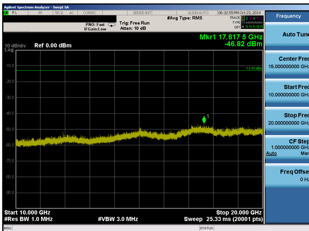
Plot 6-54. Conducted Spurious Plot (Band 4 – 3.0MHz QPSK – RB Size 1, RB Offset 0 – Low Channel)
