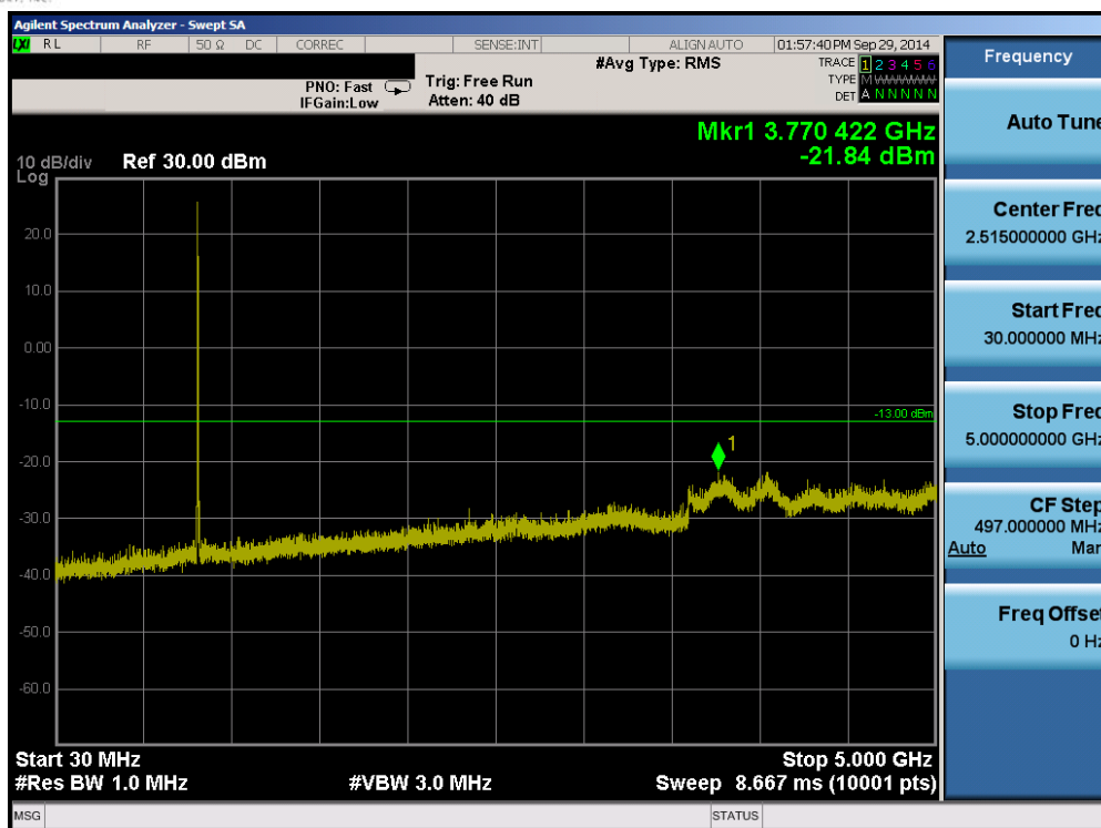
Plot 6-49. Conducted Spurious Plot (Band 5 – 10.0MHz QPSK – RB Size 1, RB Offset 0 – Mid Channel)
