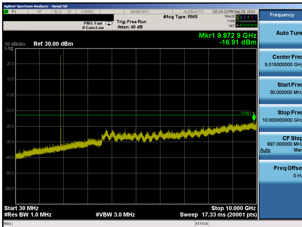
Plot 6-63. Conducted Spurious Plot (Band 2 – 5.0MHz QPSK – RB Size 1, RB Offset 0 – High Channel)
