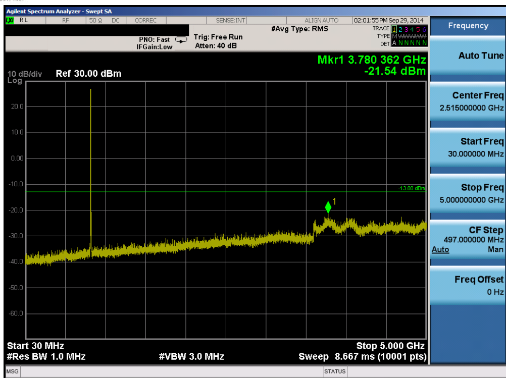
Plot 6-51. Conducted Spurious Plot (Band 5 – 10.0MHz QPSK – RB Size 1, RB Offset 0 – High Channel)
