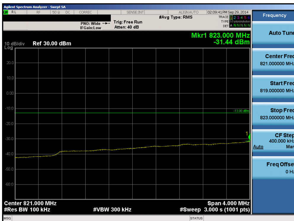
Plot 6-88. Lower Extended Band Edge Plot (Band 5 – 5.0MHz OPSK – RB Size 25)
