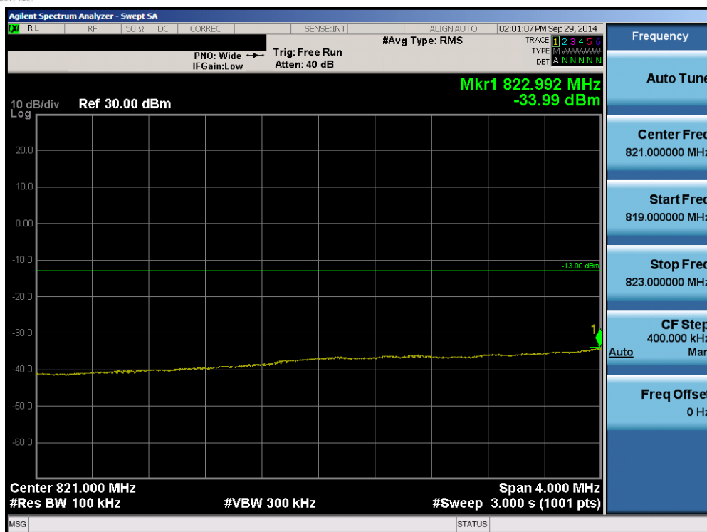
Plot 6-91. Lower Extended Band Edge Plot (Band 5 – 10.0MHz QPSK – RB Size 50)
