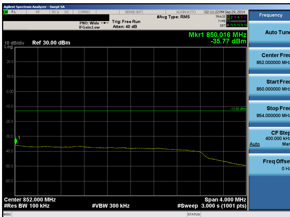
Plot 6-90. Upper Extended Band Edge Plot (Band 5 – 5.0MHz OPSK – RB Size 25)
