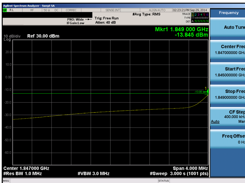
Plot 6-126. Lower Extended Band Edge Plot (Band 2 – 5.0MHz OPSK – RB Size 25)
