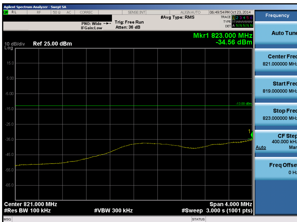
Plot 6-80. Lower Extended Band Edge Plot (Band 5 – 1.4MHz QPSK – RB Size 6)
