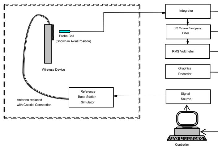
Figure 5-13 Audio Magnetic Field Test Setup
