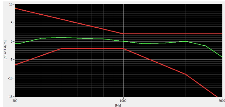
Figure 7-1 Axial Frequency Response
