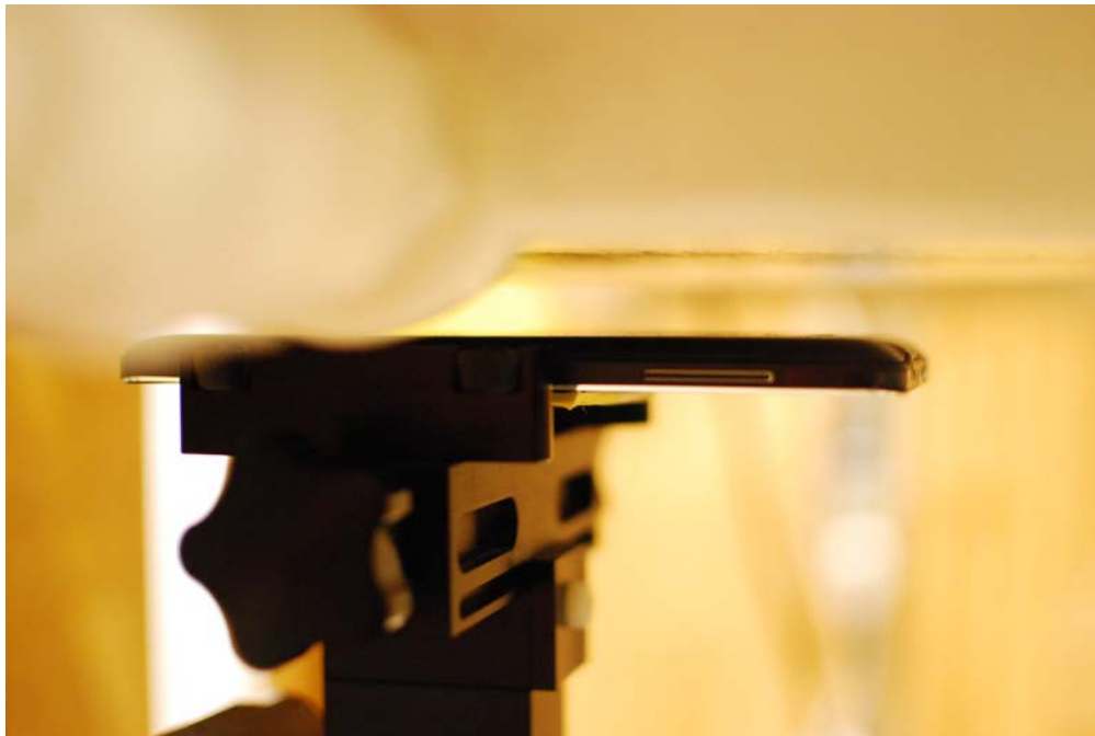
SAR Test Setup Photo 8 – Back Side at 1.5 cm, Wireless Charging Cover
