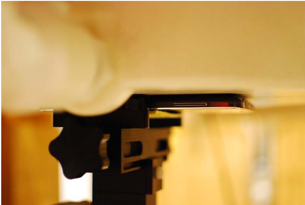
SAR Test Setup Photo 12 – Back Side at 0.0 cm, Wireless Charging Cover
