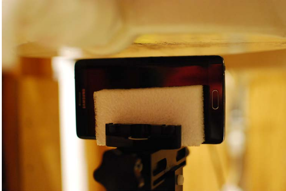
SAR Test Setup Photo 23 – Right Edge at 1.0 cm, Standard Back Cover
