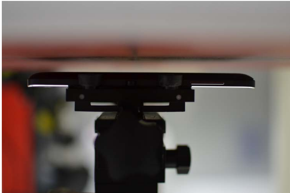
SAR Test Setup Photo 10 – Back Side at 1.0 cm, Wireless Charging Cover
