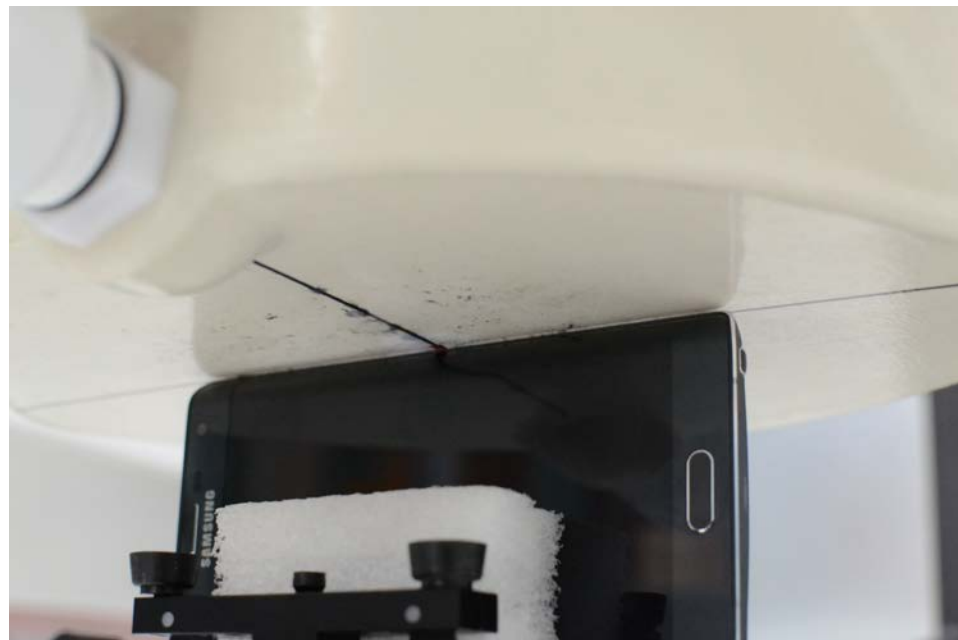
SAR Test Setup Photo 24 – Right Edge at 0.0 cm, Standard Back Cover
