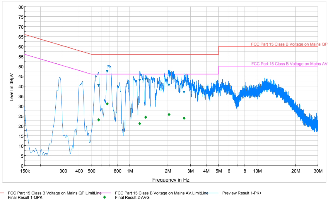
Plot 6-8. Line-Conducted Test Plot (L1)
