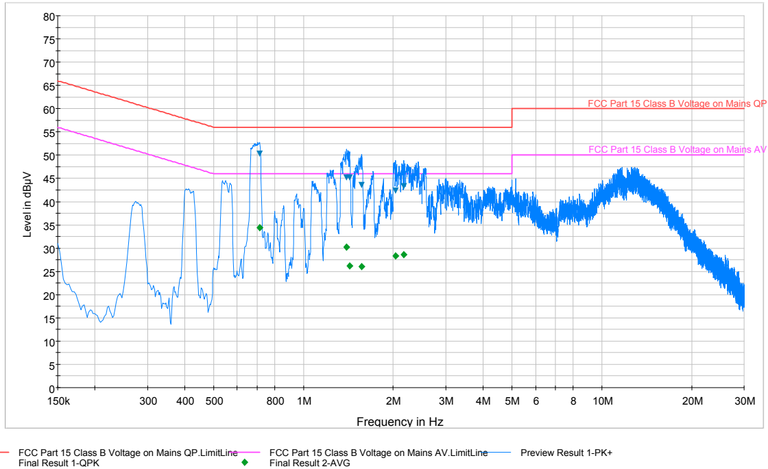
Plot 6-9. Line-Conducted Test Plot (N)
