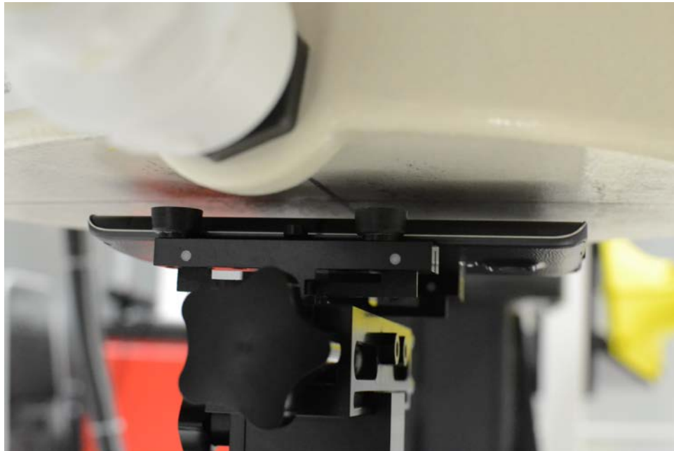
SAR Test Setup Photo 14 – Front Side at 1.0 cm
