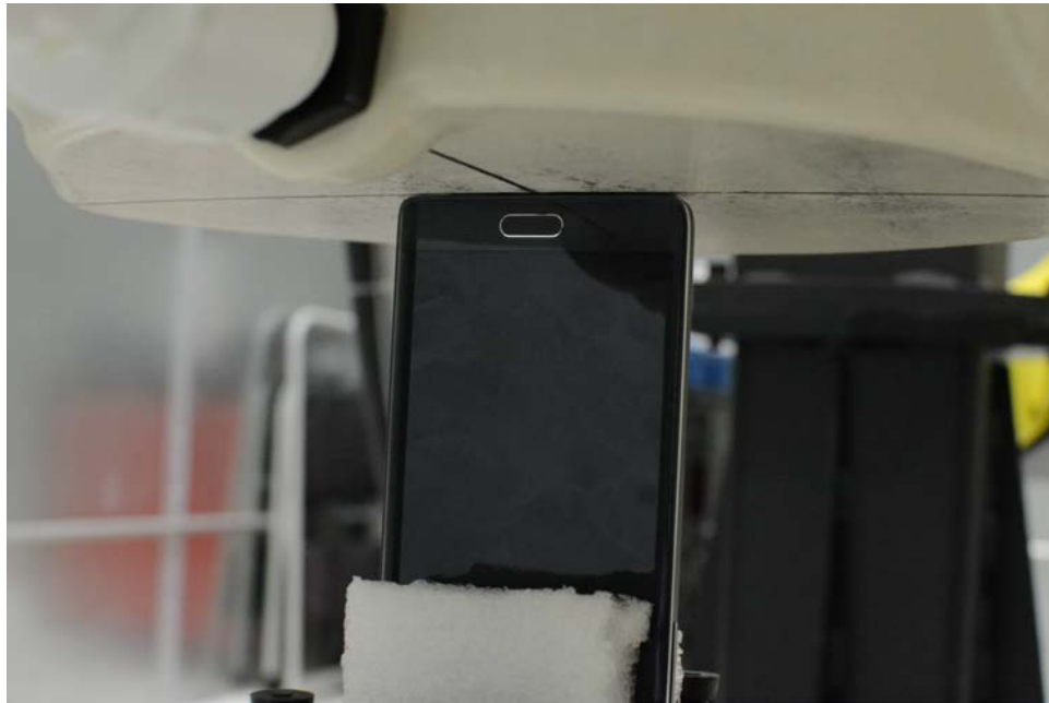
SAR Test Setup Photo 25 – Bottom Edge at 0.0 cm
