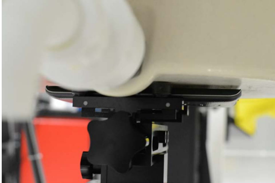
SAR Test Setup Photo 17 – Front Side at 0.3 cm with Wireless Charging Cover
