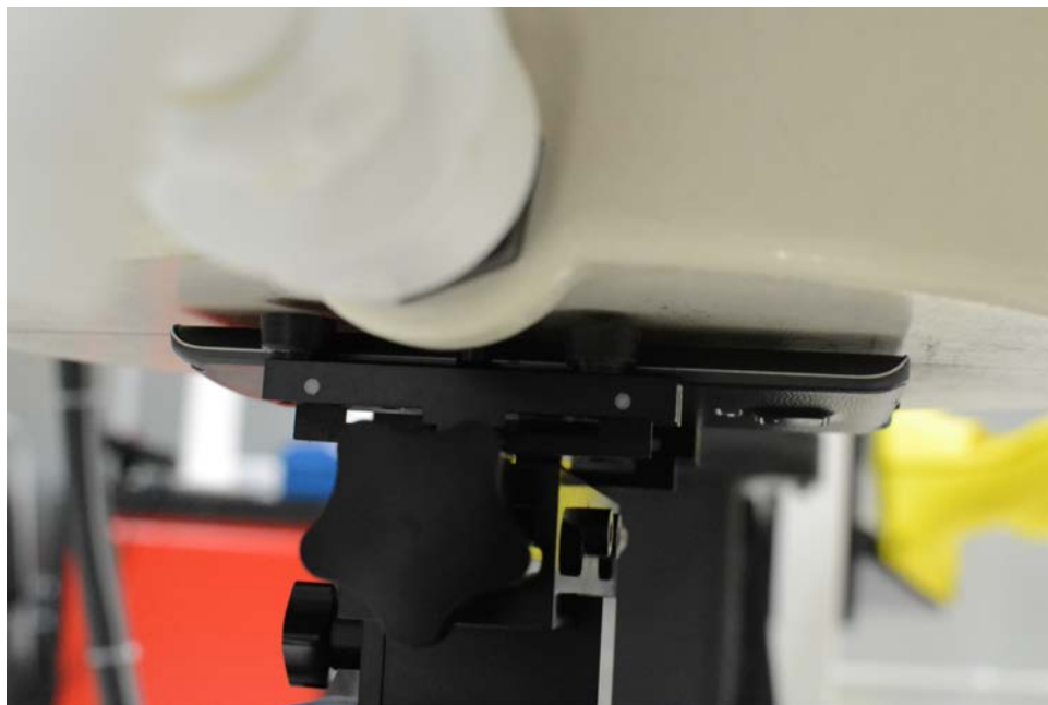
SAR Test Setup Photo 16 – Front Side at 0.3 cm
