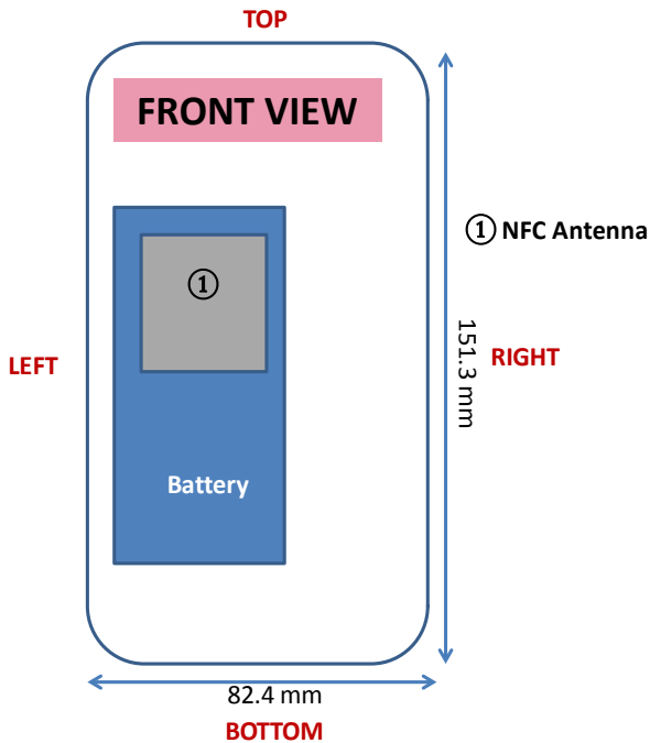
Figure F-2 NFC Antenna Location
