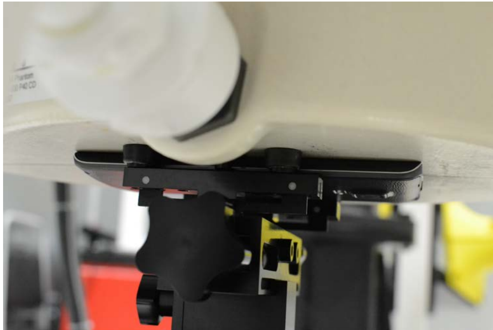
SAR Test Setup Photo 18 – Front Side at 0.0 cm
