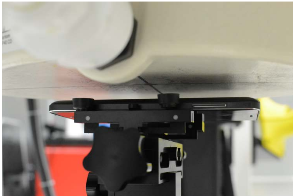
SAR Test Setup Photo 8 – Back Side at 1.5 cm with Wireless Charging Cover
