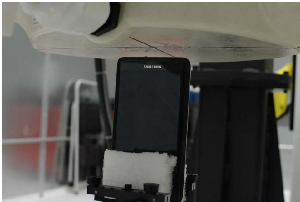
SAR Test Setup Photo 20 – Top Edge at 1.0 cm
