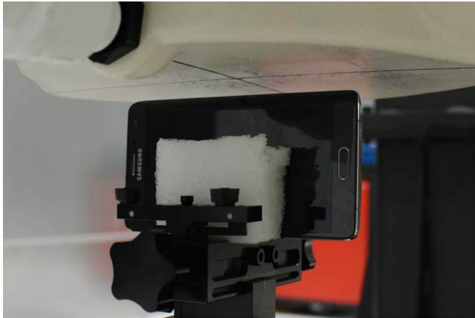
SAR Test Setup Photo 27 – Right Edge at 1.0 cm
