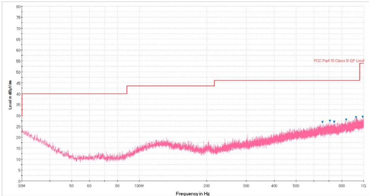
Plot 6-91. Radiated Spurious Plot below 1GHz (Pol. H)
