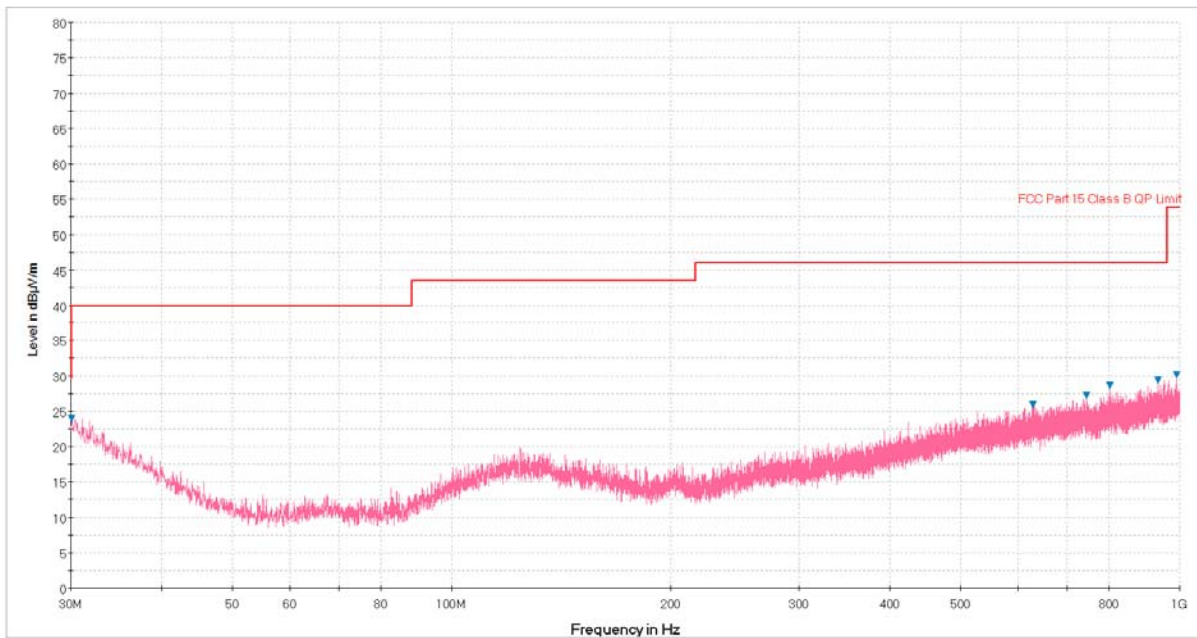
Plot 6-92. Radiated Spurious Plot below 1GHz (Pol. V)
