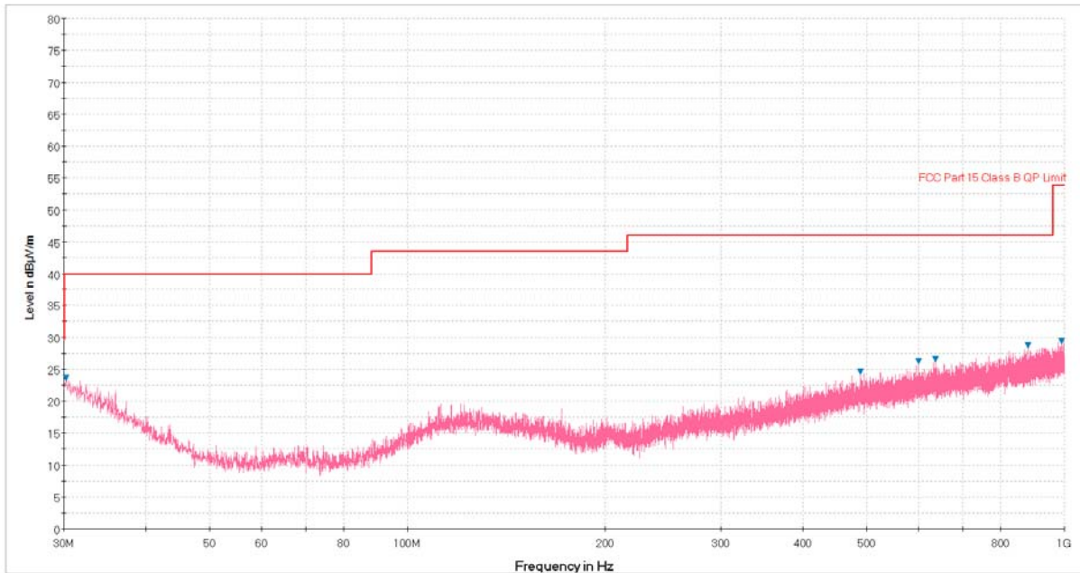
Plot 6-89. Radiated Spurious Plot below 1GHz (Pol. H)
