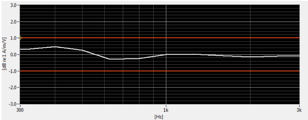
Figure 7-5 Helmholtz Coil Validation for Frequency Response
