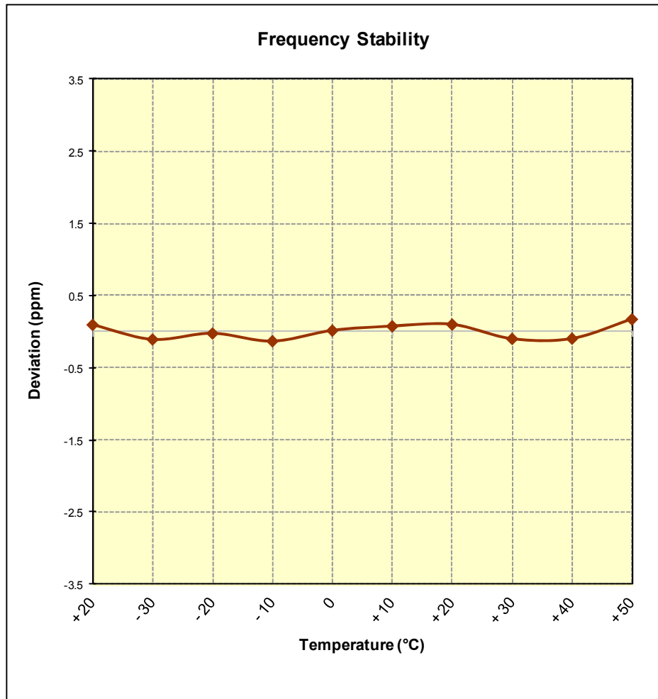
Figure 6-11. Frequency Stability Graph (PCS CDMA Mode – Ch. 600)
