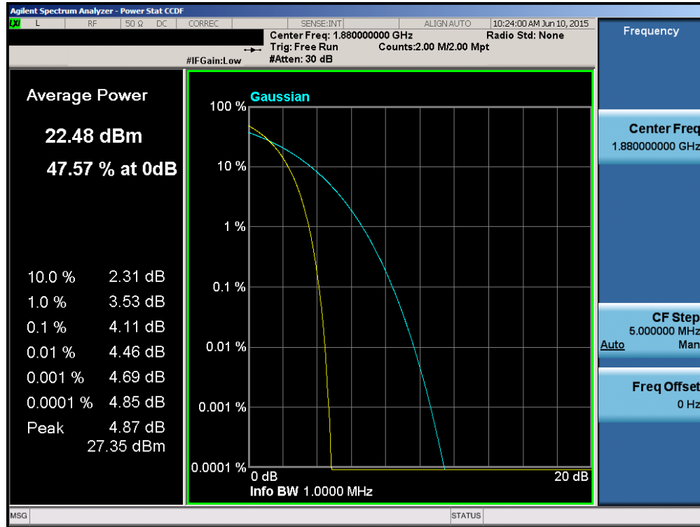
Plot 6-87. Peak-Average Ratio Plot (PCS CDMA Mode – Ch. 600)
