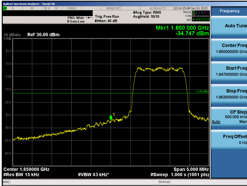
Plot 6-75. Band Edge Plot (PCS CDMA Mode – Ch. 25)
