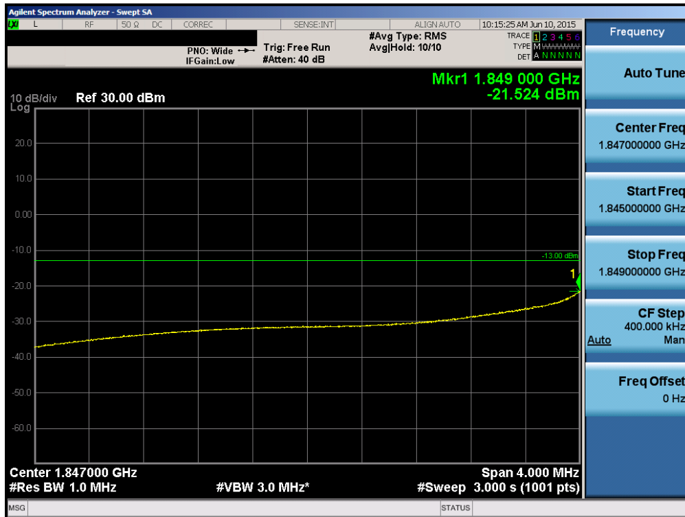
Plot 6-76. 4MHz Span Plot (PCS CDMA Mode – Ch. 25)
