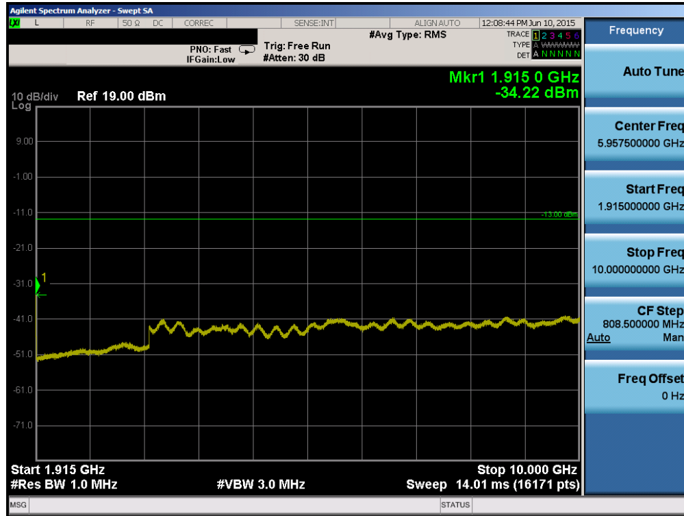
Plot 6-61. Conducted Spurious Plot (PCS WCDMA Mode – Ch. 9538)
