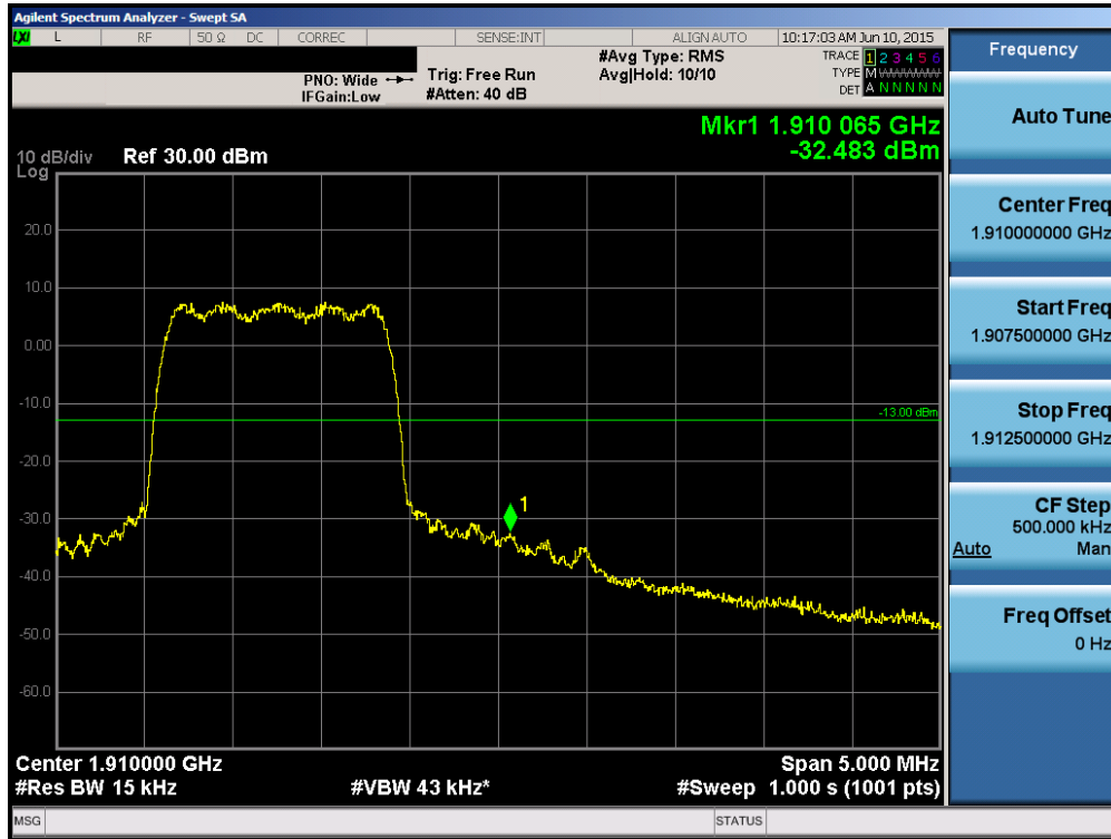
Plot 6-77. Band Edge Plot (PCS CDMA Mode – Ch. 1175)
