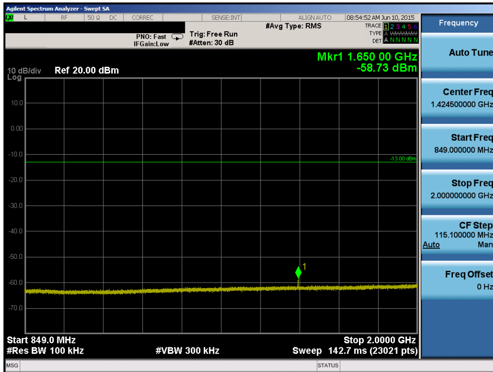
Plot 6-28. Conducted Spurious Plot (Cellular CDMA Mode – Ch. 1013)
