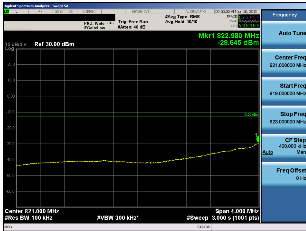
Plot 6-72. 4MHz Span Plot (Cellular CDMA Mode – Ch. 1013)
