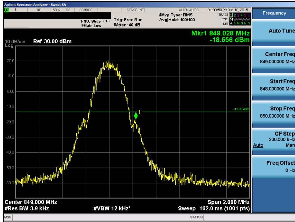
Plot 6-65. Band Edge Plot (Cellular GSM Mode – Ch. 251)
