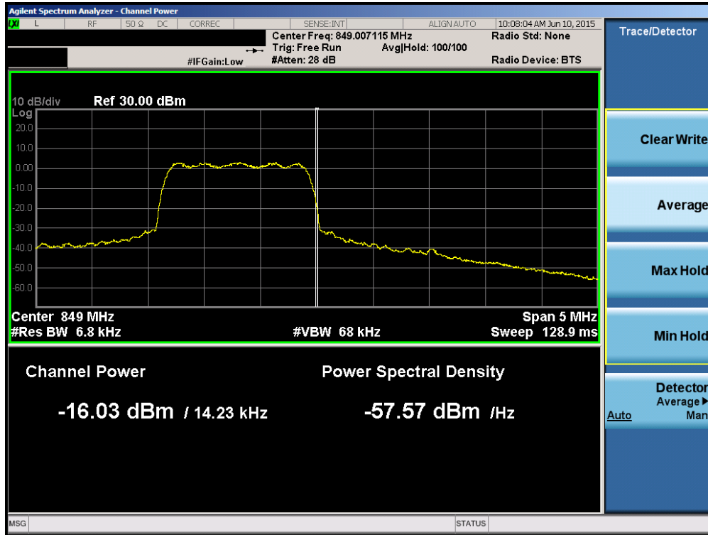
Plot 6-73. Band Edge Plot (Cellular CDMA Mode – Ch. 777)
