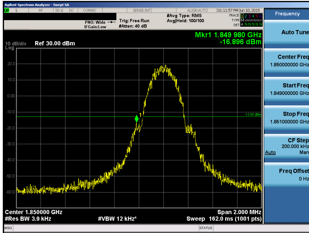
Plot 6-67. Band Edge Plot (PCS GSM Mode – Ch. 512)
