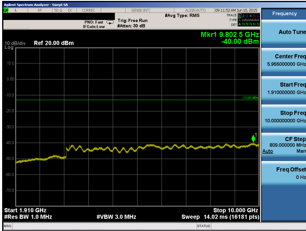
Plot 6-37. Conducted Spurious Plot (PCS CDMA Mode – Ch. 25)
