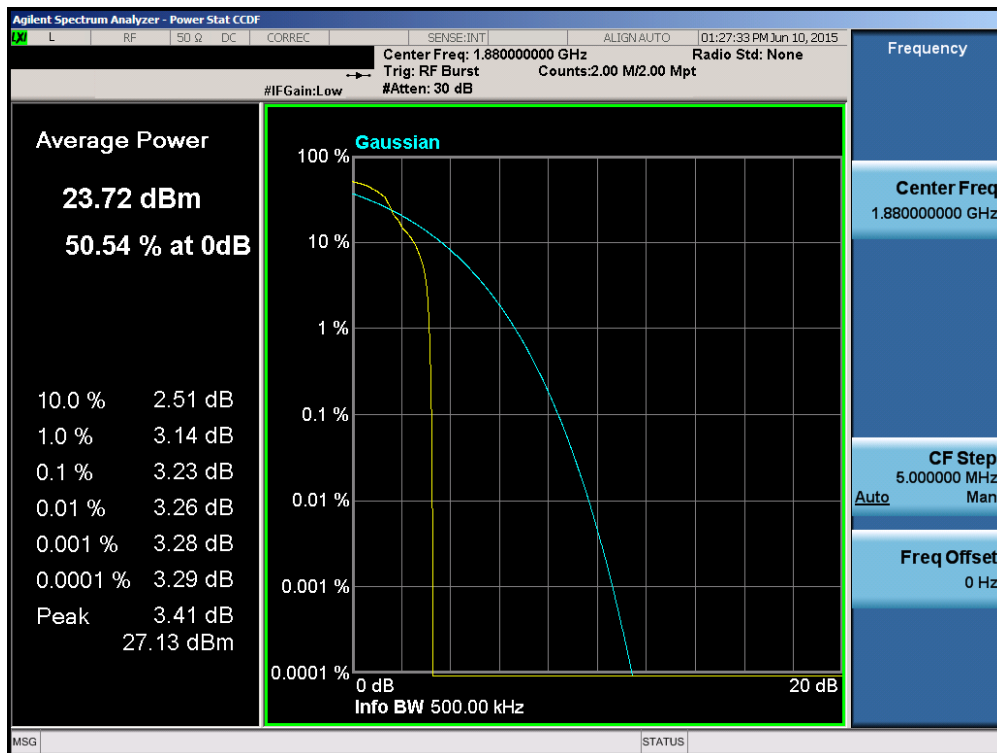
Plot 6-86. Peak-Average Ratio Plot (EDGE1900 Mode – Ch. 661)
