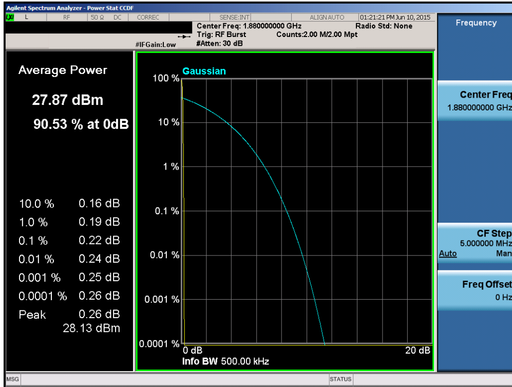
Plot 6-85. Peak-Average Ratio Plot (PCS GSM Mode – Ch. 661)
