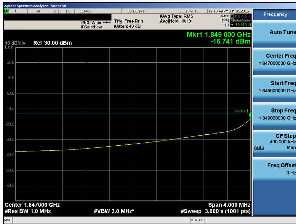
Plot 6-82. 4MHz Span Plot (PCS WCDMA Mode – Ch. 9262)
