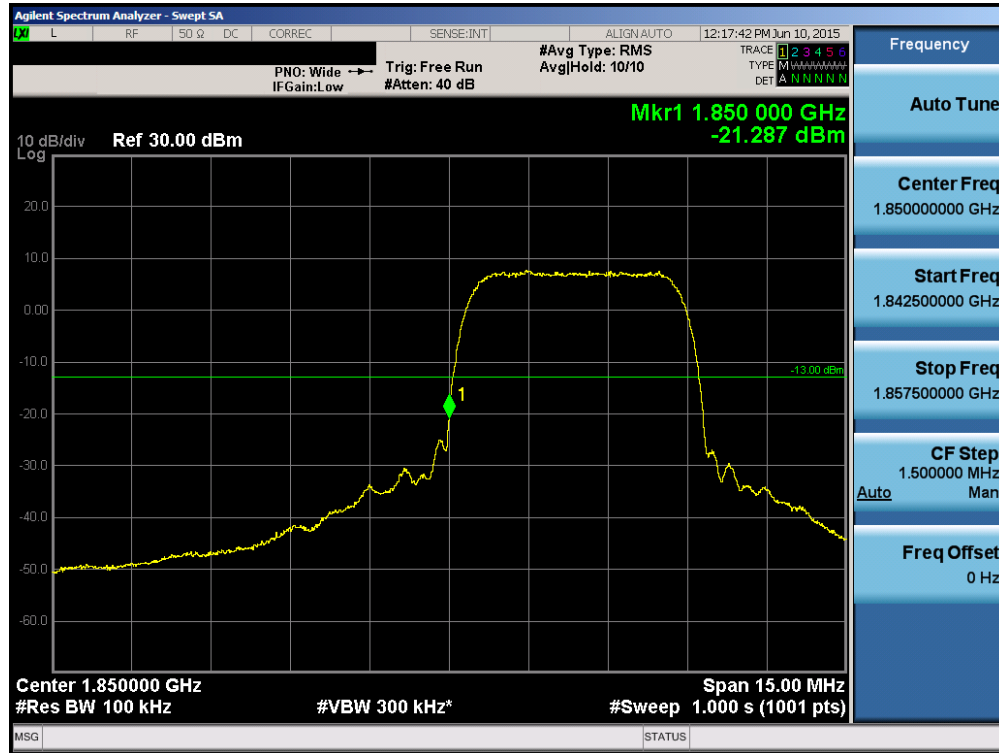
Plot 6-81. Band Edge Plot (PCS WCDMA Mode – Ch. 9262)
