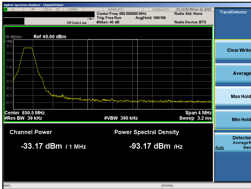
Plot 6-66. 4MHz Span Plot (Cellular GSM Mode – Ch. 251)
