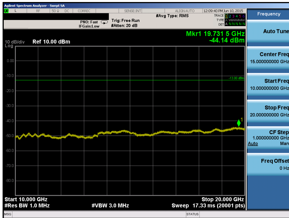
Plot 6-62. Conducted Spurious Plot (PCS WCDMA Mode – Ch. 9538)
