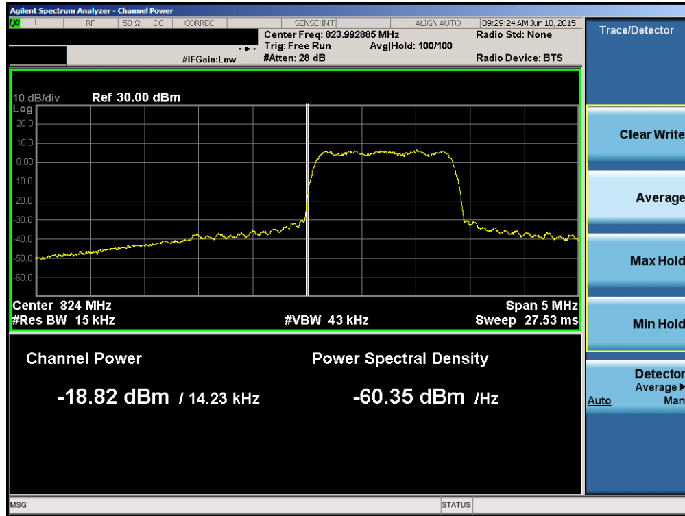
Plot 6-71. Band Edge Plot (Cellular CDMA Mode – Ch. 1013)
