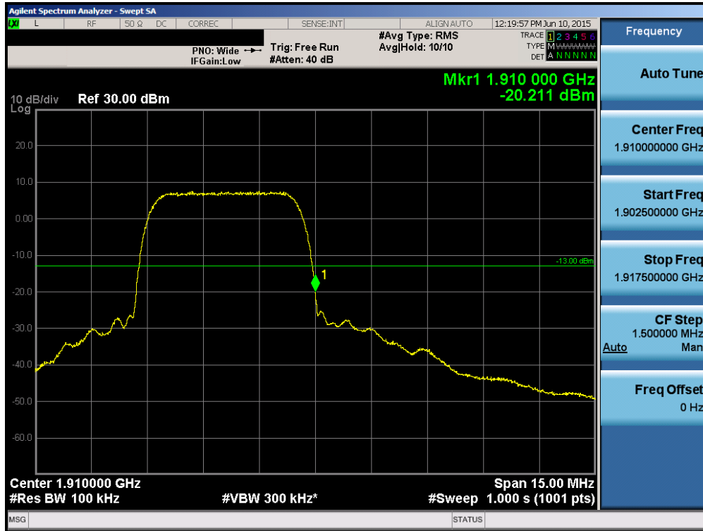
Plot 6-83. Band Edge Plot (PCS WCDMA Mode – Ch. 9538)
