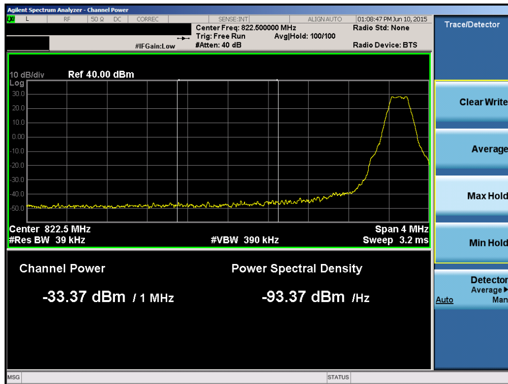
Plot 6-64. 4MHz Span Plot (Cellular GSM Mode – Ch. 128)
