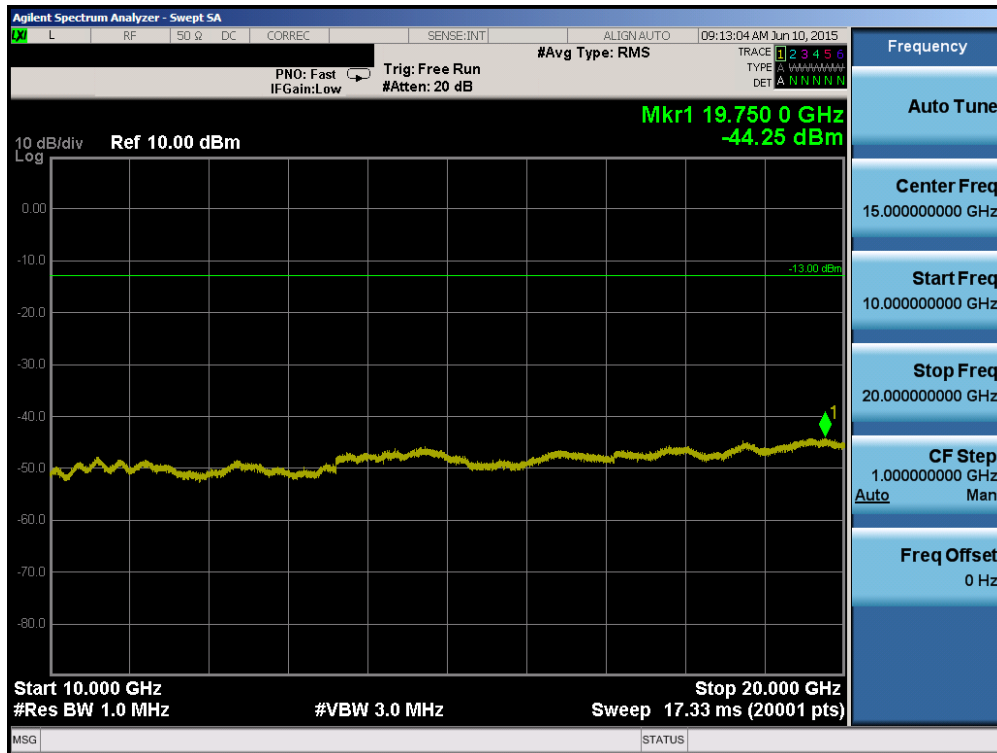
Plot 6-38. Conducted Spurious Plot (PCS CDMA Mode – Ch. 25)
