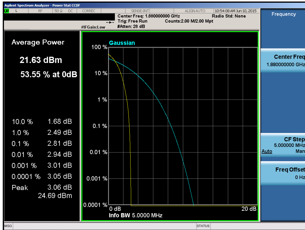
Plot 6-88. Peak-Average Ratio Plot (PCS WCDMA Mode – Ch. 9400)
