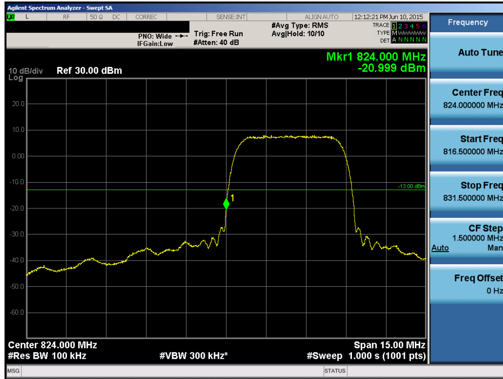
Plot 6-79. Band Edge Plot (Cellular WCDMA Mode – Ch. 4132)
