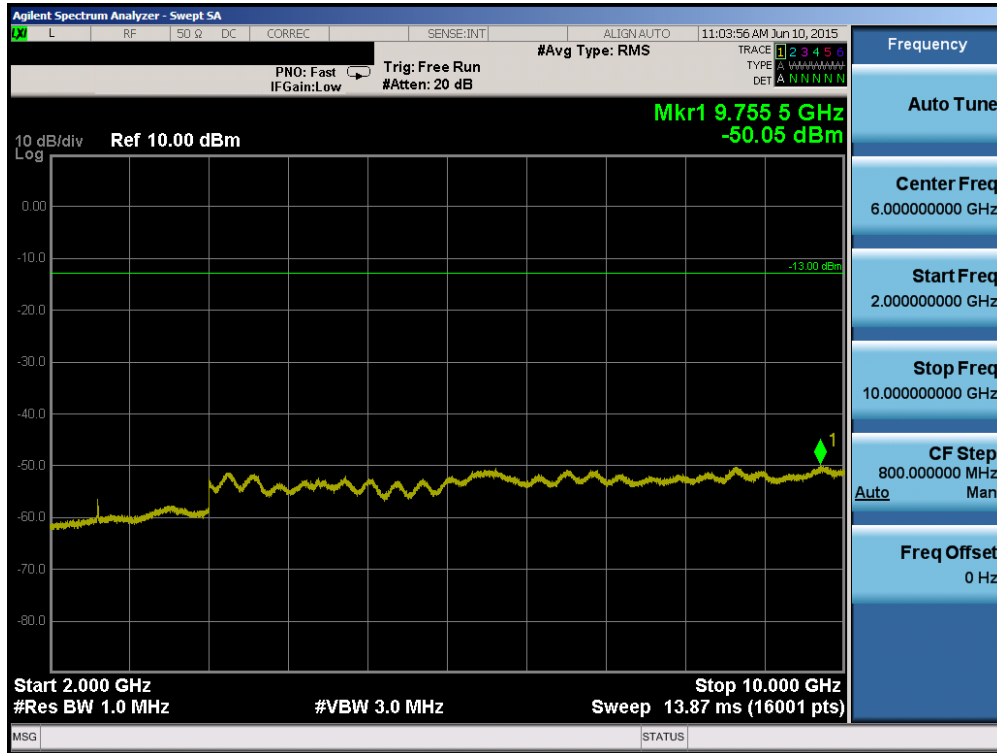
Plot 6-47. Conducted Spurious Plot (Cellular WCDMA Mode – Ch. 4132)
