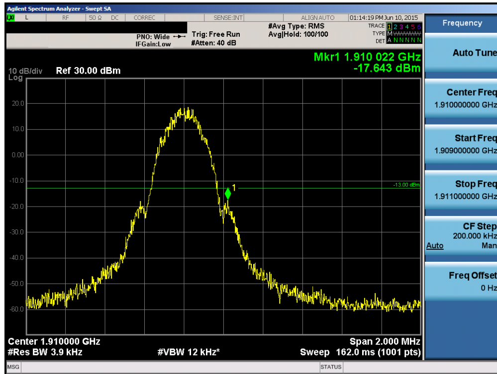
Plot 6-69. Band Edge Plot (PCS GSM Mode – Ch. 810)
