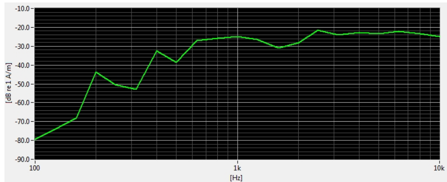
Figure 7-3 Worst-case ABM2 Plot for GSM
