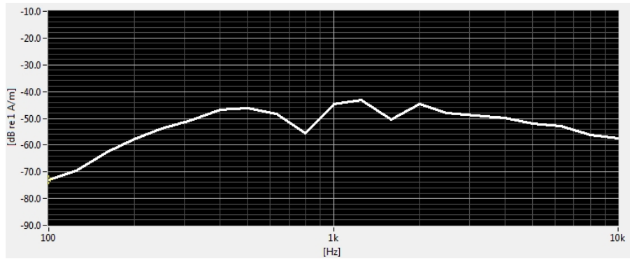
Figure 7-2 Worst-case ABM2 Plot for CDMA
