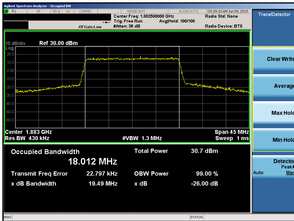
Plot 6-43. Occupied Bandwidth Plot (Band 2/25 – 20.0MHz QPSK – RB Size 100)
