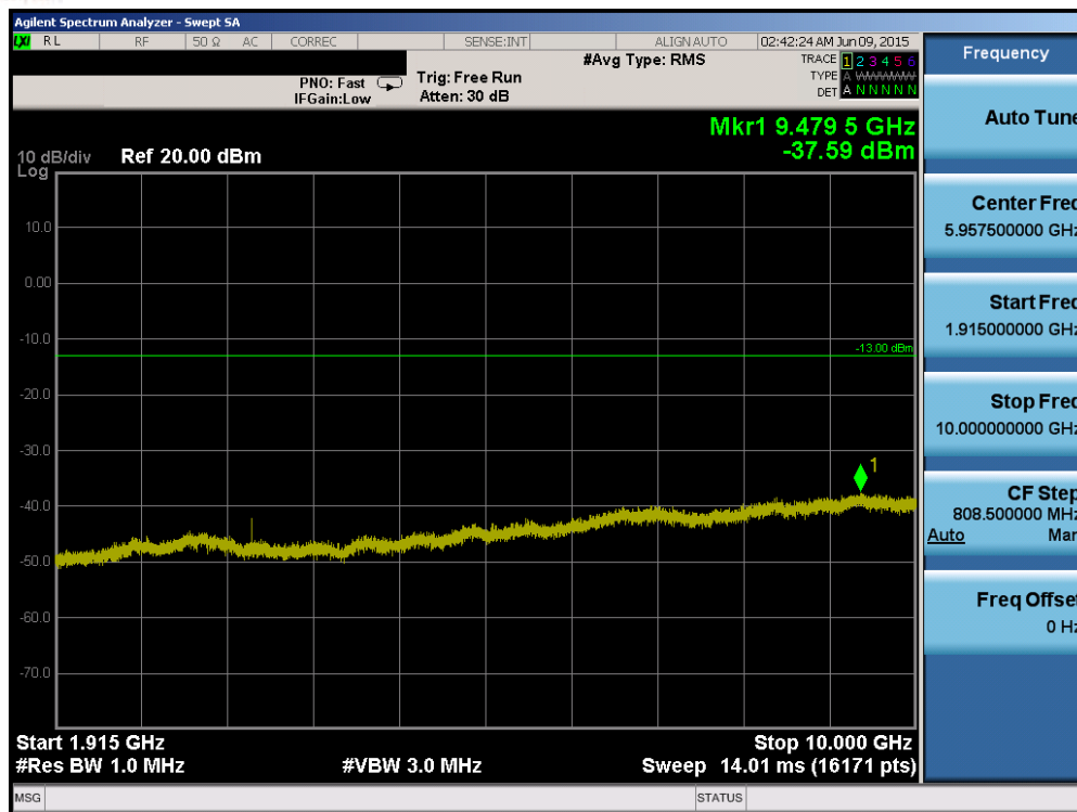
Plot 6-85. Conducted Spurious Plot (Band 2/25 – 5.0MHz QPSK – RB Size 1, RB Offset 0 – Mid Channel)
