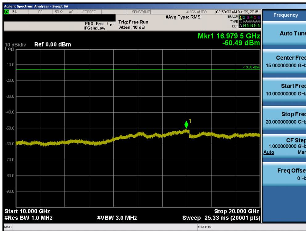
Plot 6-89. Conducted Spurious Plot (Band 2/25 – 5.0MHz QPSK – RB Size 1, RB Offset 0 – High Channel)
