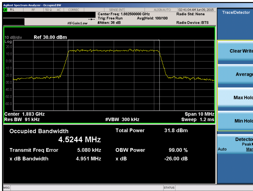
Plot 6-37. Occupied Bandwidth Plot (Band 2/25 – 5.0MHz QPSK – RB Size 25)
