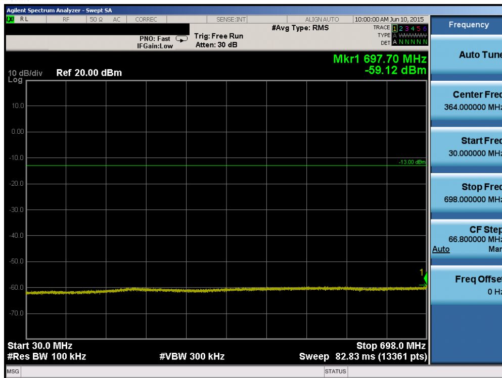
Plot 6-51. Conducted Spurious Plot (Band 12/17 – 5.0MHz QPSK – RB Size 1, RB Offset 0 – High Channel)
