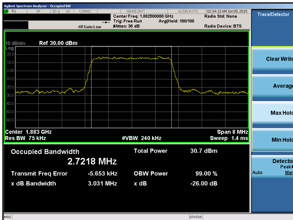
Plot 6-36. Occupied Bandwidth Plot (Band 2/25 – 3.0MHz 16-QAM – RB Size 15)
