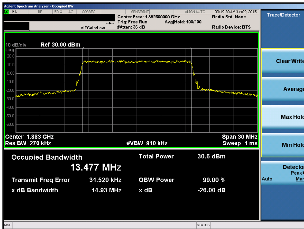
Plot 6-41. Occupied Bandwidth Plot (Band 2/25 – 15.0MHz QPSK – RB Size 75)
