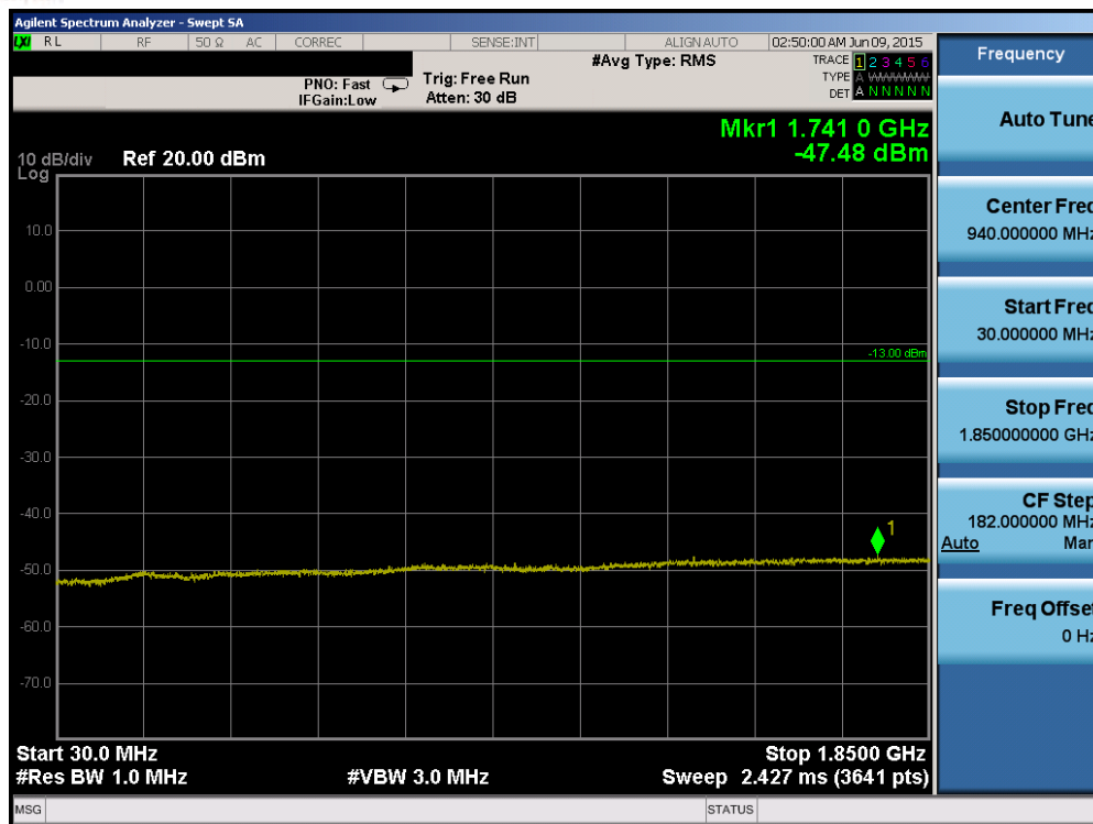
Plot 6-87. Conducted Spurious Plot (Band 2/25 – 5.0MHz QPSK – RB Size 1, RB Offset 0 – High Channel)
