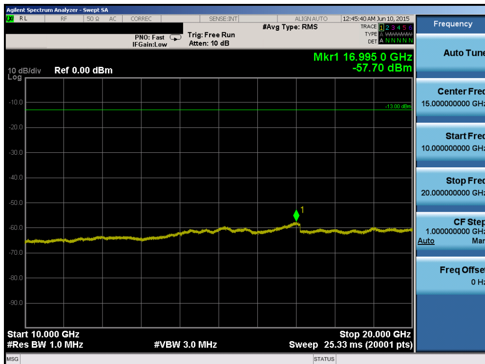
Plot 6-80. Conducted Spurious Plot (Band 4 – 1.4MHz QPSK – RB Size 1, RB Offset 0 – High Channel)
