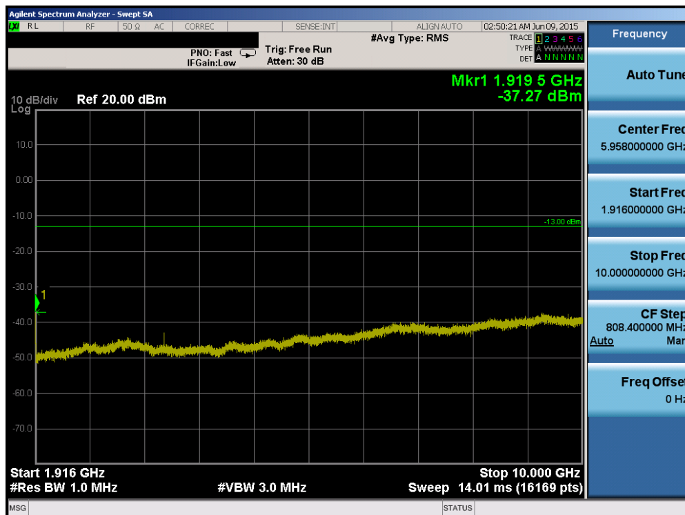
Plot 6-88. Conducted Spurious Plot (Band 2/25 – 5.0MHz QPSK – RB Size 1, RB Offset 0 – High Channel)
