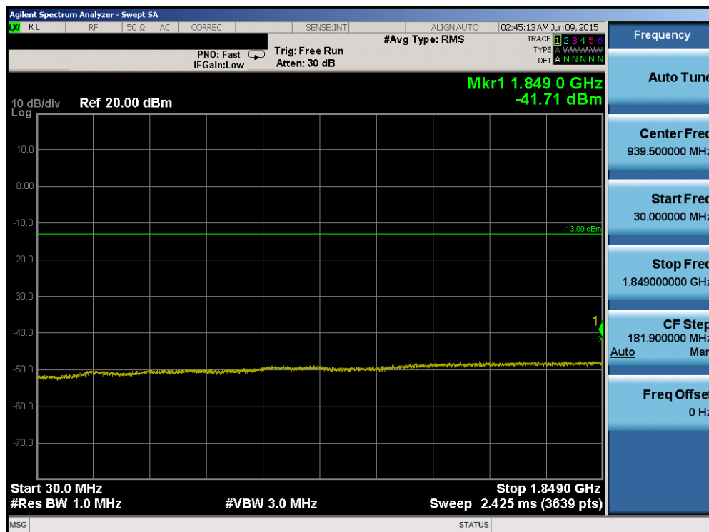
Plot 6-81. Conducted Spurious Plot (Band 2/25 – 5.0MHz QPSK – RB Size 1, RB Offset 0 – Low Channel)
