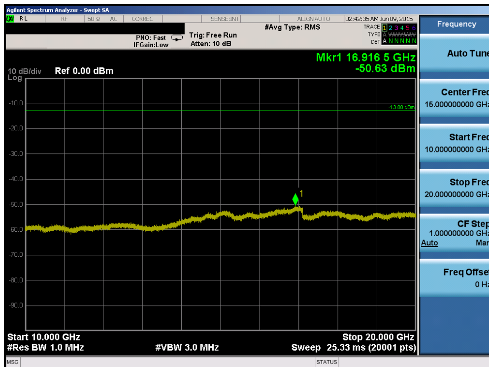
Plot 6-86. Conducted Spurious Plot (Band 2/25 – 5.0MHz QPSK – RB Size 1, RB Offset 0 – Mid Channel)
