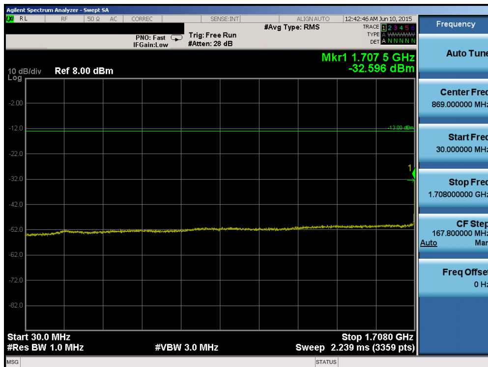
Plot 6-72. Conducted Spurious Plot (Band 4 – 1.4MHz QPSK – RB Size 1, RB Offset 0 – Low Channel)
