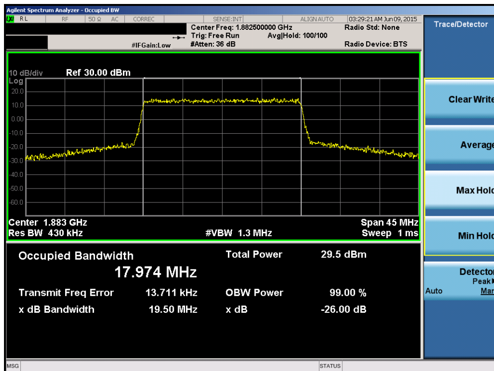
Plot 6-44. Occupied Bandwidth Plot (Band 2/25 – 20.0MHz 16-QAM – RB Size 100)
