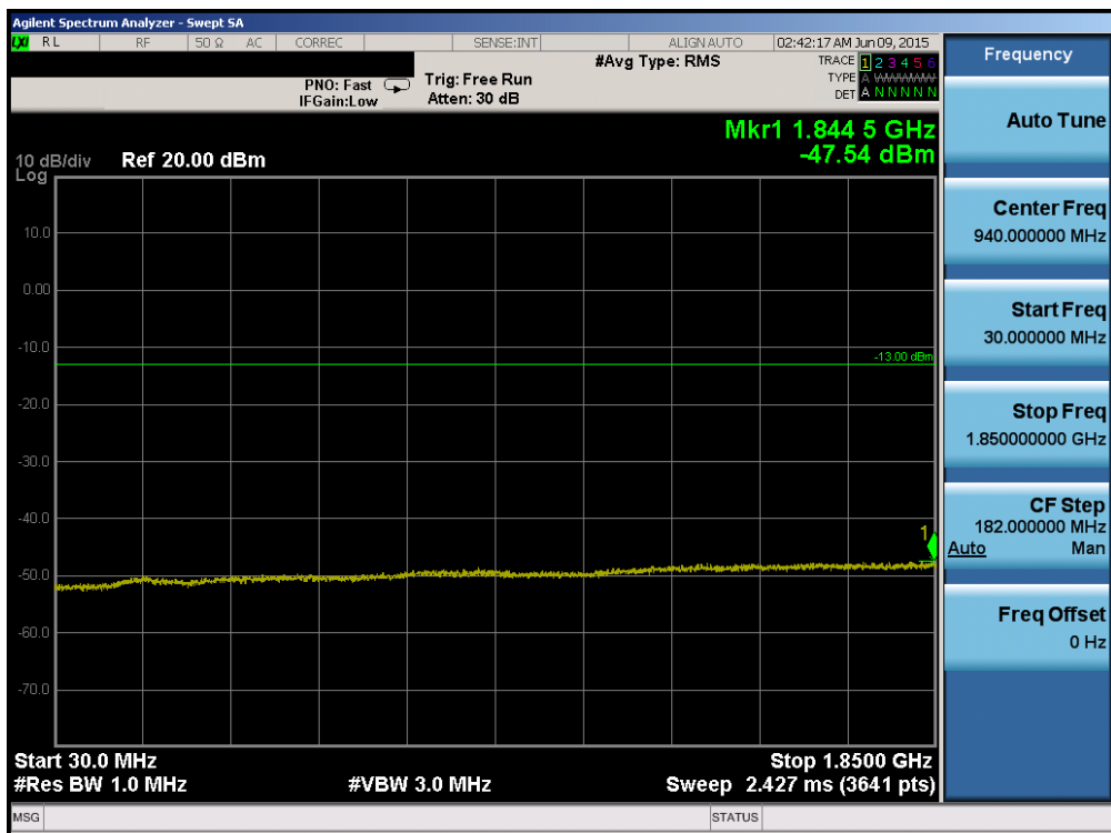
Plot 6-84. Conducted Spurious Plot (Band 2/25 – 5.0MHz QPSK – RB Size 1, RB Offset 0 – Mid Channel)
