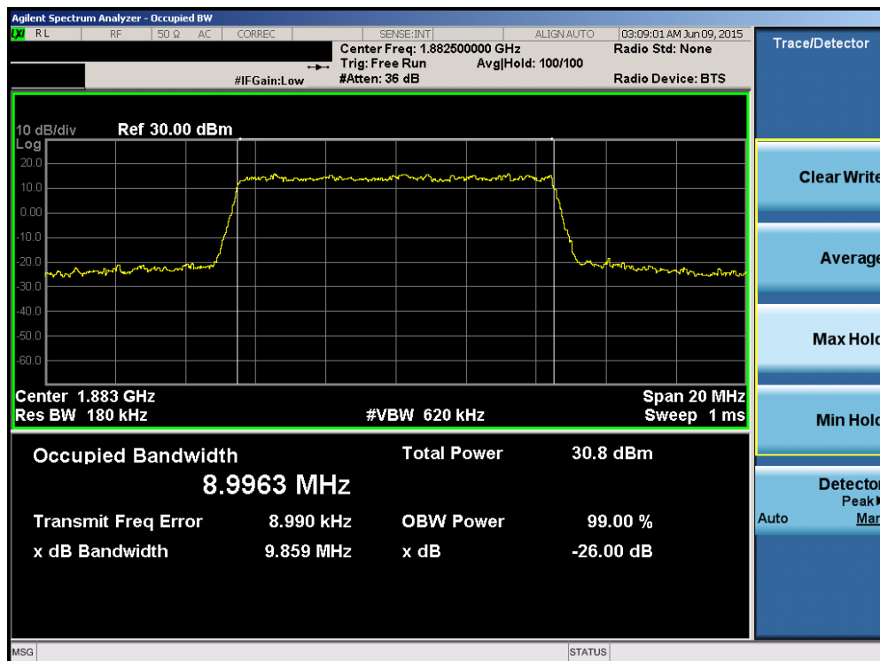
Plot 6-40. Occupied Bandwidth Plot (Band 2/25 – 10.0MHz 16-QAM – RB Size 50)
