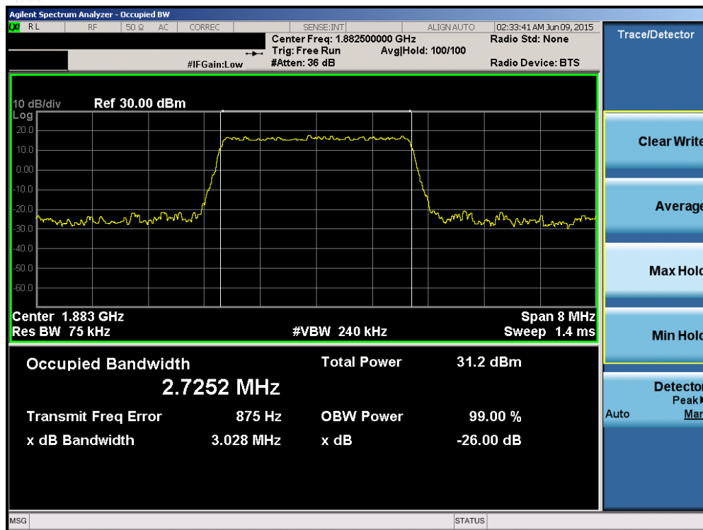
Plot 6-35. Occupied Bandwidth Plot (Band 2/25 – 3.0MHz QPSK – RB Size 15)
