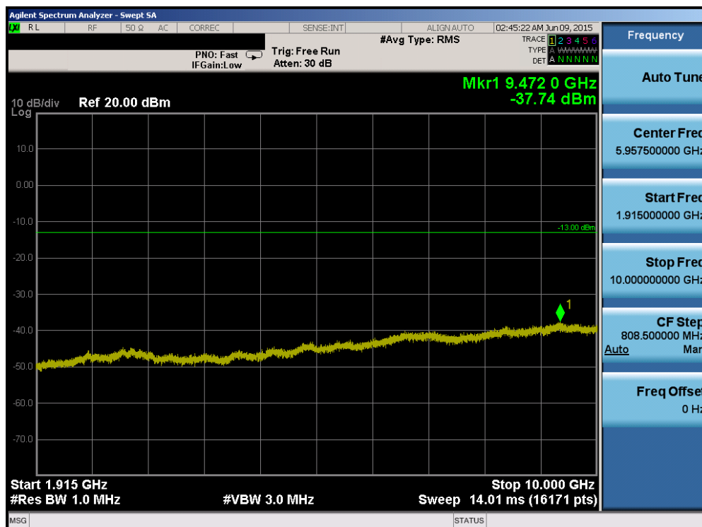
Plot 6-82. Conducted Spurious Plot (Band 2/25 – 5.0MHz QPSK – RB Size 1, RB Offset 0 – Low Channel)
