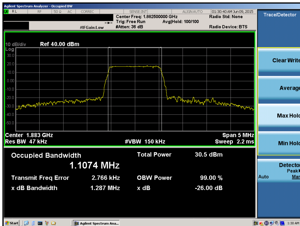
Plot 6-34. Occupied Bandwidth Plot (Band 2/25 – 1.4MHz 16-QAM – RB Size 6)
