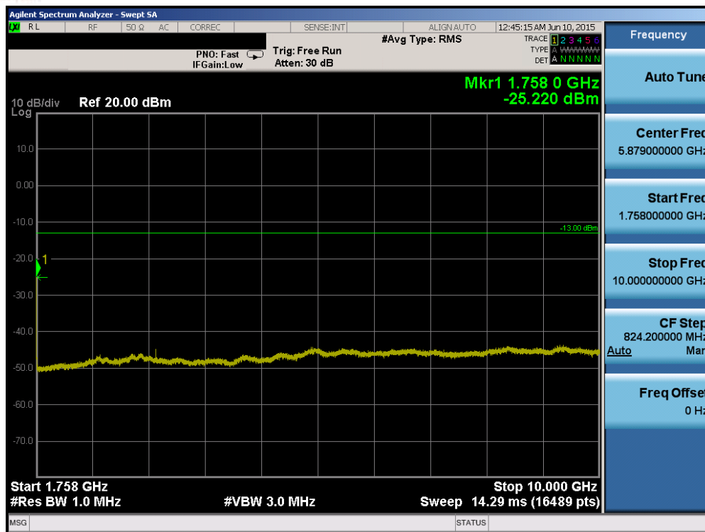
Plot 6-79. Conducted Spurious Plot (Band 4 – 1.4MHz QPSK – RB Size 1, RB Offset 0 – High Channel)
