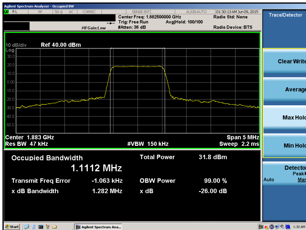
Plot 6-33. Occupied Bandwidth Plot (Band 2/25 – 1.4MHz QPSK – RB Size 6)
