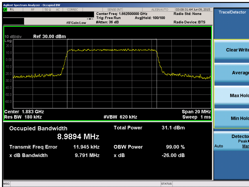
Plot 6-39. Occupied Bandwidth Plot (Band 2/25 – 10.0MHz QPSK – RB Size 50)
