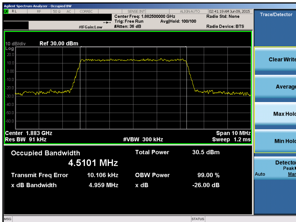
Plot 6-38. Occupied Bandwidth Plot (Band 2/25 – 5.0MHz 16-QAM – RB Size 25)
