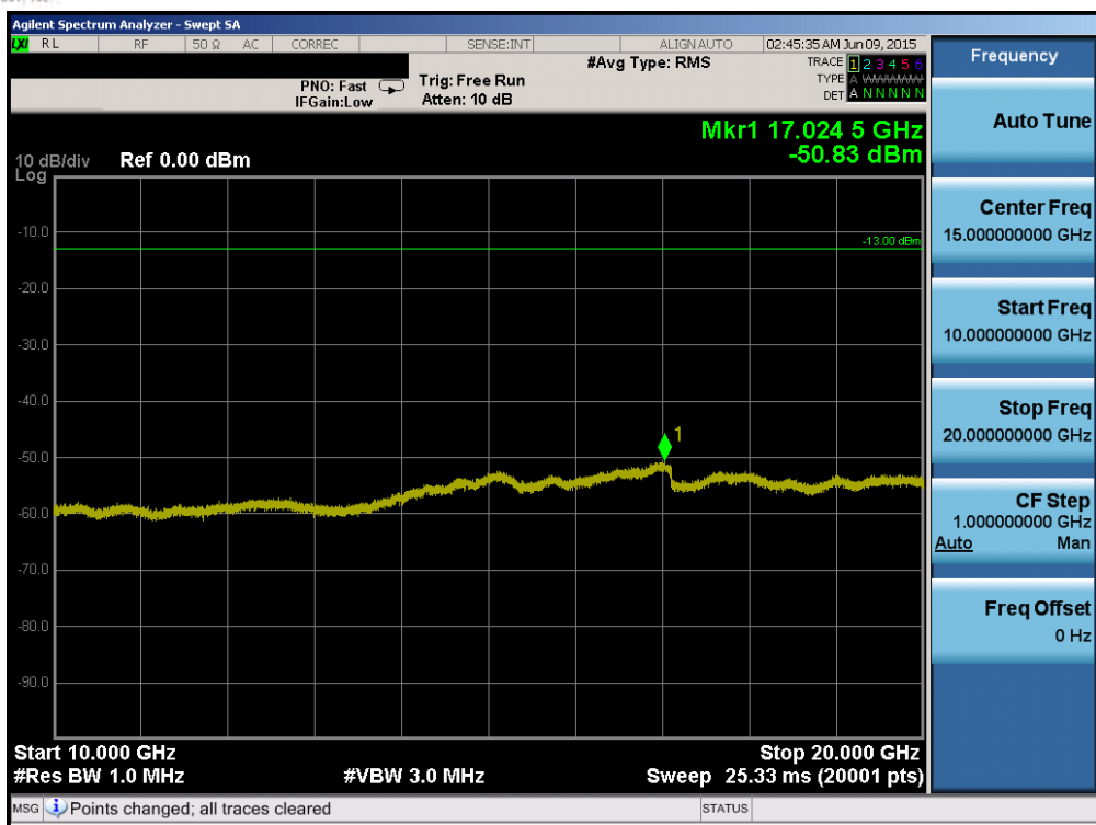
Plot 6-83. Conducted Spurious Plot (Band 2/25 – 5.0MHz QPSK – RB Size 1, RB Offset 0 – Low Channel)
