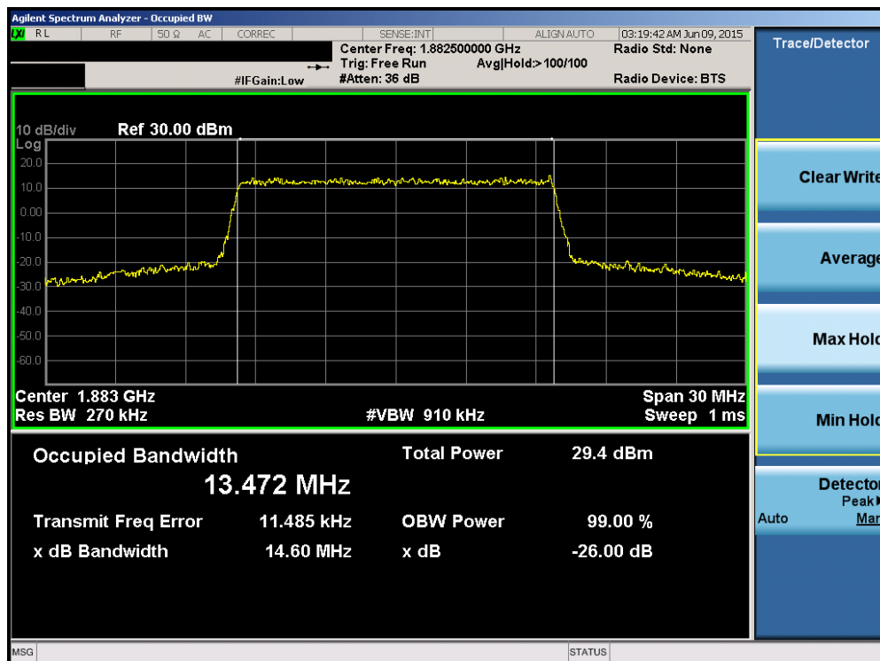
Plot 6-42. Occupied Bandwidth Plot (Band 2/25 – 15.0MHz 16-QAM – RB Size 75)
