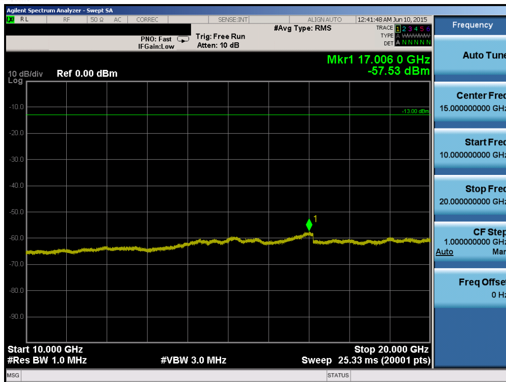
Plot 6-77. Conducted Spurious Plot (Band 4 – 1.4MHz QPSK – RB Size 1, RB Offset 0 – Mid Channel)
