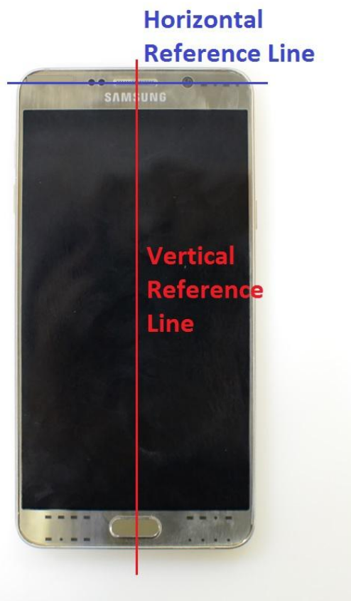
SAR Test Setup Photo 21– DUT Reference Lines
