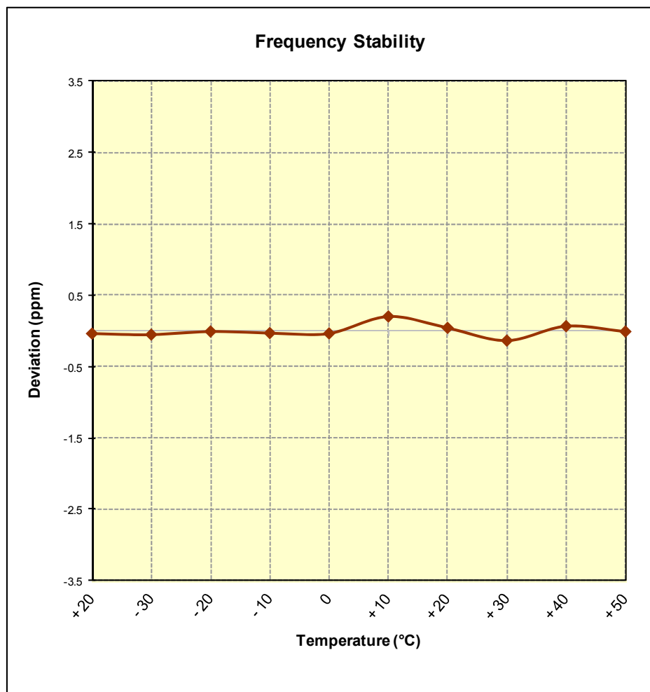
Figure 6-11. Frequency Stability Graph (PCS WCDMA Mode – Ch. 9400)
