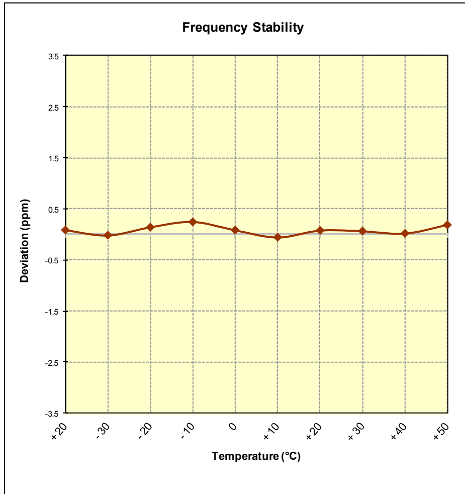
Figure 6-9. Frequency Stability Graph (AWS WCDMA Mode – Ch. 1412)
