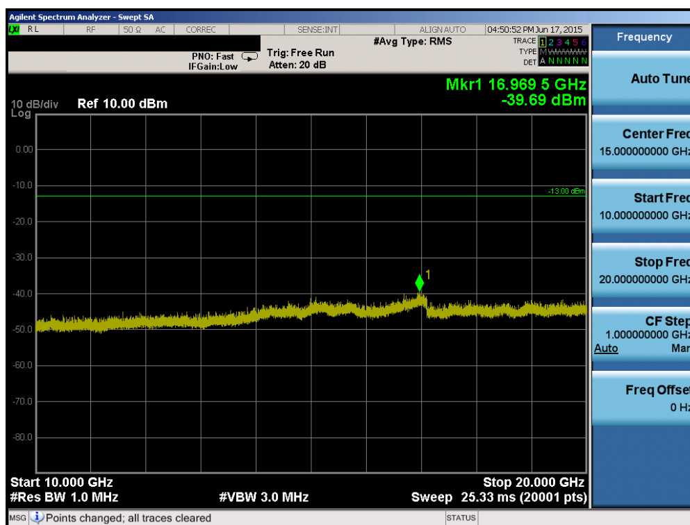
Plot 6-19. Conducted Spurious Plot (PCS GSM Mode – Ch. 512)
