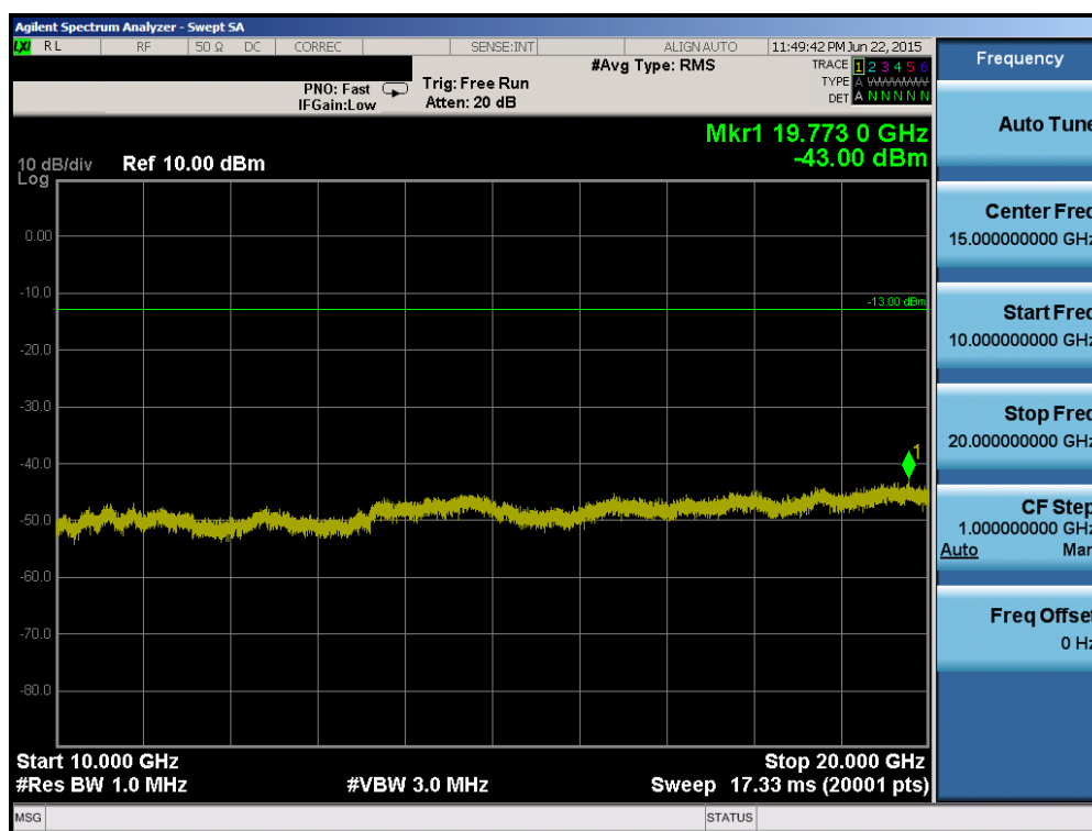
Plot 6-43. Conducted Spurious Plot (AWS WCDMA Mode – Ch. 1862)
