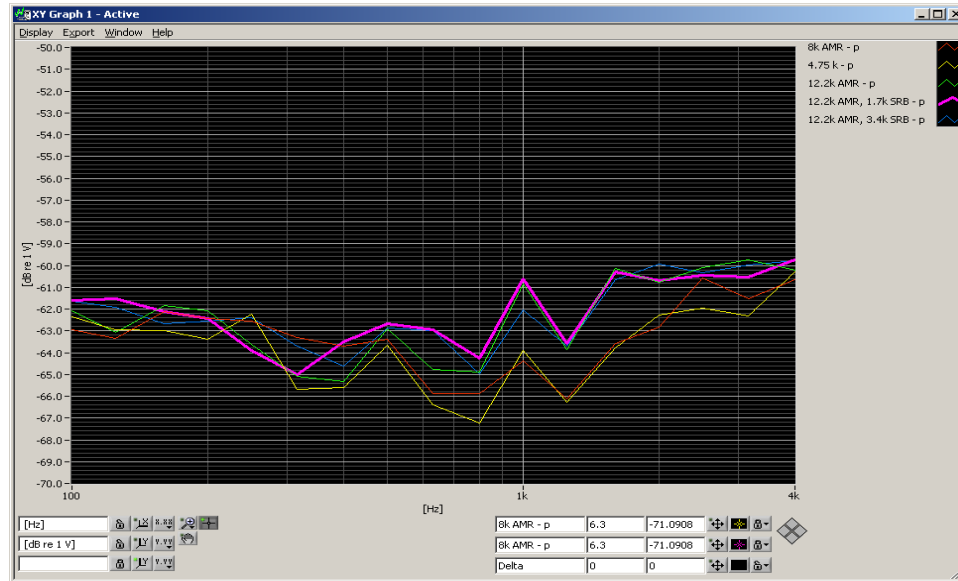
Figure 7-1 UMTS Audio Band Magnetic Noise
