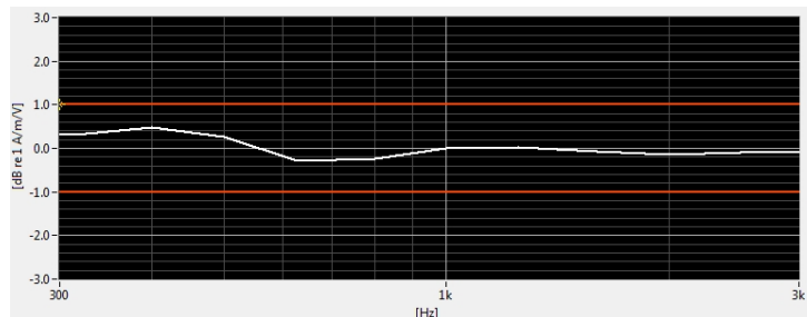
Figure 8-6 Helmholtz Coil Validation for Frequency Response
