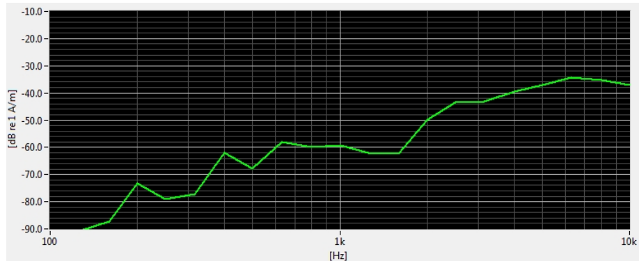
Figure 8-2 Worst-case ABM2 Plot for GSM
