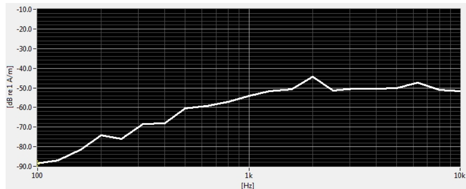
Figure 8-4 Worst-case ABM2 Plot for LTE
