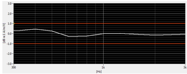
Figure 8-5 Helmholtz Coil Validation for Frequency Response
