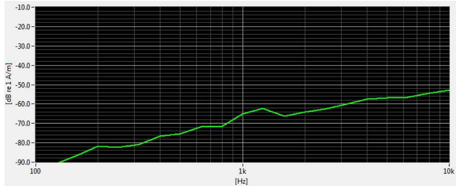
Figure 8-3 Worst-case ABM2 Plot for UMTS
