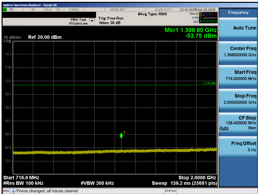
Plot 6-50. Conducted Spurious Plot (Band 12/17 – 5.0MHz QPSK – RB Size 1, RB Offset 0 – Low Channel)
