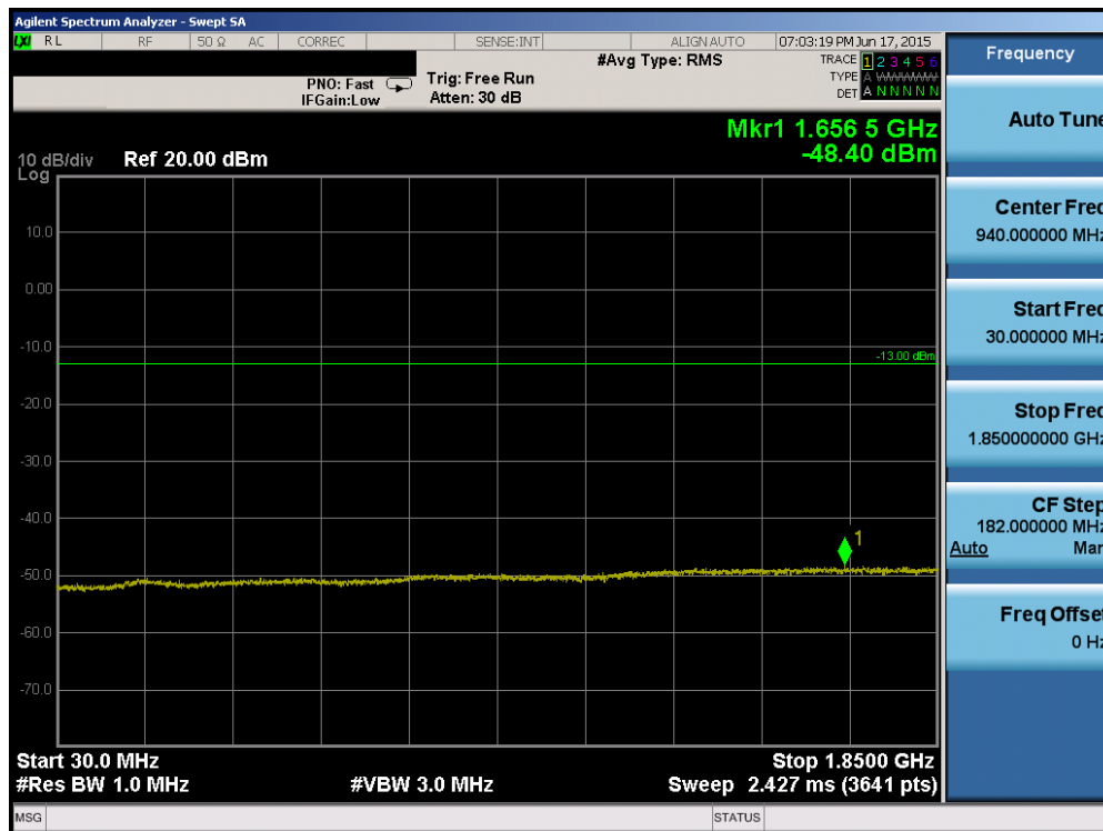
Plot 6-92. Conducted Spurious Plot (Band 2 – 10.0MHz QPSK – RB Size 1, RB Offset 0 – High Channel)
