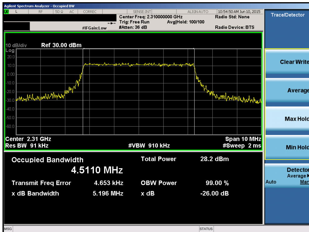
Plot 6-46. Occupied Bandwidth Plot (Band 30 – 5.0MHz 16-QAM – RB Size 25)
