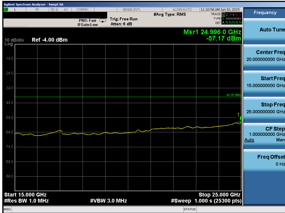
Plot 6-97. Conducted Spurious Plot (Band 30 – 10.0MHz QPSK – RB Size 1, RB Offset 0 – Mid Channel)
