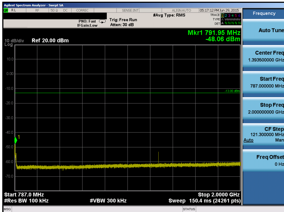
Plot 6-62. Conducted Spurious Plot (Band 13 – 5.0MHz QPSK – RB Size 1, RB Offset 0 – Mid Channel)
