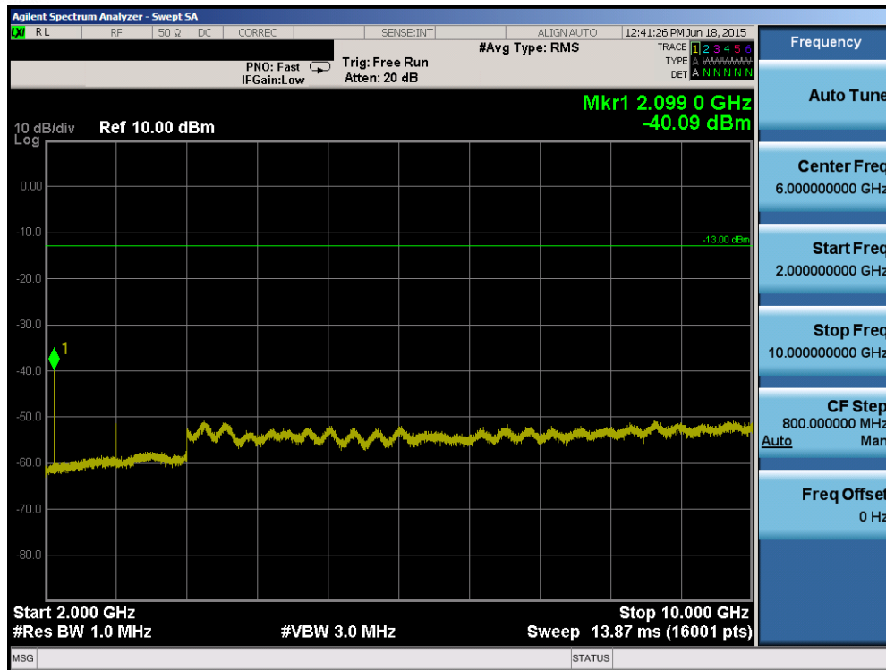
Plot 6-51. Conducted Spurious Plot (Band 12/17 – 5.0MHz QPSK – RB Size 1, RB Offset 0 – Low Channel)
