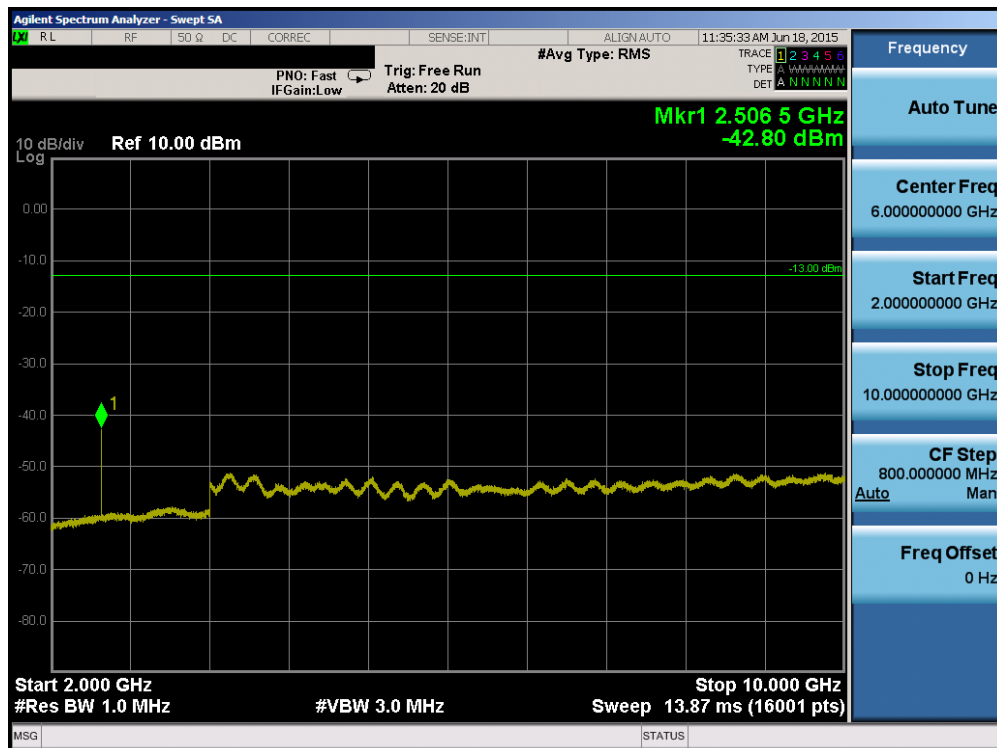
Plot 6-72. Conducted Spurious Plot (Band 5 – 3.0MHz QPSK – RB Size 1, RB Offset 0 – Mid Channel)
