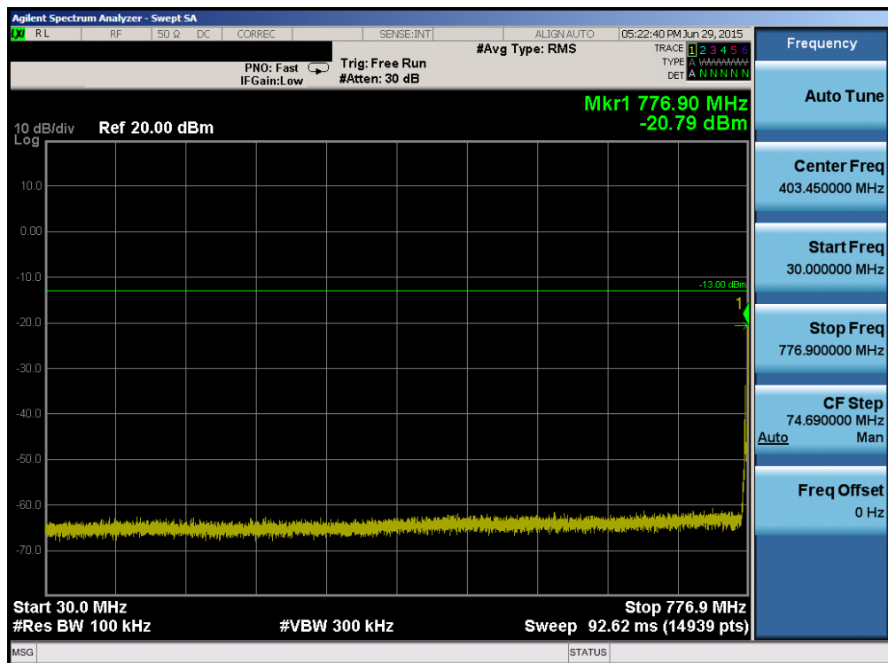
Plot 6-58. Conducted Spurious Plot (Band 13 – 5.0MHz QPSK – RB Size 1, RB Offset 0 – Low Channel)
