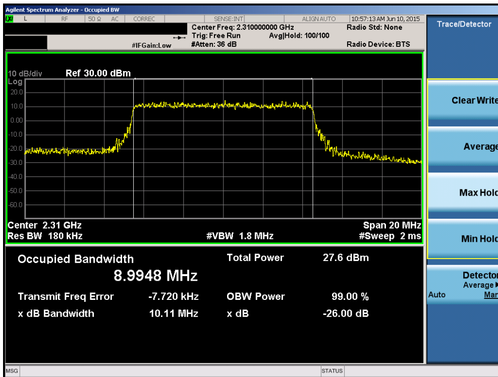
Plot 6-48. Occupied Bandwidth Plot (Band 30 – 10.0MHz 16-QAM – RB Size 50)
