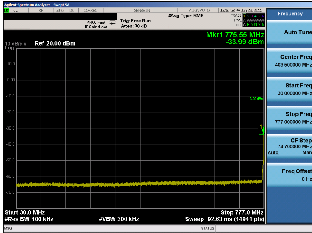
Plot 6-61. Conducted Spurious Plot (Band 13 – 5.0MHz QPSK – RB Size 1, RB Offset 0 – Mid Channel)
