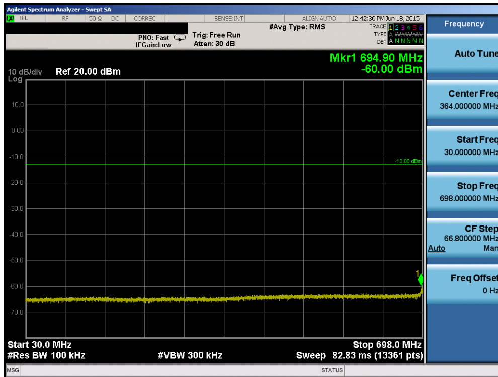
Plot 6-55. Conducted Spurious Plot (Band 12/17 – 5.0MHz QPSK – RB Size 1, RB Offset 0 – High Channel)
