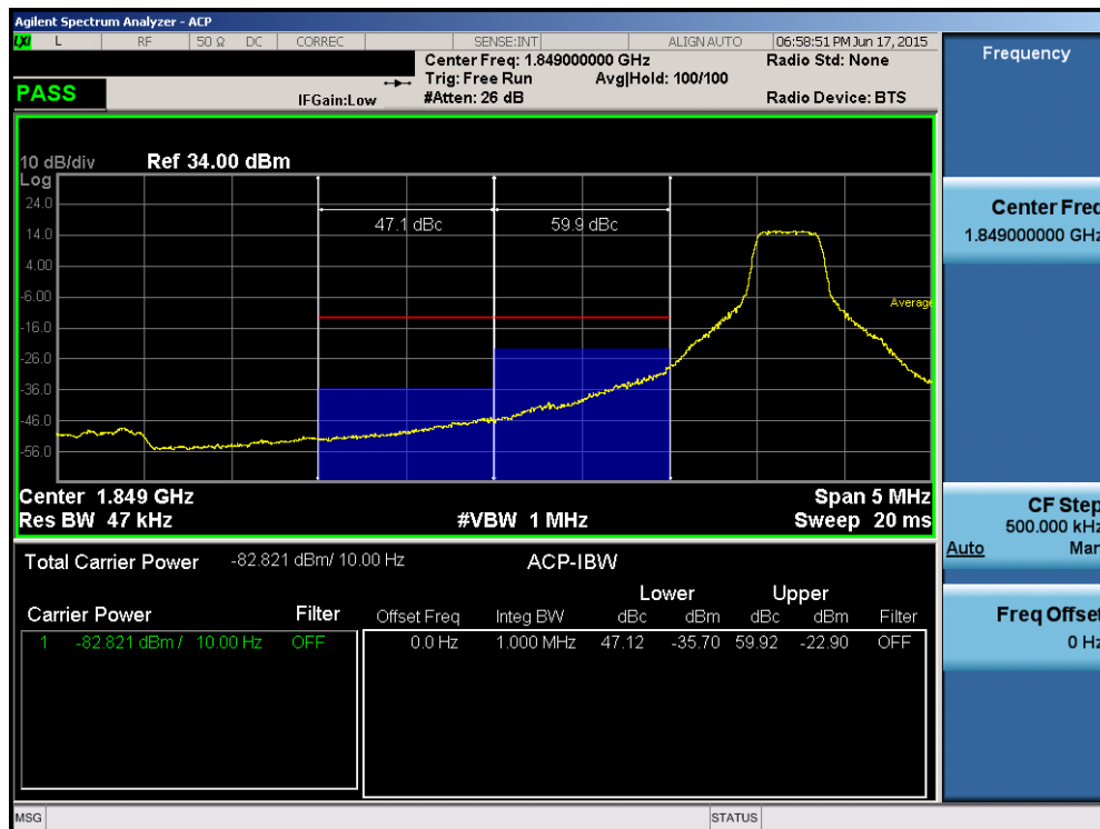
Plot 6-86. Conducted Spurious Plot (Band 2 – 10.0MHz QPSK – RB Size 1, RB Offset 0– Low Channel)
