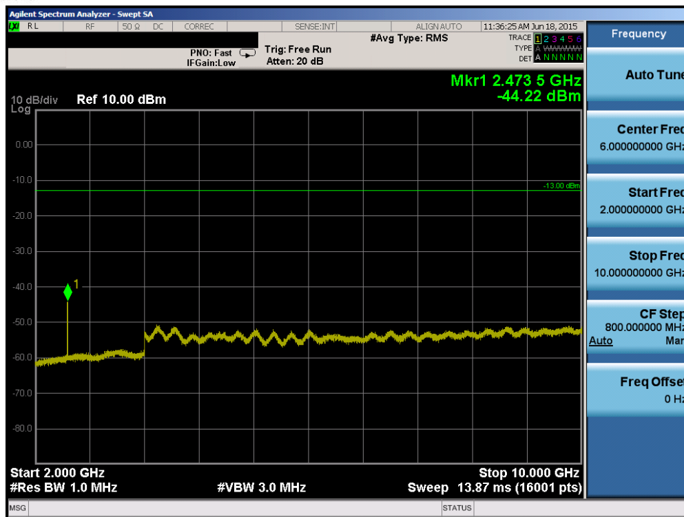
Plot 6-69. Conducted Spurious Plot (Band 5 – 3.0MHz QPSK – RB Size 1, RB Offset 0 – Low Channel)
