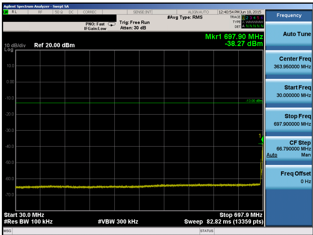
Plot 6-49. Conducted Spurious Plot (Band 12/17 – 5.0MHz QPSK – RB Size 1, RB Offset 0 – Low Channel)
