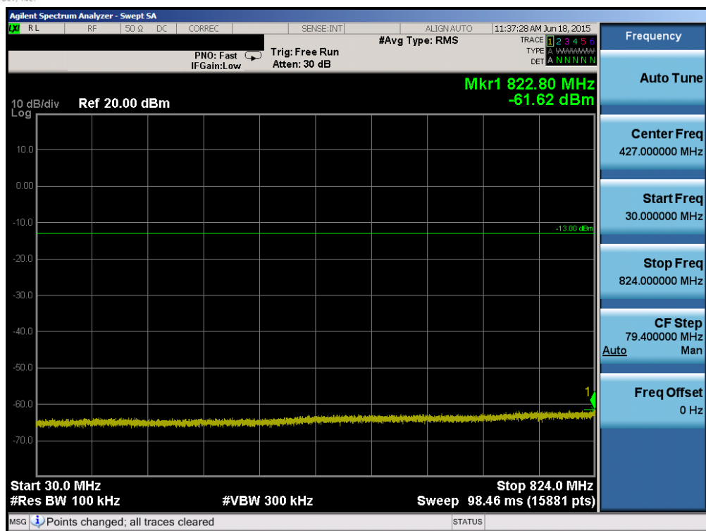
Plot 6-73. Conducted Spurious Plot (Band 5 – 3.0MHz QPSK – RB Size 1, RB Offset 0 – High Channel)
