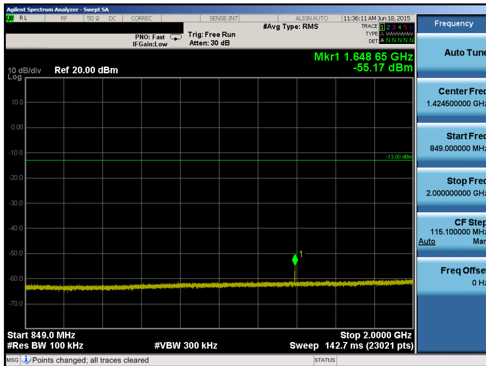
Plot 6-68. Conducted Spurious Plot (Band 5 – 3.0MHz QPSK – RB Size 1, RB Offset 0 – Low Channel)
