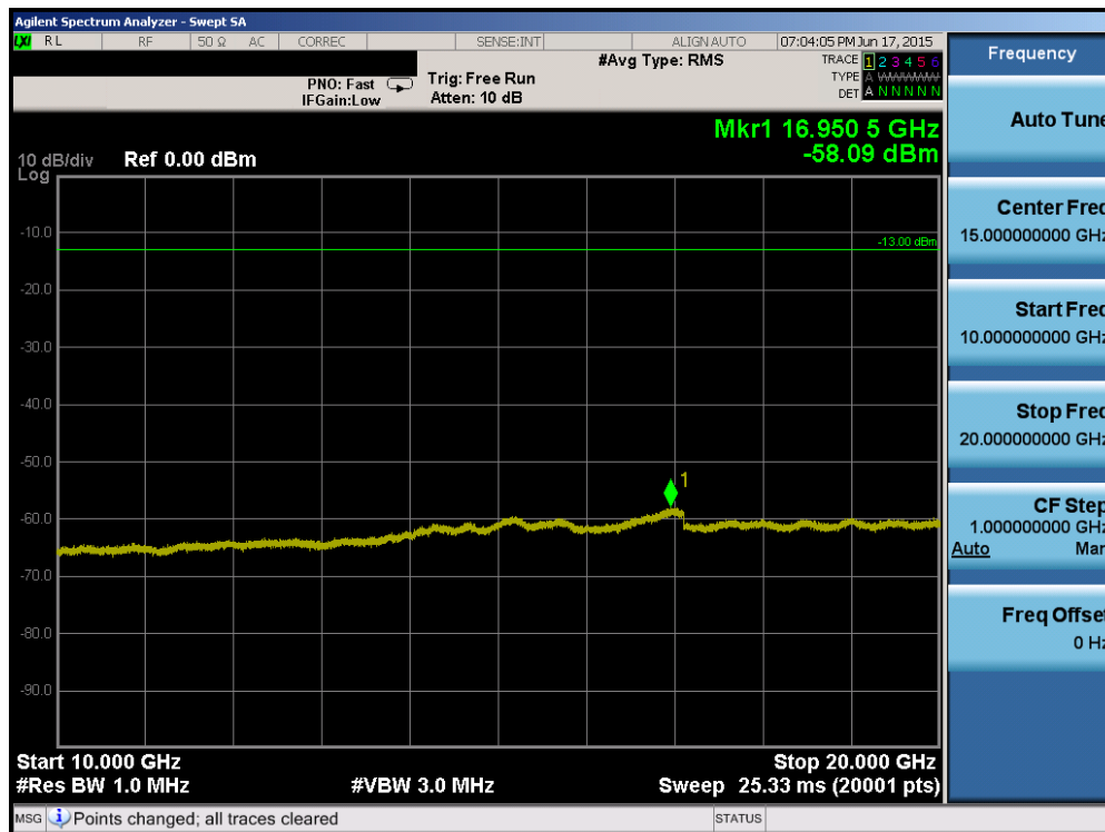
Plot 6-94. Conducted Spurious Plot (Band 2 – 10.0MHz QPSK – RB Size 1, RB Offset 0 – High Channel)
