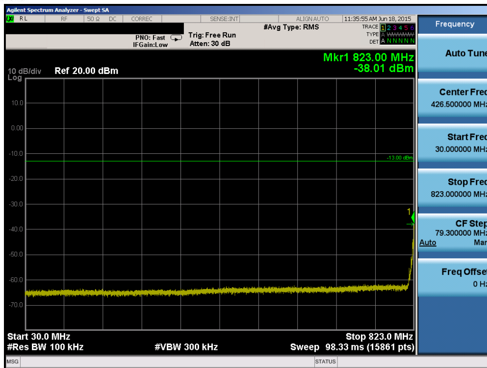
Plot 6-67. Conducted Spurious Plot (Band 5 – 3.0MHz QPSK – RB Size 1, RB Offset 0 – Low Channel)
