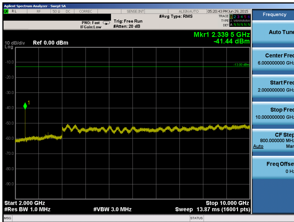
Plot 6-63. Conducted Spurious Plot (Band 13 – 5.0MHz QPSK – RB Size 1, RB Offset 0 – Mid Channel)
