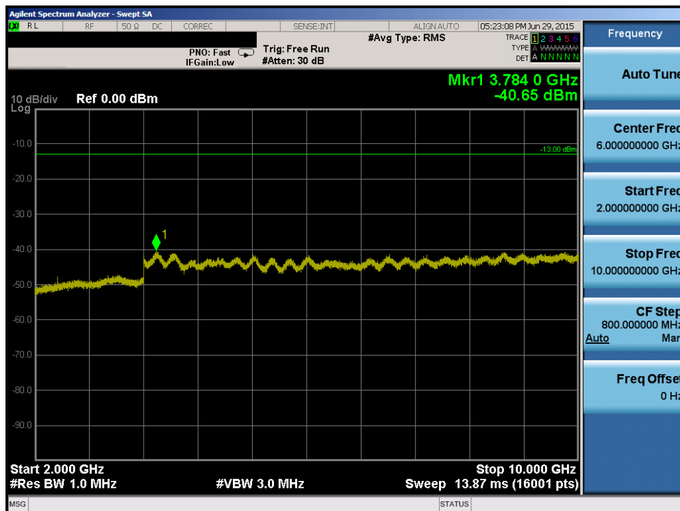
Plot 6-60. Conducted Spurious Plot (Band 13 – 5.0MHz QPSK – RB Size 1, RB Offset 0 – Low Channel)
