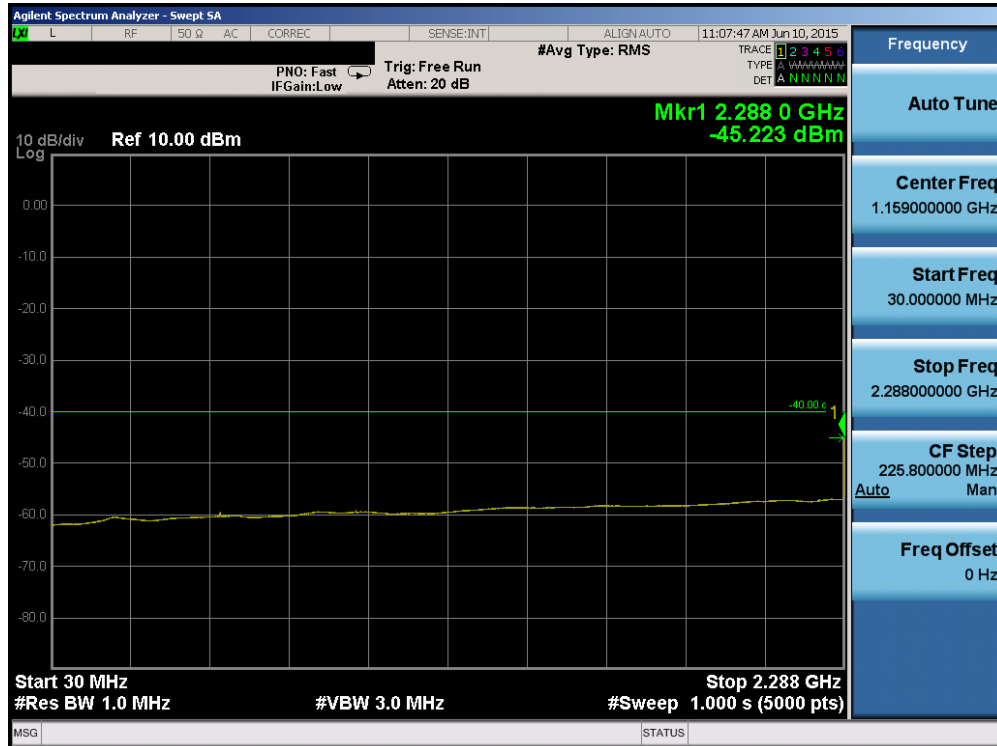
Plot 6-95. Conducted Spurious Plot (Band 30 – 10.0MHz QPSK – RB Size 1, RB Offset 0 – Mid Channel)
