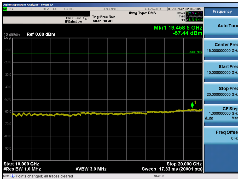
Plot 6-78. Conducted Spurious Plot (Band 4 - 5.0MHz QPSK - RB Size 1, RB Offset 0 - Low Channel)
