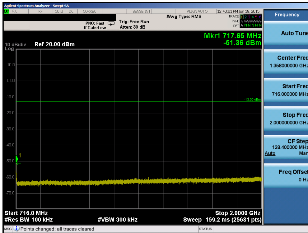
Plot 6-53. Conducted Spurious Plot (Band 12/17 – 5.0MHz QPSK – RB Size 1, RB Offset 0 – Mid Channel)
