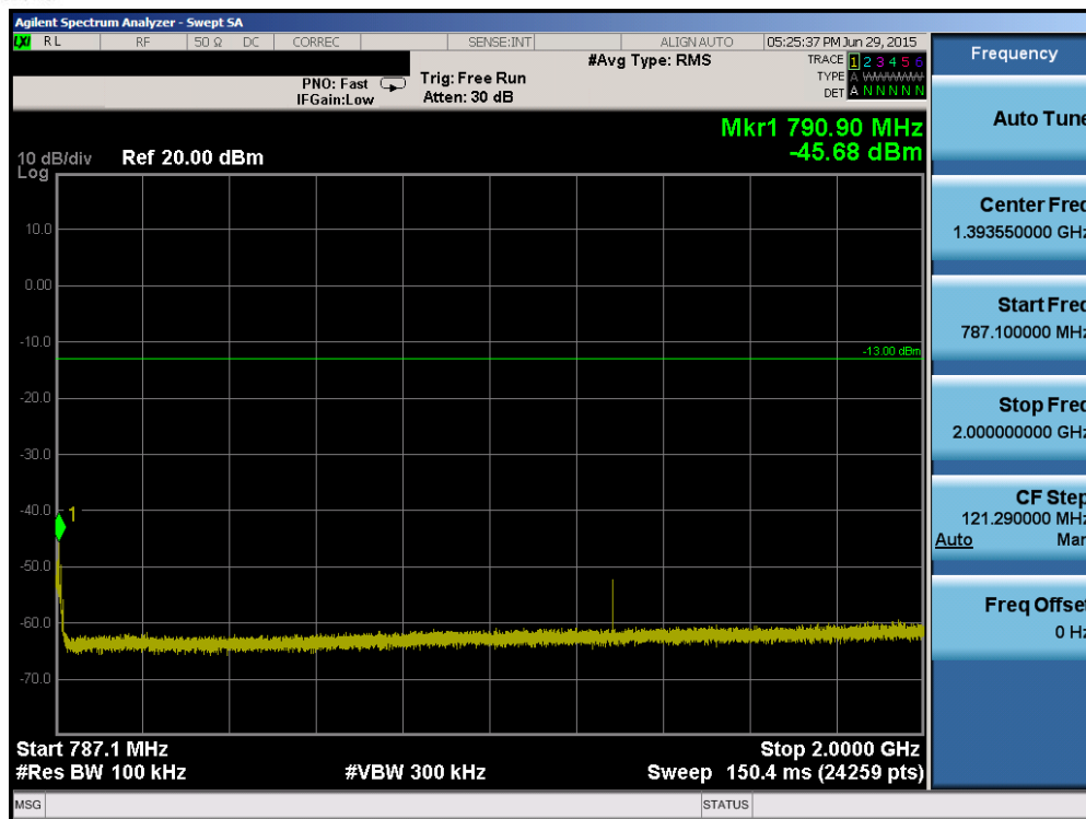
Plot 6-65. Conducted Spurious Plot (Band 13 – 5.0MHz QPSK – RB Size 1, RB Offset 0 – High Channel)
