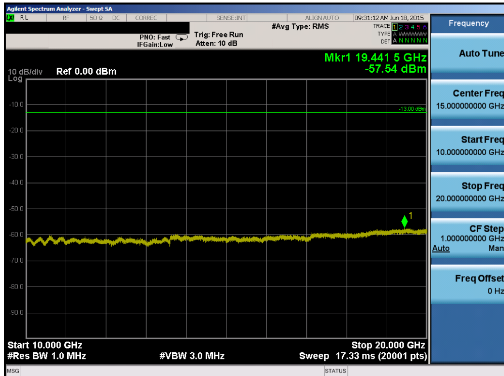
Plot 6-84. Conducted Spurious Plot (Band 4 – 5.0MHz QPSK – RB Size 1, RB Offset 0 – High Channel)
