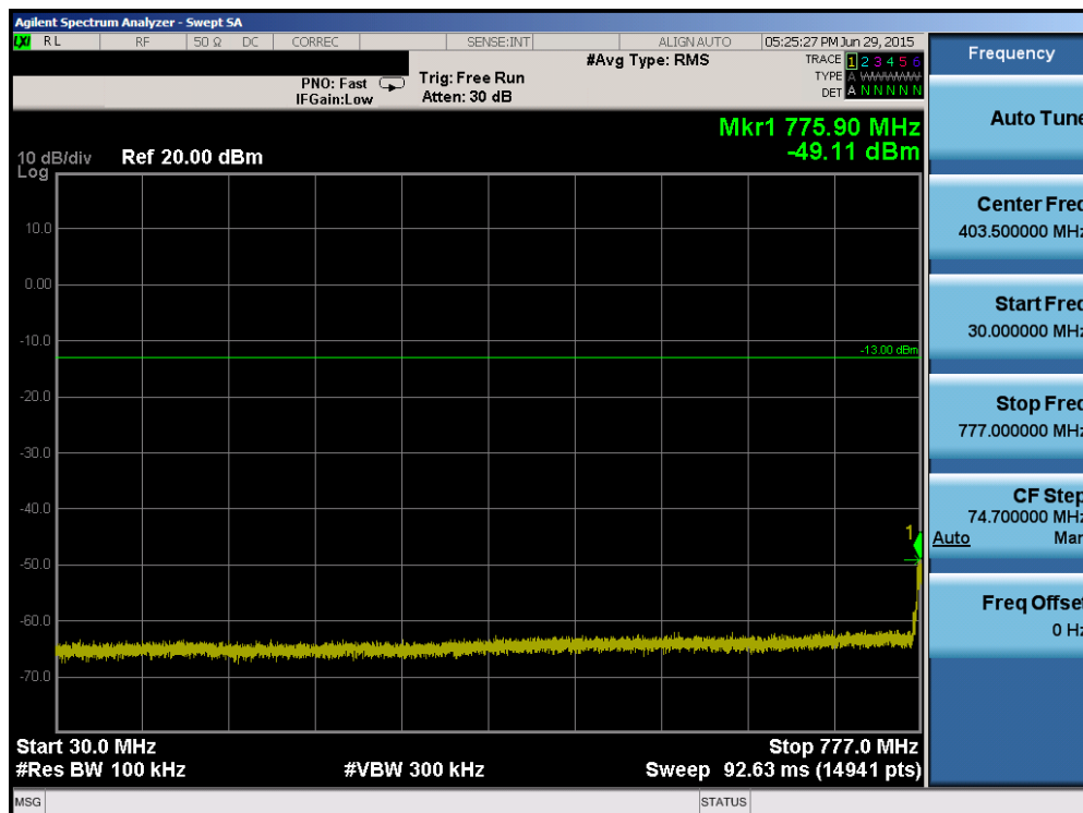
Plot 6-64. Conducted Spurious Plot (Band 13 – 5.0MHz QPSK – RB Size 1, RB Offset 0 – High Channel)
