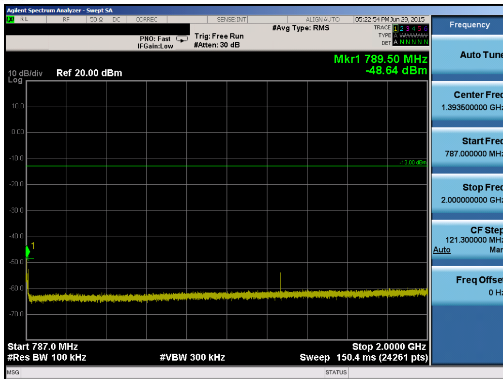
Plot 6-59. Conducted Spurious Plot (Band 13 – 5.0MHz QPSK – RB Size 1, RB Offset 0 – Low Channel)
