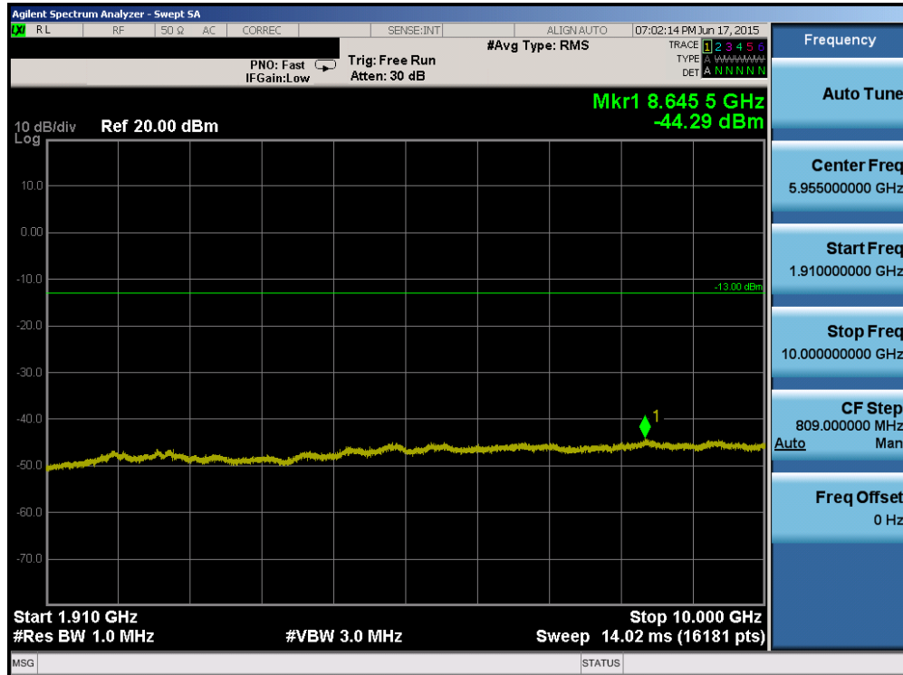
Plot 6-87. Conducted Spurious Plot (Band 2 – 10.0MHz QPSK – RB Size 1, RB Offset 0 – Low Channel)
