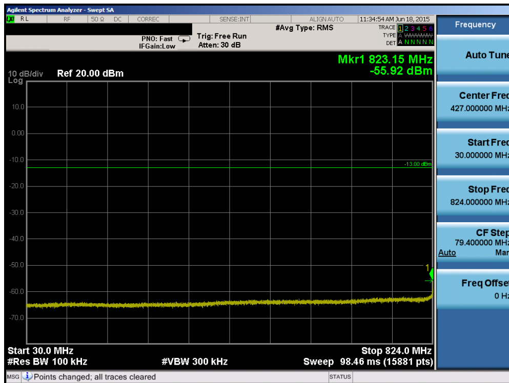
Plot 6-70. Conducted Spurious Plot (Band 5 – 3.0MHz QPSK – RB Size 1, RB Offset 0 – Mid Channel)
