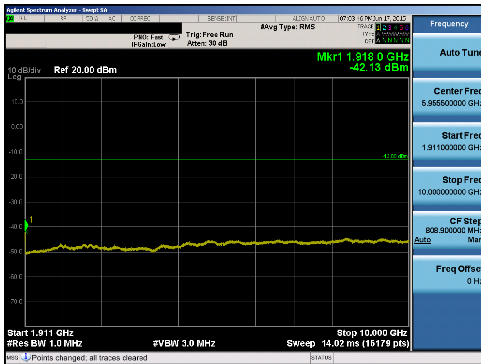
Plot 6-93. Conducted Spurious Plot (Band 2 – 10.0MHz QPSK – RB Size 1, RB Offset 0 – High Channel)
