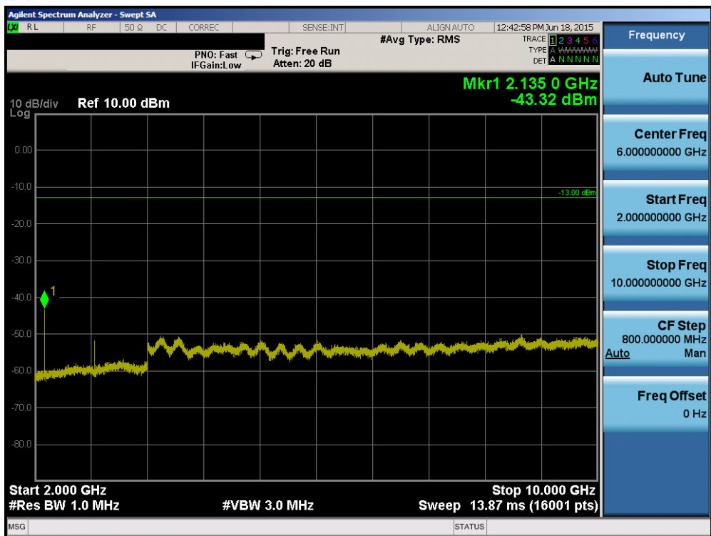
Plot 6-57. Conducted Spurious Plot (Band 12/17 – 5.0MHz QPSK – RB Size 1, RB Offset 0 – High Channel)
