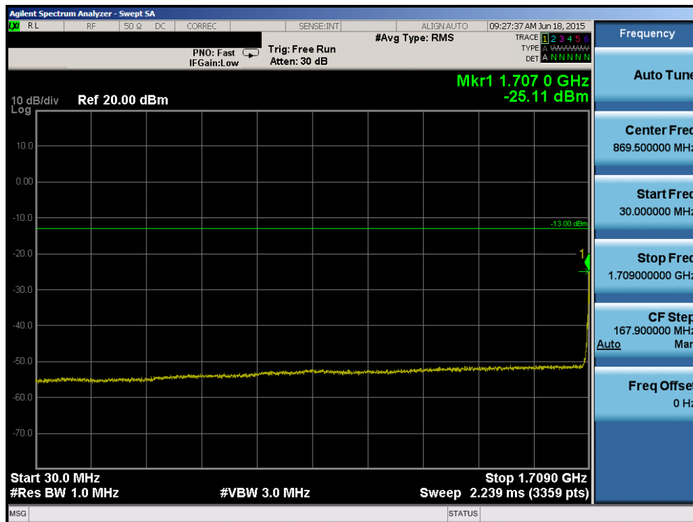
Plot 6-76. Conducted Spurious Plot (Band 4 – 5.0MHz QPSK – RB Size 1, RB Offset 0 – Low Channel)
