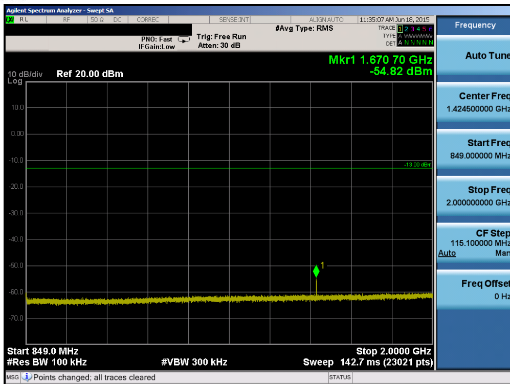
Plot 6-71. Conducted Spurious Plot (Band 5 – 3.0MHz QPSK – RB Size 1, RB Offset 0 – Mid Channel)
