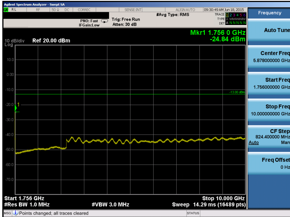
Plot 6-83. Conducted Spurious Plot (Band 4 – 5.0MHz QPSK – RB Size 1, RB Offset 0 – High Channel)
