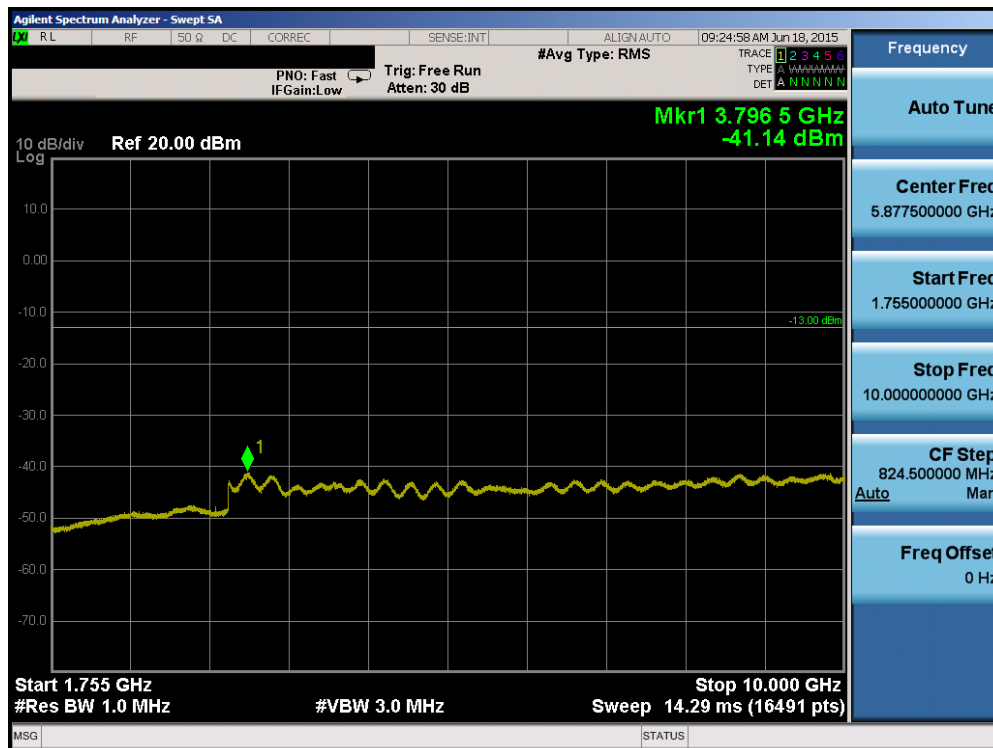
Plot 6-80. Conducted Spurious Plot (Band 4 – 5.0MHz QPSK – RB Size 1, RB Offset 0 – Mid Channel)
