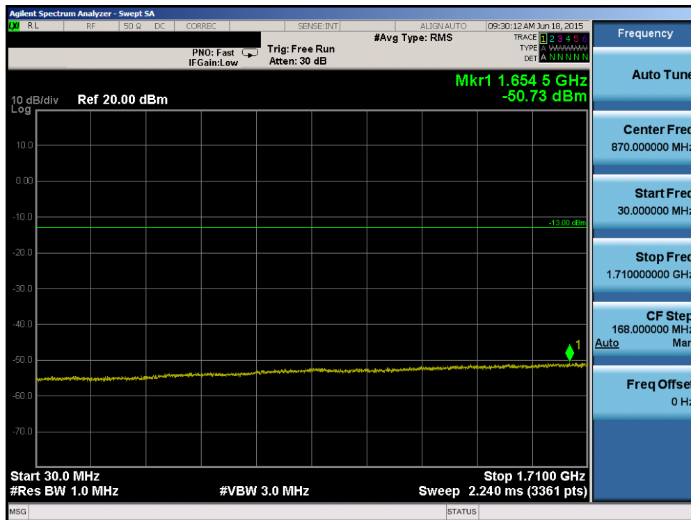
Plot 6-82. Conducted Spurious Plot (Band 4 – 5.0MHz QPSK – RB Size 1, RB Offset 0 – High Channel)
