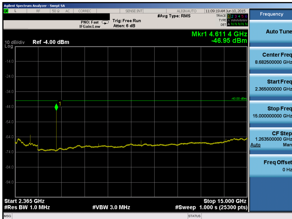
Plot 6-96. Conducted Spurious Plot (Band 30 – 10.0MHz QPSK – RB Size 1, RB Offset 0 – Mid Channel)
