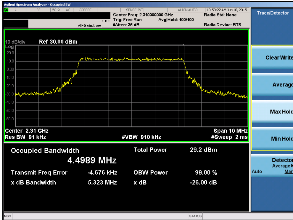
Plot 6-45. Occupied Bandwidth Plot (Band 30 – 5.0MHz QPSK – RB Size 25)
