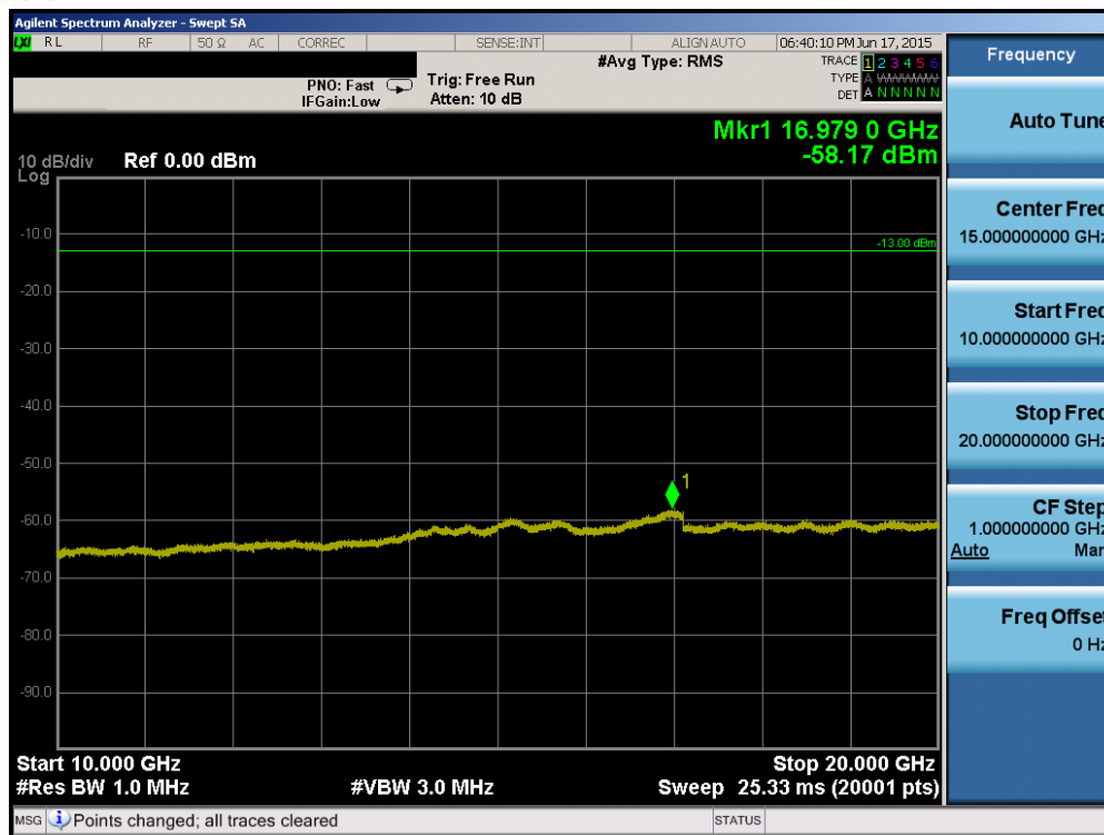
Plot 6-91. Conducted Spurious Plot (Band 2 – 10.0MHz QPSK – RB Size 1, RB Offset 0 – Mid Channel)
