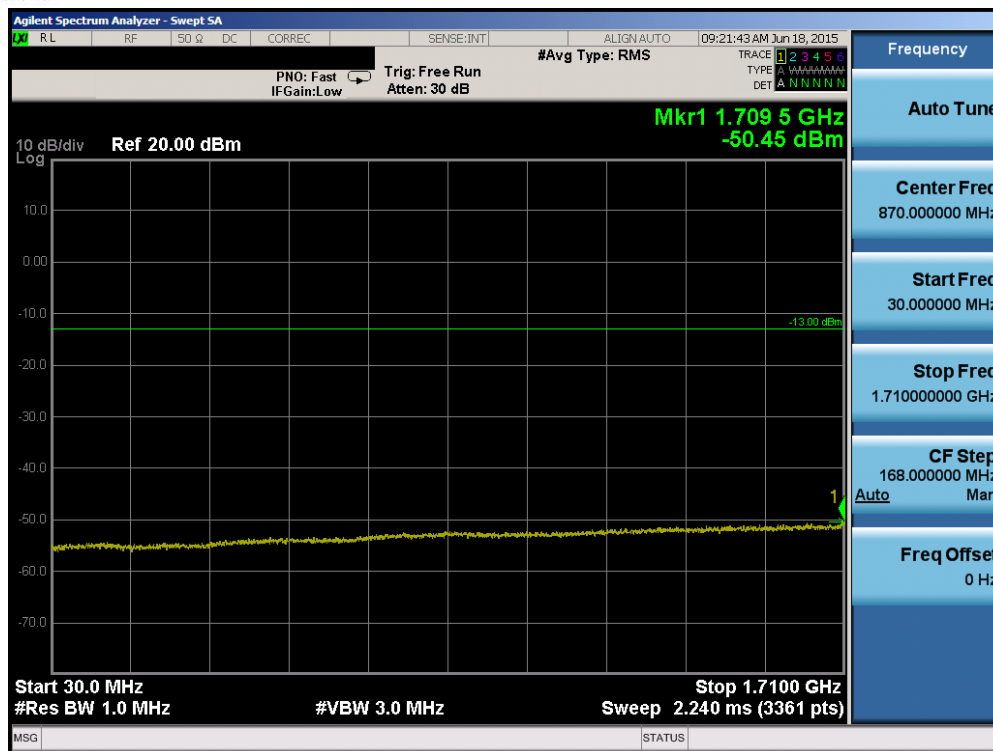
Plot 6-79. Conducted Spurious Plot (Band 4 – 5.0MHz QPSK – RB Size 1, RB Offset 0 – Mid Channel)
