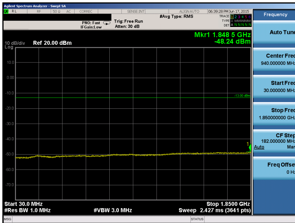
Plot 6-89. Conducted Spurious Plot (Band 2 – 10.0MHz QPSK – RB Size 1, RB Offset 0 – Mid Channel)
