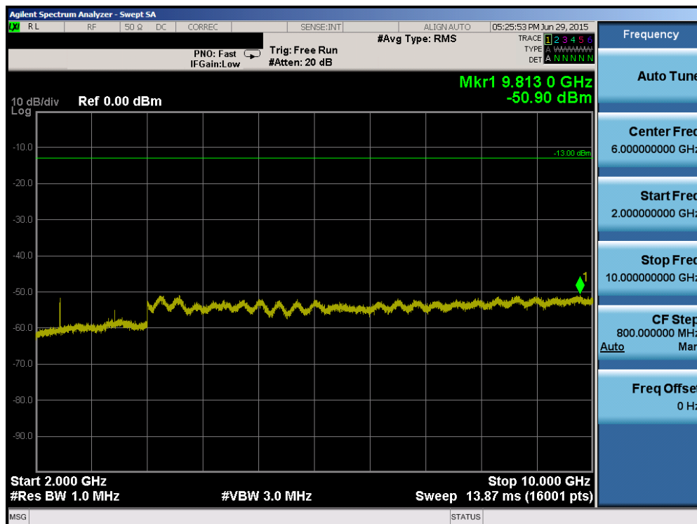
Plot 6-66. Conducted Spurious Plot (Band 13 – 5.0MHz QPSK – RB Size 1, RB Offset 0 – High Channel)
