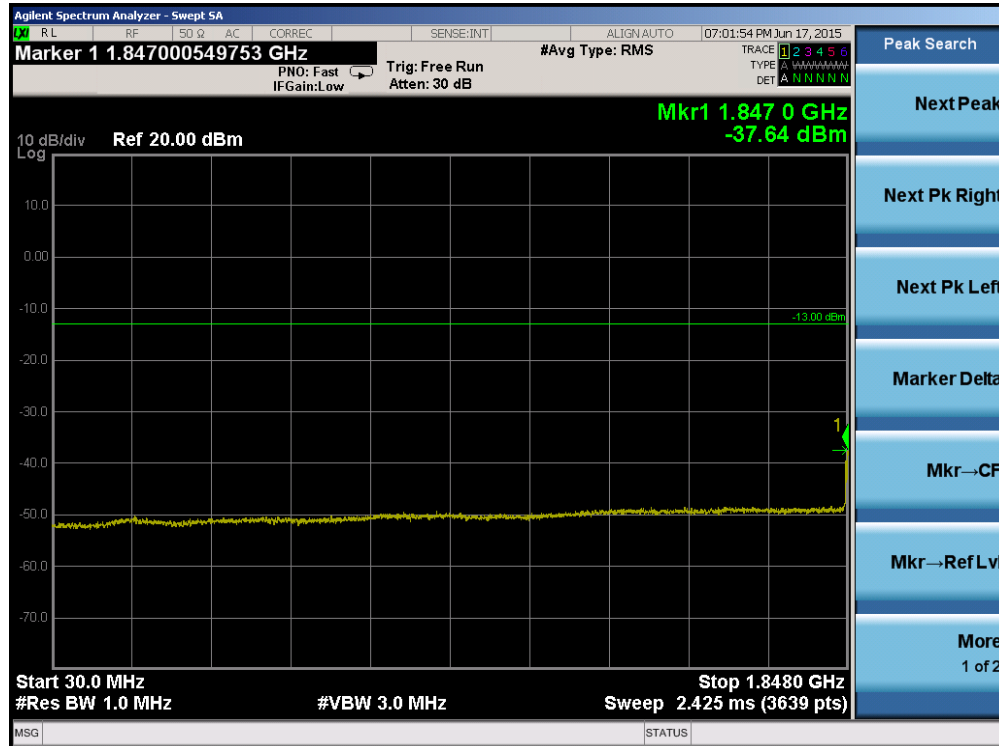
Plot 6-85. Conducted Spurious Plot (Band 2 – 10.0MHz QPSK – RB Size 1, RB Offset 0– Low Channel)
