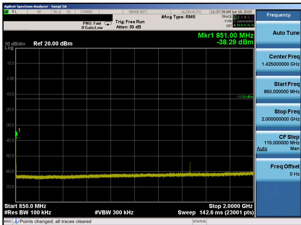
Plot 6-74. Conducted Spurious Plot (Band 5 – 3.0MHz QPSK – RB Size 1, RB Offset 0 – High Channel)
