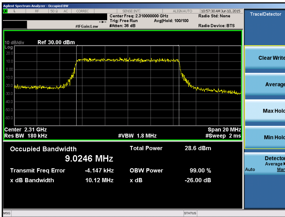
Plot 6-47. Occupied Bandwidth Plot (Band 30 – 10.0MHz QPSK – RB Size 50)
