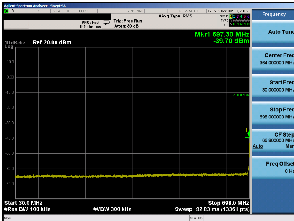
Plot 6-52. Conducted Spurious Plot (Band 12/17 – 5.0MHz QPSK – RB Size 1, RB Offset 0 – Mid Channel)
