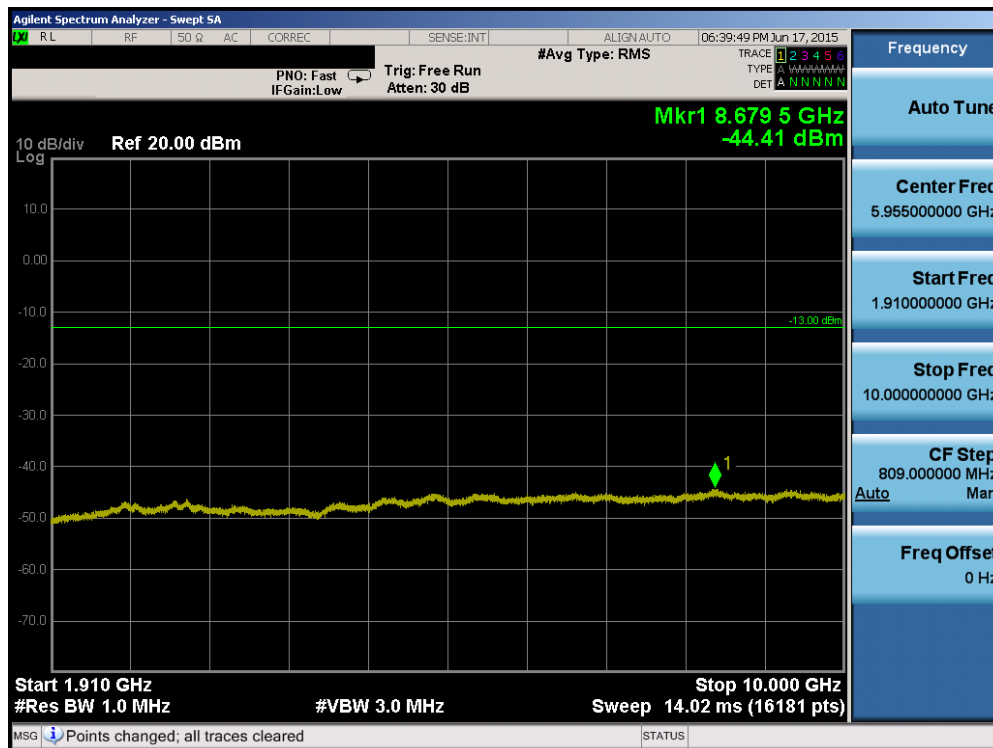
Plot 6-90. Conducted Spurious Plot (Band 2 – 10.0MHz QPSK – RB Size 1, RB Offset 0 – Mid Channel)
