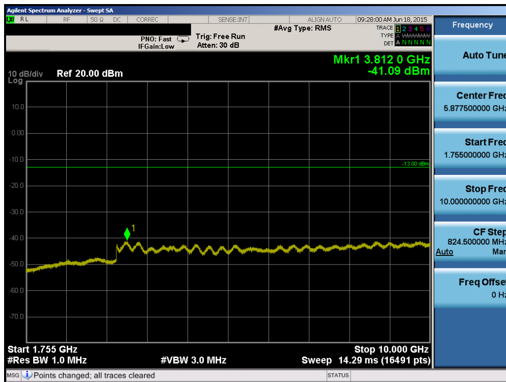
Plot 6-77. Conducted Spurious Plot (Band 4 - 5.0MHz QPSK - RB Size 1, RB Offset 0 - Low Channel)
