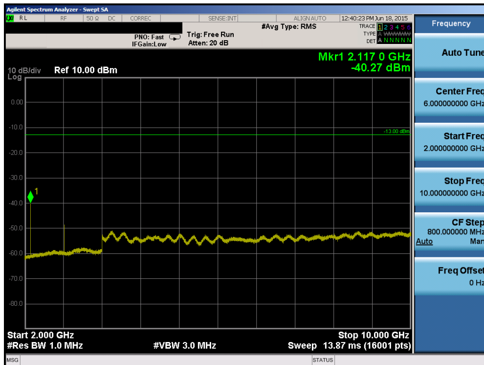
Plot 6-54. Conducted Spurious Plot (Band 12/17 – 5.0MHz QPSK – RB Size 1, RB Offset 0 – Mid Channel)
