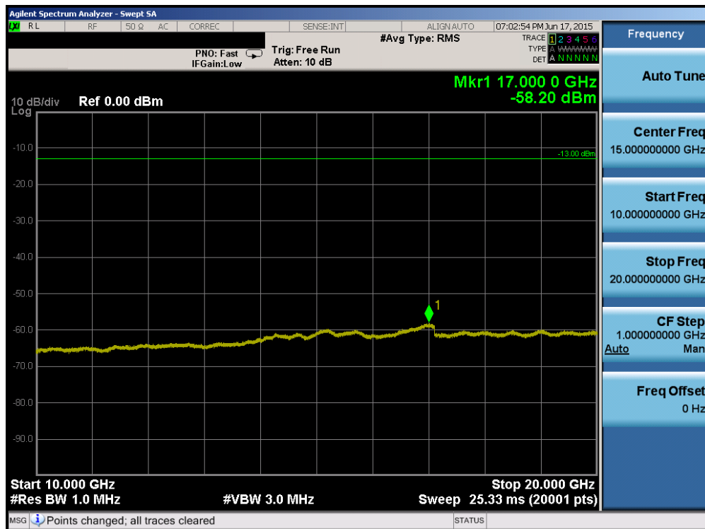
Plot 6-88. Conducted Spurious Plot (Band 2 – 10.0MHz QPSK – RB Size 1, RB Offset 0 – Low Channel)
