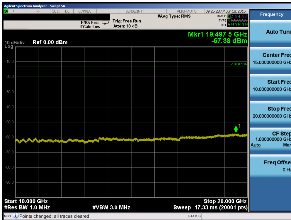
Plot 6-81. Conducted Spurious Plot (Band 4 – 5.0MHz QPSK – RB Size 1, RB Offset 0 – Mid Channel)
