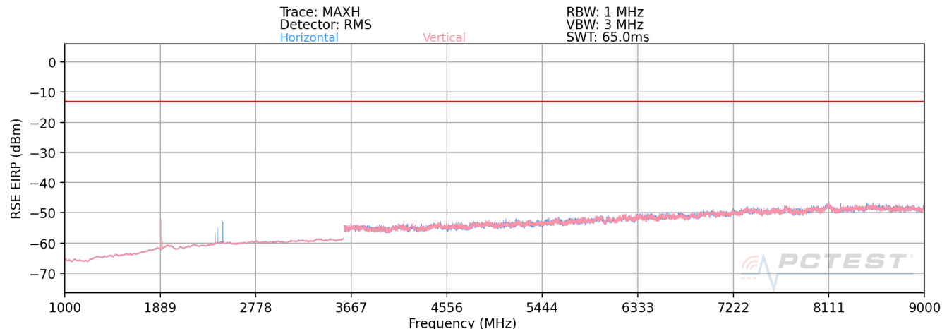
Plot 7-85. Radiated Spurious Plot above 1GHz (Cellular WCDMA Mode)
