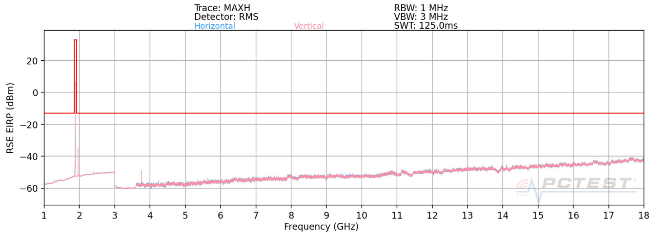
Plot 7-88. Radiated Spurious Plot above 1GHz (PCS WCDMA Mode)
