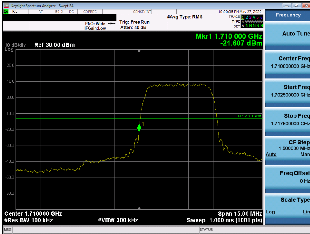
Plot 7-73. Band Edge Plot (AWS WCDMA Mode - Low Channel)
