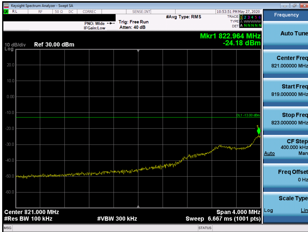
Plot 7-68. 4MHz Span Plot (Cellular CDMA Mode - Low Channel)
