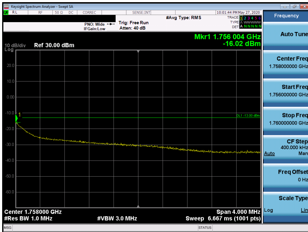
Plot 7-76. 4MHz Span Plot (AWS WCDMA Mode - High Channel)
