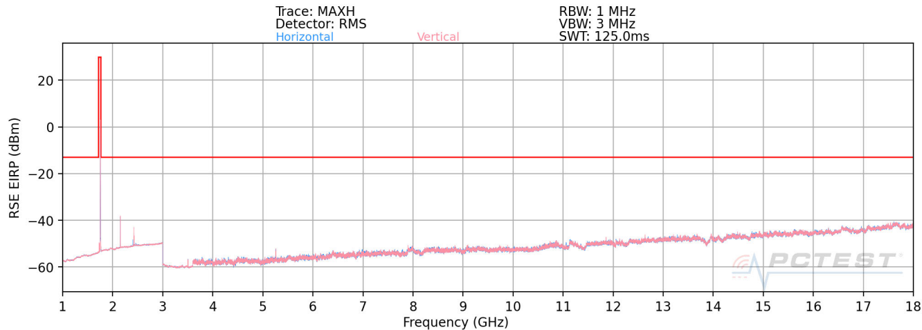
Plot 7-86. Radiated Spurious Plot above 1GHz (AWS WCDMA Mode)
