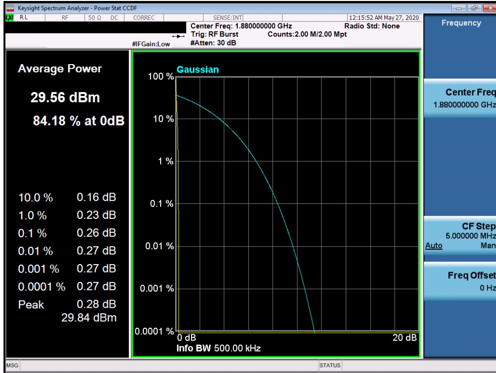
Plot 7-79. Peak-Average Ratio Plot (PCS GPRS Mode)
