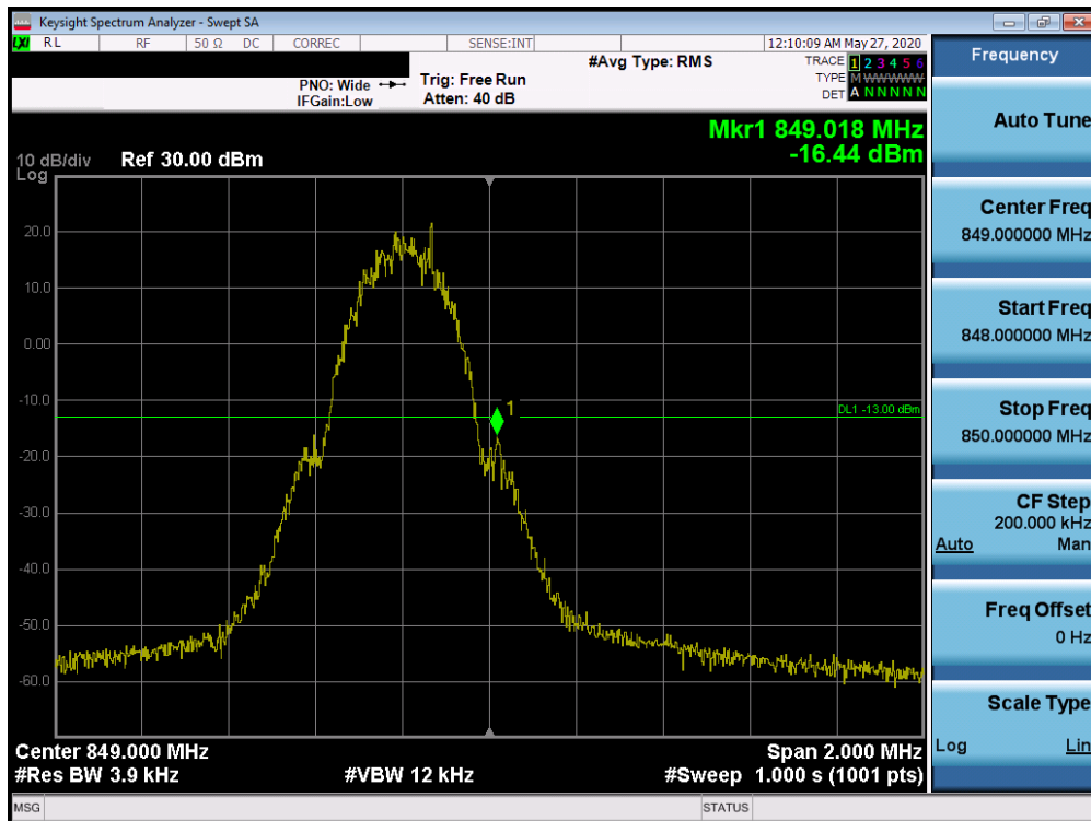
Plot 7-64. Band Edge Plot (Cell GSM Mode - High Channel)
