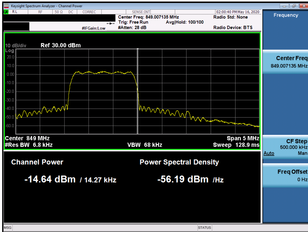
Plot 7-69. Band Edge Plot (Cellular CDMA Mode - High Channel)
