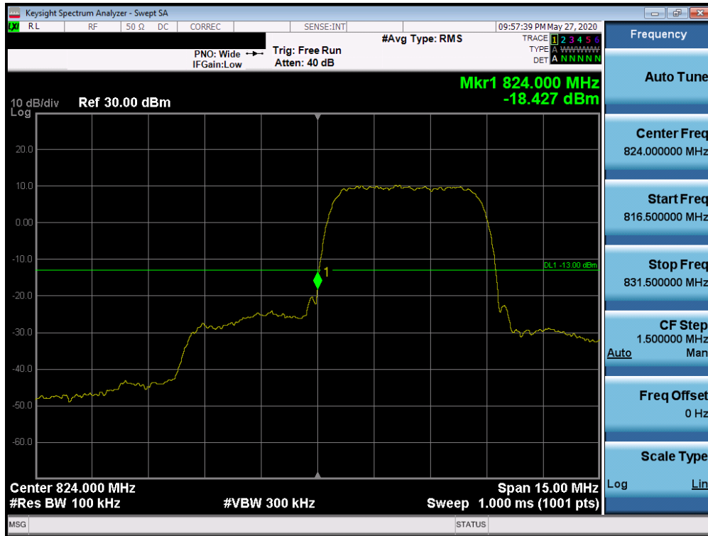
Plot 7-71. Band Edge Plot (Cellular WCDMA Mode - Low Channel)
