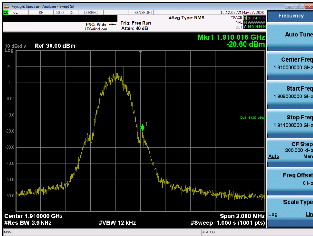
Plot 7-66. Band Edge Plot (PCS GSM Mode - High Channel)
