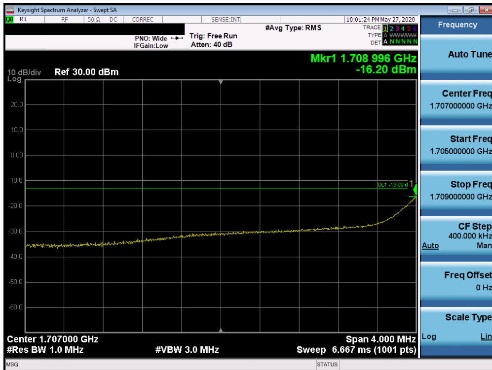
Plot 7-74. 4MHz Span Plot (AWS WCDMA Mode - Low Channel)
