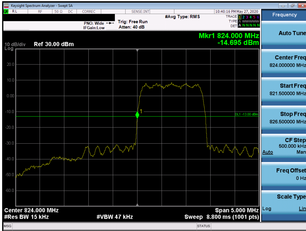
Plot 7-67. Band Edge Plot (Cellular CDMA Mode - Low Channel)
