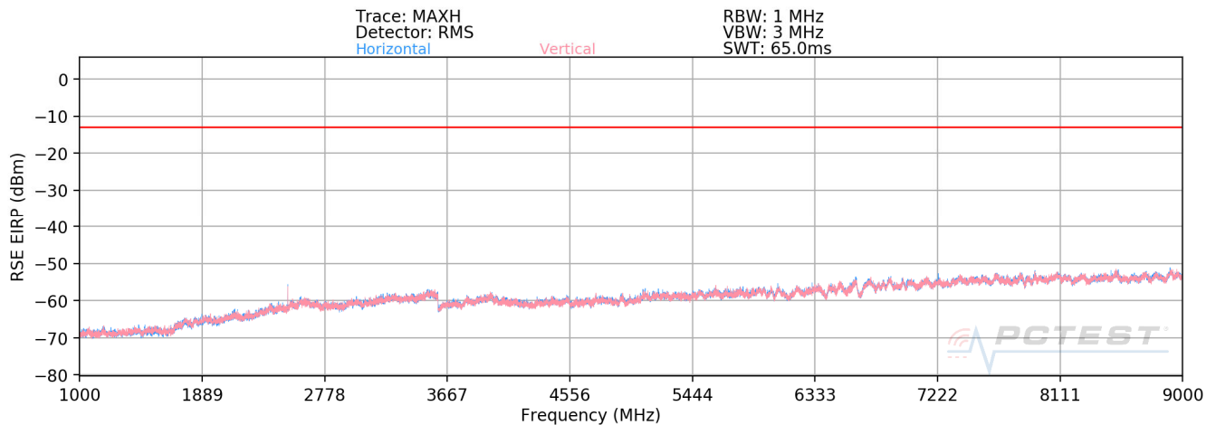
Plot 7-83. Radiated Spurious Plot above 1GHz (Cellular GPRS Mode)
