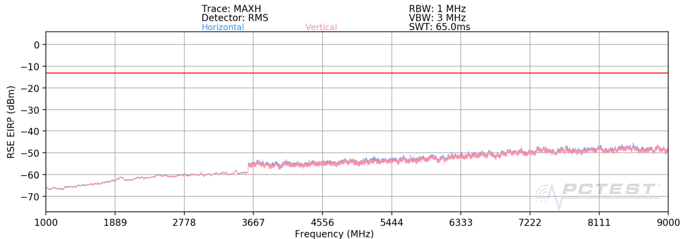
Plot 7-84. Radiated Spurious Plot above 1GHz (Cellular CDMA Mode)
