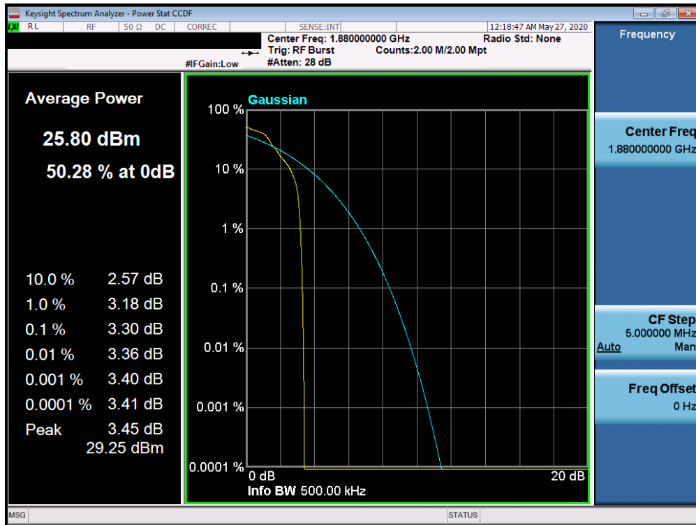
Plot 7-80. Peak-Average Ratio Plot (EDGE1900 Mode)
