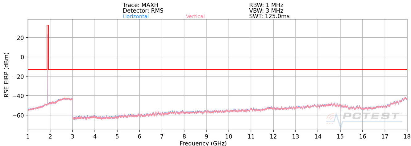
Plot 7-87. Radiated Spurious Plot above 1GHz (PCS GPRS Mode)
