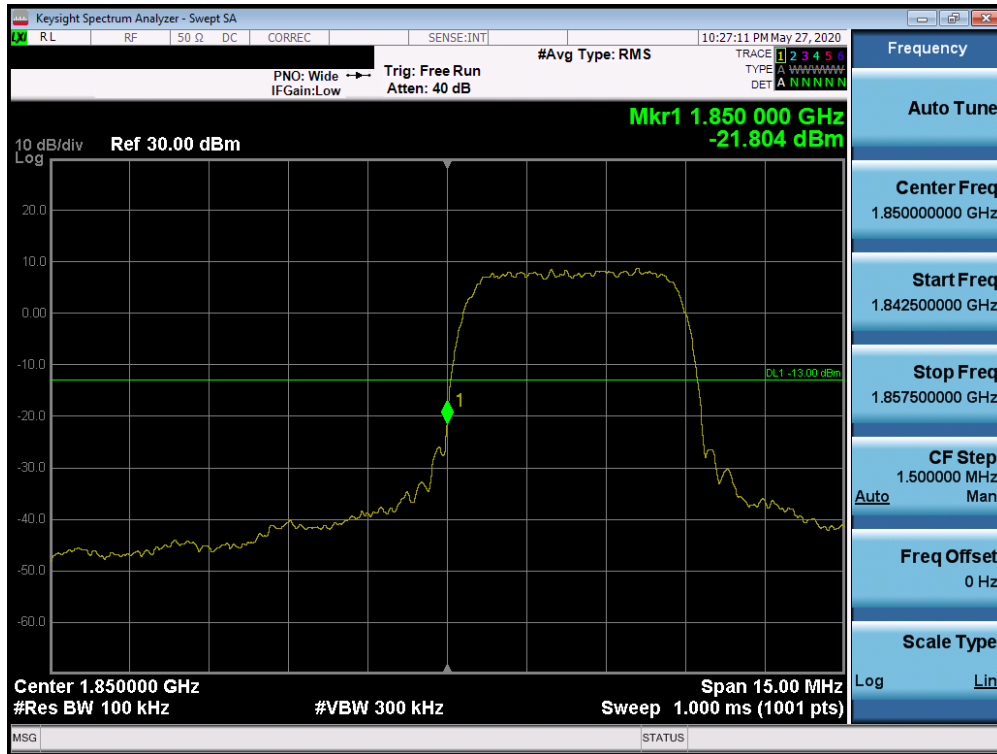
Plot 7-77. Band Edge Plot (PCS WCDMA Mode - Low Channel)
