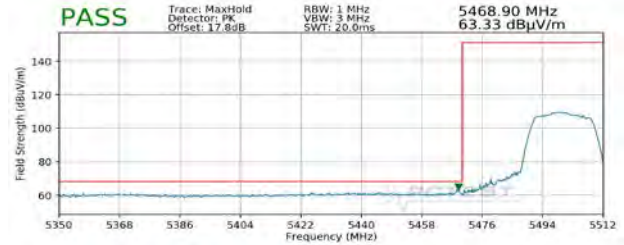
Plot 7-308. Radiated Lower Band Edge Plot SISO ANT2 (Peak - UNII Band 2C)
