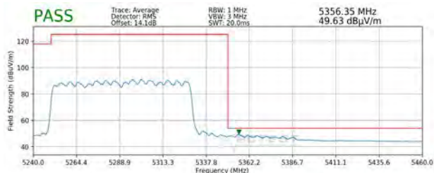
Plot 7-340. Radiated Upper Band Edge Plot MIMO (Average – UNII Band 2A)
