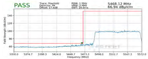
Plot 7-301. Radiated Lower Band Edge Plot SISO ANT1 (Peak - UNII Band 2C)
