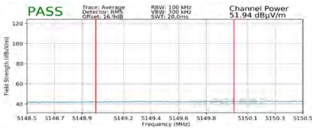
Plot 7-282. Radiated Lower Band Edge Plot SISO ANT1 (Average - UNII Band 1)
