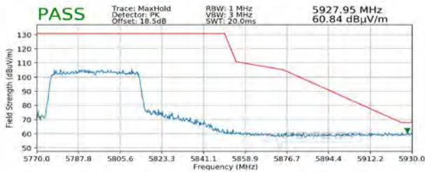
Plot 7-295. Radiated Upper Band Edge Plot SISO ANT1 (Peak - UNII Band 3)
