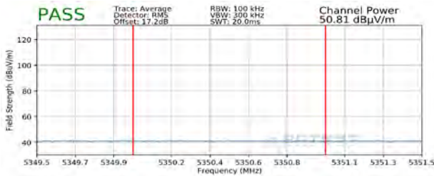
Plot 7-298. Radiated Upper Band Edge Plot SISO ANT1 (Average - UNII Band 2A)
