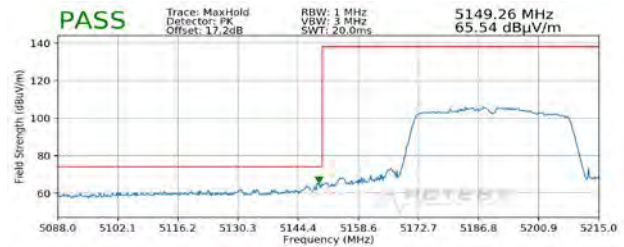
Plot 7-311. Radiated Lower Band Edge Plot SISO ANT2 (Peak - UNII Band 1)
