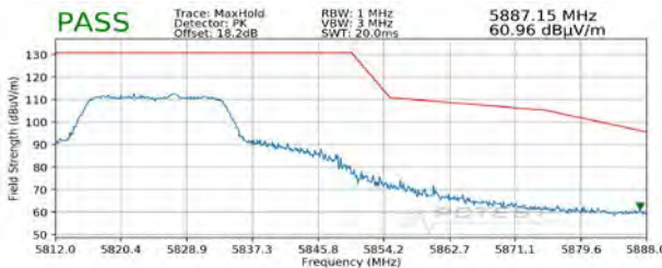
Plot 7-330. Radiated Upper Band Edge Plot MIMO (Peak – UNII Band 3)
