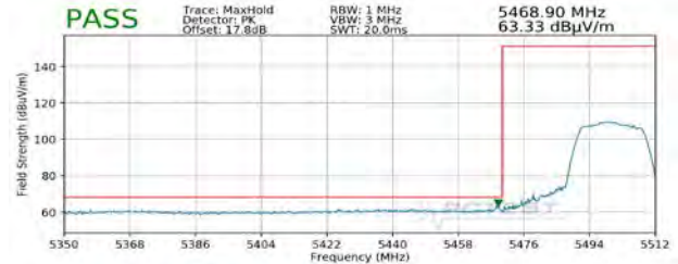
Plot 7-329. Radiated Lower Band Edge Plot MIMO (Peak – UNII Band 2C)
