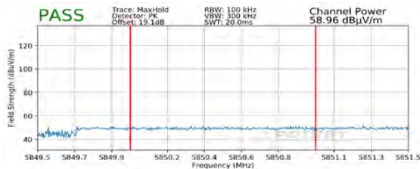
Plot 7-337. Radiated Upper Band Edge Plot MIMO (Peak – UNII Band 3)
