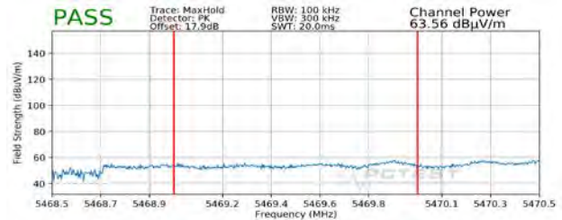
Plot 7-336. Radiated Lower Band Edge Plot MIMO (Peak – UNII Band 2C)
