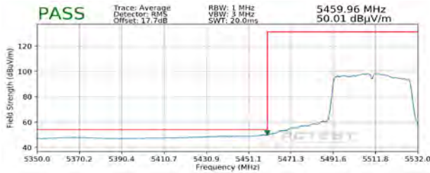
Plot 7-314. Radiated Lower Band Edge Plot SISO ANT2 (Average - UNII Band 2C)
