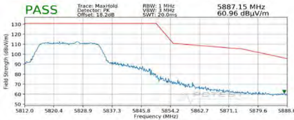
Plot 7-309. Radiated Upper Band Edge Plot SISO ANT2 (Peak - UNII Band 3)
