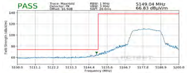
Plot 7-304. Radiated Lower Band Edge Plot SISO ANT2 (Peak - UNII Band 1)
