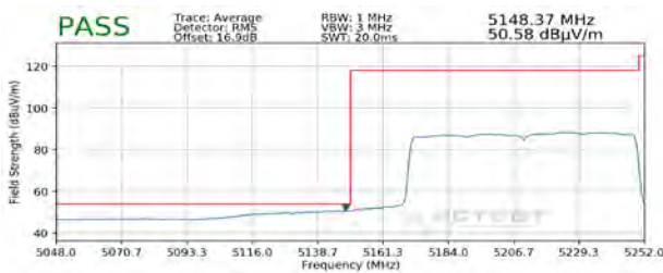
Plot 7-296. Radiated Lower Band Edge Plot SISO ANT1 (Average - UNII Band 1)
