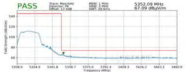
Plot 7-306. Radiated Upper Band Edge Plot SISO ANT2 (Peak - UNII Band 2A)
