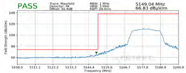
Plot 7-325. Radiated Lower Band Edge Plot MIMO (Peak – UNII Band 1)
