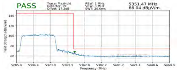
Plot 7-292. Radiated Upper Band Edge Plot SISO ANT1 (Peak - UNII Band 2A)
