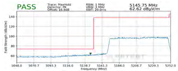
Plot 7-297. Radiated Lower Band Edge Plot SISO ANT1 (Peak - UNII Band 1)
