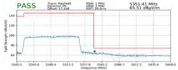
Plot 7-299. Radiated Upper Band Edge Plot SISO ANT1 (Peak - UNII Band 2A)
