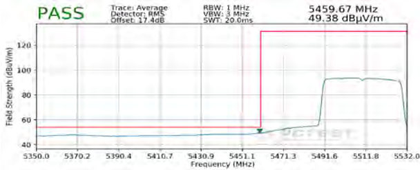
Plot 7-293. Radiated Lower Band Edge Plot SISO ANT1 (Average - UNII Band 2C)
