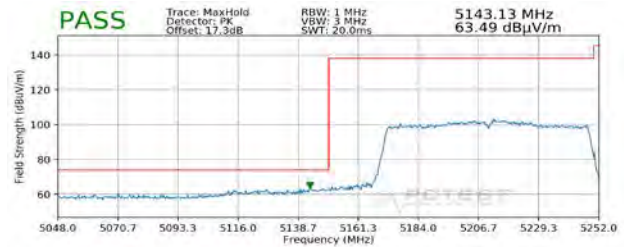
Plot 7-318. Radiated Lower Band Edge Plot SISO ANT2 (Peak – UNII Band 1)
