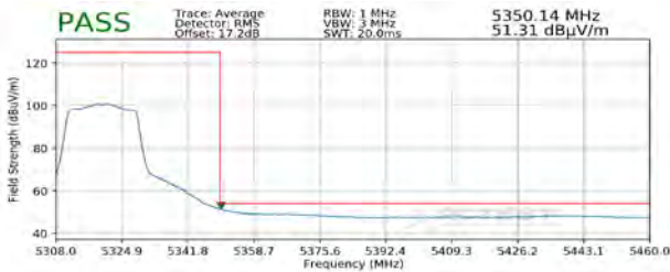
Plot 7-284. Radiated Upper Band Edge Plot SISO ANT1 (Average - UNII Band 2A)
