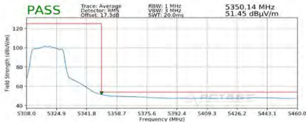
Plot 7-305. Radiated Upper Band Edge Plot SISO ANT2 (Average - UNII Band 2A)
