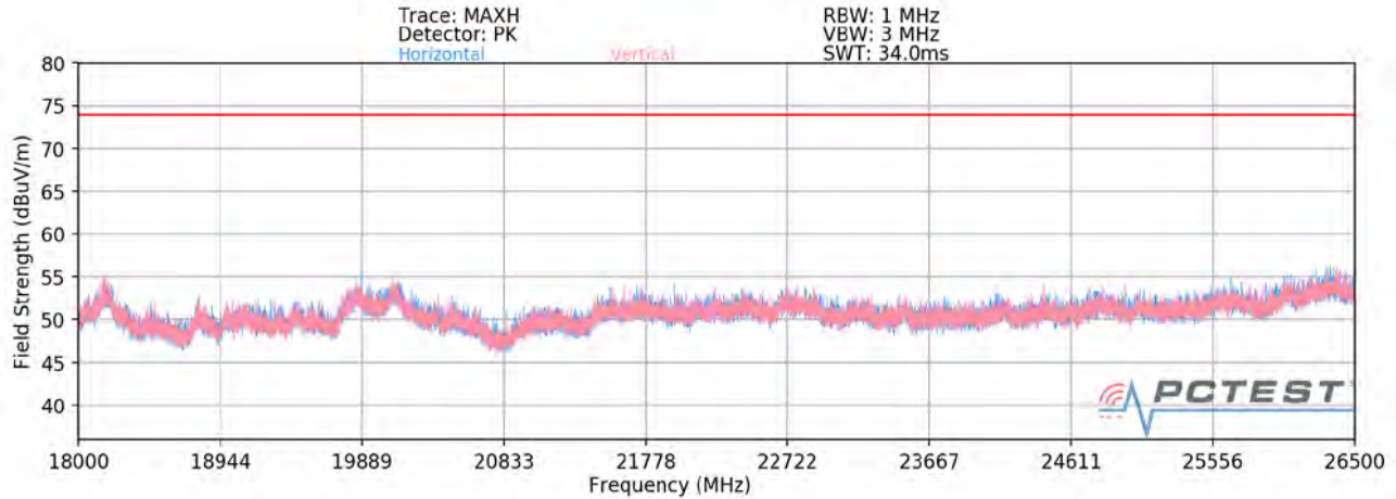
Plot 7-271. Radiated Spurious Plot above 18GHz - 26.5GHz MIMO (802.11a)
