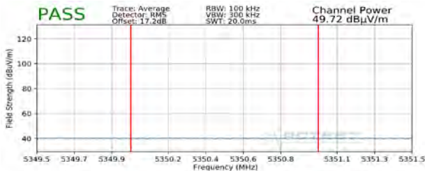
Plot 7-291. Radiated Upper Band Edge Plot SISO ANT1 (Average - UNII Band 2A)
