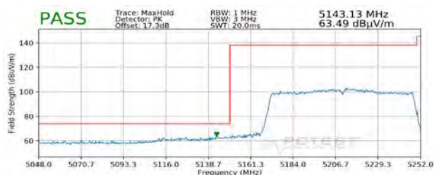
Plot 7-339. Radiated Lower Band Edge Plot MIMO (Peak – UNII Band 1)
