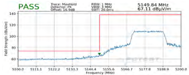
Plot 7-283. Radiated Lower Band Edge Plot SISO ANT1 (Peak - UNII Band 1)
