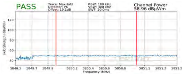
Plot 7-316. Radiated Upper Band Edge Plot SISO ANT2 (Peak - UNII Band 3)
