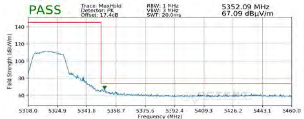
Plot 7-327. Radiated Upper Band Edge Plot MIMO (Peak – UNII Band 2A)
