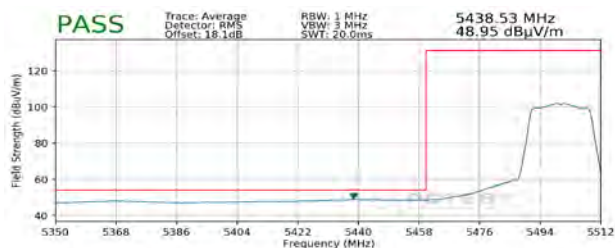
Plot 7-286. Radiated Lower Band Edge Plot SISO ANT1 (Average - UNII Band 2C)
