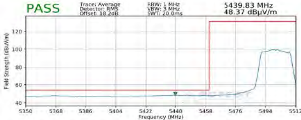
Plot 7-328. Radiated Lower Band Edge Plot MIMO (Average – UNII Band 2C)
