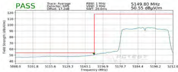
Plot 7-310. Radiated Lower Band Edge Plot SISO ANT2 (Average - UNII Band 1)
