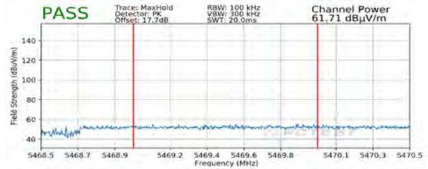
Plot 7-294. Radiated Lower Band Edge Plot SISO ANT1 (Peak - UNII Band 2C)
