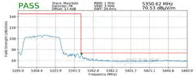
Plot 7-313. Radiated Upper Band Edge Plot SISO ANT2 (Peak - UNII Band 2A)
