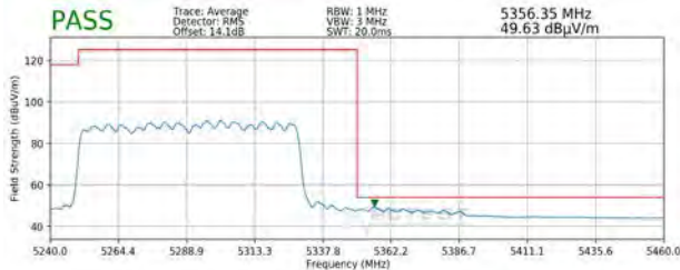
Plot 7-319. Radiated Upper Band Edge Plot SISO ANT2 (Average – UNII Band 2A)
