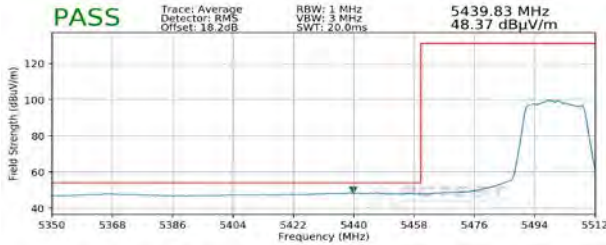
Plot 7-307. Radiated Lower Band Edge Plot SISO ANT2 (Average - UNII Band 2C)
