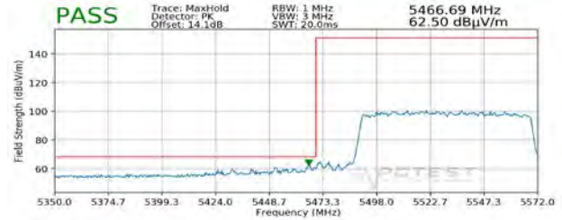
Plot 7-322. Radiated Lower Band Edge Plot SISO ANT2 (Peak - UNII Band 2C)
