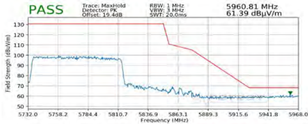
Plot 7-323. Radiated Upper Band Edge Plot SISO ANT2 (Peak - UNII Band 3)
