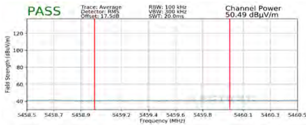
Plot 7-300. Radiated Lower Band Edge Plot SISO ANT1 (Average - UNII Band 2C)
