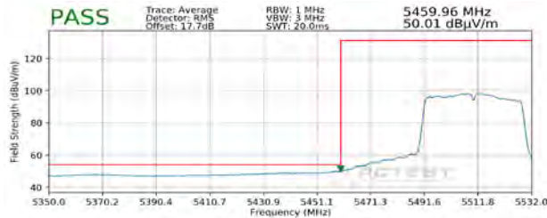
Plot 7-335. Radiated Lower Band Edge Plot MIMO (Average – UNII Band 2C)
