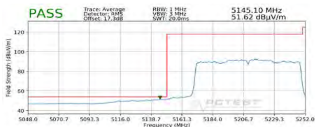
Plot 7-338. Radiated Lower Band Edge Plot MIMO (Average – UNII Band 1)
