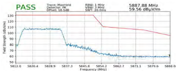
Plot 7-288. Radiated Upper Band Edge Plot SISO ANT1 (Peak - UNII Band 3)
