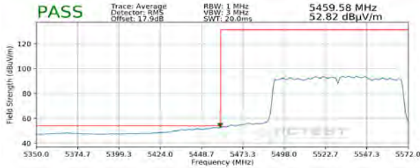
Plot 7-321. Radiated Lower Band Edge Plot SISO ANT2 (Average - UNII Band 2C)
