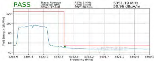
Plot 7-312. Radiated Upper Band Edge Plot SISO ANT2 (Average - UNII Band 2A)
