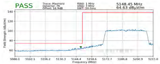
Plot 7-290. Radiated Lower Band Edge Plot SISO ANT1 (Peak - UNII Band 1)
