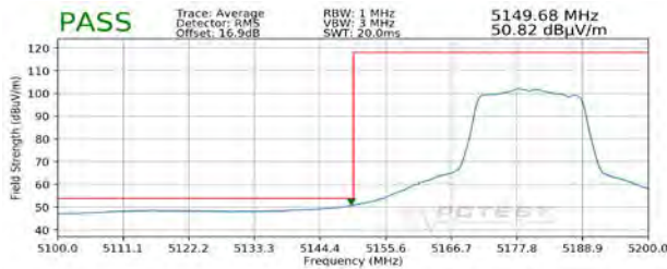
Plot 7-324. Radiated Lower Band Edge Plot MIMO (Average – UNII Band 1)
