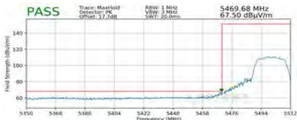
Plot 7-287. Radiated Lower Band Edge Plot SISO ANT1 (Peak - UNII Band 2C)
