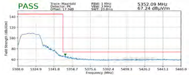
Plot 7-285. Radiated Upper Band Edge Plot SISO ANT1 (Peak - UNII Band 2A)
