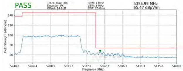
Plot 7-320. Radiated Upper Band Edge Plot SISO ANT2 (Peak – UNII Band 2A)
