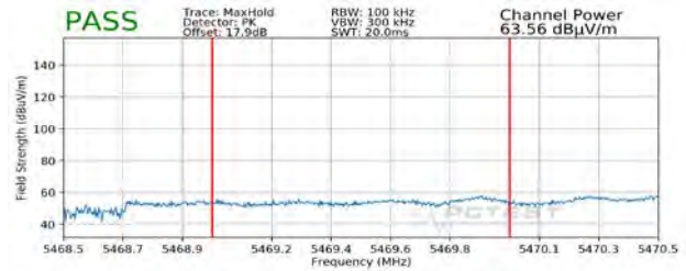
Plot 7-315. Radiated Lower Band Edge Plot SISO ANT2 (Peak - UNII Band 2C)
