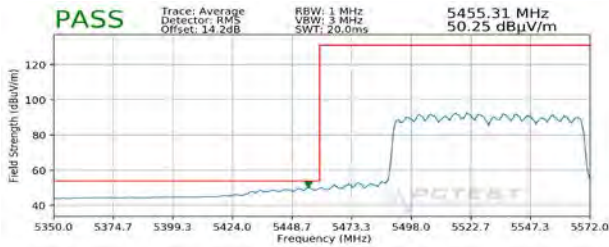
Plot 7-342. Radiated Lower Band Edge Plot MIMO (Average – UNII Band 2C)
