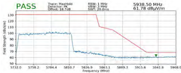
Plot 7-302. Radiated Upper Band Edge Plot SISO ANT1 (Peak - UNII Band 3)
