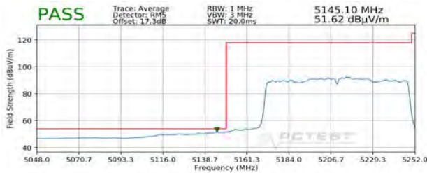
Plot 7-317. Radiated Lower Band Edge Plot SISO ANT2 (Average – UNII Band 1)
