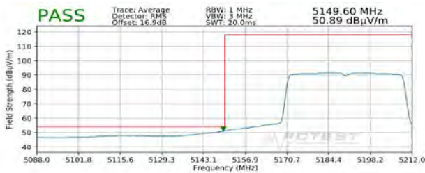
Plot 7-289. Radiated Lower Band Edge Plot SISO ANT1 (Average - UNII Band 1)
