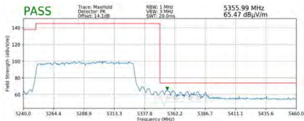
Plot 7-341. Radiated Upper Band Edge Plot MIMO (Peak – UNII Band 2A)
