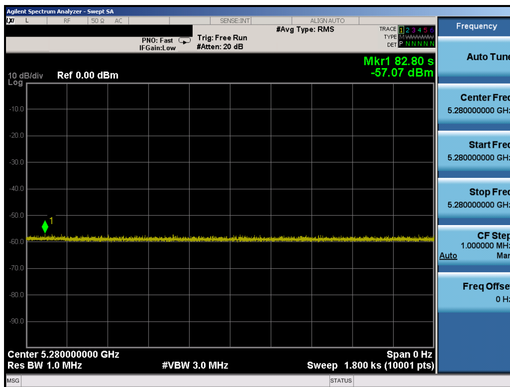
Figure 5-6 Non-occupancy Period - Monitoring live spectrum - Elapse time 30 minutes
