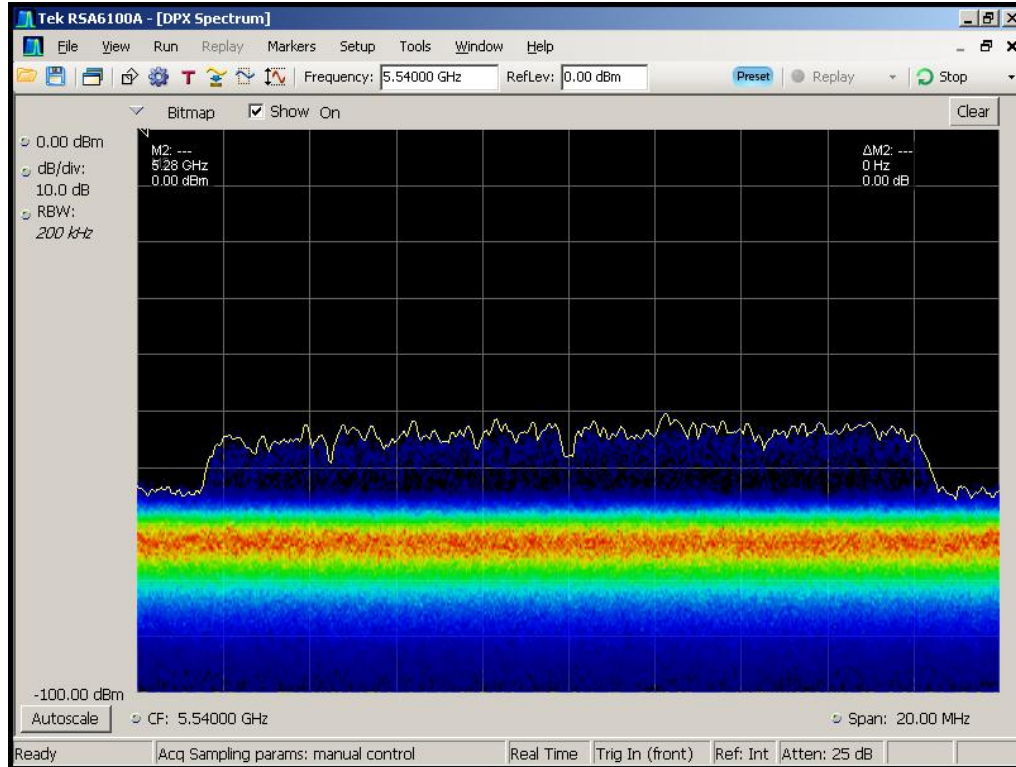
Figure 6-3. Real-Time Spectrum Display, No WLAN Traffic
