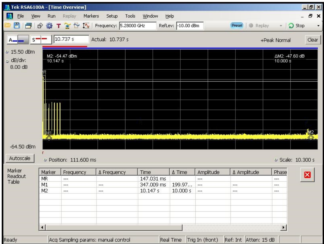
Figure 5-5. Channel Move Time (< 10sec)
