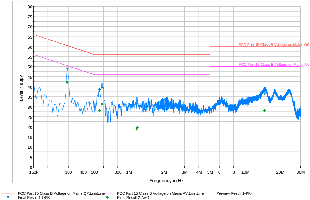
Plot 6-87. Line Conducted Plot with 802.11a UNII Band 3 (N)
