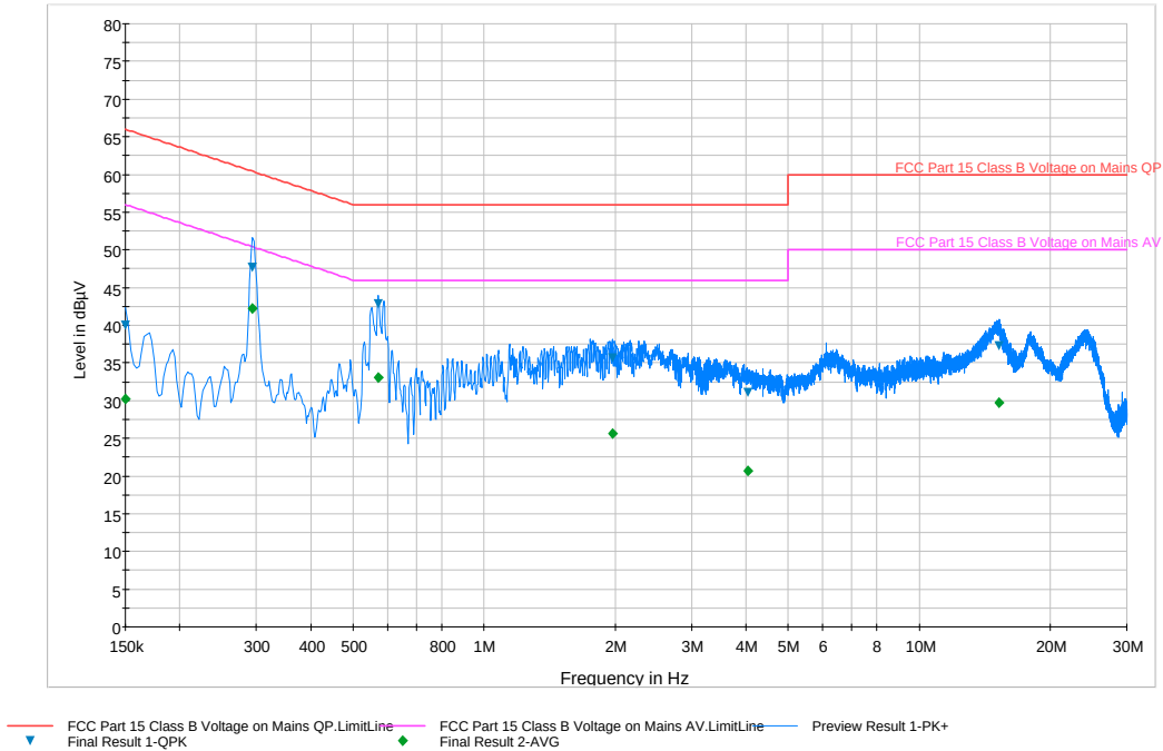
Plot 6-86. Line Conducted Plot with 802.11a UNII Band 3 (L1)
