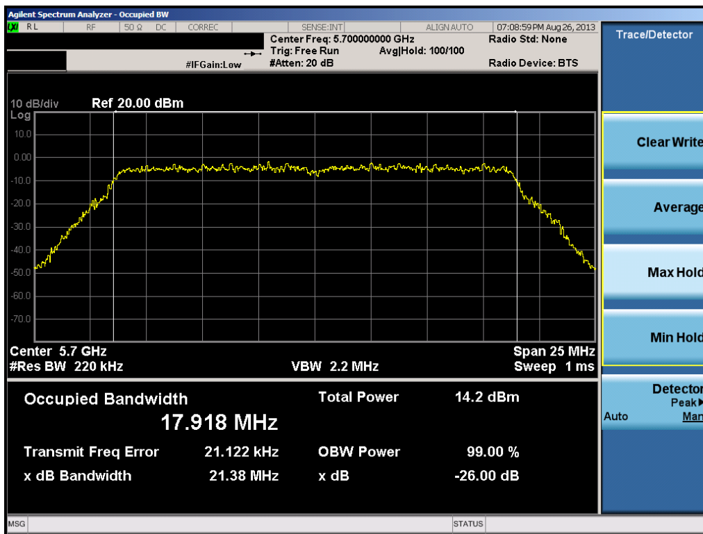
Plot 6-24. 26dB Bandwidth Plot (20MHz BW 802.11n (UNII Band 3) – Ch. 140)
