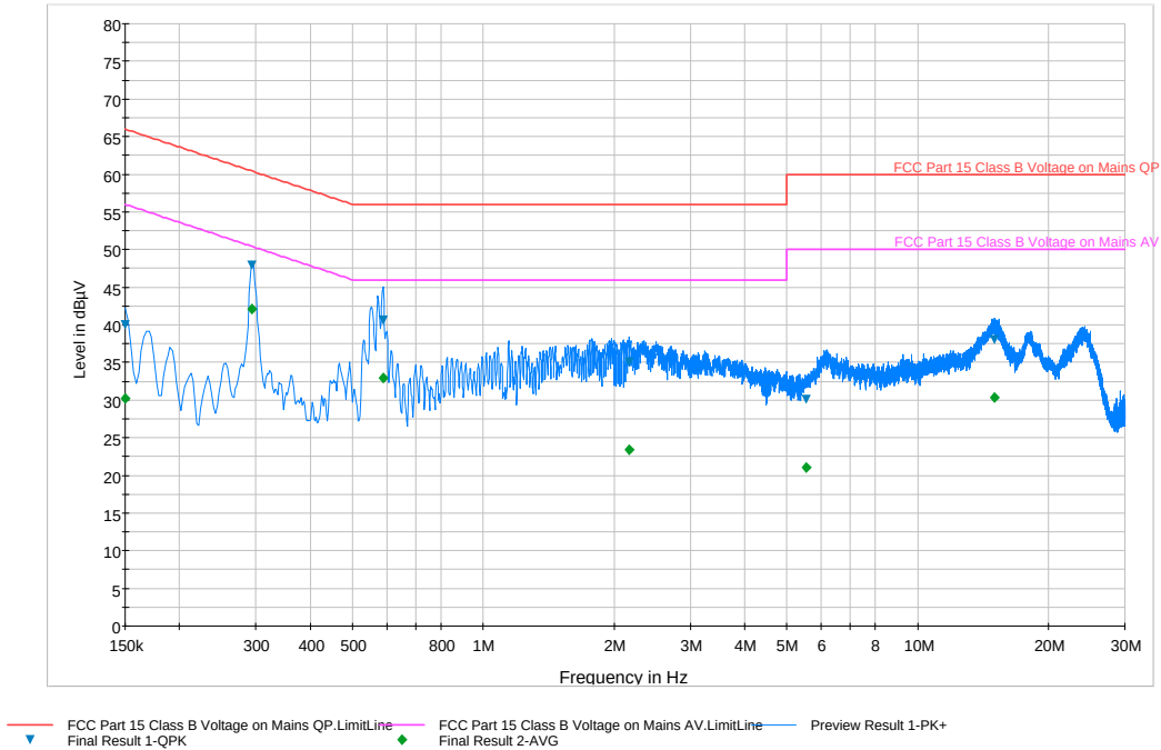
Plot 6-84. Line Conducted Plot with 802.11a UNII Band 2 (L1)
