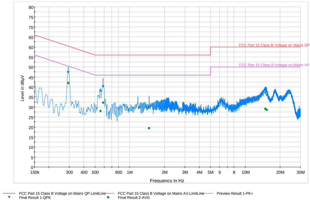
Plot 6-83. Line Conducted Plot with 802.11a UNII Band 1 (N)
