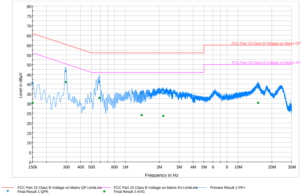
Plot 6-82. Line Conducted Plot with 802.11a UNII Band 1 (L1)
