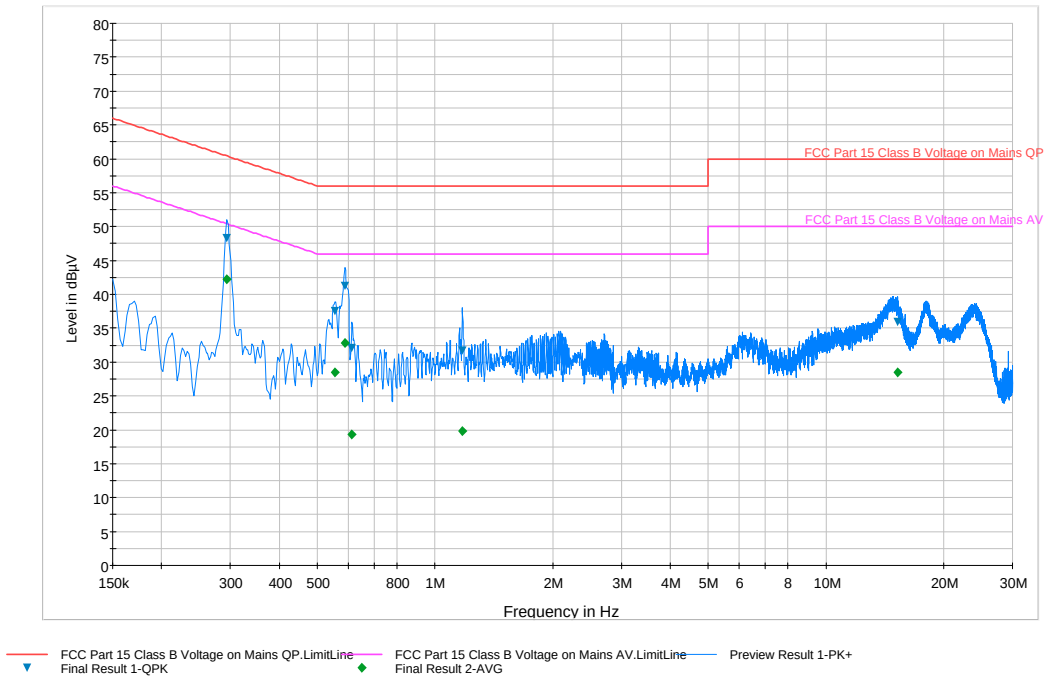
Plot 6-85. Line Conducted Plot with 802.11a UNII Band 2 (N)
