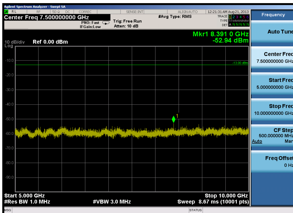
Plot 7-13. Conducted Spurious Plot (5.0MHz QPSK – RB Size 1, RB Offset 0 – Low Channel)
