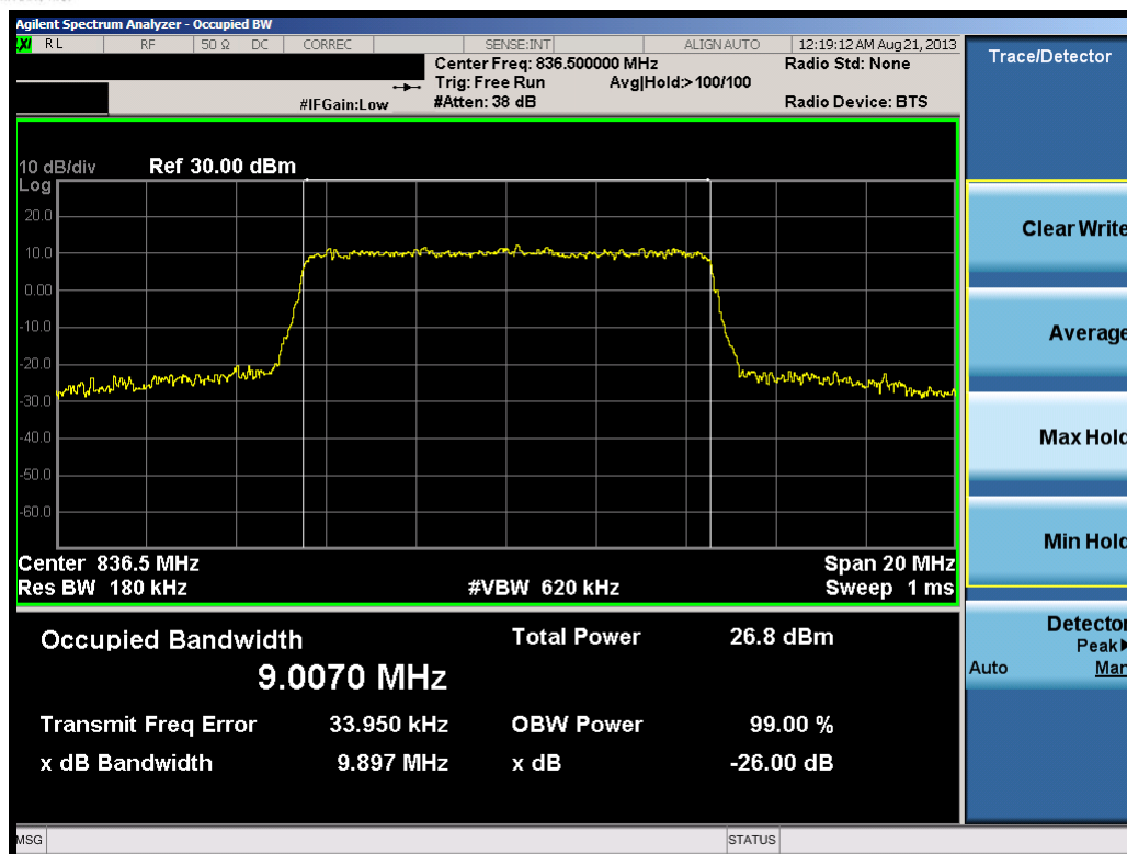
Plot 7-22. Occupied Bandwidth Plot (10.0MHz 16-QAM – RB Size 50)
