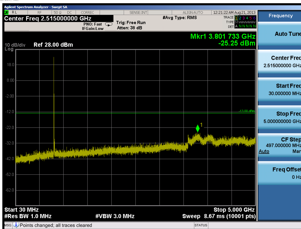
Plot 7-12. Conducted Spurious Plot (5.0MHz QPSK – RB Size 1, RB Offset 0 – Low Channel)
