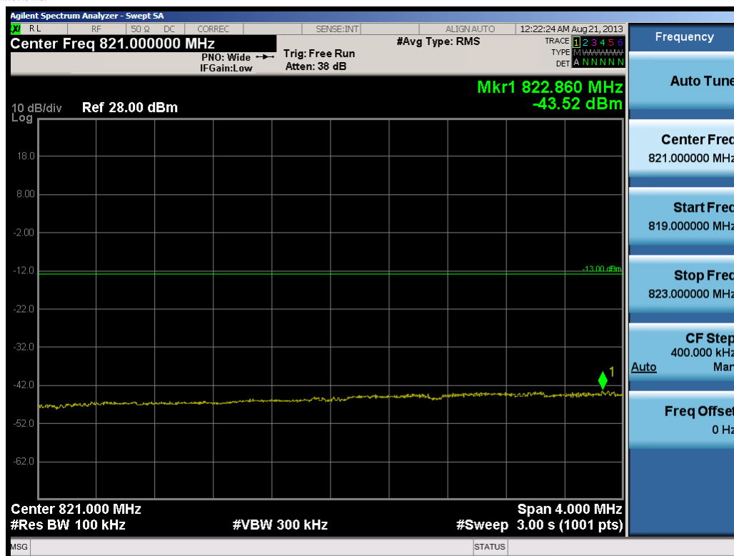
Plot 7-20. Lower Extended Band Edge Plot (10.0MHz QPSK – RB Size 50)
