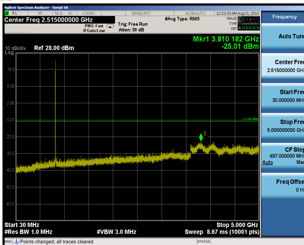
Plot 7-16. Conducted Spurious Plot (5.0MHz QPSK – RB Size 1, RB Offset 0 – High Channel)
