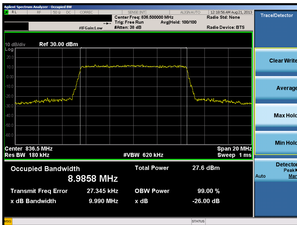
Plot 7-21. Occupied Bandwidth Plot (10.0MHz QPSK – RB Size 50)
