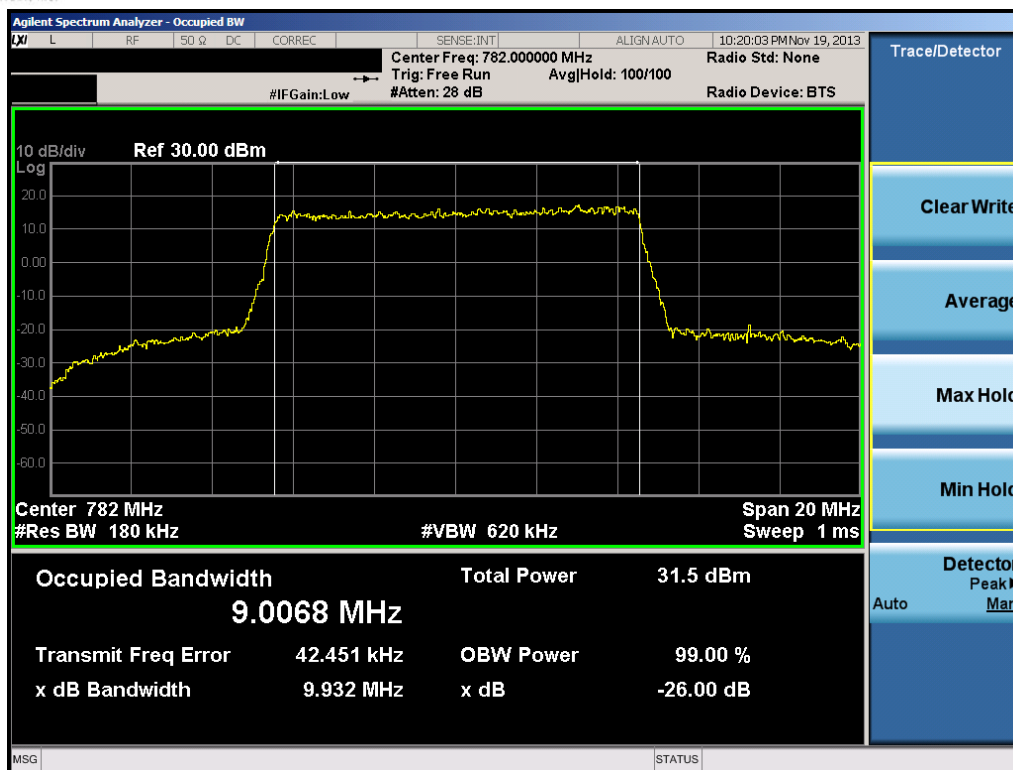
Plot 7-3. Occupied Bandwidth Plot (10.0MHz QPSK – RB Size 50)
