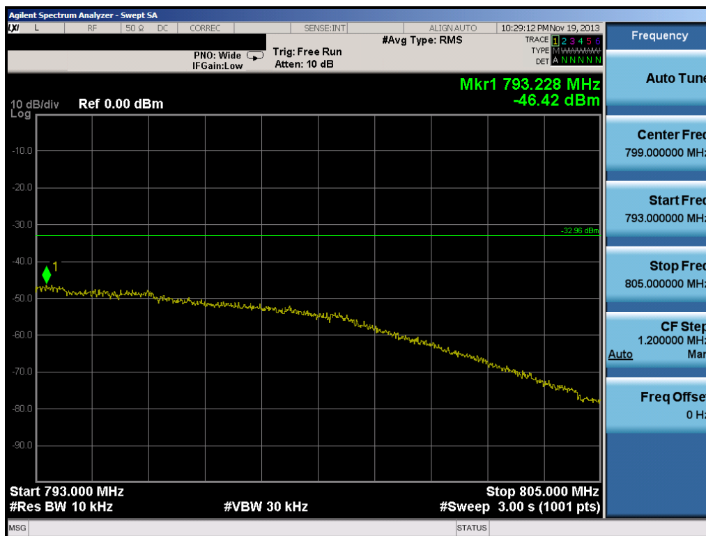
Plot 7-8. Upper Extended Band Edge Plot (10.0MHz QPSK – RB Size 50)
