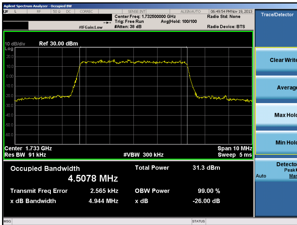
Plot 8-3. Occupied Bandwidth Plot (5.0MHz QPSK – RB Size 25)
