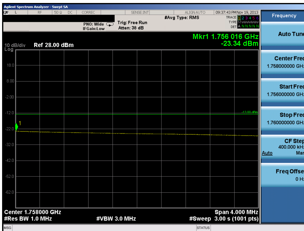
Plot 8-54. Upper Extended Band Edge Plot (20.0MHz QPSK - RB Size 100)
