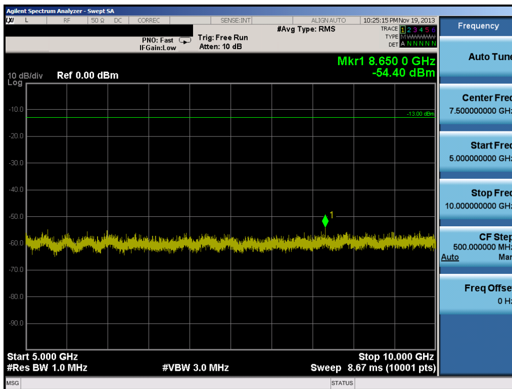
Plot 7-6. Conducted Spurious Plot (10.0MHz QPSK – RB Size 1, RB Offset 0)
