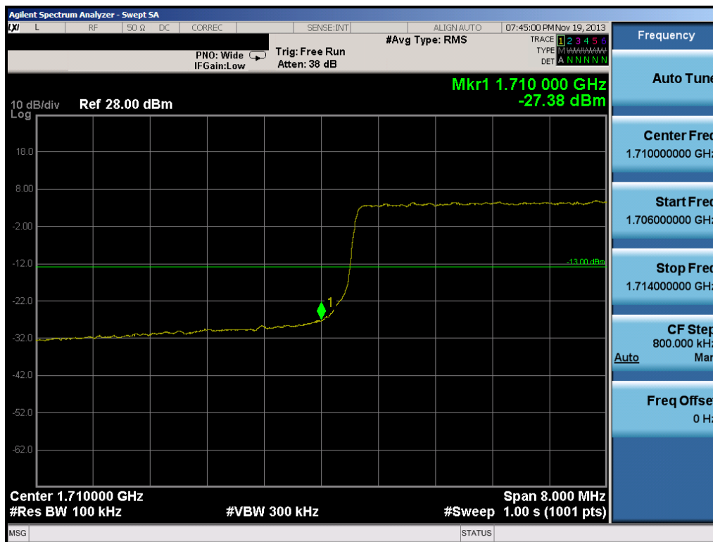
Plot 8-15. Lower Band Edge Plot (10.0MHz QPSK – RB Size 50)
