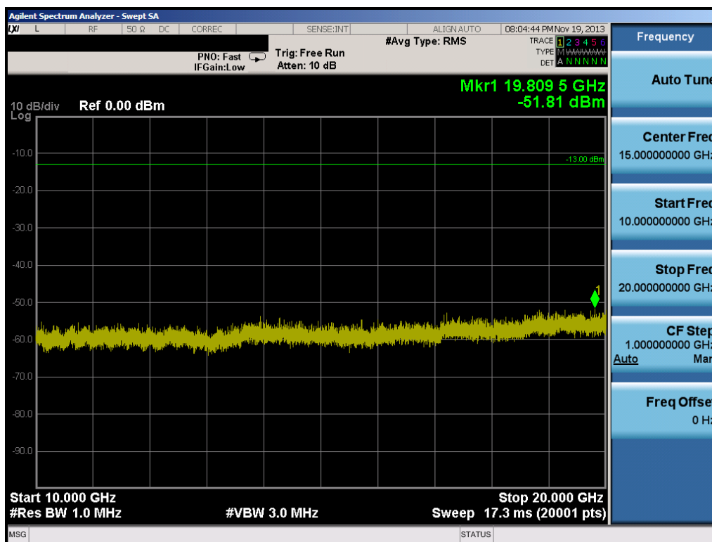
Plot 8-24. Conducted Spurious Plot (10.0MHz QPSK – RB Size 1, RB Offset 0 – High Channel)
