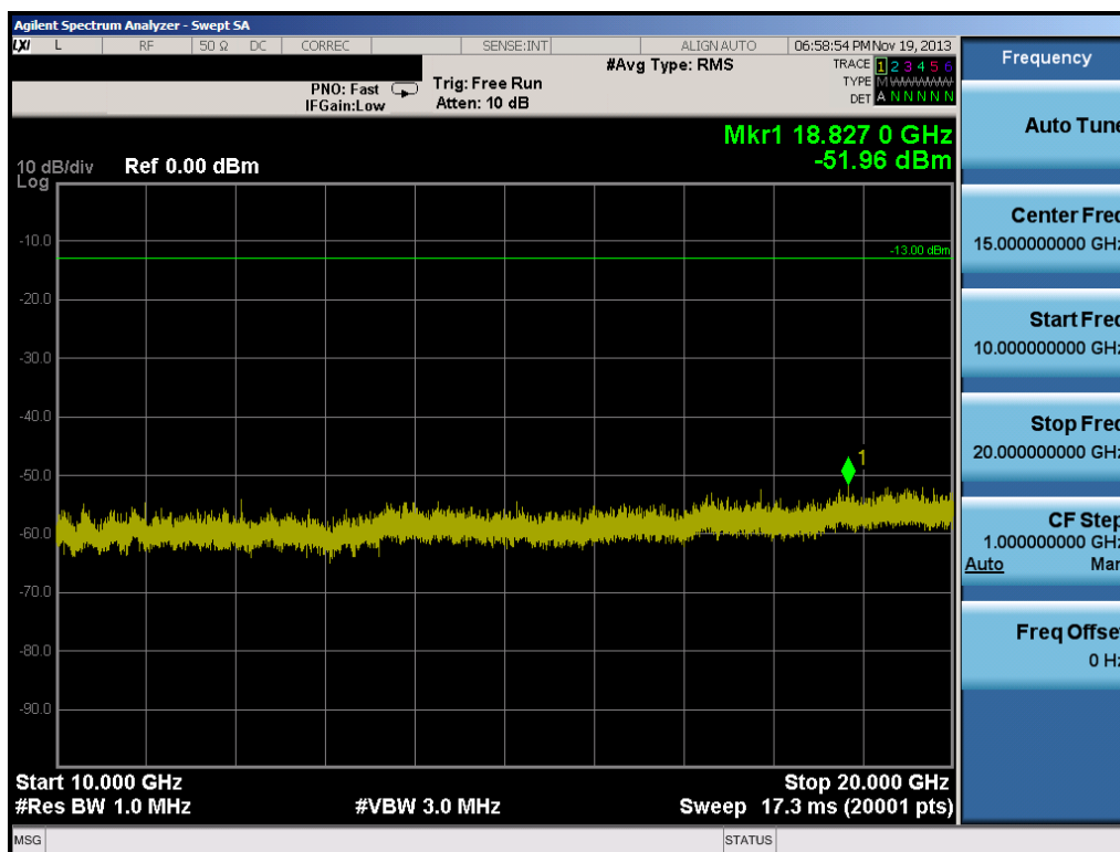
Plot 8-10. Conducted Spurious Plot (5.0MHz QPSK – RB Size 1, RB Offset 0 – High Channel)
