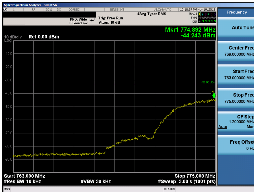
Plot 7-2. Lower Extended Band Edge Plot (10.0MHz QPSK - RB Size 50)
