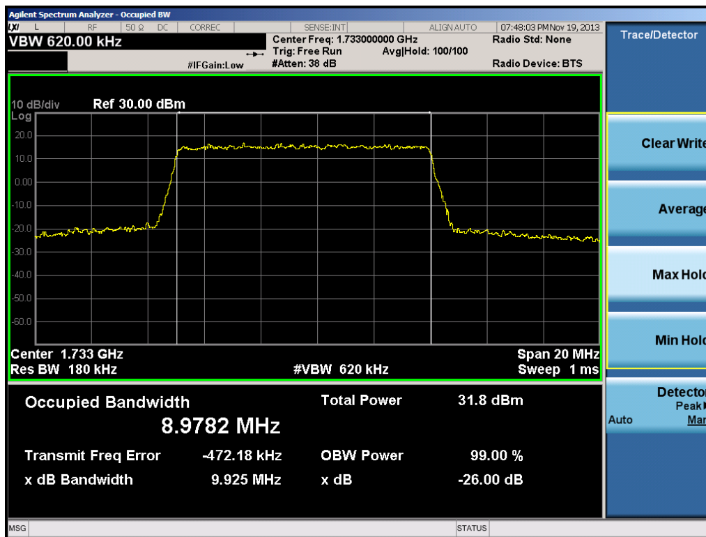
Plot 8-17. Occupied Bandwidth Plot (10.0MHz QPSK – RB Size 50)
