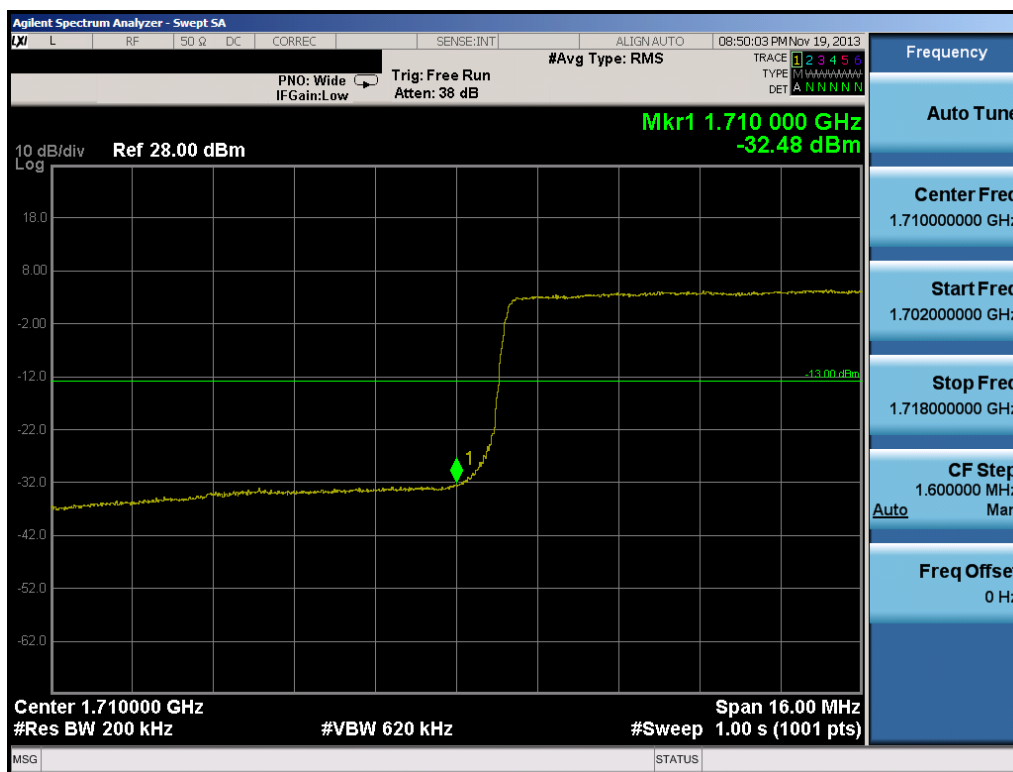
Plot 8-43. Lower Band Edge Plot (20.0MHz QPSK - RB Size 100)
