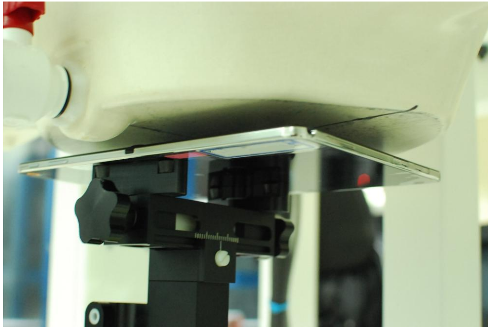
SAR Test Setup Photo 2 – Back Side at 13 mm
