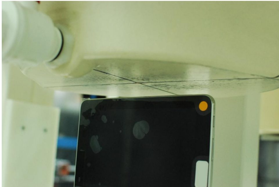
SAR Test Setup Photo 6 – Left Edge at 14 mm
