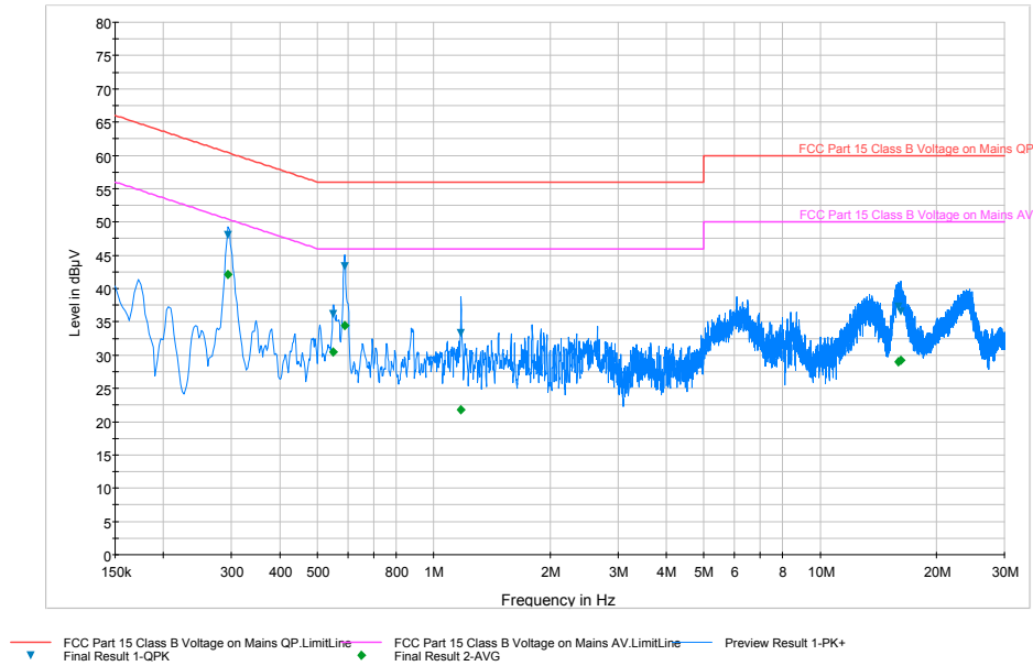
Plot 6-6. Line-Conducted Test Plot (N)
