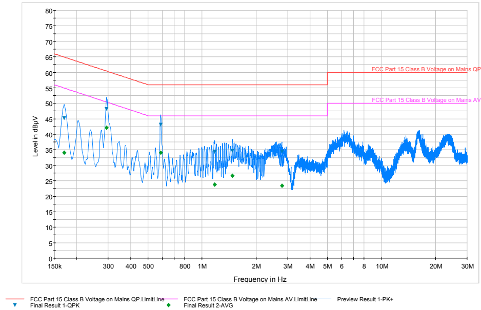
Plot 6-5. Line-Conducted Test Plot (L1)
