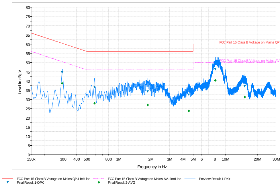
Plot 6-6. Line Conducted Plot with Bluetooth LE (L1)
