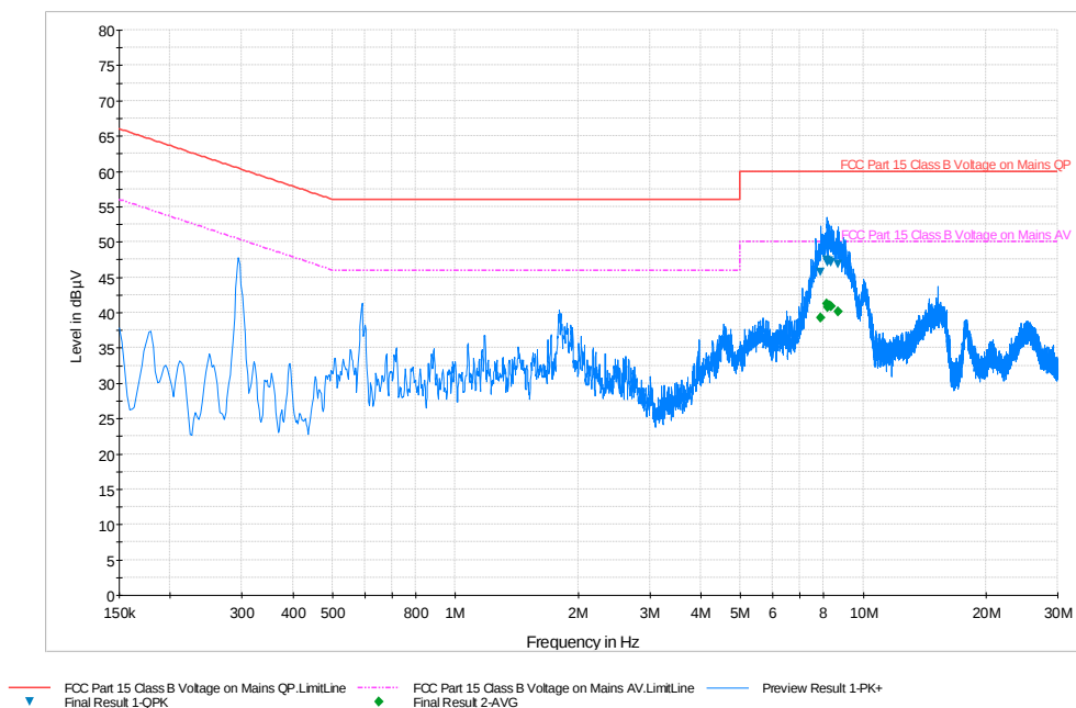
Plot 6-7. Line Conducted Plot with Bluetooth LE (N)
