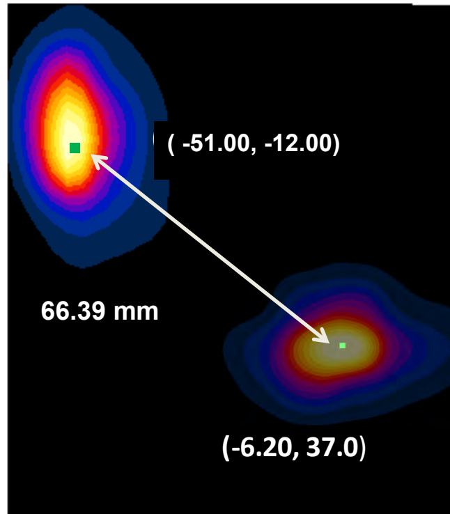
Figure 10-7 Peak SAR Location Plot of UMTS 1900 MHz and 2.4 GHz WLAN MIMO
