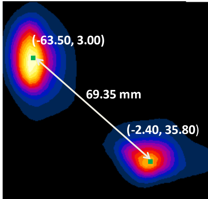
Figure 10-2 Peak SAR Location Plot of UMTS 850 MHz and 2.4 GHz WLAN Antenna 1
