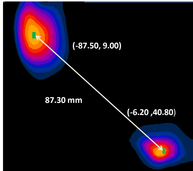
Figure 10-12 Peak SAR Location Plot of GPRS 1900 MHz and 2.4 GHz WLAN Antenna 1
