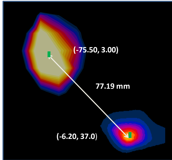
Figure 10-6 Peak SAR Location Plot of GPRS 850 MHz and 2.4 GHz WLAN MIMO
