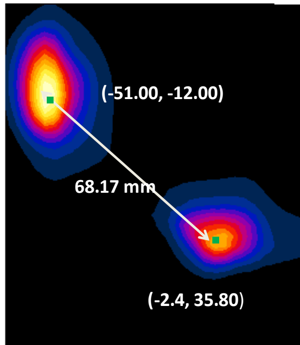
Figure 10-4 Peak SAR Location Plot of UMTS 1900 MHz and 2.4 GHz WLAN Antenna 1
