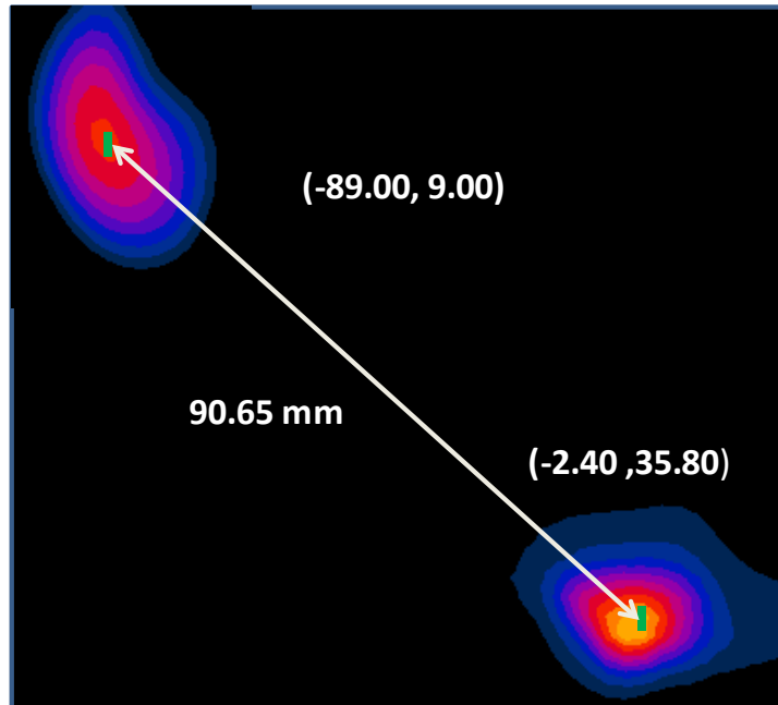
Figure 10-13 Peak SAR Location Plot of UMTS 1900 MHz and 2.4 GHz WLAN Antenna 1
