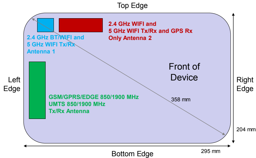
Figure 1-1 DUT Antenna Locations
