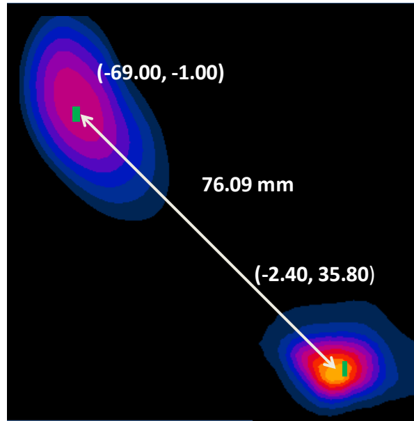
Figure 10-11 Peak SAR Location Plot of GPRS 850 MHz and 2.4 GHz WLAN Antenna 1
