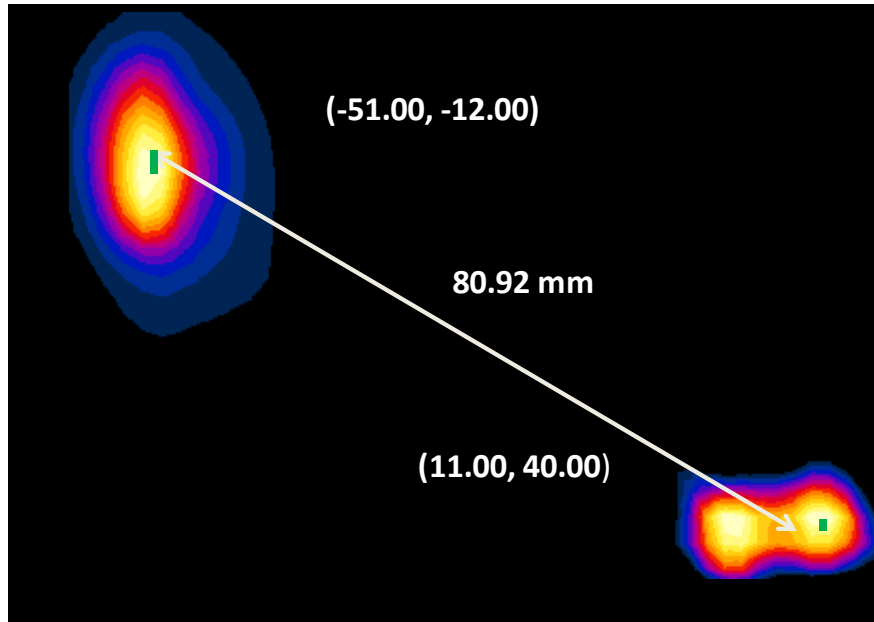
Figure 10-10 Peak SAR Location Plot of UMTS 1900 MHz and 5 GHz WLAN MIMO
