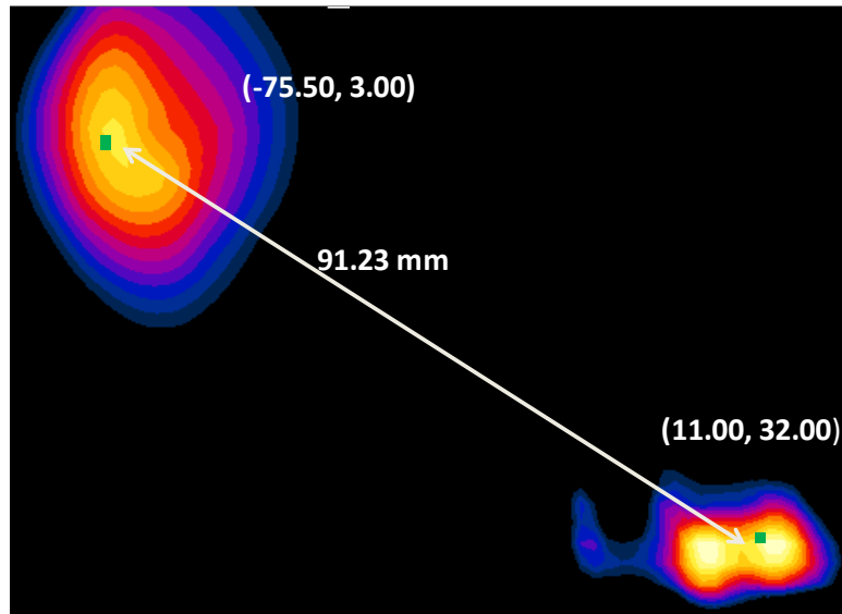
Figure 10-8 Peak SAR Location Plot of GPRS 850 MHz and 5 GHz WLAN Antenna 2
