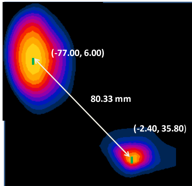
Figure 10-3 Peak SAR Location Plot of GPRS 1900 MHz and 2.4 GHz WLAN Antenna 1
