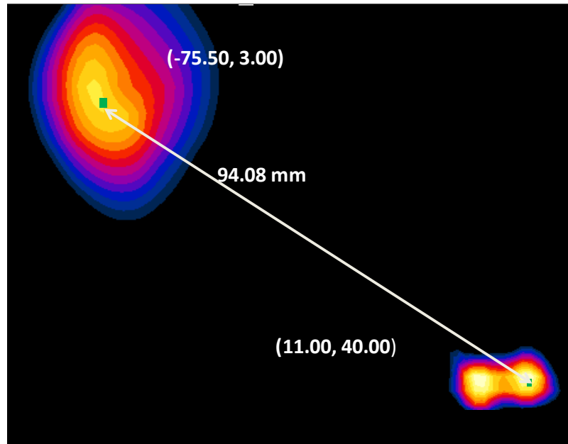
Figure 10-9 Peak SAR Location Plot of GPRS 850 MHz and 5 GHz WLAN MIMO
