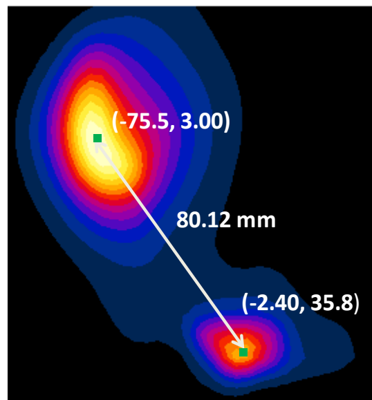
Figure 10-1 Peak SAR Location Plot of GPRS 850 MHz and 2.4 GHz WLAN Antenna 1
