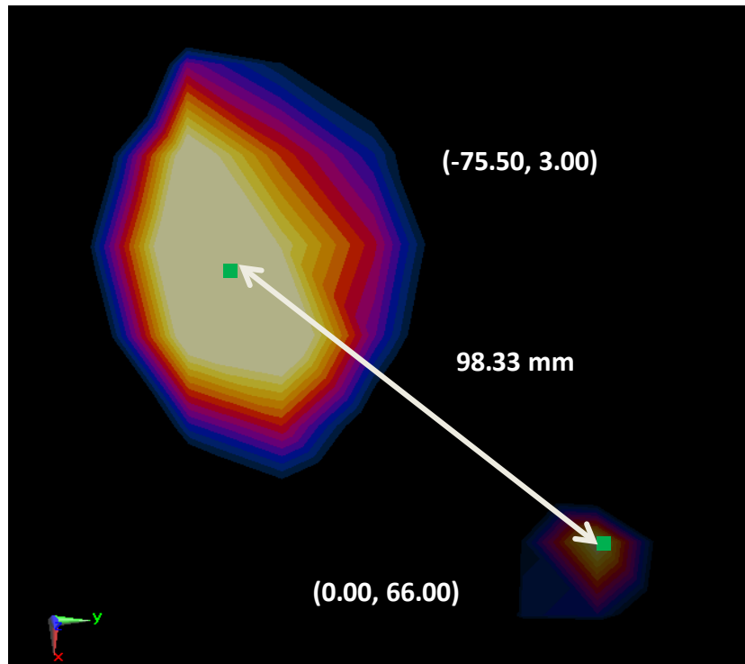
Figure 10-5 Peak SAR Location Plot of GPRS 850 MHz and 2.4 GHz WLAN Antenna 2
