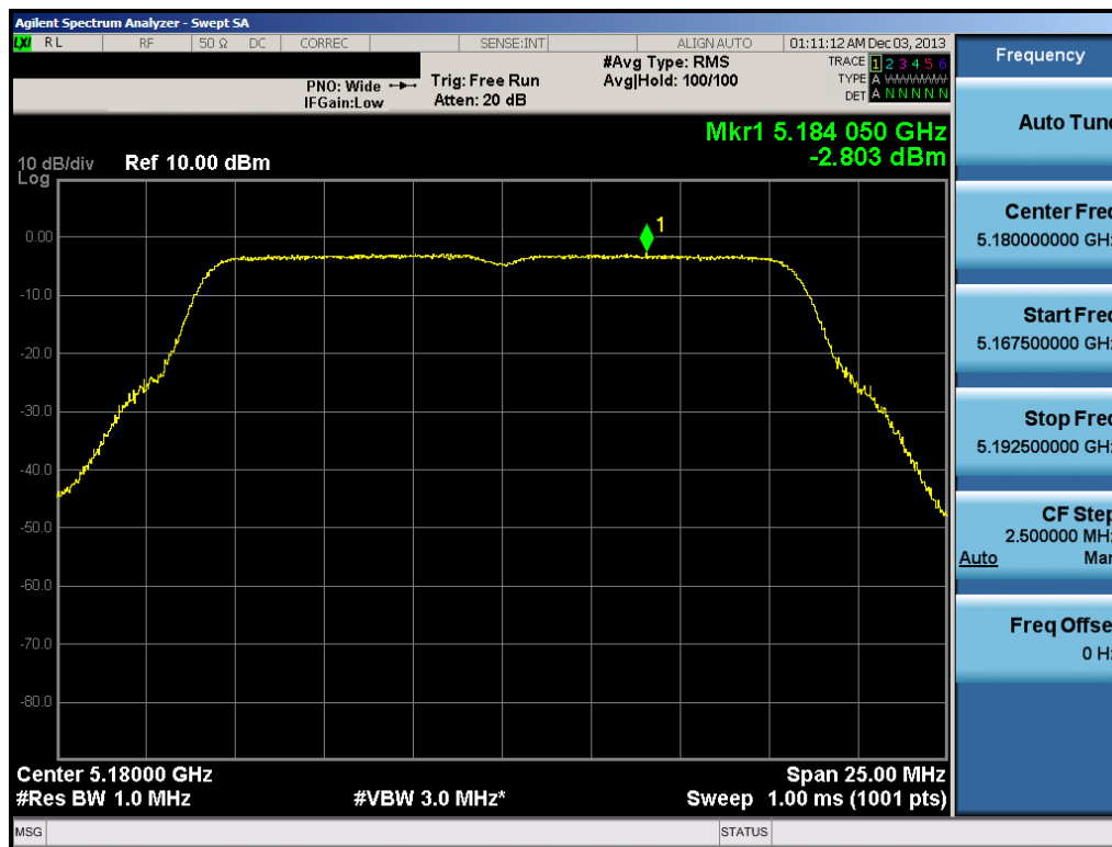
Plot 6-93. Peak Power Spectral Density Plot (802.11a (UNII Band 1) – Ch. 36)
