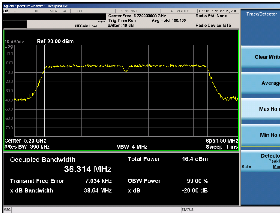
Plot 6-31. 20dB Bandwidth Plot (40MHz BW 802.11n (UNII Band 1) – Ch. 46)
