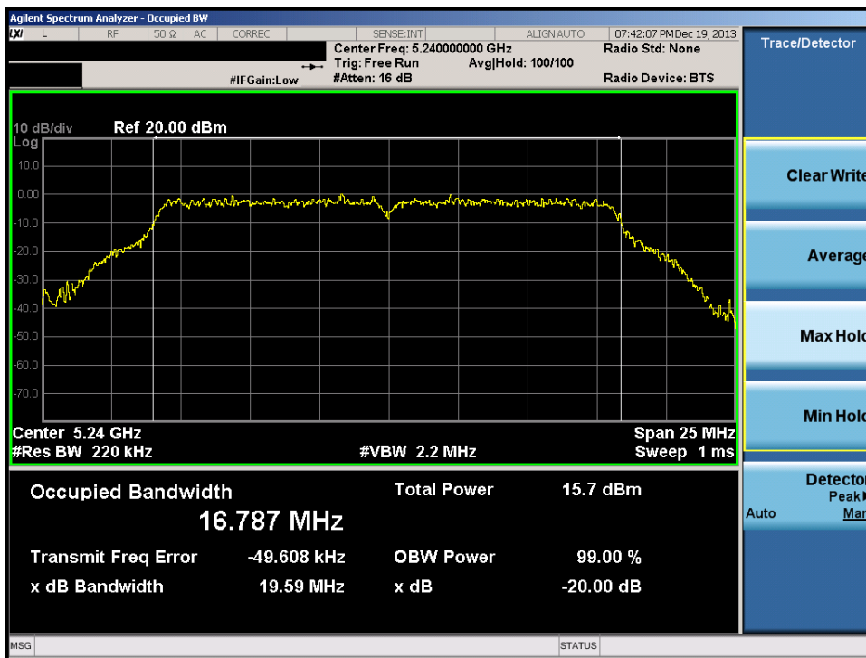
Plot 6-62. 20dB Bandwidth Plot (20MHz BW 802.11a (UNII Band 1) – Ch. 48)
