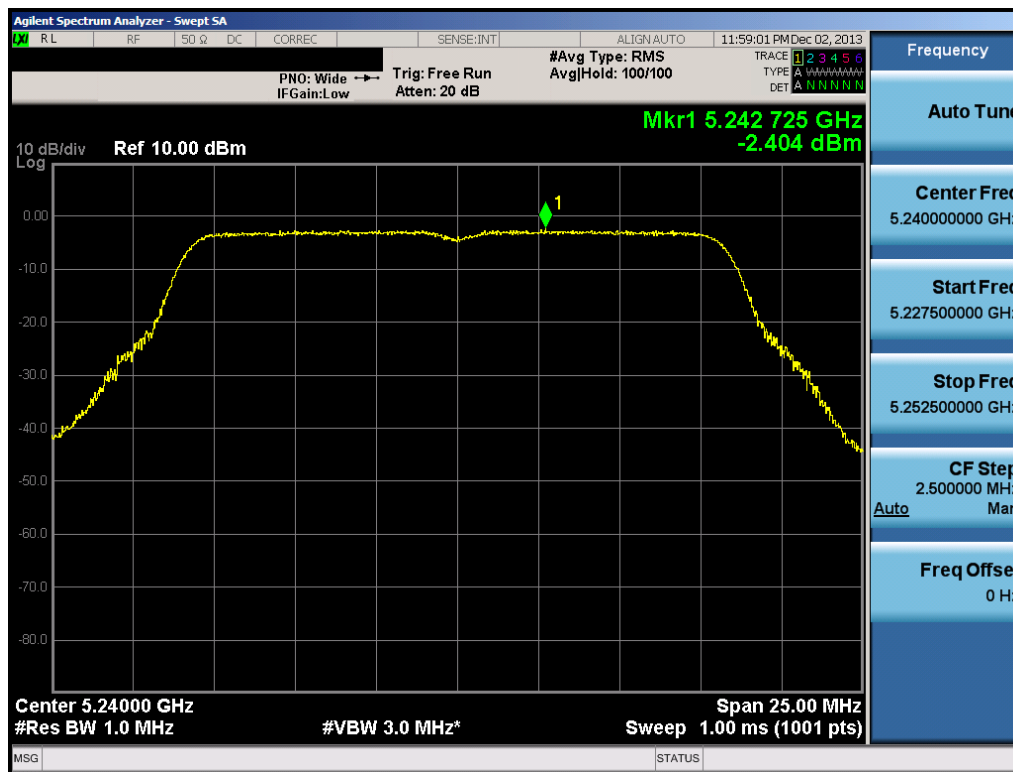
Plot 6-67. Peak Power Spectral Density Plot (802.11a (UNII Band 1) – Ch. 48)
