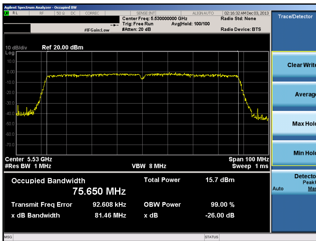
Plot 6-61. 26dB Bandwidth Plot (80MHz BW 802.11ac (UNII Band 2C) – Ch. 106)
