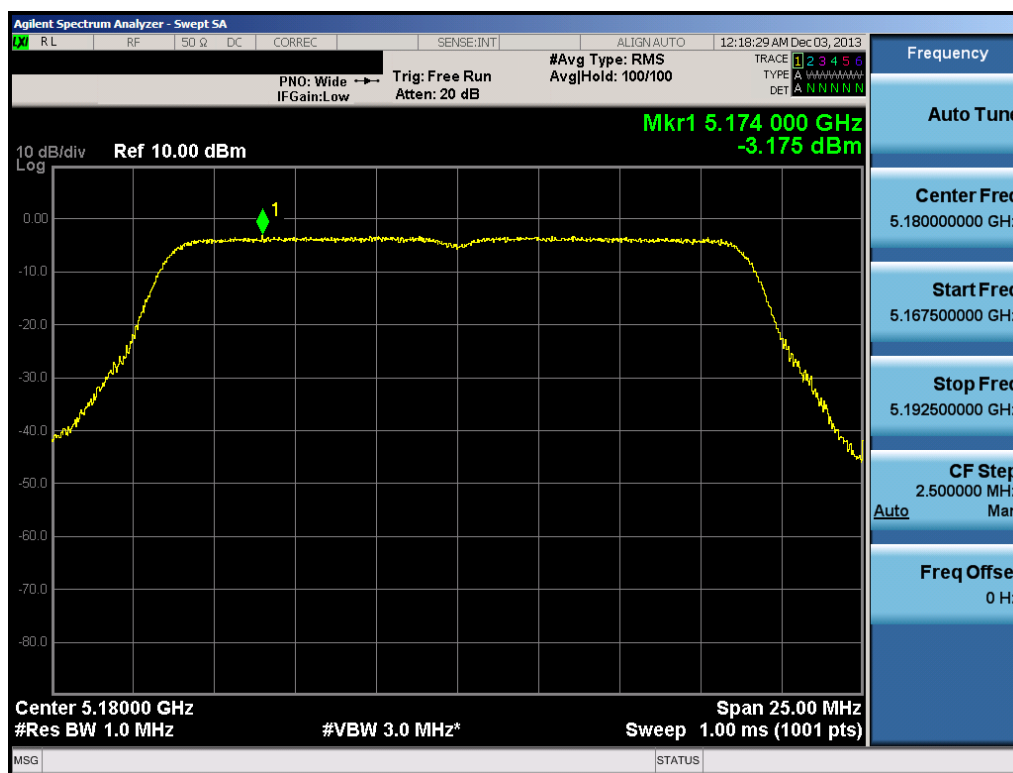
Plot 6-68. Peak Power Spectral Density Plot (20MHz BW 802.11n (UNII Band 1) – Ch. 36)
