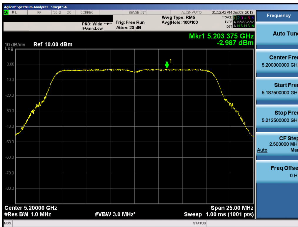
Plot 6-94. Peak Power Spectral Density Plot (802.11a (UNII Band 1) – Ch. 40)
