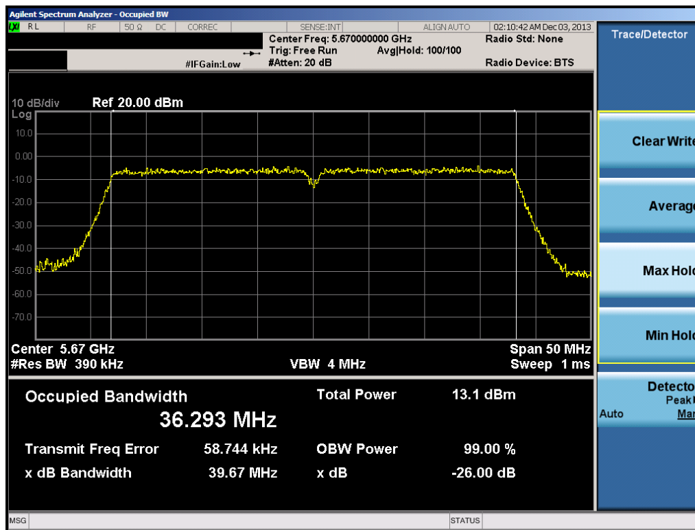
Plot 6-60. 26dB Bandwidth Plot (40MHz BW 802.11n (UNII Band 2C) – Ch. 134)
