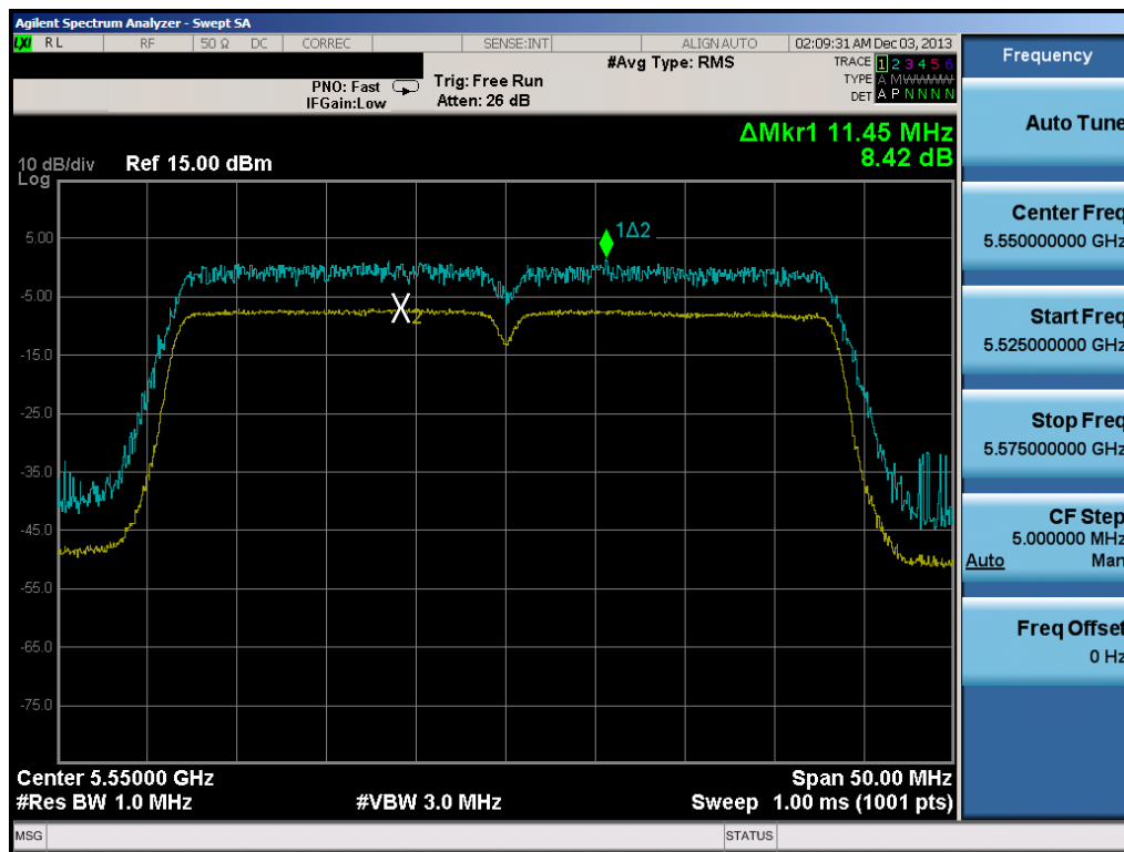
Plot 6-127. Peak Excursion Ratio Plot (40MHz BW 802.11n)
