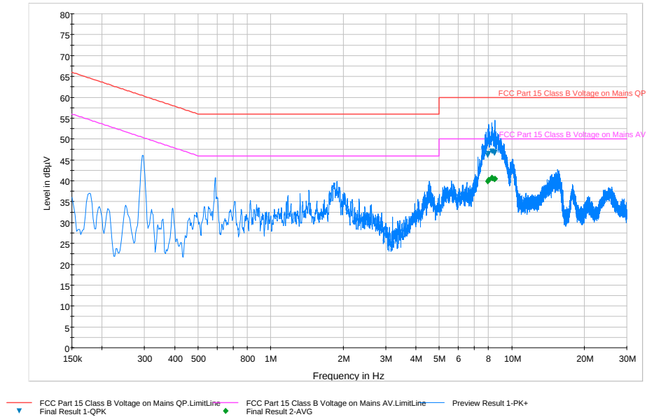
Plot 6-190. Line Conducted Plot with 802.11a UNII Band 1 (N)
