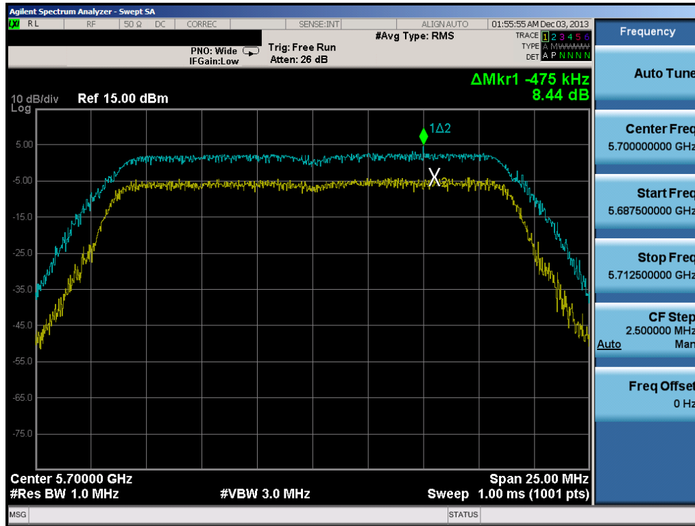
Plot 6-126. Peak Excursion Ratio Plot (20MHz BW 802.11n)
