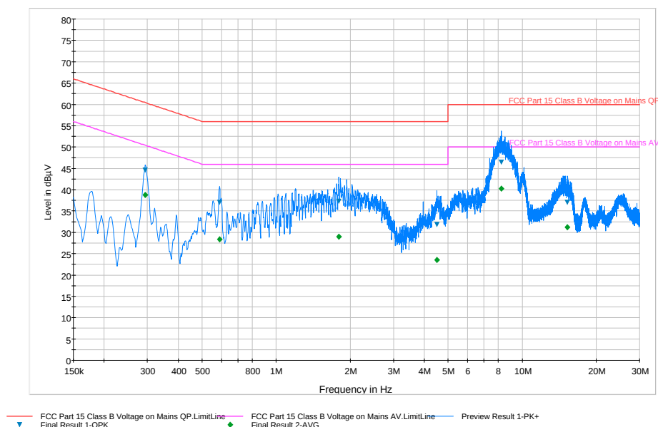
Plot 6-189. Line Conducted Plot with 802.11a UNII Band 1 (L1)
