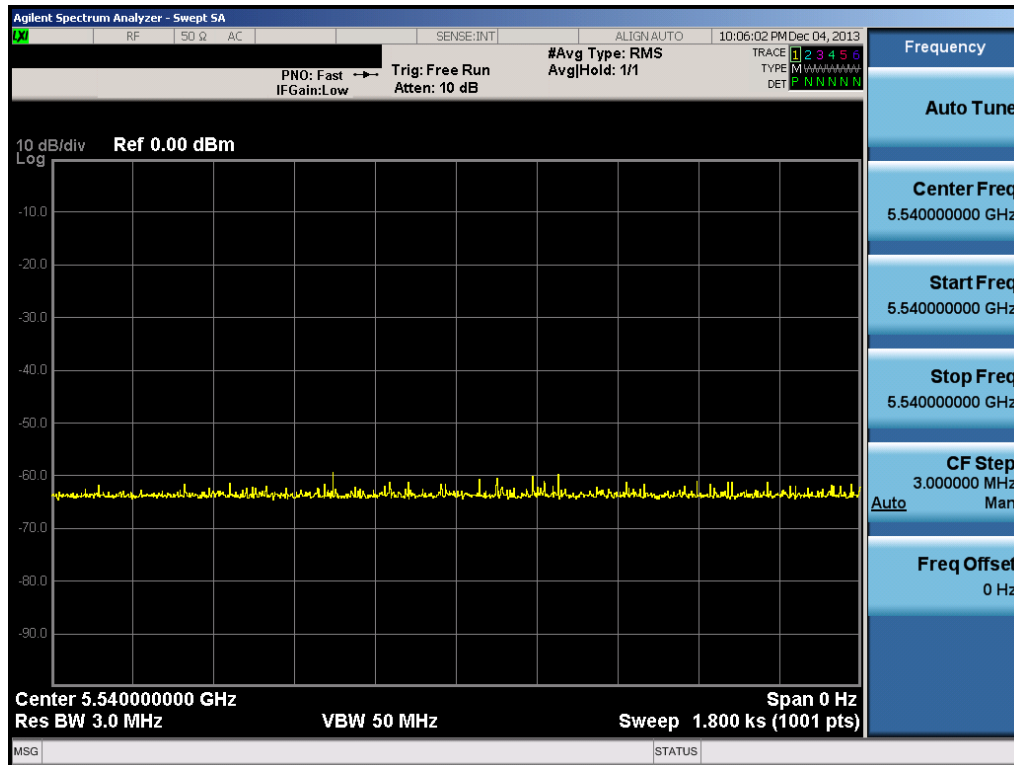
Figure 6-4. Non-occupancy Period - Monitoring live spectrum - Elapse time 30 minutes
