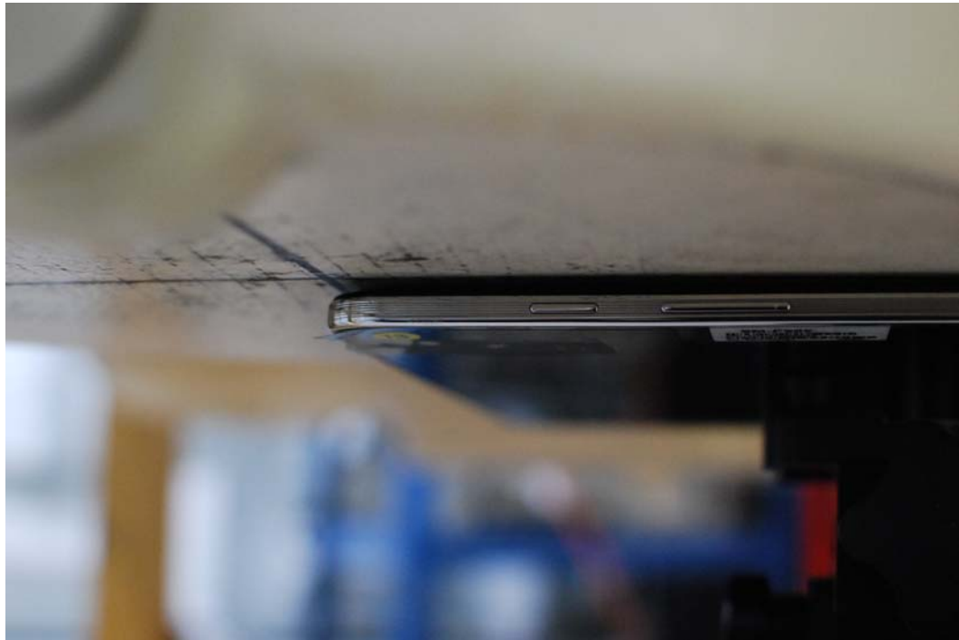
SAR Test Setup Photo 1: Back at 0 mm
