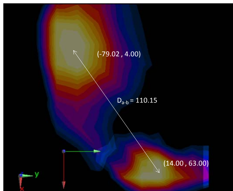
Figure 11-2 Peak SAR Locations of 2.4 GHz WLAN and LTE Band 4
