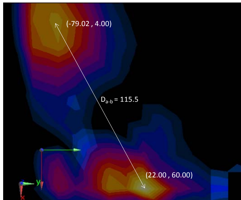
Figure 11-6 Peak SAR Location of 5 GHz WLAN and LTE Band 4
