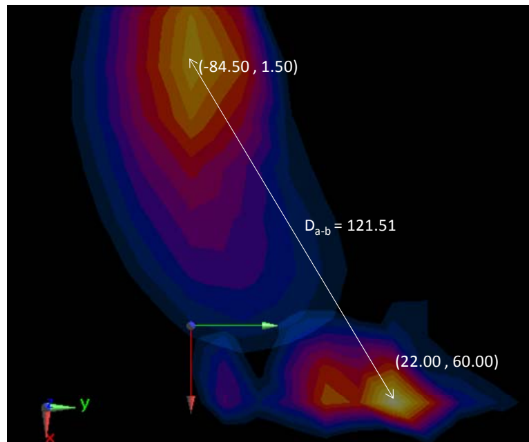
Figure 11-8 Peak SAR Location of 5 GHz WLAN and LTE Band 4
