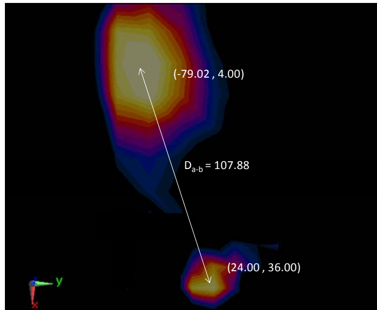
Figure 11-10 Peak SAR Location of 5 GHz WLAN and LTE Band 4
