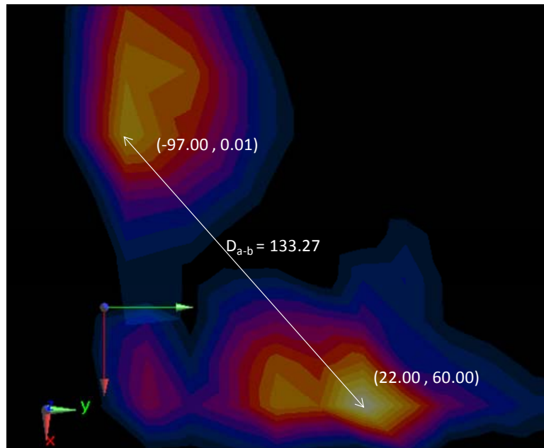
Figure 11-3 Peak SAR Location of 5 GHz WLAN and UMTS 1900 MHz
