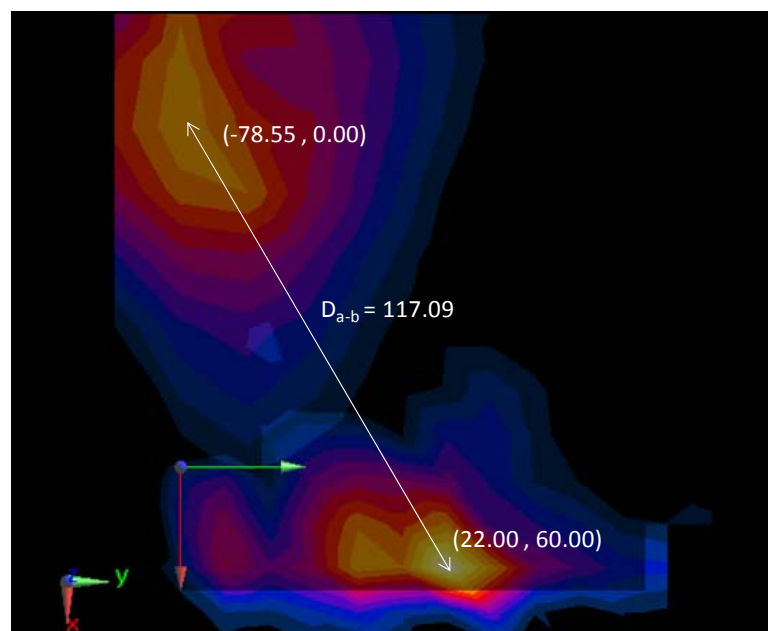
Figure 11-5 Peak SAR Location of 5 GHz WLAN and LTE Band 5
