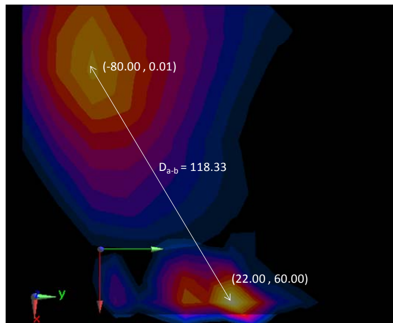
Figure 11-4 Peak SAR Location of 5 GHz WLAN and LTE Band 17
