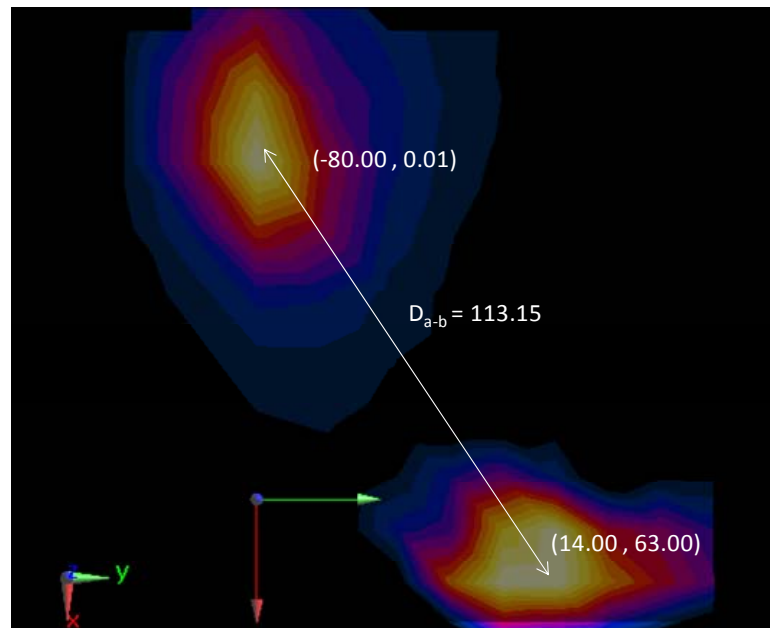
Figure 11-1 Peak SAR Locations of 2.4 GHz WLAN and LTE Band 17
