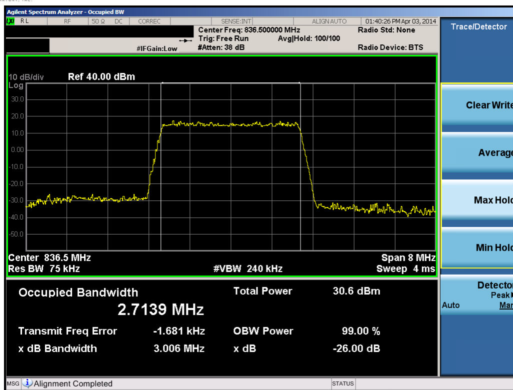
Plot 8-7. Occupied Bandwidth Plot (3.0MHz 16-QAM – RB Size 15)
