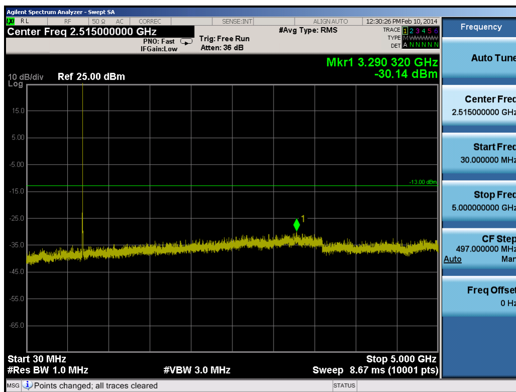
Plot 7-6. Conducted Spurious Plot (5.0MHz QPSK – RB Size 1, RB Offset 0 – Mid Channel)
