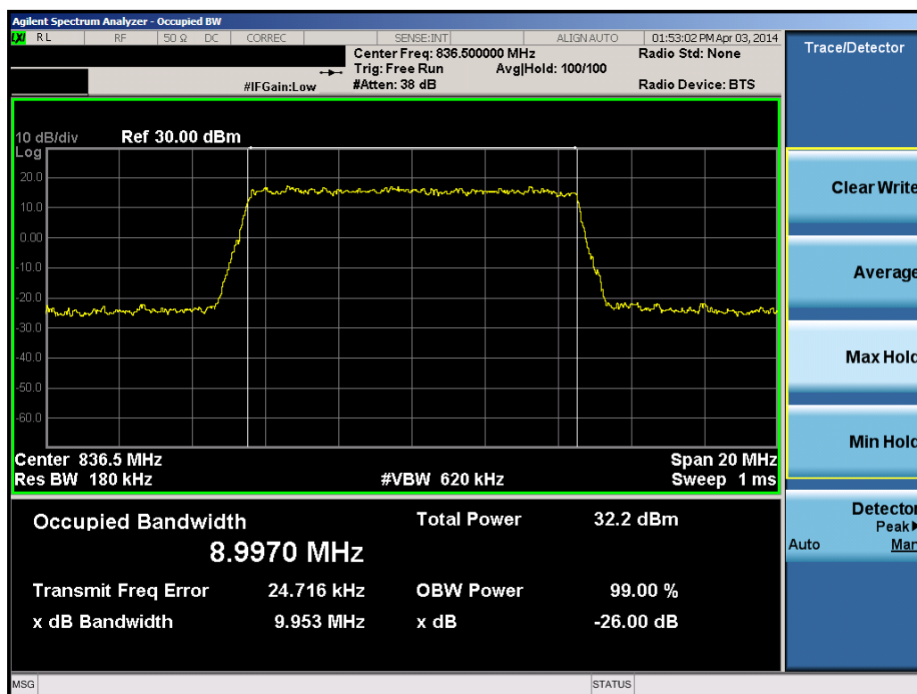
Plot 8-20. Occupied Bandwidth Plot (10.0MHz QPSK – RB Size 50)
