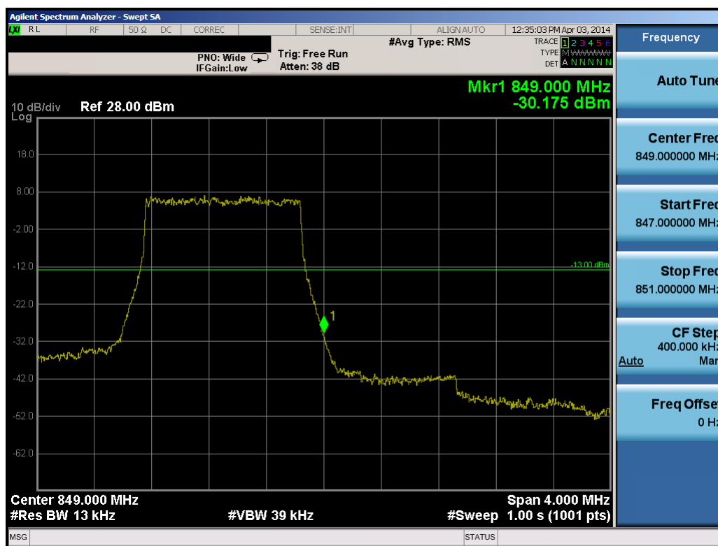
Plot 8-4. Upper Band Edge Plot (1.4MHz QPSK – RB Size 6)
