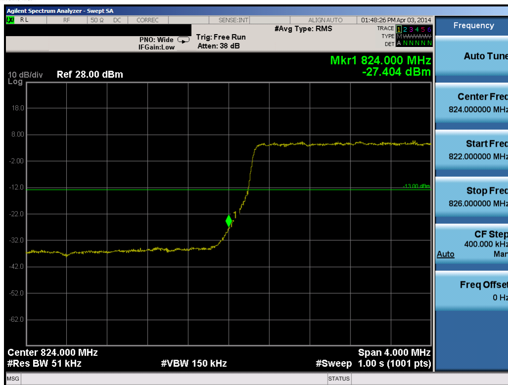
Plot 8-9. Lower Band Edge Plot (5.0MHz QPSK – RB Size 25)
