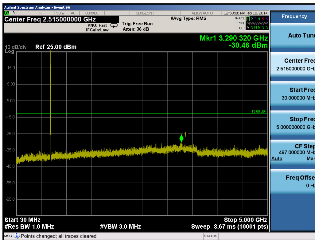
Plot 7-18. Conducted Spurious Plot (10.0MHz QPSK – RB Size 1, RB Offset 0 – High Channel)
