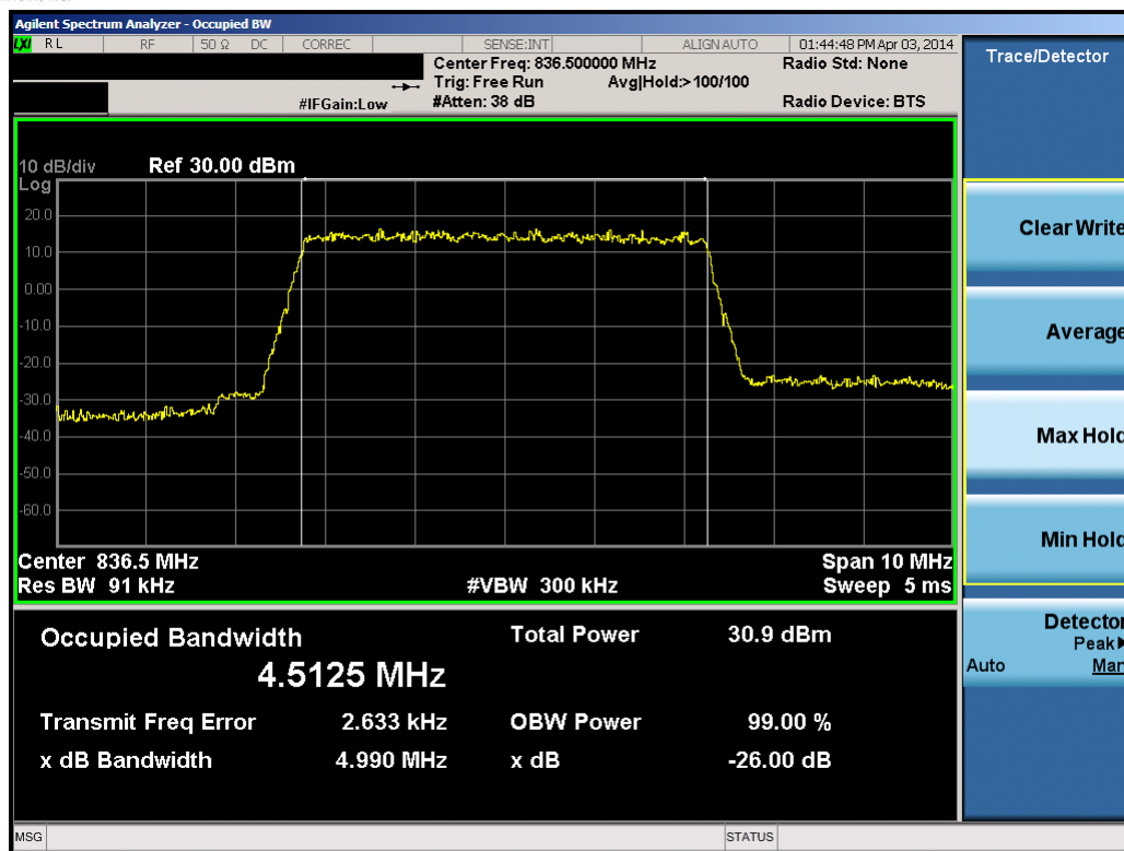
Plot 8-11. Occupied Bandwidth Plot (5.0MHz 16-QAM – RB Size 25)
