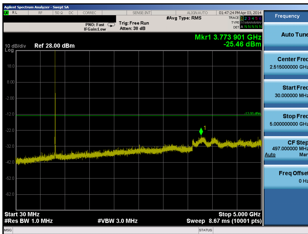
Plot 8-12. Conducted Spurious Plot (5.0MHz QPSK – RB Size 1, RB Offset 0 – Low Channel)
