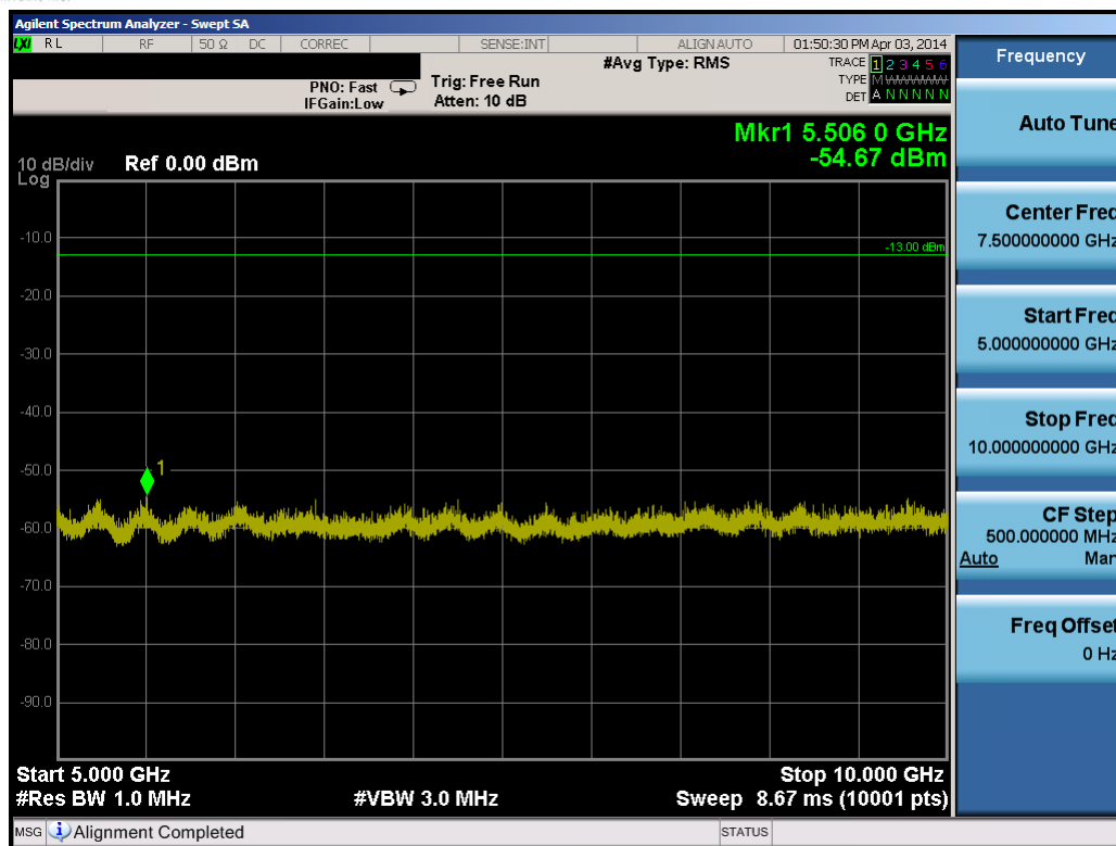
Plot 8-17. Conducted Spurious Plot (5.0MHz QPSK – RB Size 1, RB Offset 0 – High Channel)
