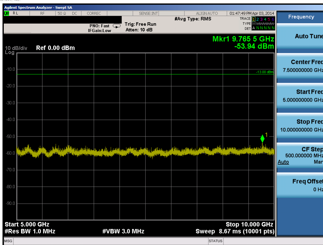
Plot 8-13. Conducted Spurious Plot (5.0MHz QPSK – RB Size 1, RB Offset 0 – Low Channel)
