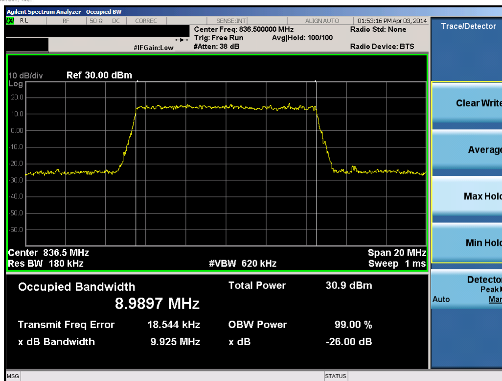
Plot 8-21. Occupied Bandwidth Plot (10.0MHz 16-QAM – RB Size 50)
