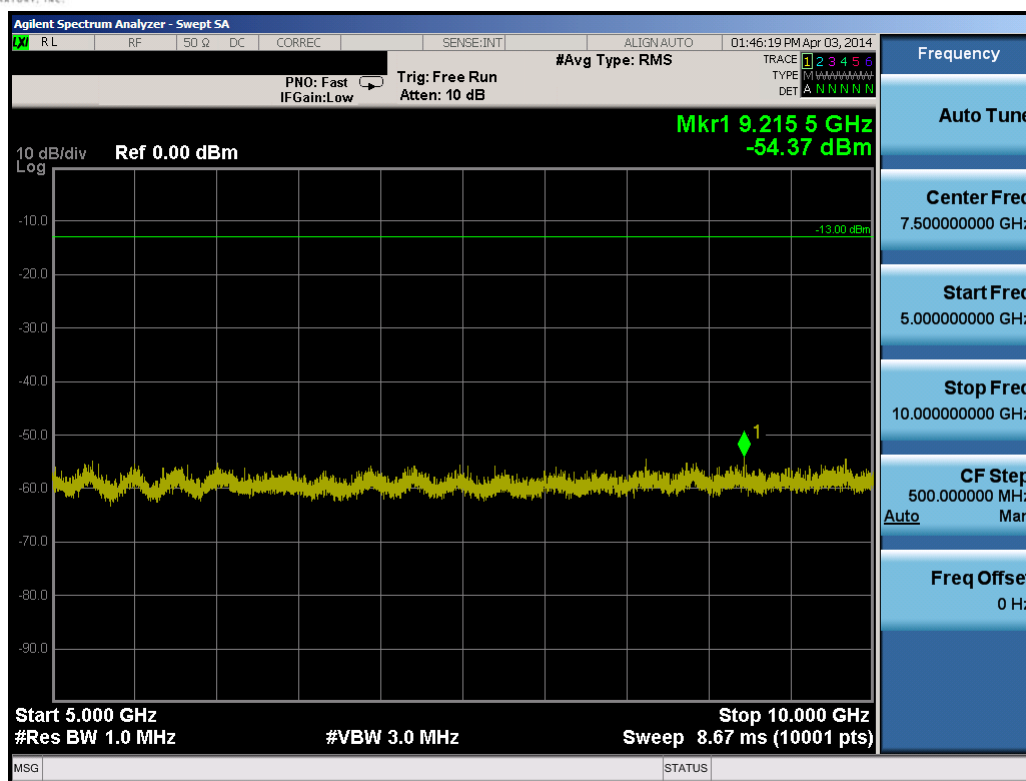
Plot 8-15. Conducted Spurious Plot (5.0MHz QPSK – RB Size 1, RB Offset 0 – Mid Channel)
