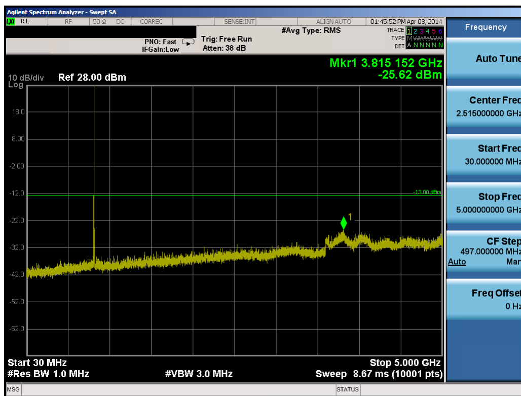
Plot 8-14. Conducted Spurious Plot (5.0MHz QPSK – RB Size 1, RB Offset 0 – Mid Channel)
