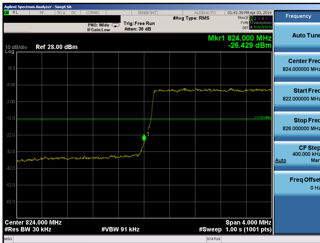
Plot 8-5. Lower Band Edge Plot (3.0MHz QPSK – RB Size 15)
