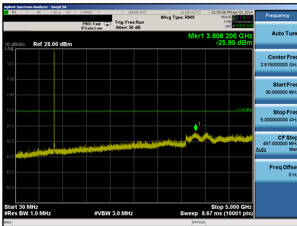
Plot 8-16. Conducted Spurious Plot (5.0MHz QPSK – RB Size 1, RB Offset 0 – High Channel)
