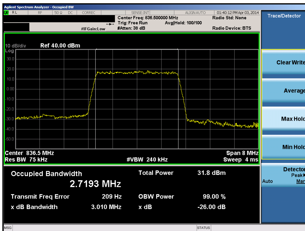
Plot 8-6. Occupied Bandwidth Plot (3.0MHz QPSK – RB Size 15)
