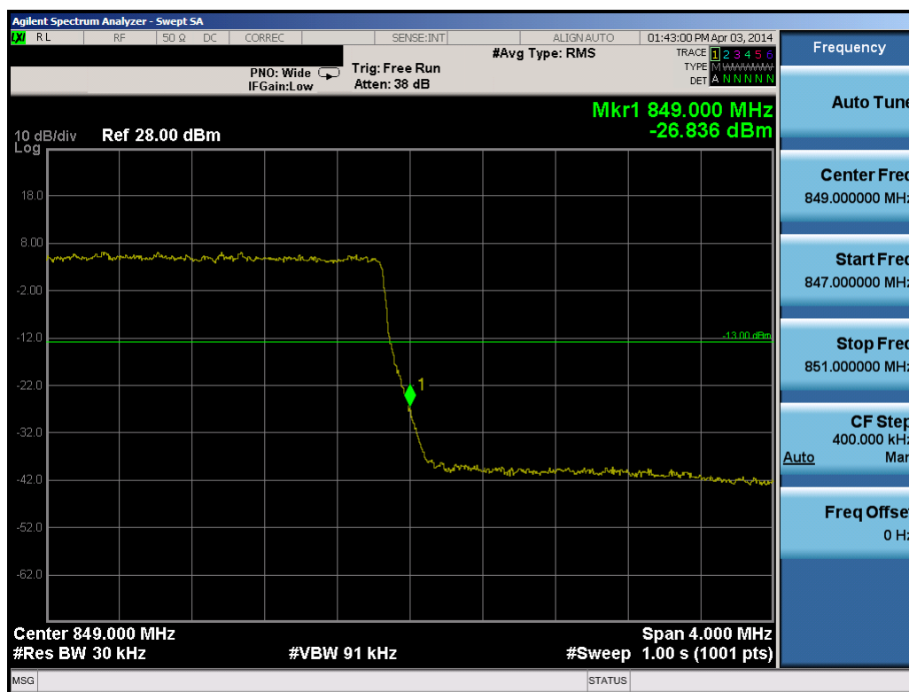
Plot 8-8. Upper Band Edge Plot (3.0MHz QPSK – RB Size 15)
