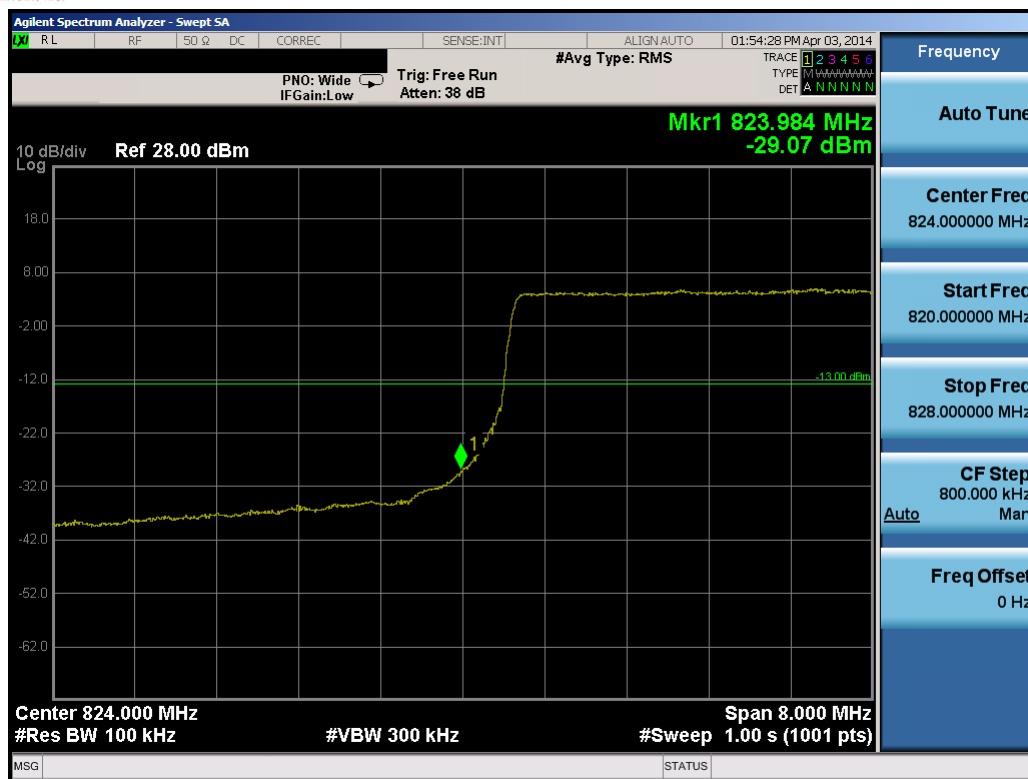
Plot 8-19. Lower Band Edge Plot (10.0MHz QPSK – RB Size 50)
