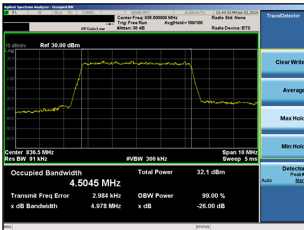
Plot 8-10. Occupied Bandwidth Plot (5.0MHz QPSK – RB Size 25)
