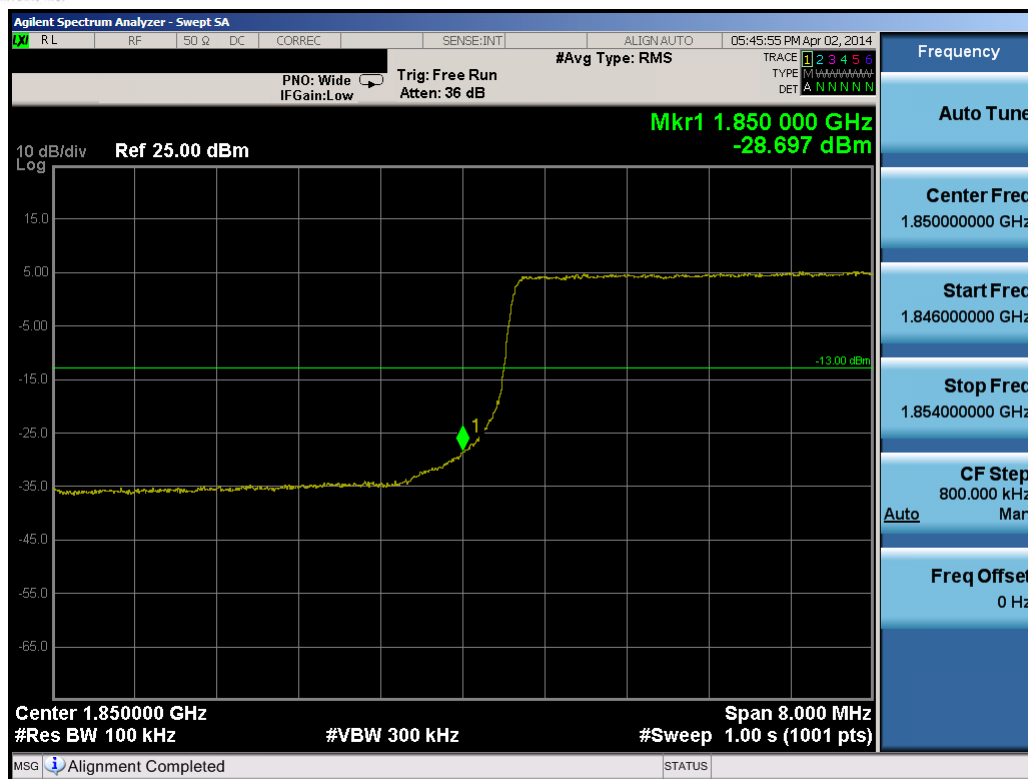
Plot 10-25. Lower Band Edge Plot (10.0MHz QPSK – RB Size 50)
