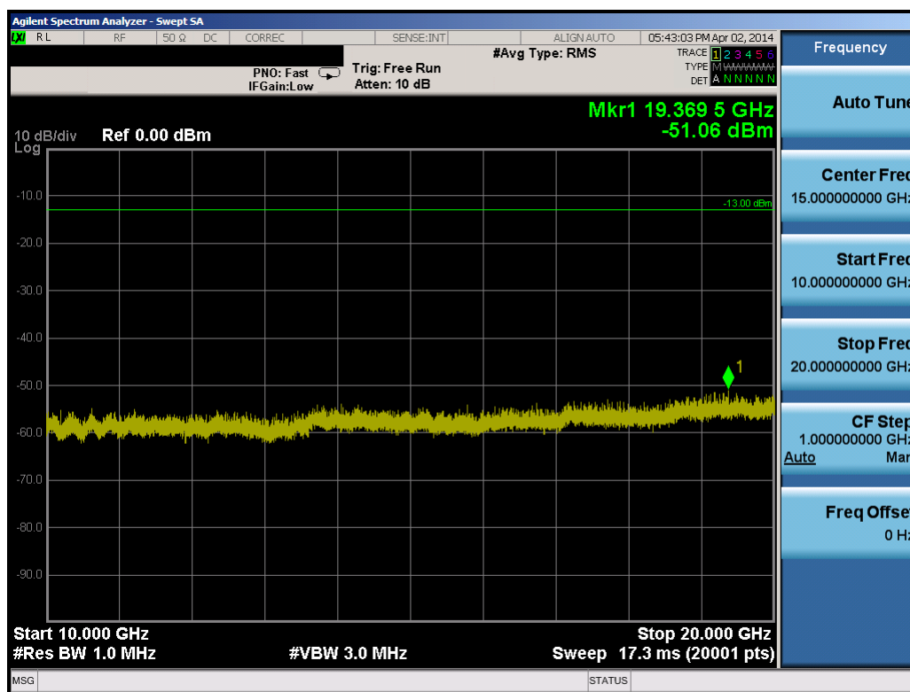
Plot 10-32. Conducted Spurious Plot (10.0MHz QPSK – RB Size 1, RB Offset 0 – Mid Channel)
