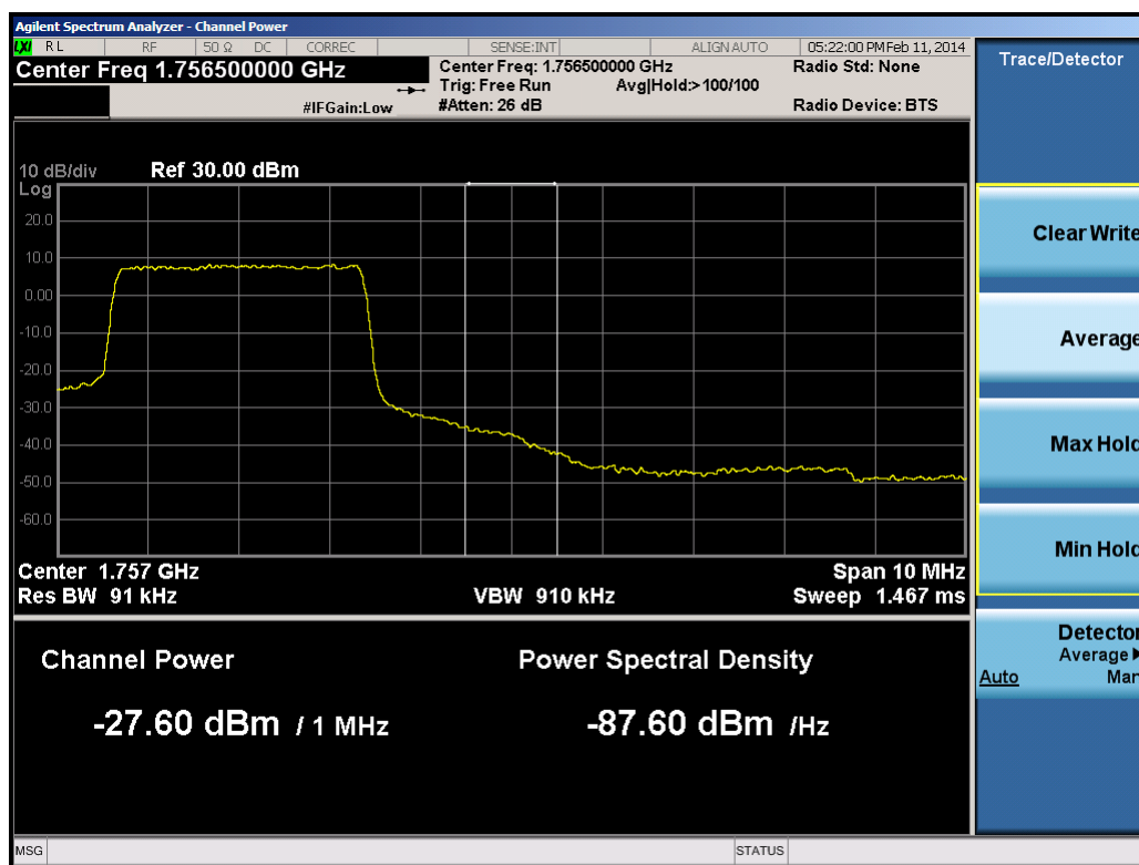
Plot 9-26. Upper Extended Band Edge Plot (3.0MHz QPSK – RB Size 15)
