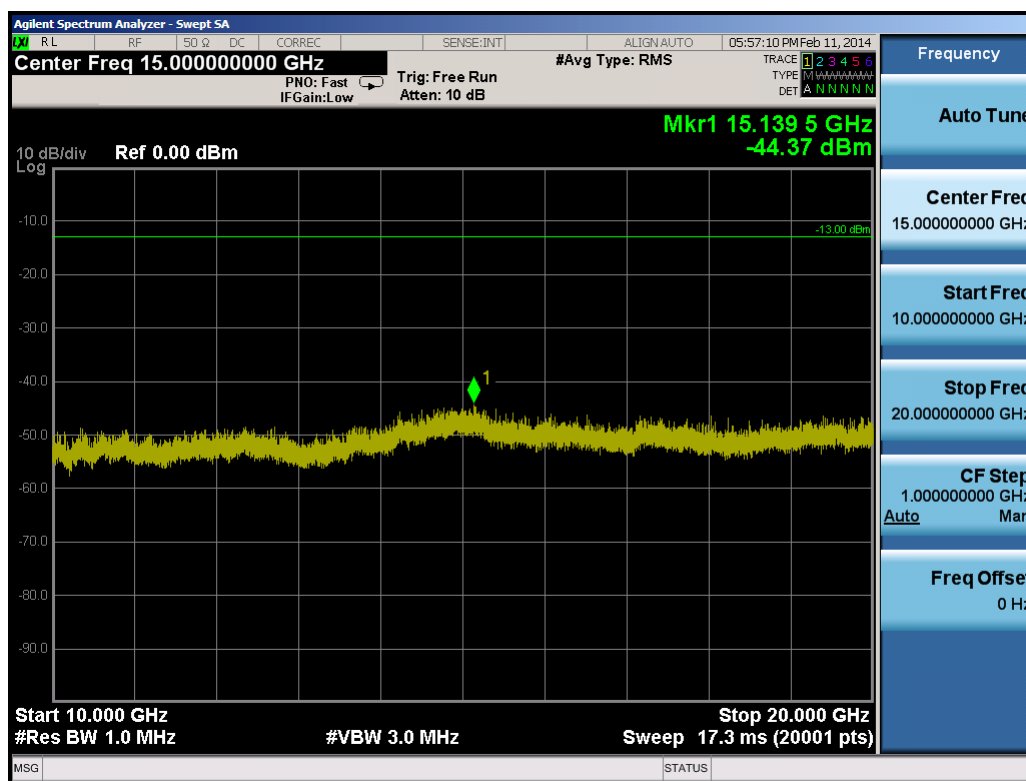
Plot 9-80. Conducted Spurious Plot (20.0MHz QPSK – RB Size 1, RB Offset 0 – High Channel)
