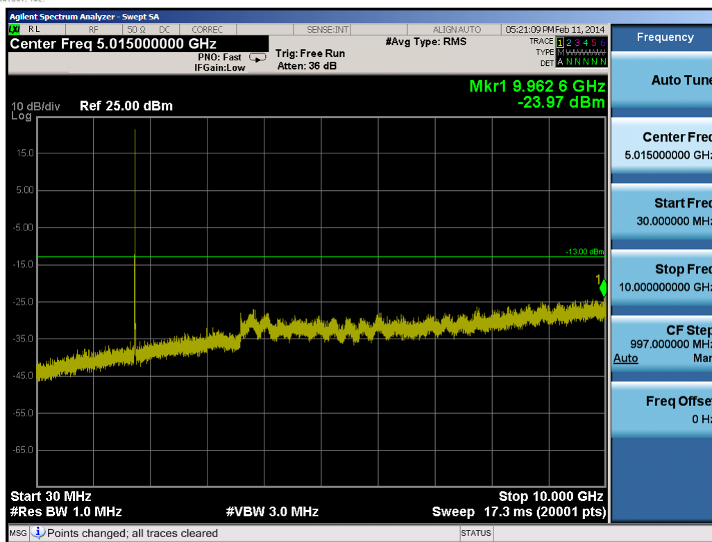
Plot 9-23. Conducted Spurious Plot (3.0MHz QPSK – RB Size 1, RB Offset 0 – High Channel)
