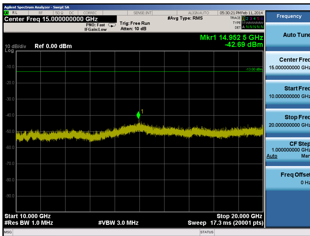
Plot 9-48. Conducted Spurious Plot (10.0MHz QPSK – RB Size 1, RB Offset 0 – Low Channel)
