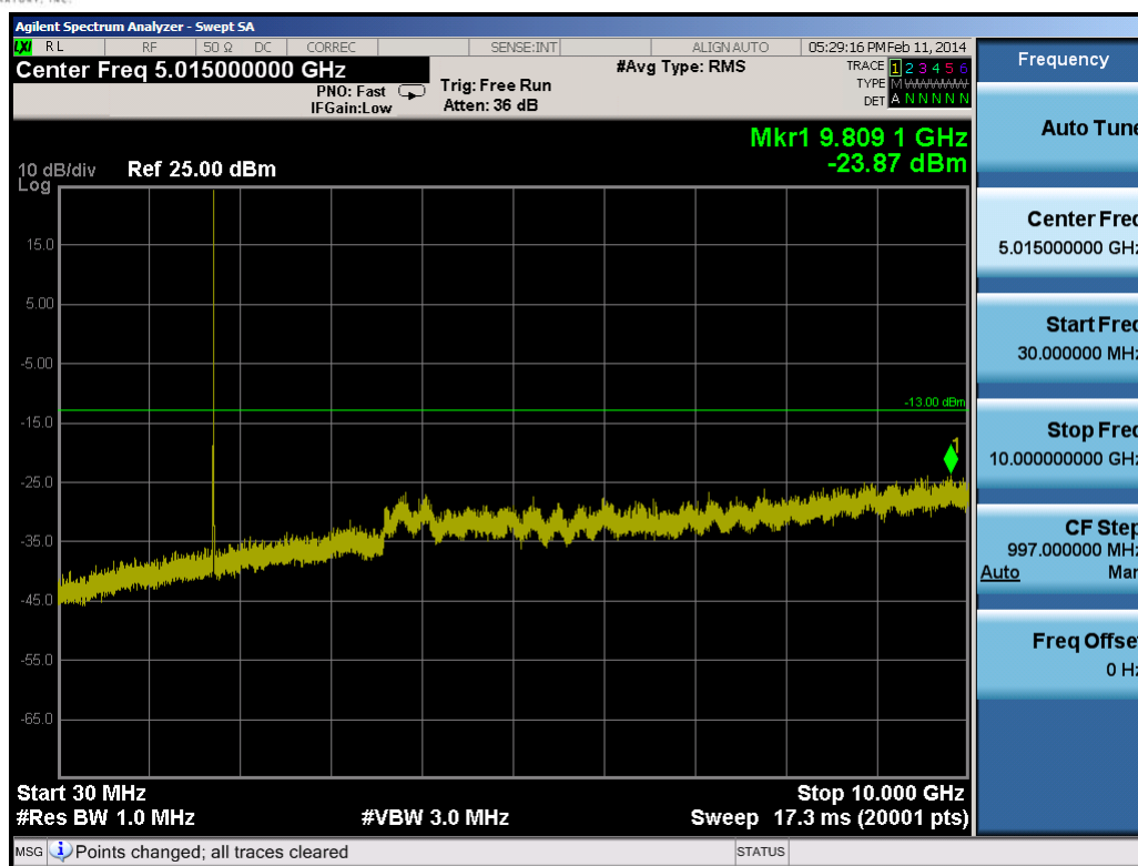
Plot 9-49. Conducted Spurious Plot (10.0MHz QPSK – RB Size 1, RB Offset 0 – Mid Channel)
