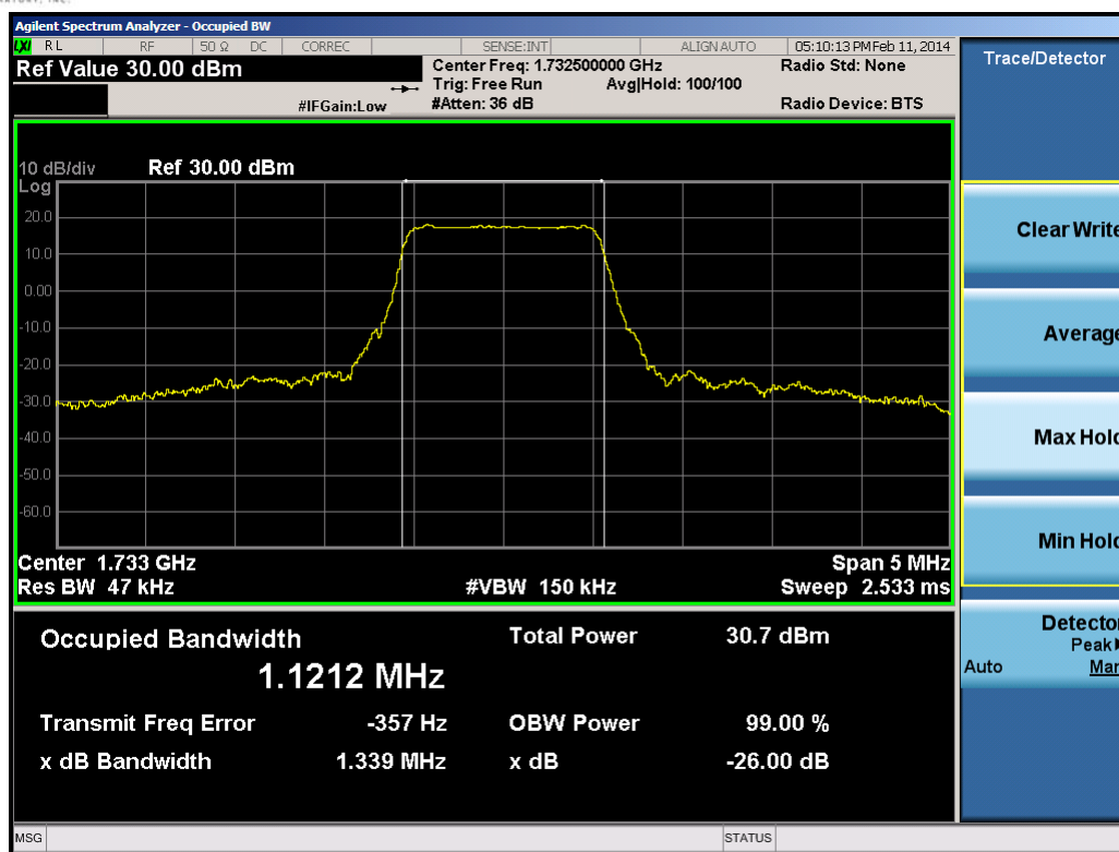
Plot 9-3. Occupied Bandwidth Plot (1.4MHz QPSK – RB Size 6)
