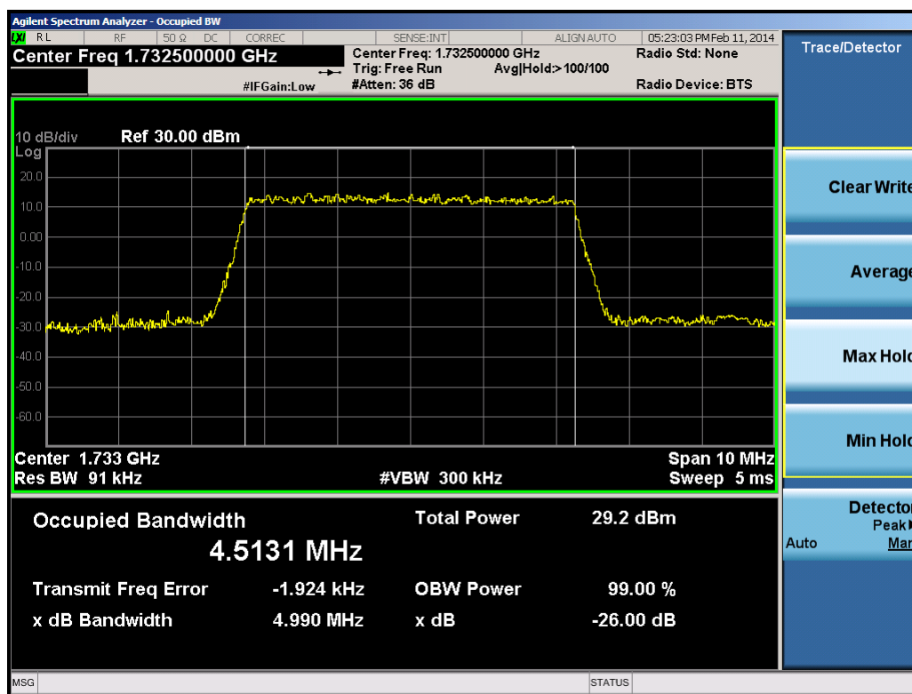
Plot 9-32. Occupied Bandwidth Plot (5.0MHz 16-QAM – RB Size 25)
