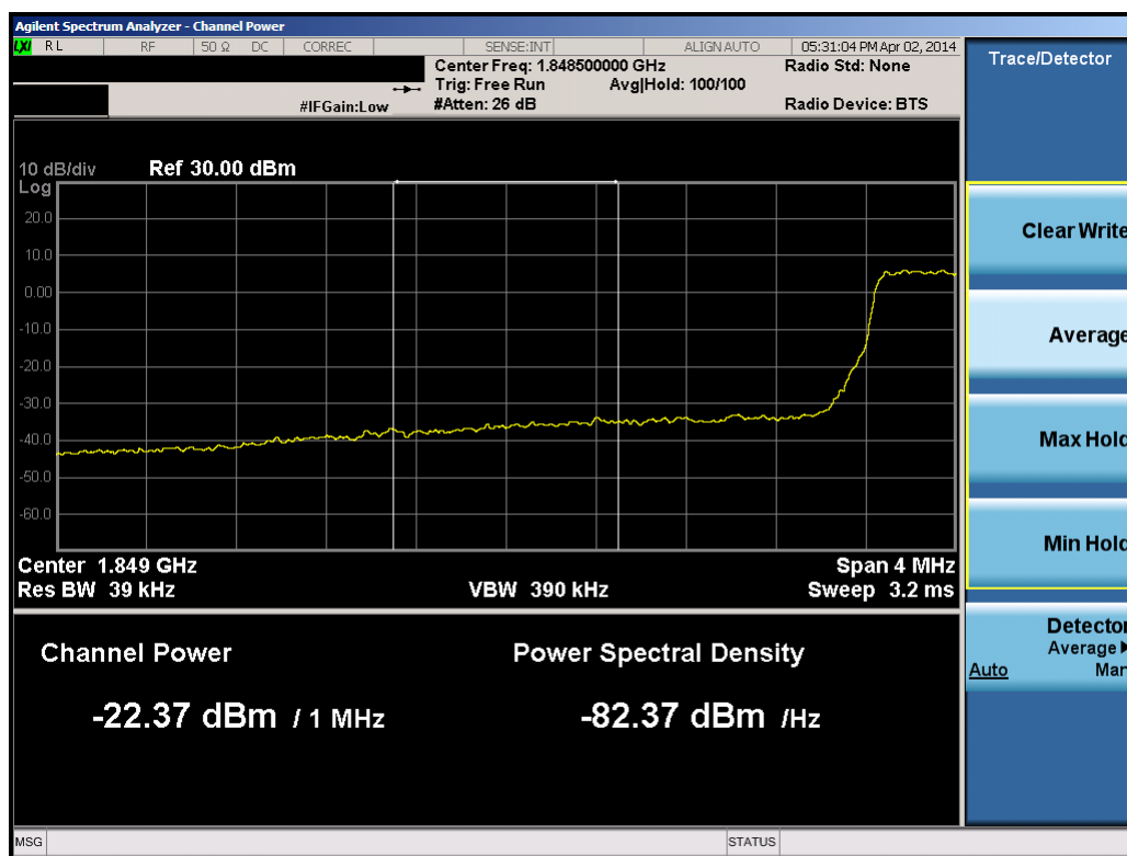
Plot 10-10. Lower Extended Band Edge Plot (3.0MHz QPSK – RB Size 15)
