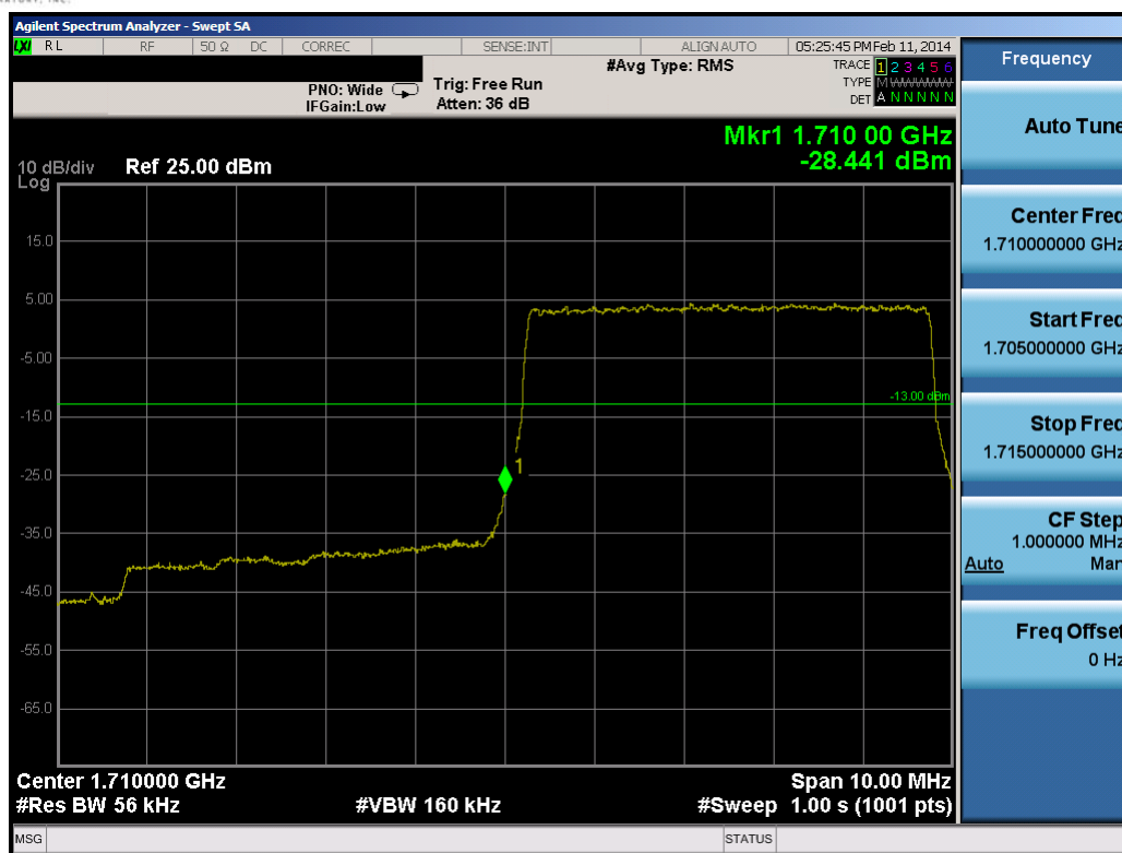
Plot 9-29. Lower Band Edge Plot (5.0MHz QPSK – RB Size 25)
