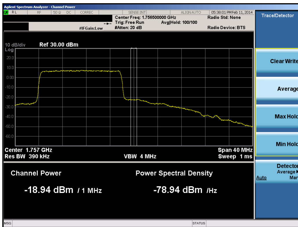
Plot 9-68. Upper Extended Band Edge Plot (15.0MHz QPSK – RB Size 75)
