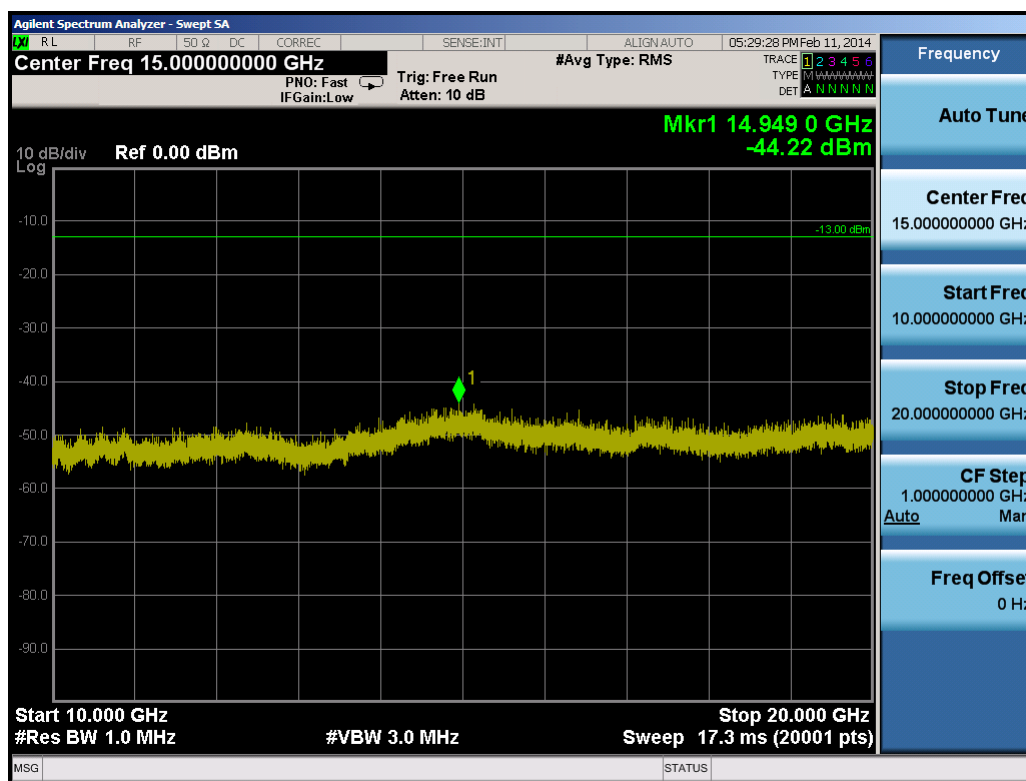
Plot 9-50. Conducted Spurious Plot (10.0MHz QPSK – RB Size 1, RB Offset 0 – Mid Channel)
