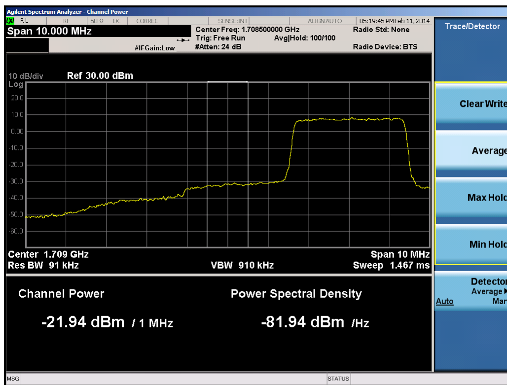
Plot 9-16. Lower Extended Band Edge Plot (3.0MHz QPSK – RB Size 15)
