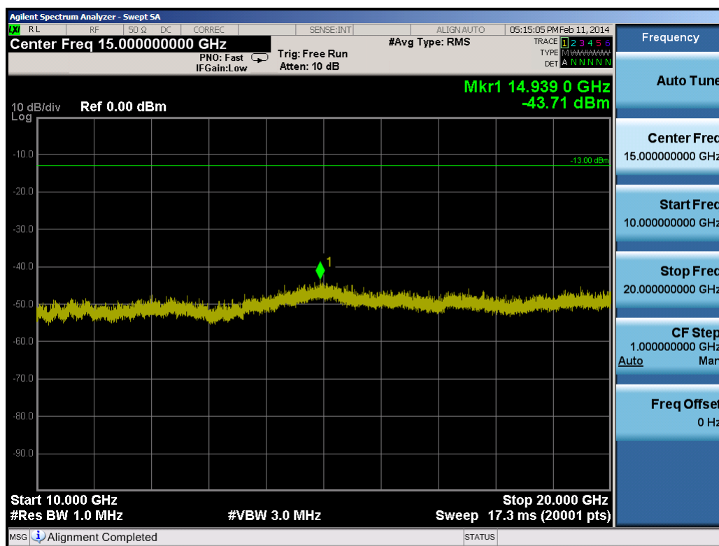
Plot 9-10. Conducted Spurious Plot (1.4MHz QPSK – RB Size 1, RB Offset 0 – High Channel)
