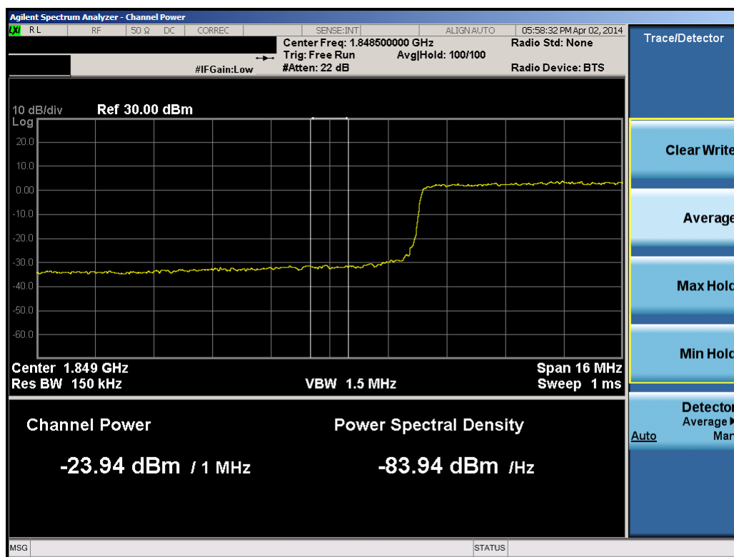
Plot 10-48. Lower Extended Band Edge Plot (20.0MHz QPSK – RB Size 100)
