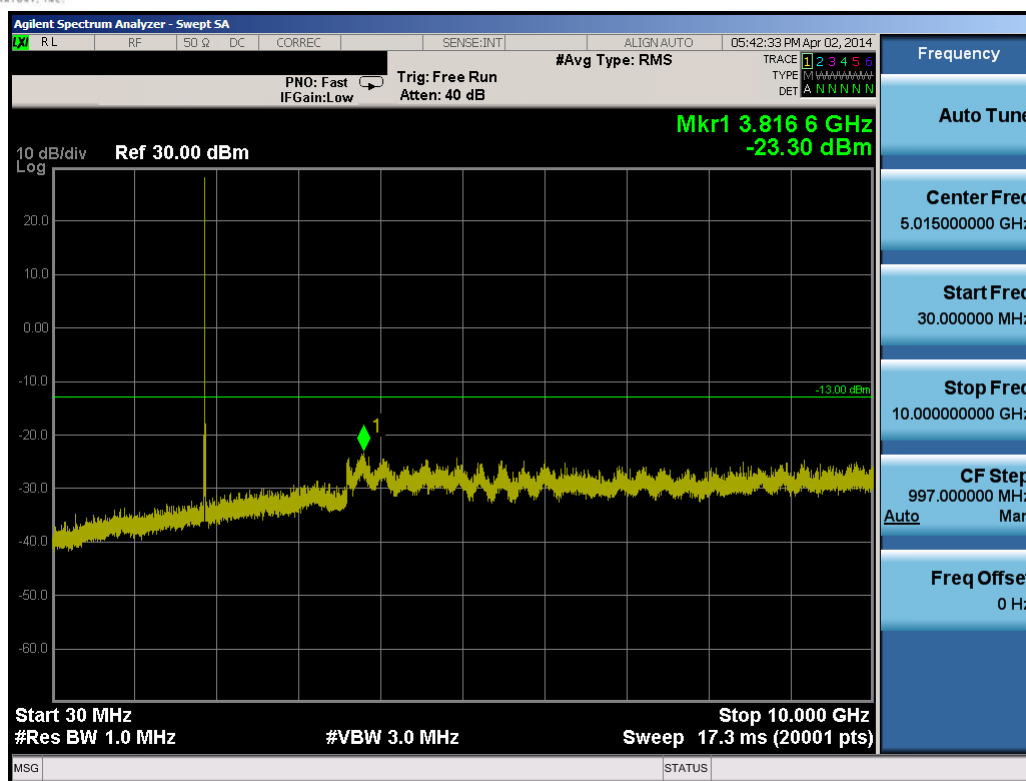
Plot 10-31. Conducted Spurious Plot (10.0MHz QPSK – RB Size 1, RB Offset 0 – Mid Channel)
