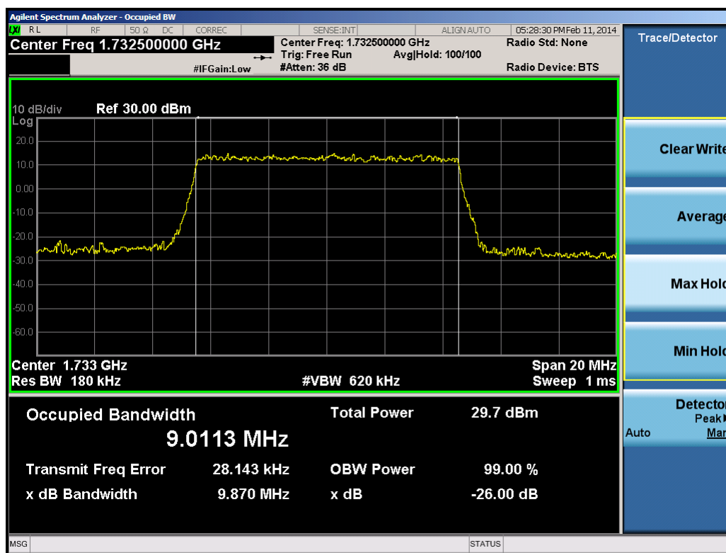
Plot 9-46. Occupied Bandwidth Plot (10.0MHz 16-QAM – RB Size 50)
