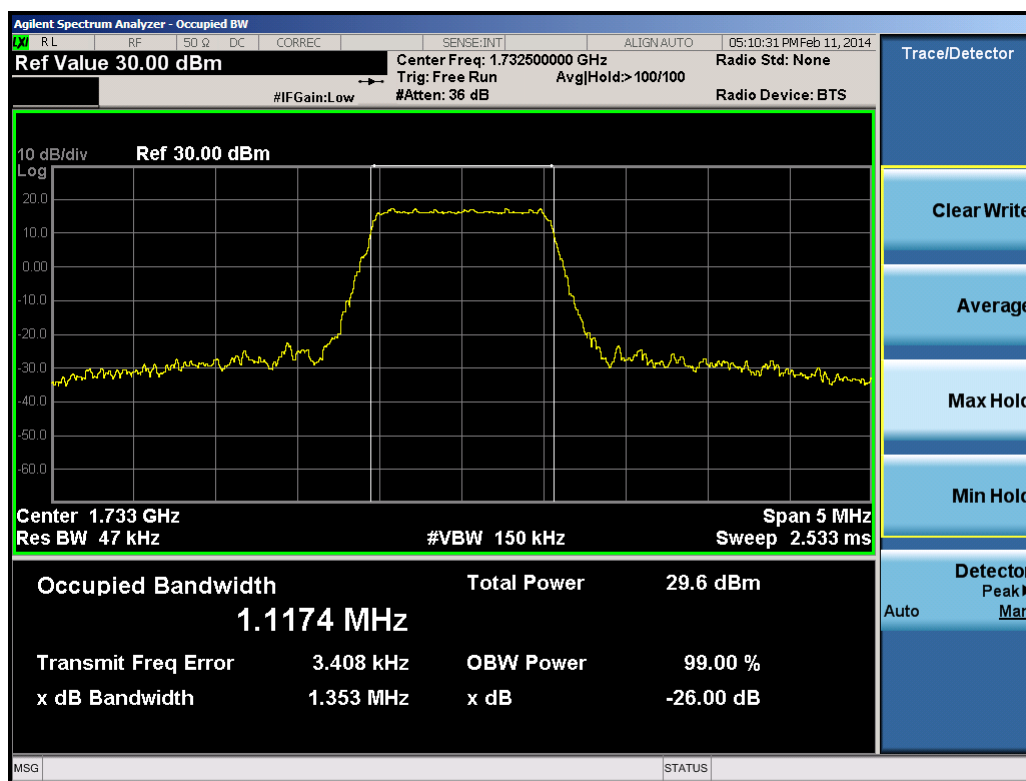
Plot 9-4. Occupied Bandwidth Plot (1.4MHz 16-QAM – RB Size 6)
