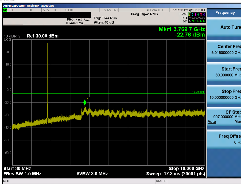
Plot 10-29. Conducted Spurious Plot (10.0MHz QPSK – RB Size 1, RB Offset 0– Low Channel)
