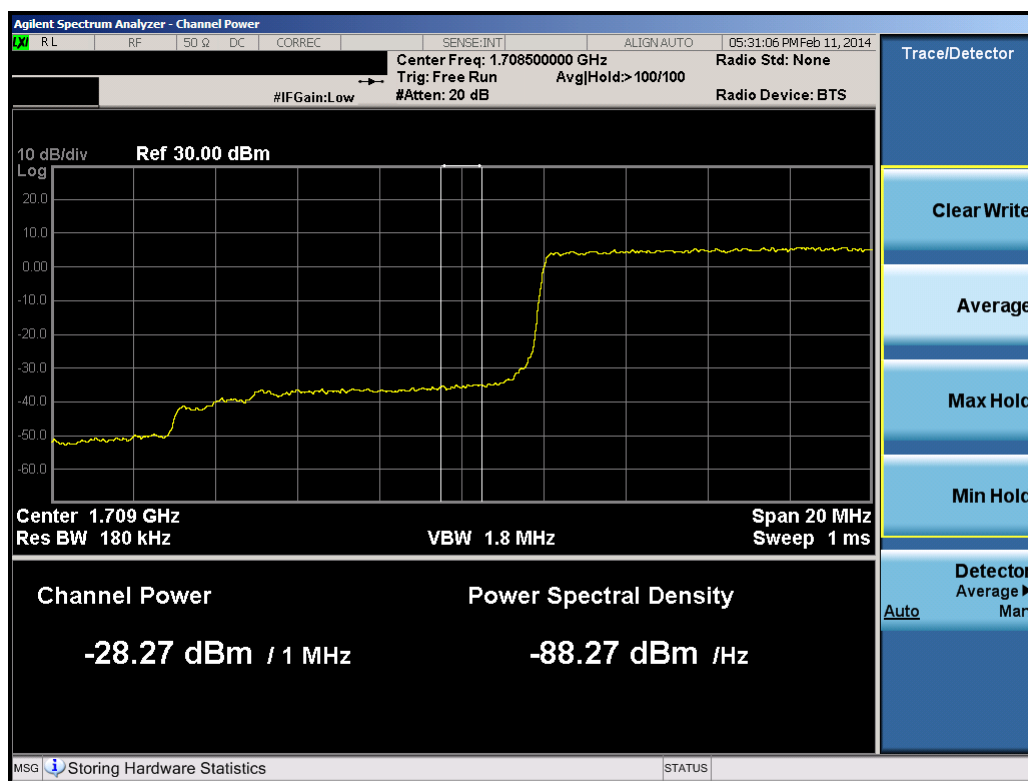
Plot 9-44. Lower Extended Band Edge Plot (10.0MHz QPSK – RB Size 50)
