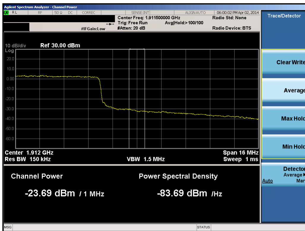
Plot 10-52. Upper Extended Band Edge Plot (20.0MHz QPSK – RB Size 100)
