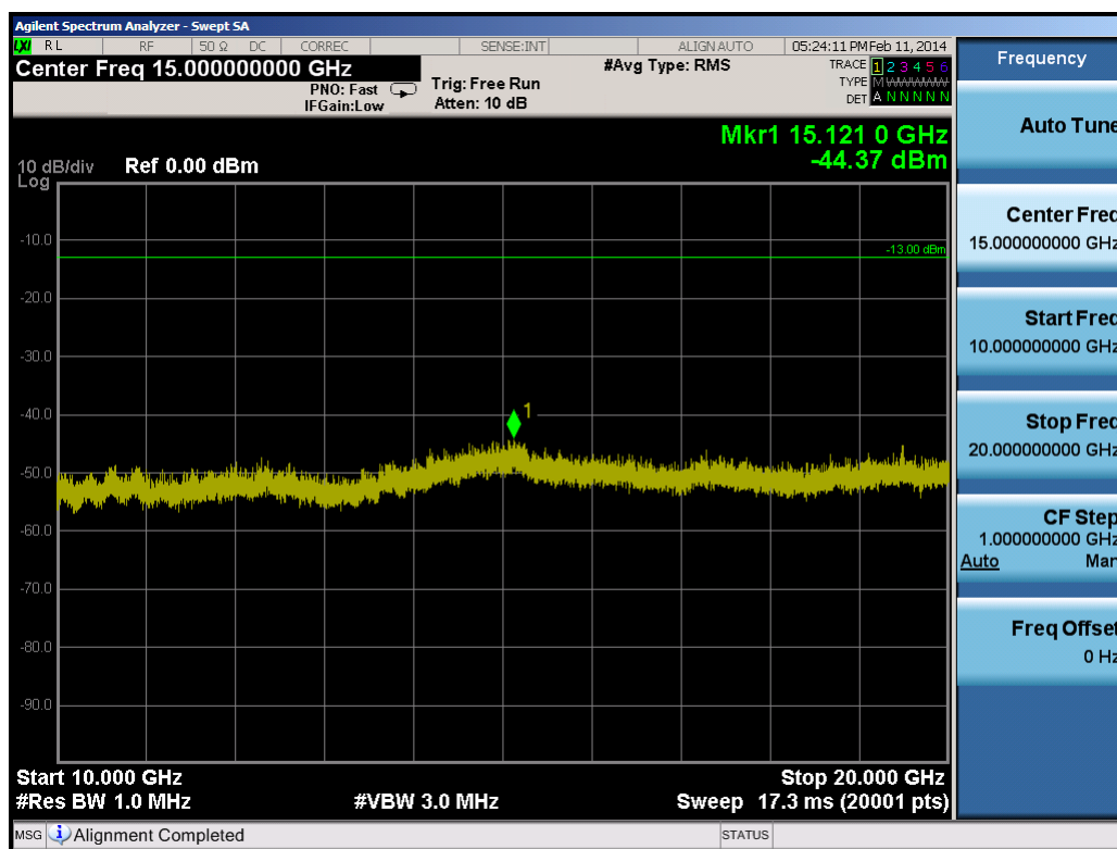
Plot 9-36. Conducted Spurious Plot (5.0MHz QPSK – RB Size 1, RB Offset 0 – Mid Channel)
