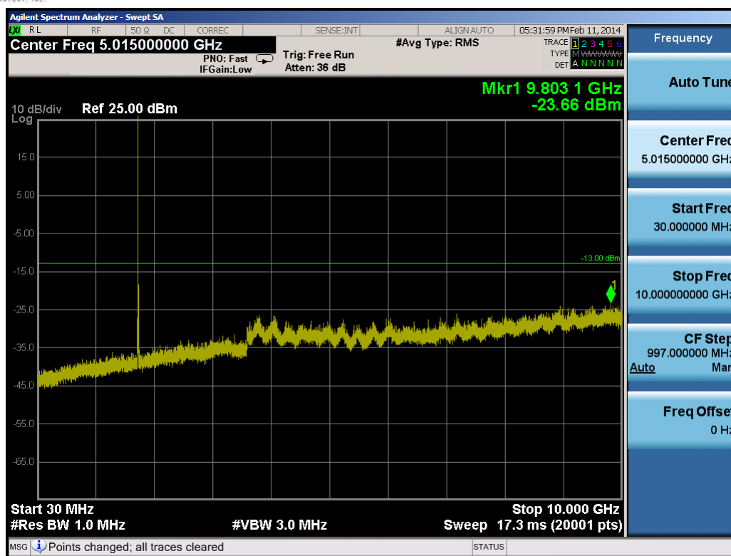
Plot 9-51. Conducted Spurious Plot (10.0MHz QPSK – RB Size 1, RB Offset 0 – High Channel)
