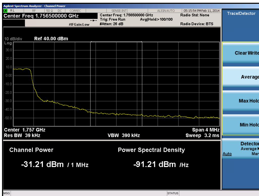
Plot 9-12. Upper Extended Band Edge Plot (1.4MHz QPSK – RB Size 6)
