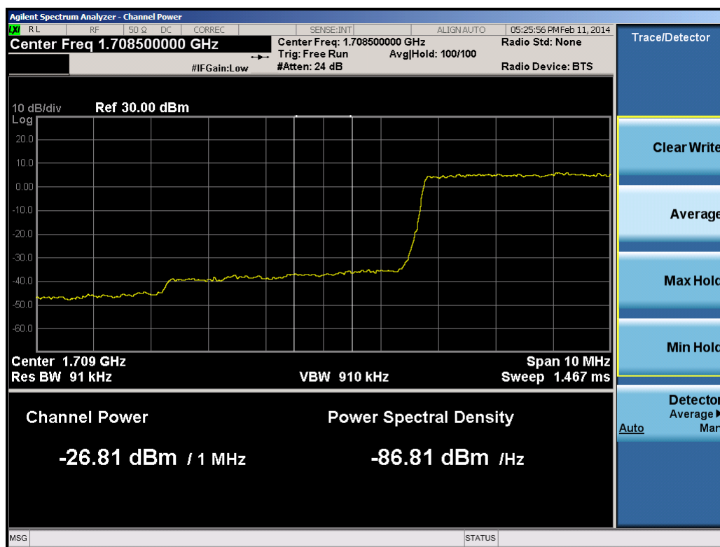
Plot 9-30. Lower Extended Band Edge Plot (5.0MHz QPSK – RB Size 25)
