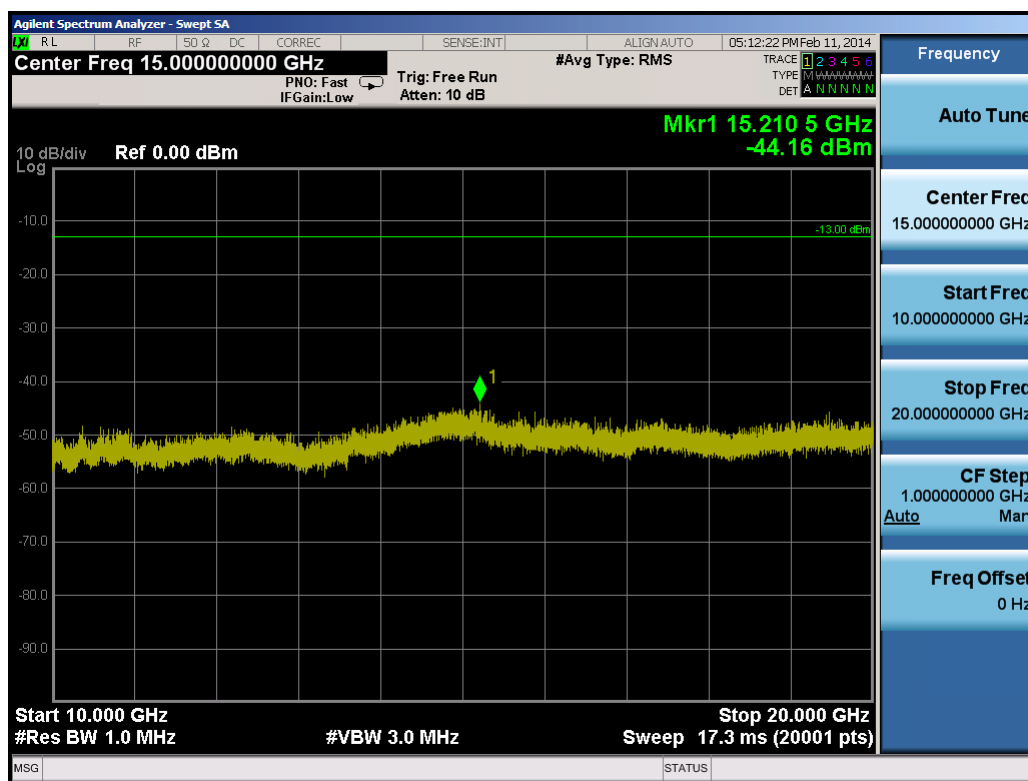
Plot 9-6. Conducted Spurious Plot (1.4MHz QPSK – RB Size 1, RB Offset 0 – Low Channel)
