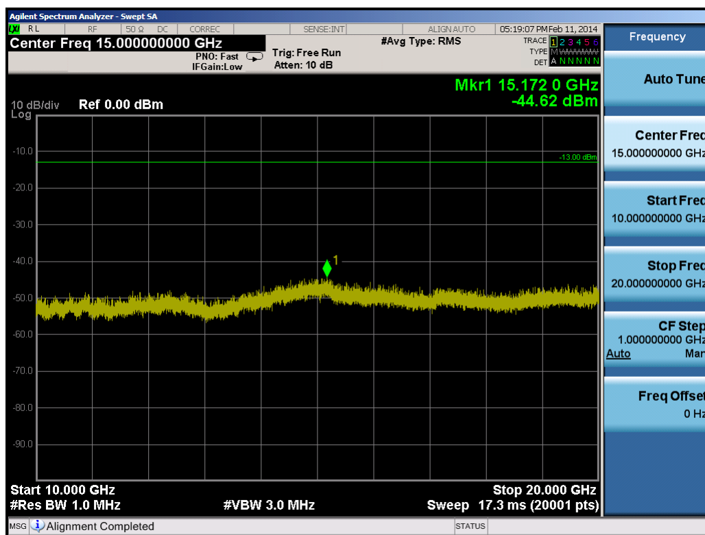
Plot 9-20. Conducted Spurious Plot (3.0MHz QPSK – RB Size 1, RB Offset 0 – Low Channel)
