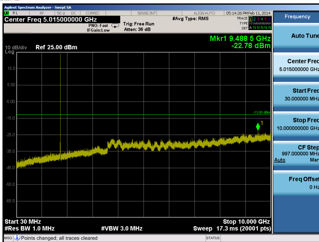
Plot 9-9. Conducted Spurious Plot (1.4MHz QPSK – RB Size 1, RB Offset 0 – High Channel)
