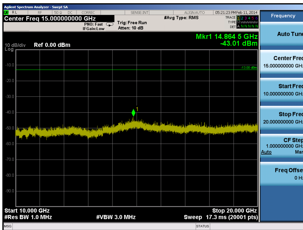
Plot 9-24. Conducted Spurious Plot (3.0MHz QPSK – RB Size 1, RB Offset 0 – High Channel)
