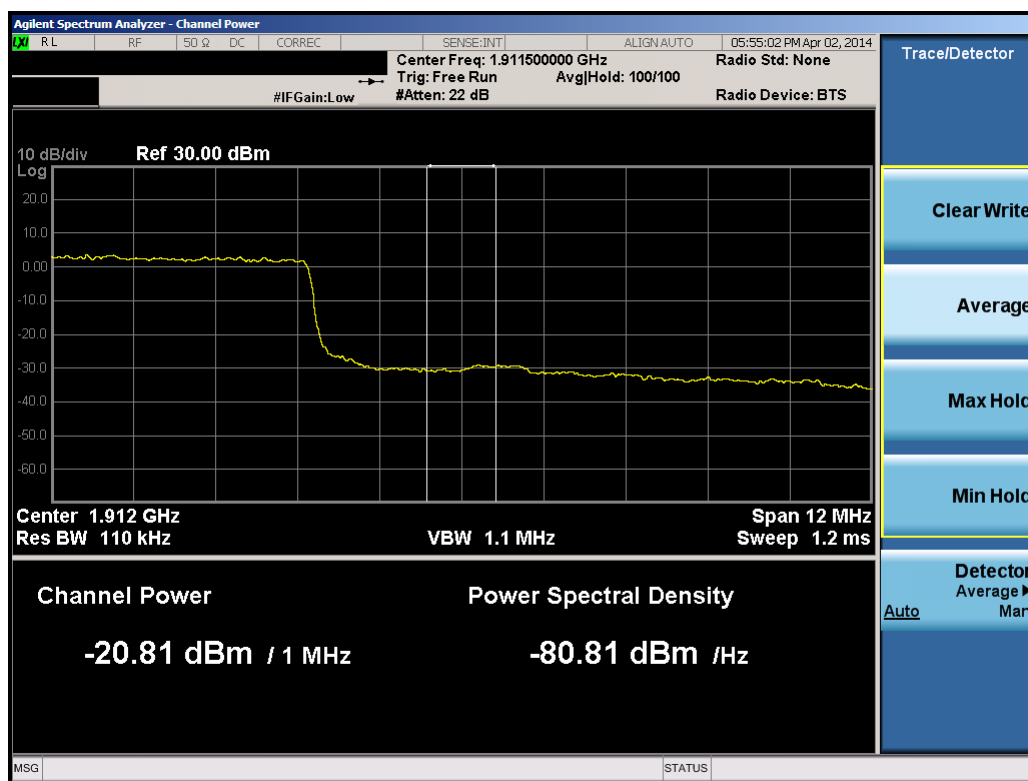
Plot 10-44. Upper Extended Band Edge Plot (15.0MHz QPSK – RB Size 75)
