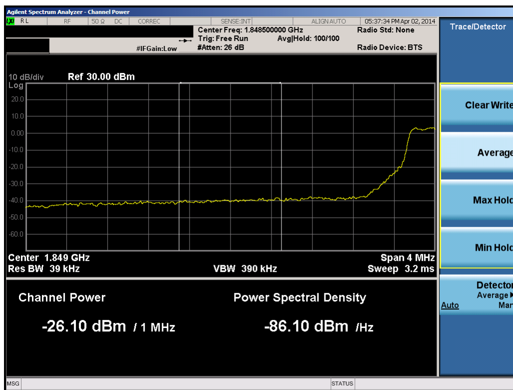
Plot 10-18. Lower Extended Band Edge Plot (5.0MHz QPSK – RB Size 25)
