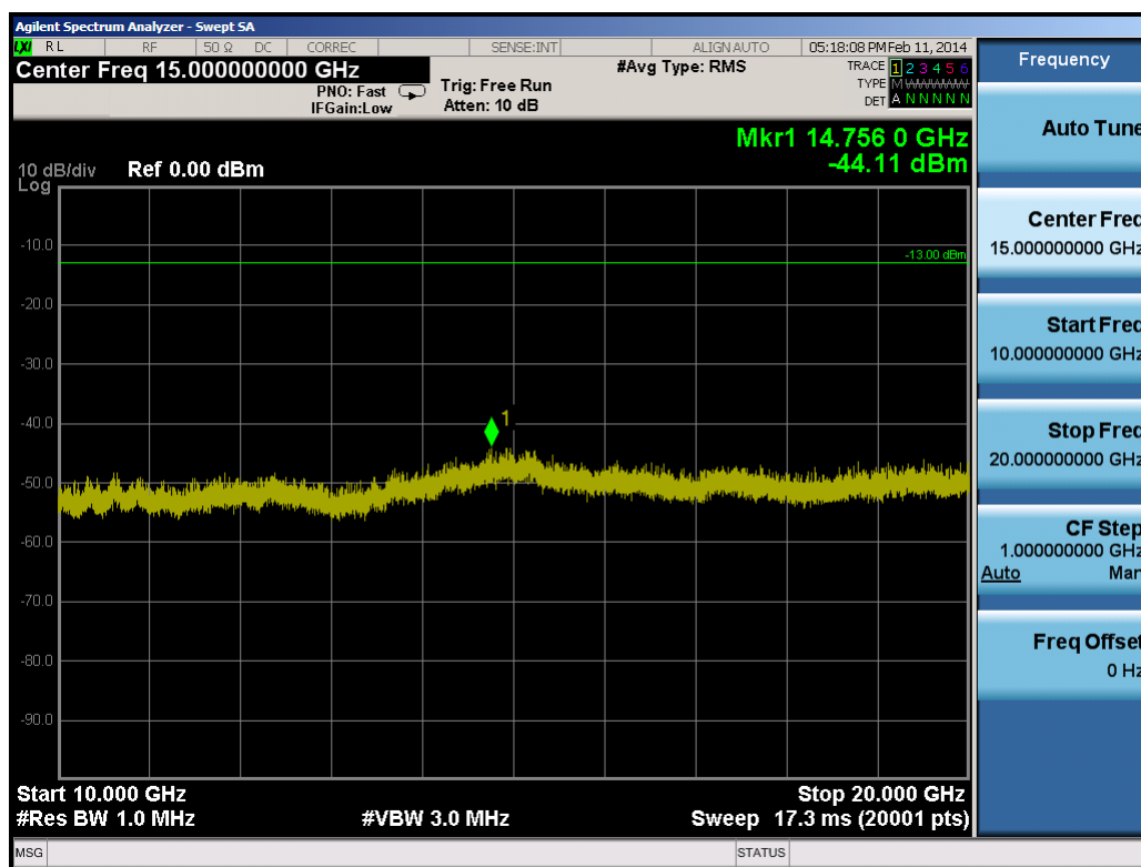
Plot 9-22. Conducted Spurious Plot (3.0MHz QPSK – RB Size 1, RB Offset 0 – Mid Channel)
