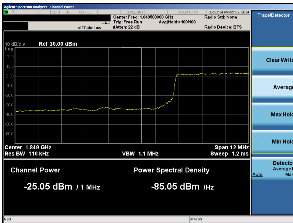
Plot 10-40. Lower Extended Band Edge Plot (15.0MHz QPSK – RB Size 75)
