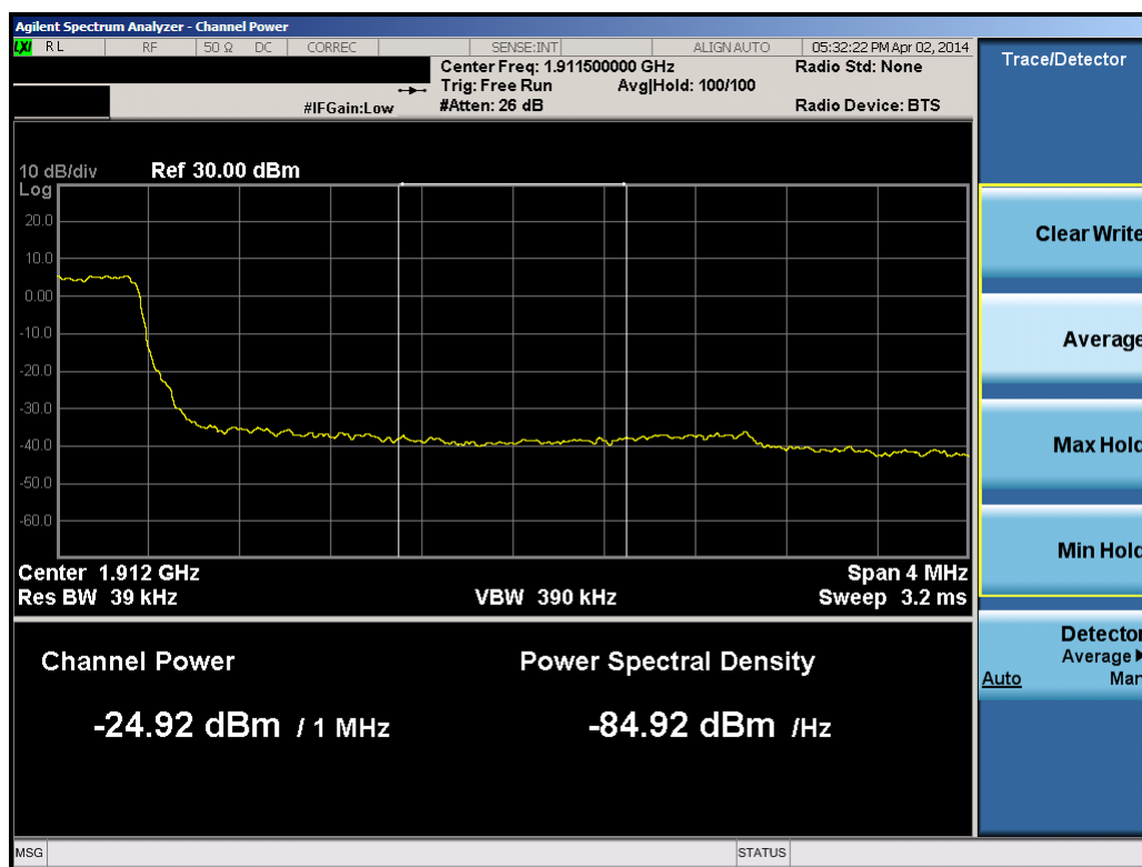
Plot 10-14. Upper Extended Band Edge Plot (3.0MHz QPSK – RB Size 15)
