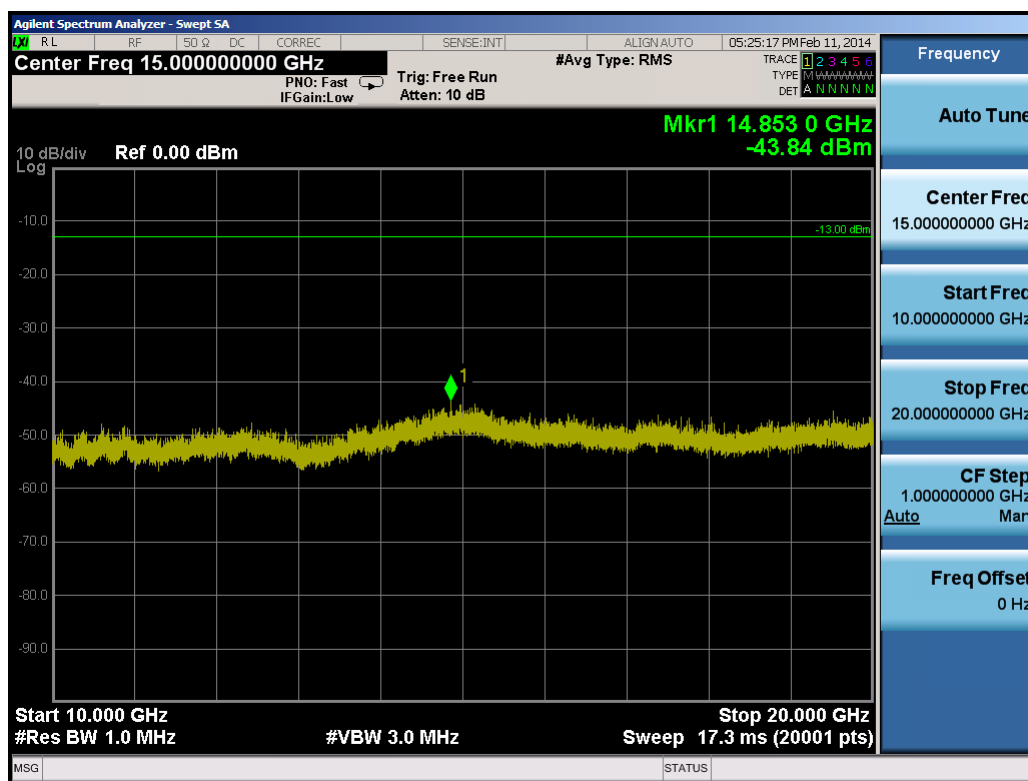
Plot 9-34. Conducted Spurious Plot (5.0MHz QPSK – RB Size 1, RB Offset 0 – Low Channel)
