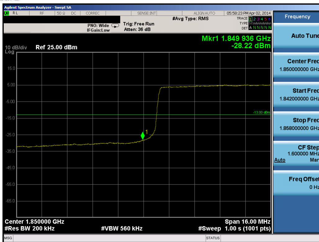
Plot 10-47. Lower Band Edge Plot (20.0MHz QPSK – RB Size 100)
