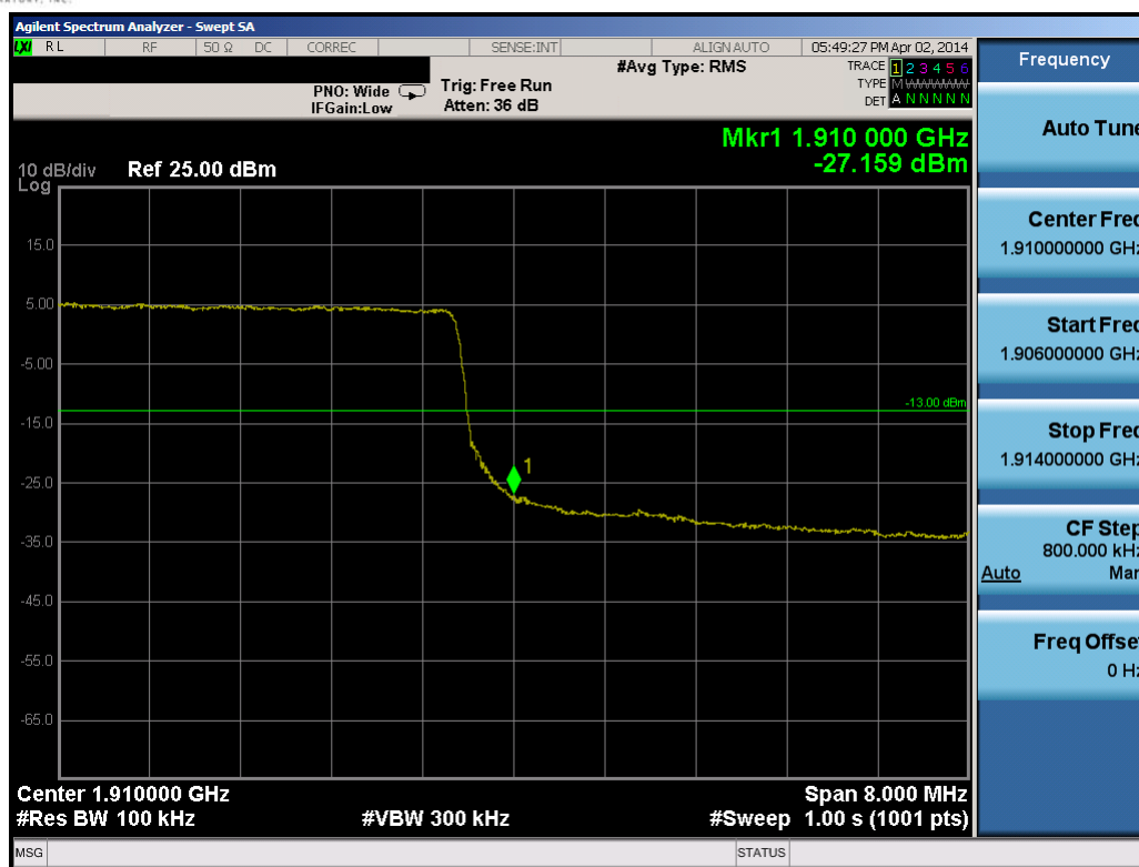
Plot 10-35. Upper Band Edge Plot (10.0MHz QPSK – RB Size 50)
