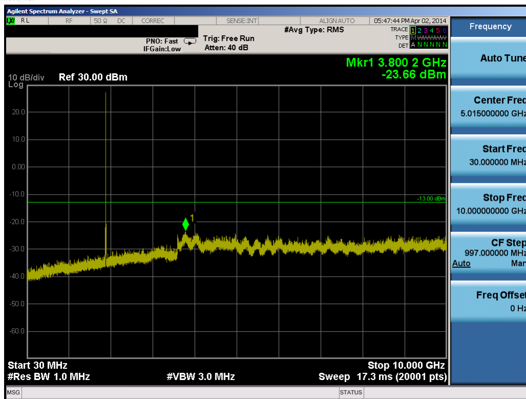
Plot 10-33. Conducted Spurious Plot (10.0MHz QPSK – RB Size 1, RB Offset 0 – High Channel)
