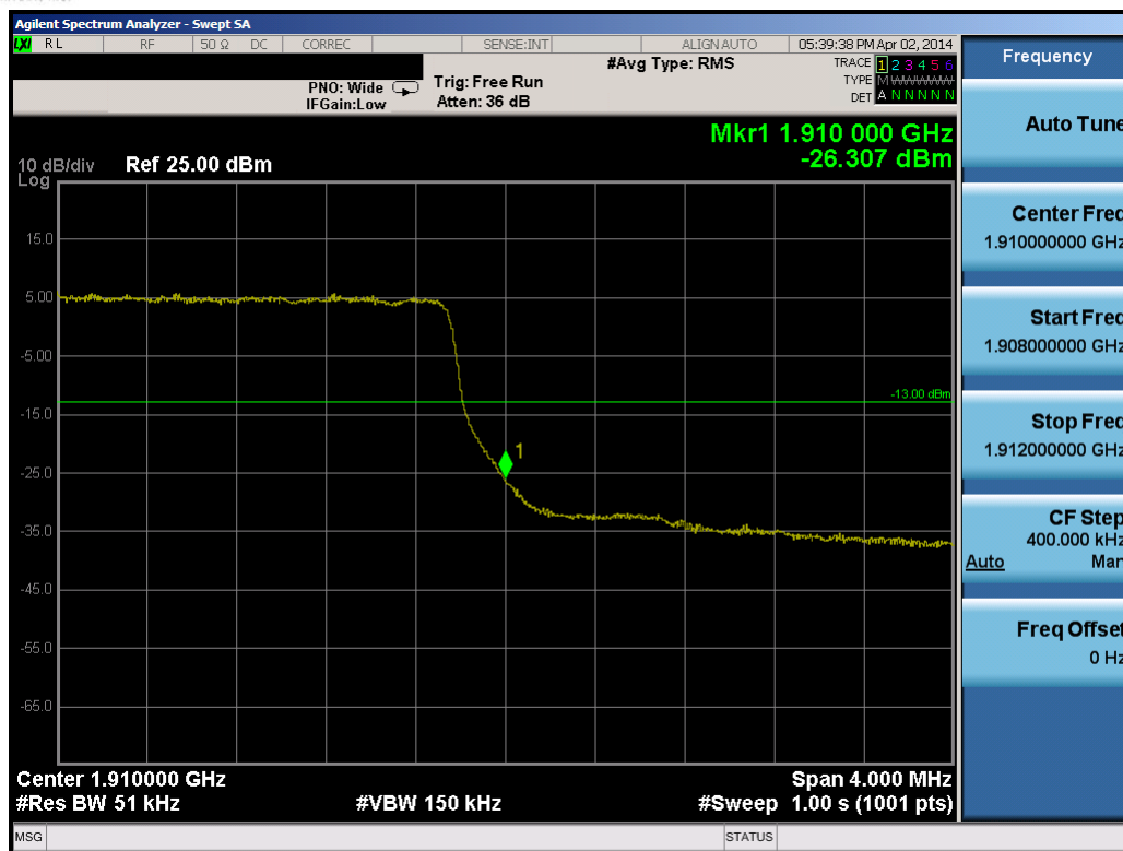
Plot 10-21. Upper Band Edge Plot (5.0MHz QPSK – RB Size 25)
