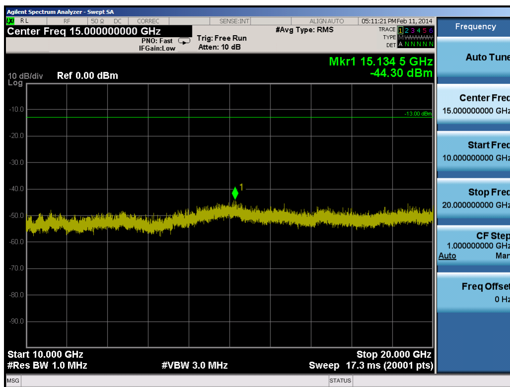
Plot 9-8. Conducted Spurious Plot (1.4MHz QPSK – RB Size 1, RB Offset 0 – Mid Channel)
