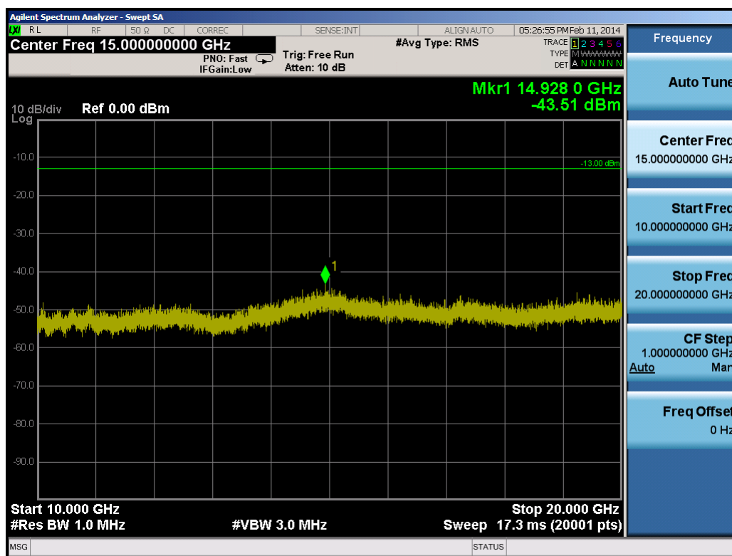
Plot 9-38. Conducted Spurious Plot (5.0MHz QPSK – RB Size 1, RB Offset 0 – High Channel)
