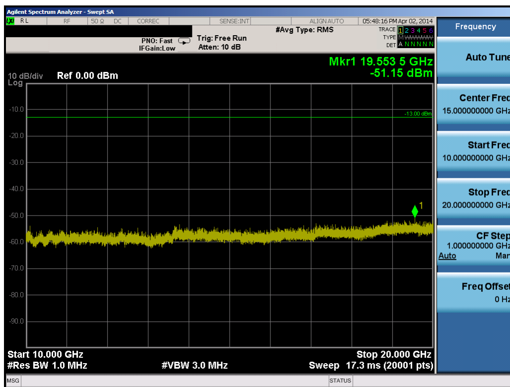
Plot 10-34. Conducted Spurious Plot (10.0MHz QPSK – RB Size 1, RB Offset 0 – High Channel)
