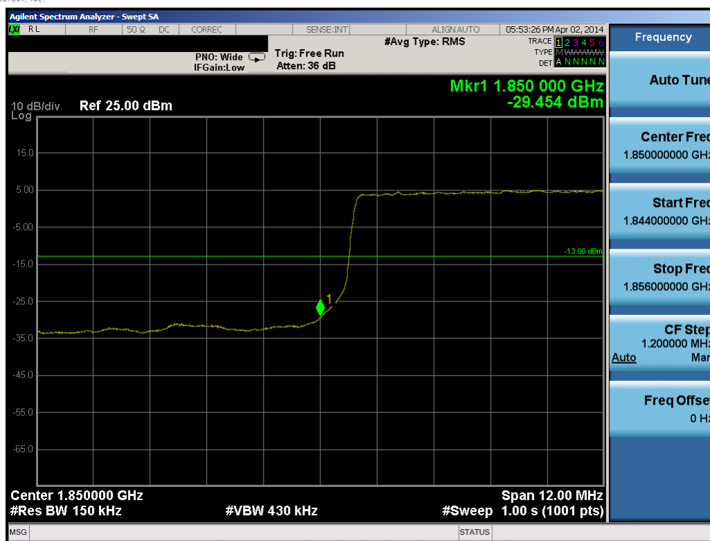
Plot 10-39. Lower Band Edge Plot (15.0MHz QPSK – RB Size 75)
