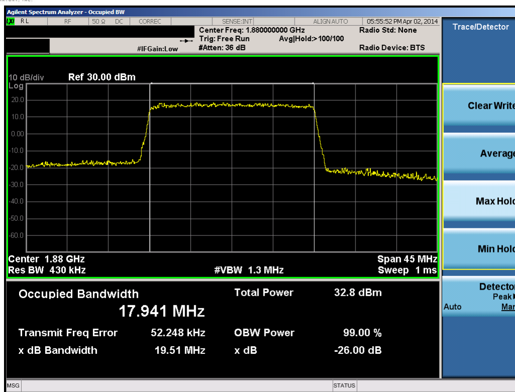
Plot 10-49. Occupied Bandwidth Plot (20.0MHz QPSK – RB Size 100)
