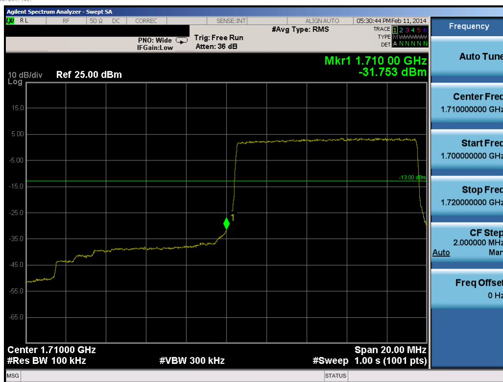
Plot 9-43. Lower Band Edge Plot (10.0MHz QPSK – RB Size 50)
