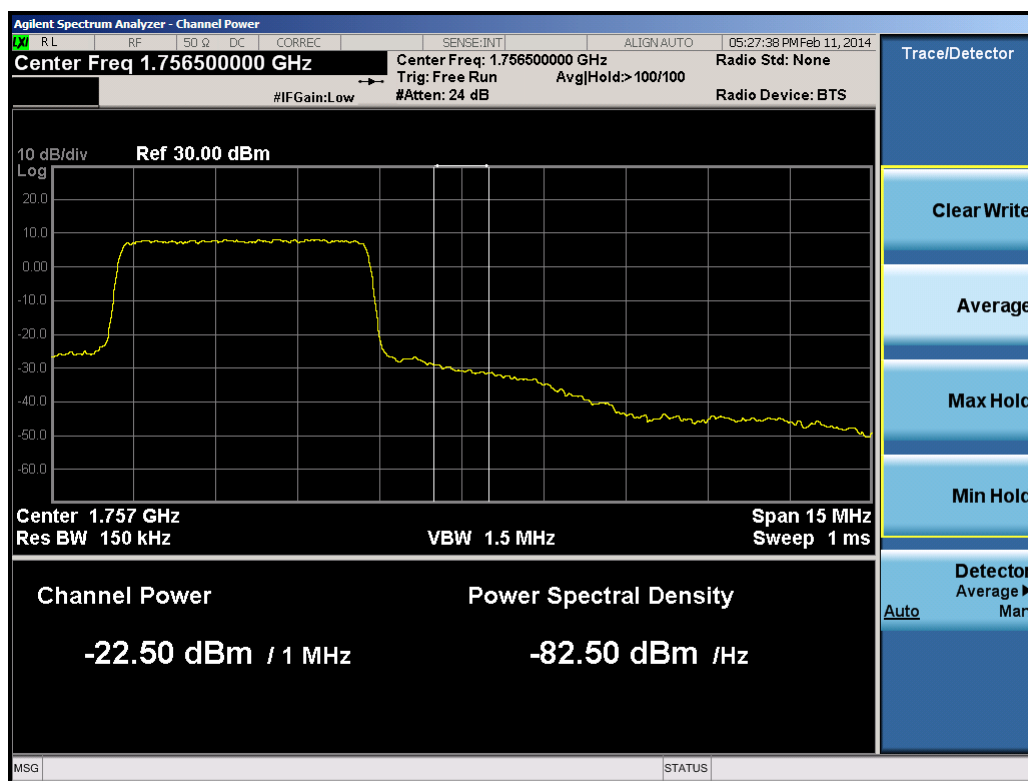
Plot 9-40. Upper Extended Band Edge Plot (5.0MHz QPSK – RB Size 25)
