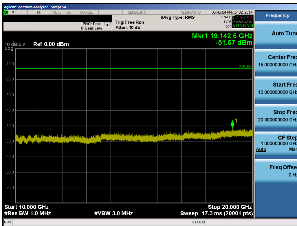
Plot 10-30. Conducted Spurious Plot (10.0MHz QPSK – RB Size 1, RB Offset 0 – Low Channel)
