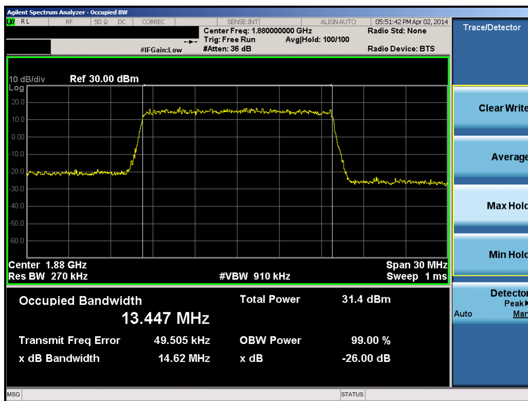
Plot 10-42. Occupied Bandwidth Plot (15.0MHz 16-QAM – RB Size 75)
