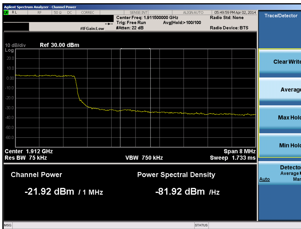
Plot 10-36. Upper Extended Band Edge Plot (10.0MHz QPSK – RB Size 50)
