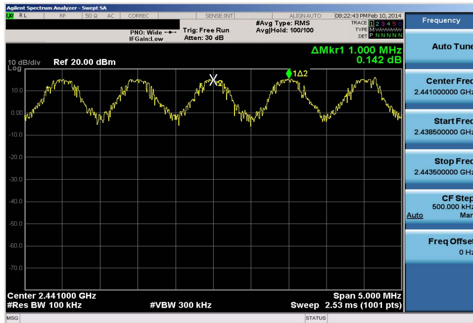
Plot 6-32. Channel Spacing Plot (Bluetooth)
