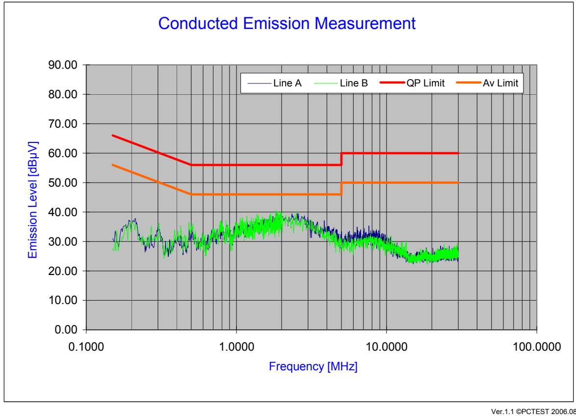
Plot 6-42. Line Conducted Plot with Bluetooth
