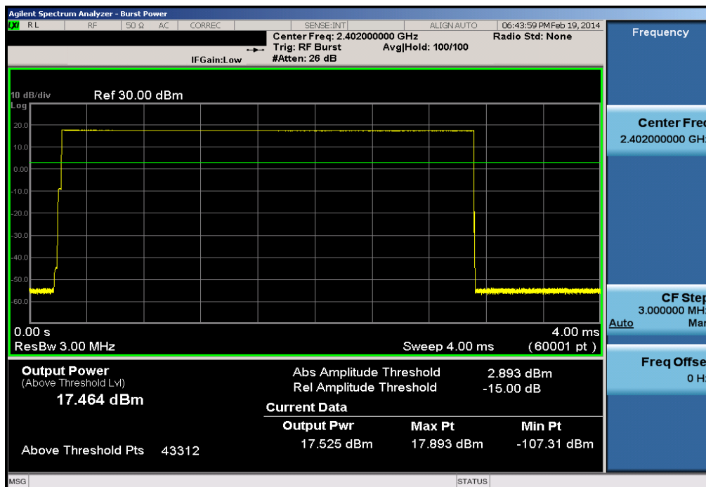
Plot 6-19. Average Conducted Power (1Mbps – Ch. 0)
