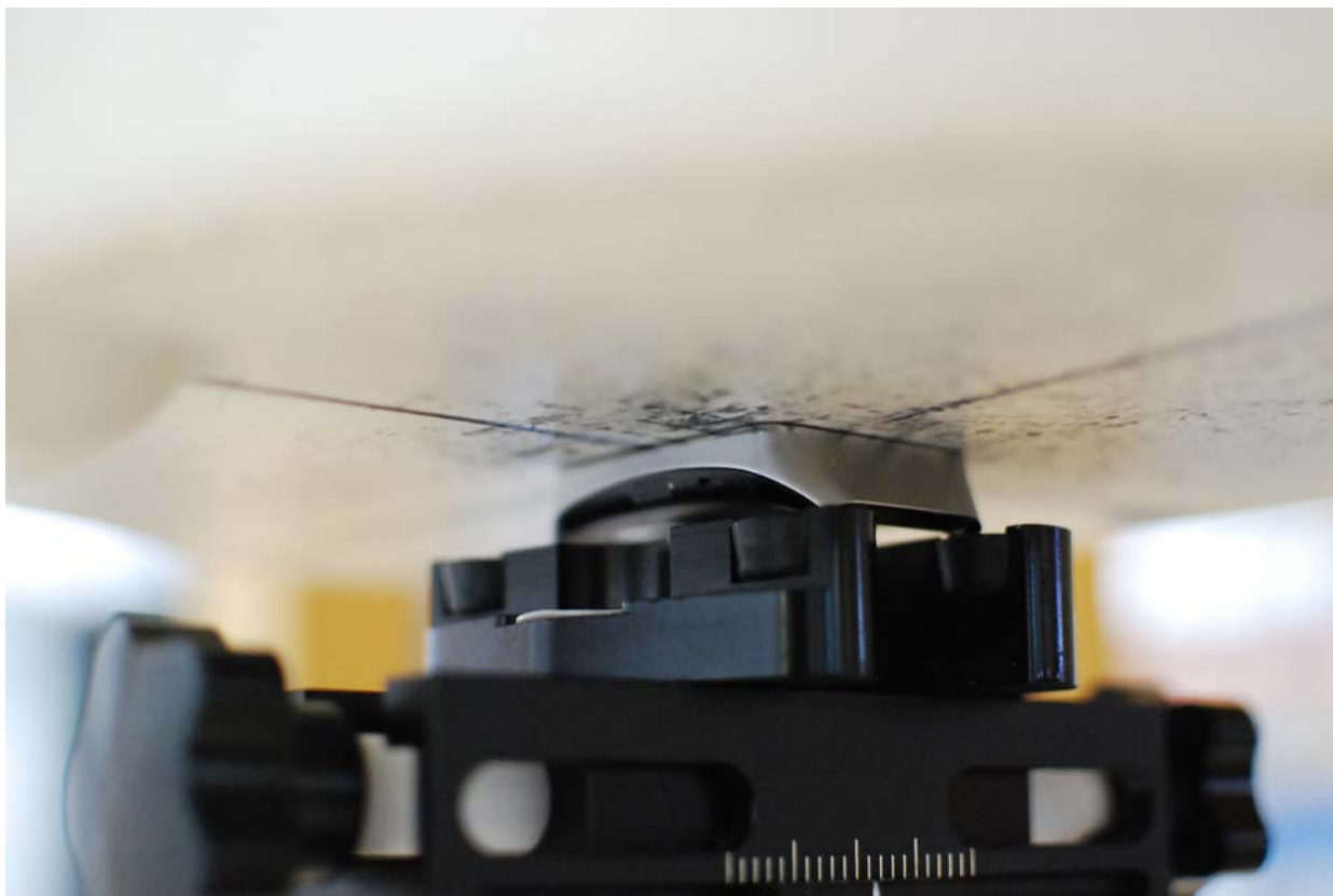
SAR Test Setup Photo 3: Front Side at 0.0 cm
