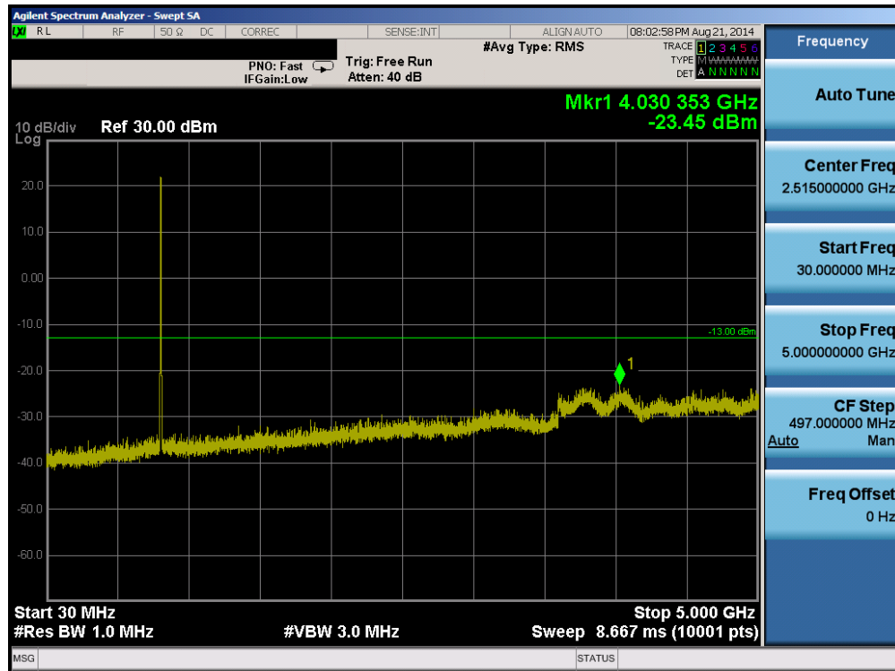
Plot 6-13. Conducted Spurious Plot (Cellular WCDMA Mode – Ch. 4132)
