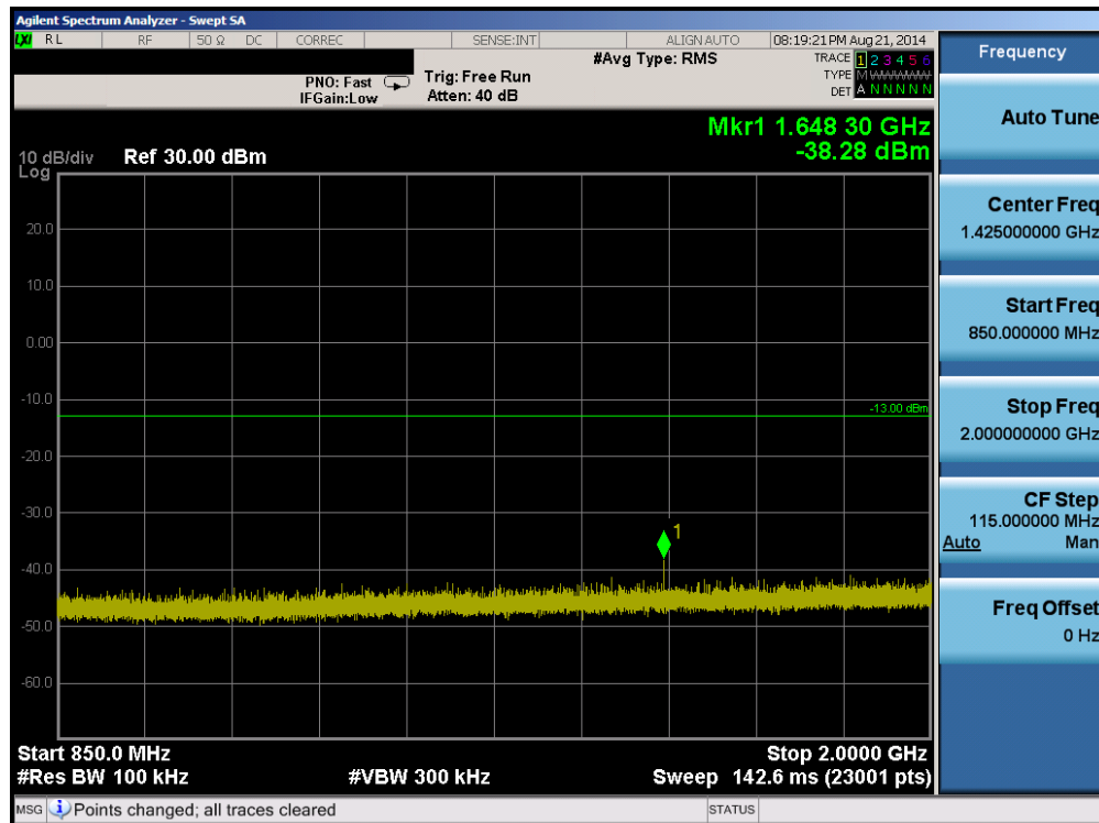
Plot 6-5. Conducted Spurious Plot (Cellular GPRS Mode – Ch. 128)
