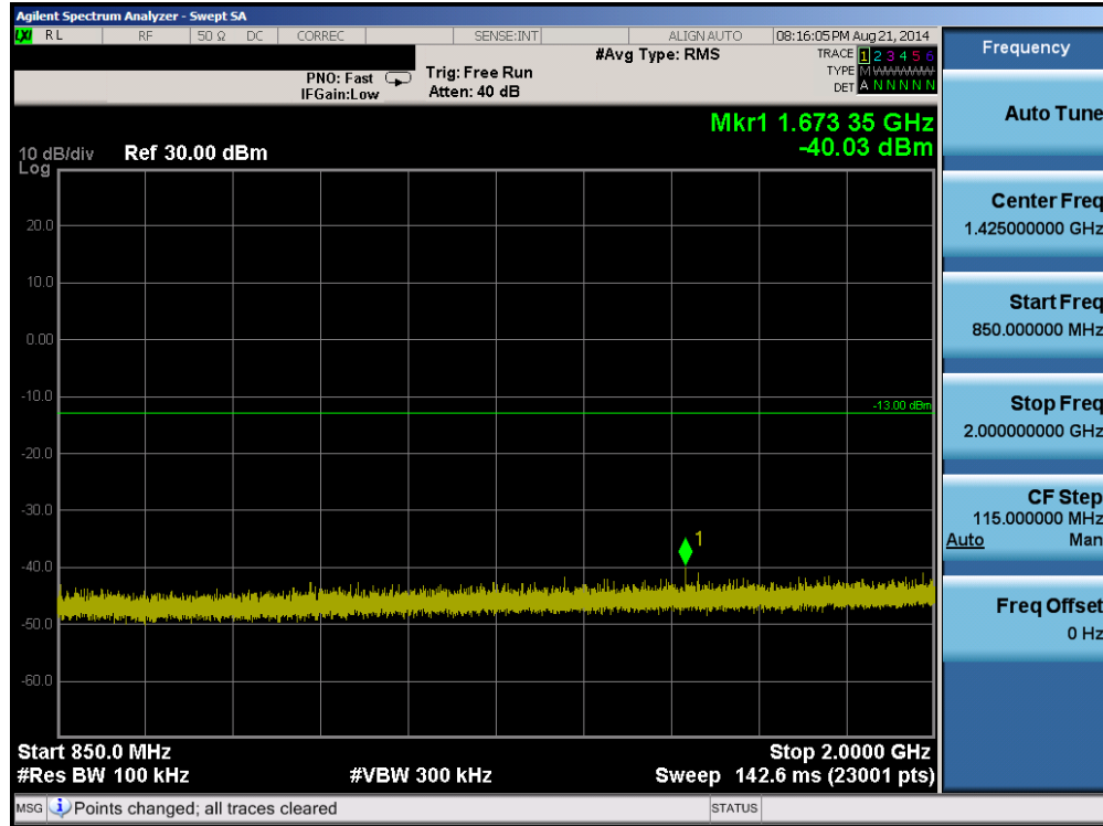
Plot 6-8. Conducted Spurious Plot (Cellular GPRS Mode – Ch. 190)
