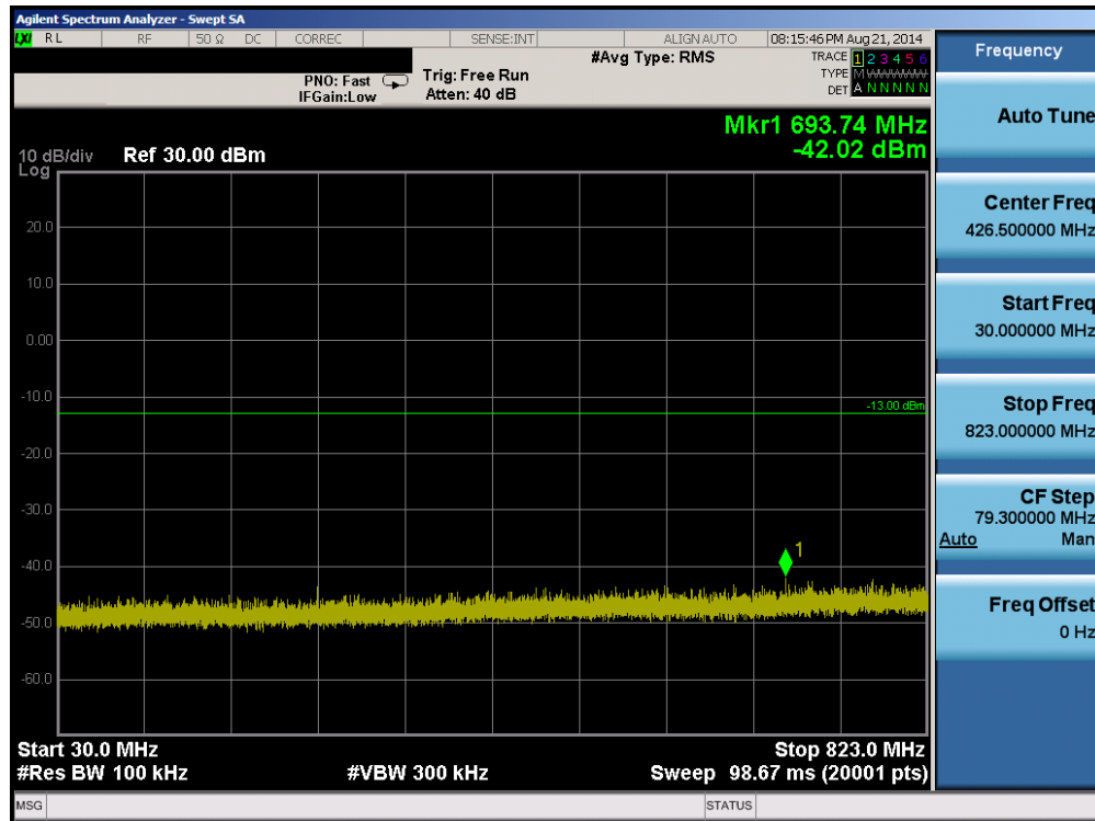
Plot 6-7. Conducted Spurious Plot (Cellular GPRS Mode – Ch. 190)
