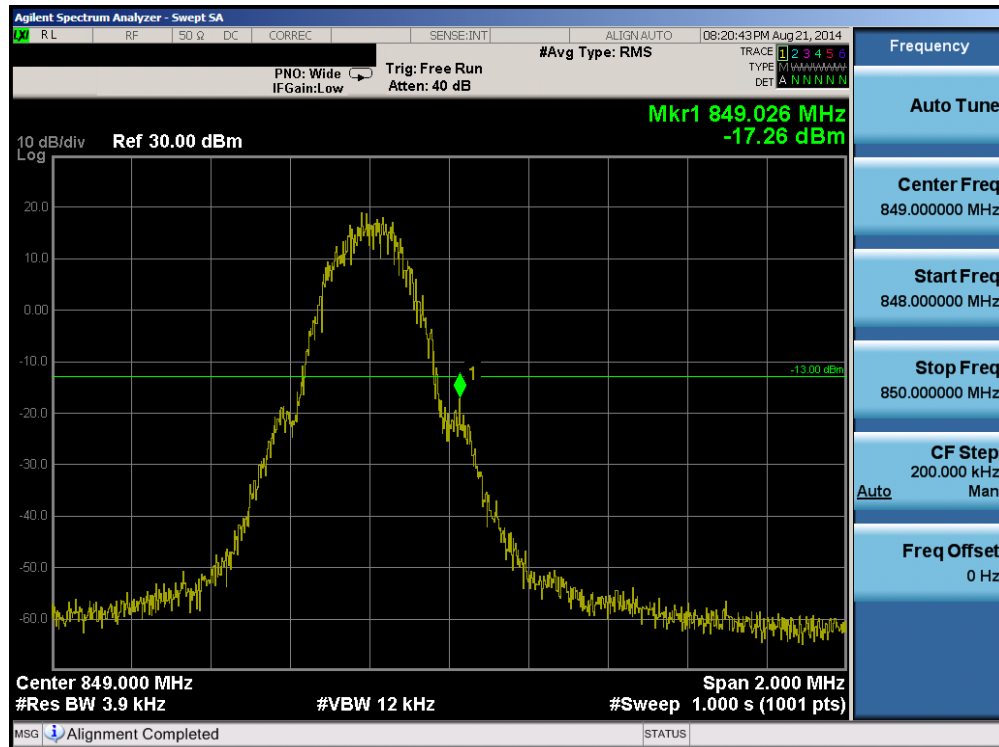
Plot 6-20. Band Edge Plot (Cellular GPRS Mode – Ch. 251)
