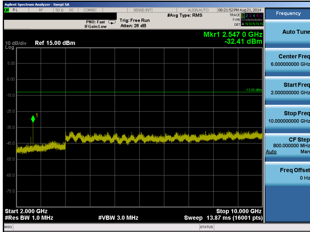
Plot 6-12. Conducted Spurious Plot (Cellular GPRS Mode – Ch. 251)
