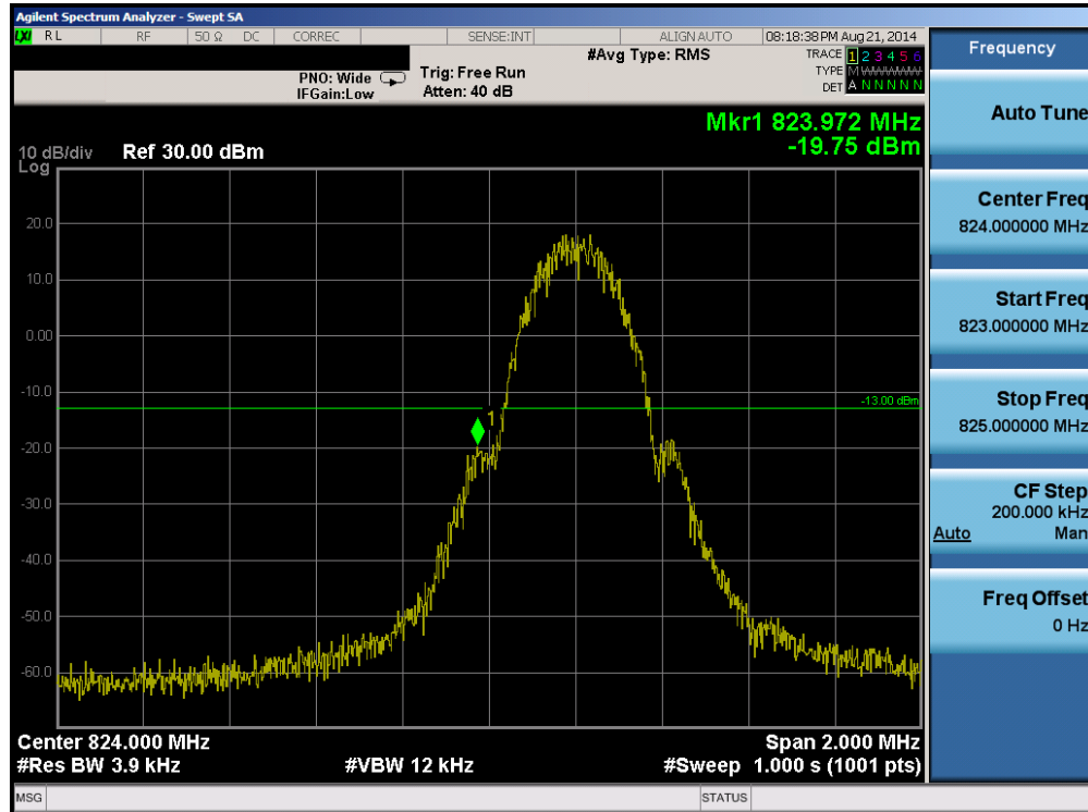
Plot 6-19. Band Edge Plot (Cellular GPRS Mode – Ch. 128)
