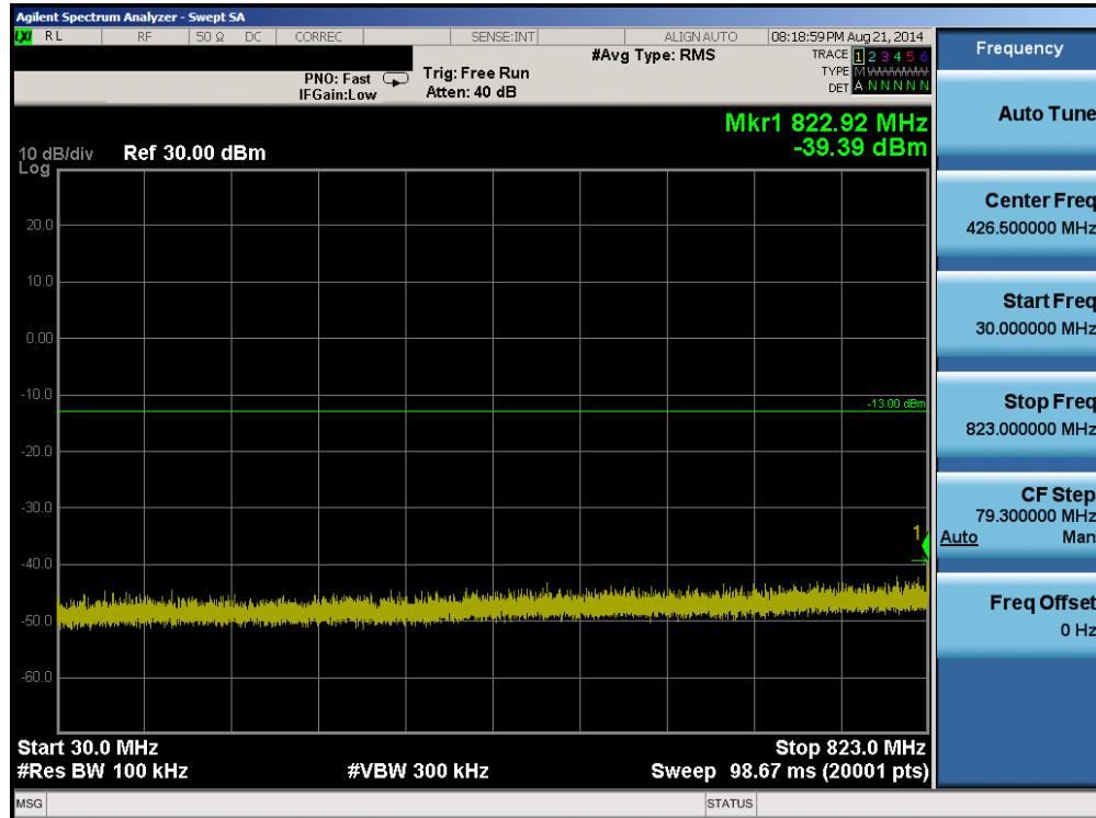
Plot 6-4. Conducted Spurious Plot (Cellular GPRS Mode – Ch. 128)
