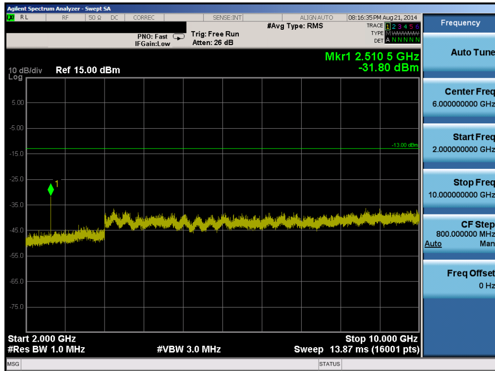
Plot 6-9. Conducted Spurious Plot (Cellular GPRS Mode – Ch. 190)
