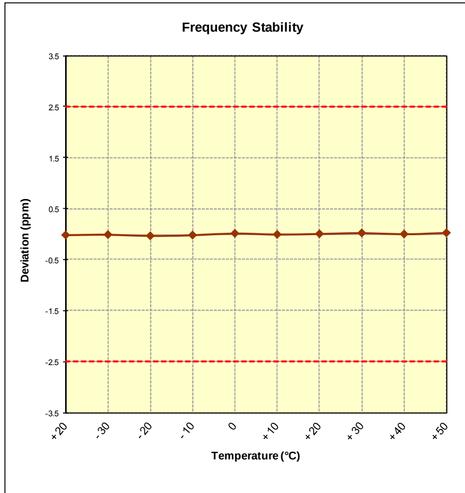
Figure 6-6. Frequency Stability Graph (Cellular GPRS Mode – Ch. 190)
