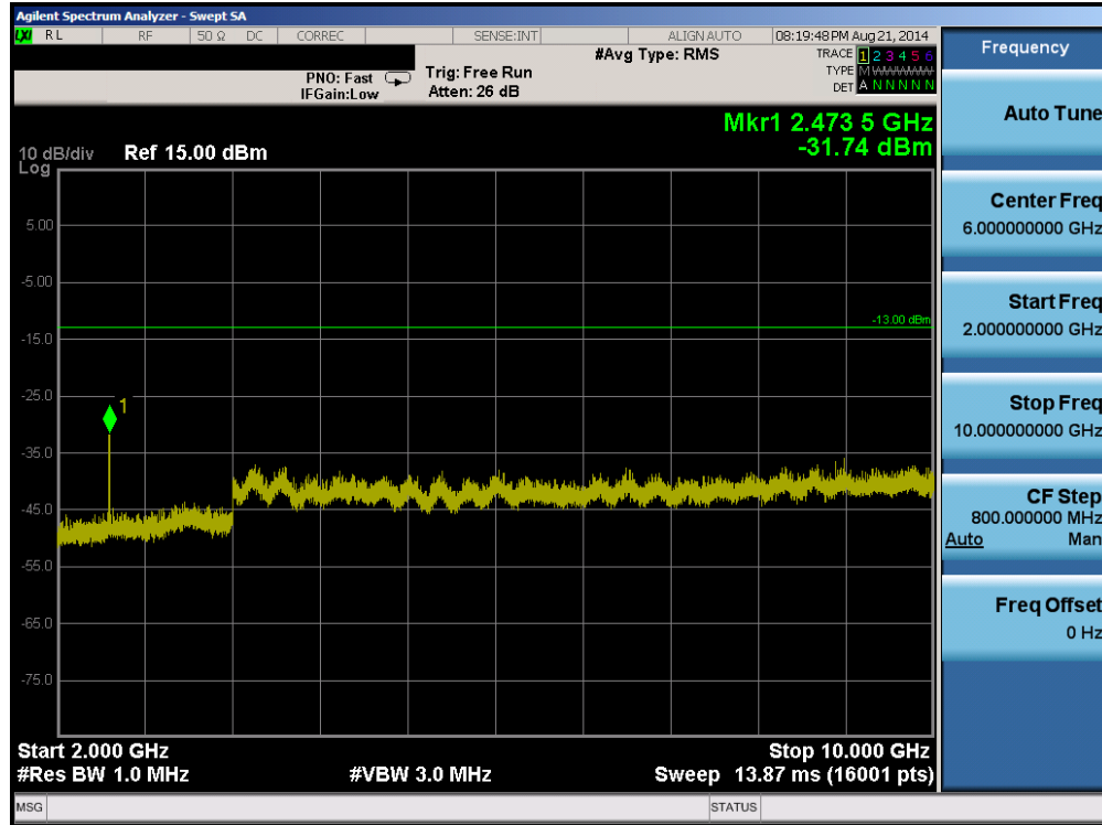
Plot 6-6. Conducted Spurious Plot (Cellular GPRS Mode – Ch. 128)
