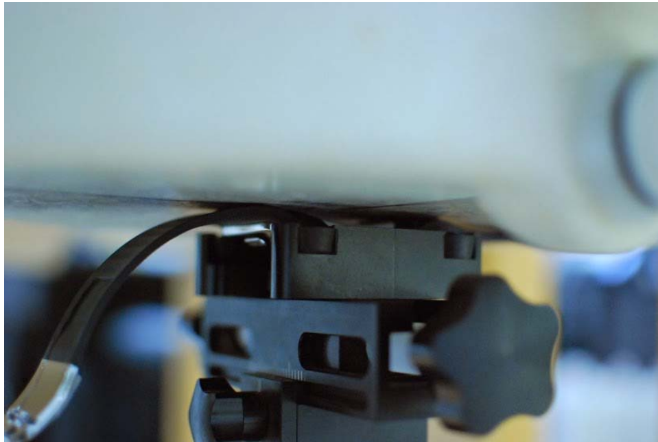
SAR Test Setup Photo 3 - Back Side at 0.0 cm (Side view)
