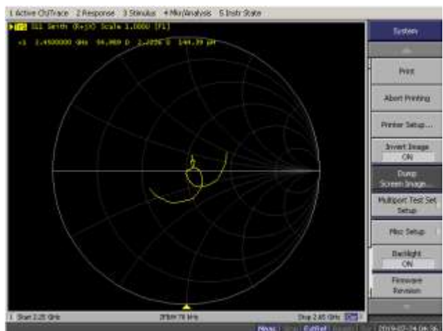
&lt; Figure 2. Measurement result of Head Impedance &gt;
