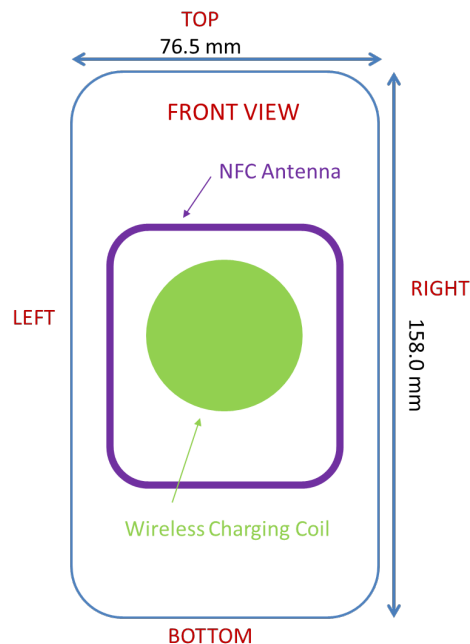
Figure K-2 NFC Antenna Locations
