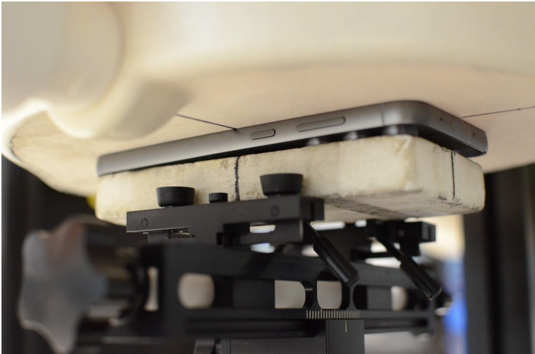
SAR Test Setup Photo 8 – Phablet, Front Side at 0 mm
