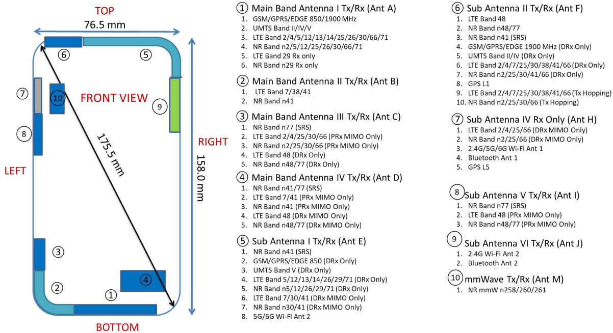
Figure K-1 DUT Antenna Locations
