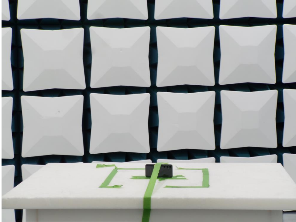
Figure 7. Test Setup – Y Position – 30MHz-1GHz
