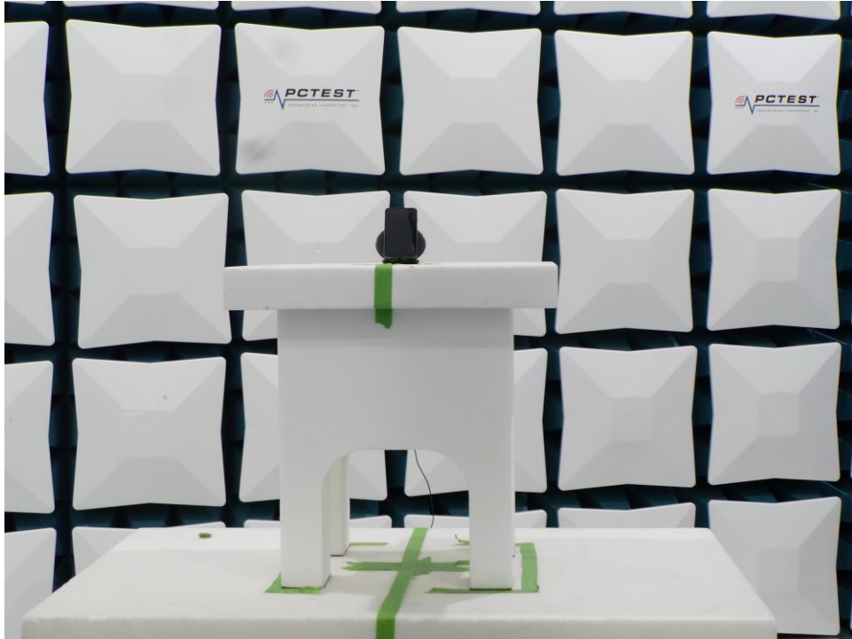
Figure 5. Test Setup – WCP Position – 1GHz-18GHz
