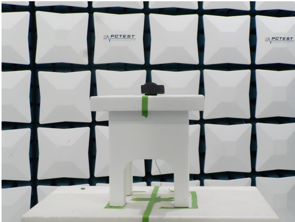
Figure 4. Test Setup – WCP Position – 1GHz-18GHz
