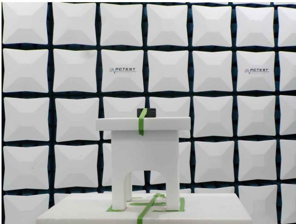
Figure 2. Test Setup – Y Position – 1GHz-18GHz
