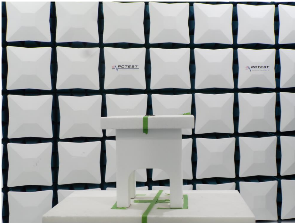
Figure 1. Test Setup – X Position – 1GHz-18GHz
