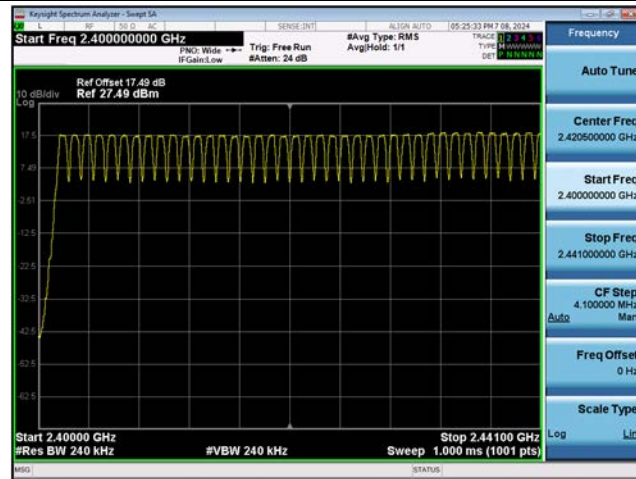
ANT.1 8DPSK Number of Channels (2.4 GHz - 2.441 GHz)
