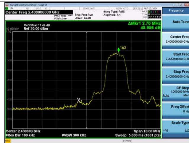
Dual ANT.2 8DPSK Band Edge(CH.0)
