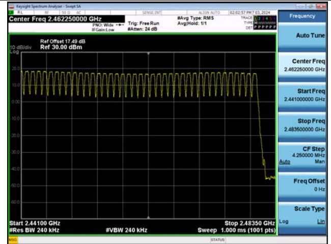
ANT.1 8DPSK Number of Channels (2.441 GHz - 2.483.5 GHz)
