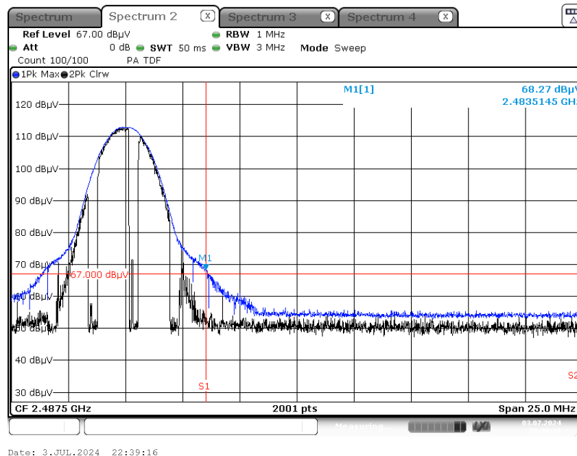
Radiated Restricted Band Edges plot – Average & Peak Result ( \pi/4 DQPSK, Ch.78, X-H)
