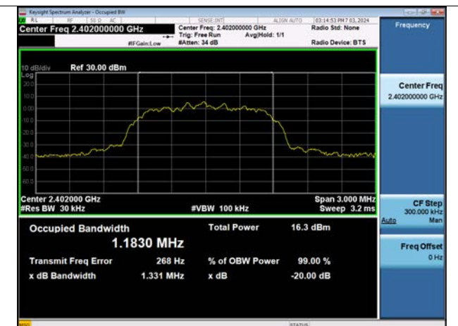
Dual ANT. 2 \pi/4 DQPSK 20 dB BW & 99% OBW (CH. 0)
