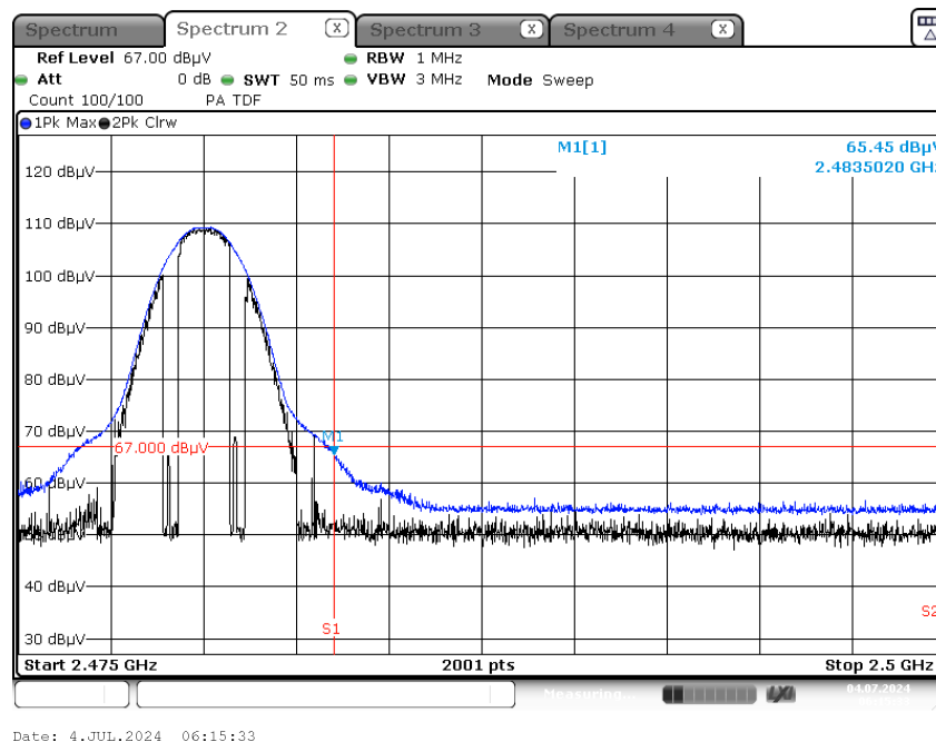
Radiated Restricted Band Edges plot – Average & Peak Result ( \pi/4 DQPSK, Ch. 78, Y-H)
