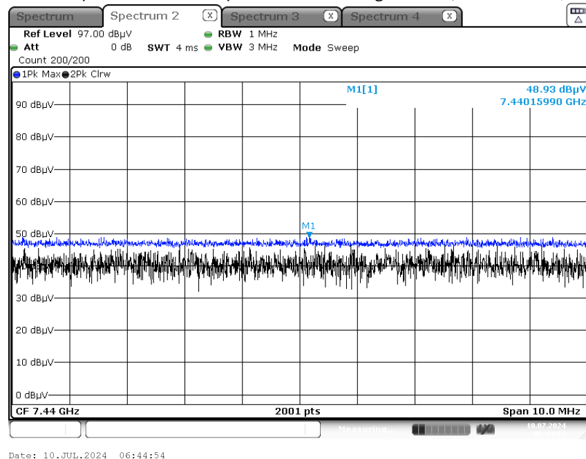
Radiated Spurious Emissions plot – Peak & Average Result (3rd Harmonic, Z-H)
