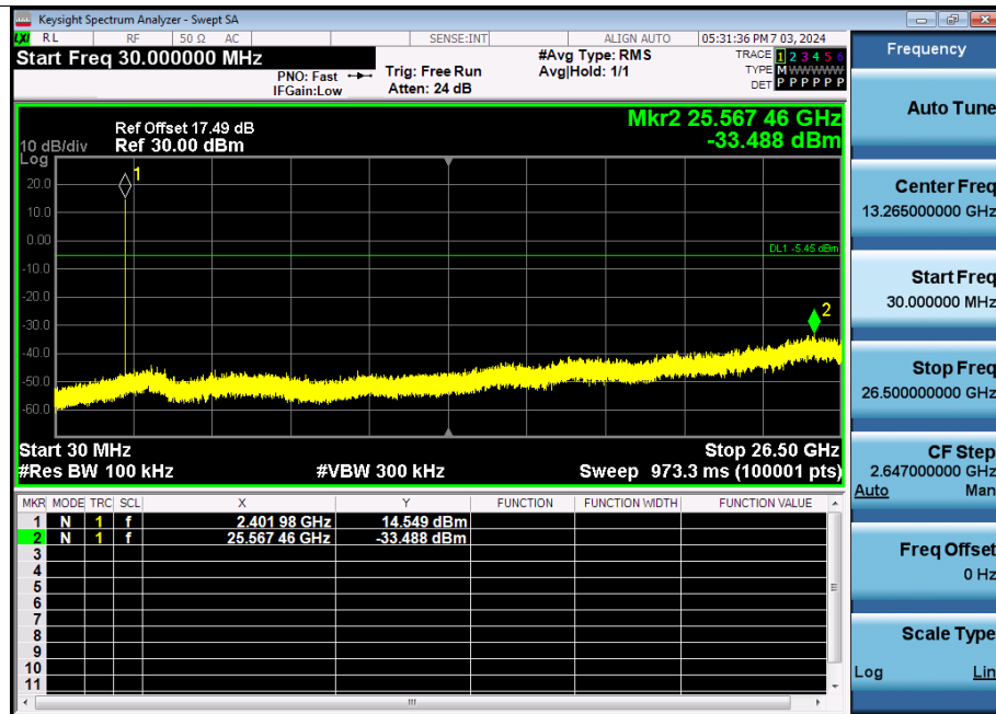
Spurious Emission (30 MHz – 26.50 GHz) Ant.2, GFSK_CH.0
