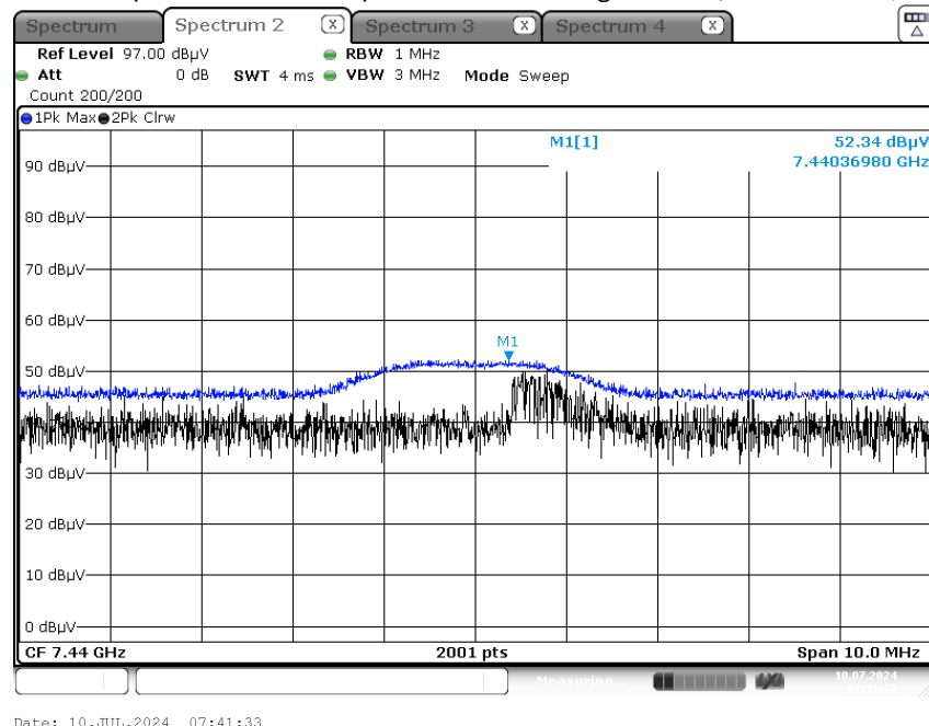
Radiated Spurious Emissions plot – Peak & Average Result (3rd Harmonic, Y-V)
