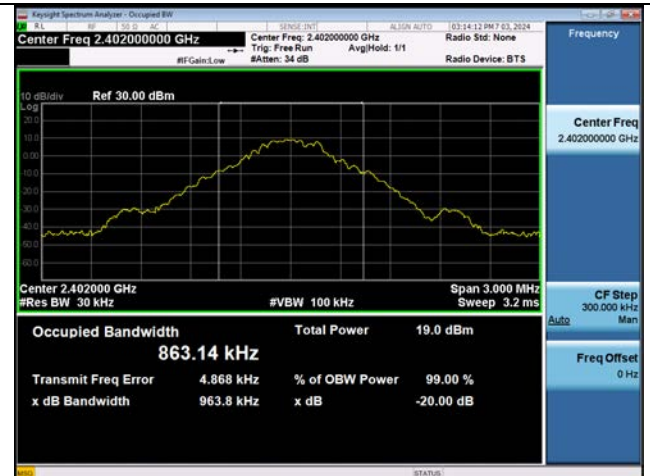
Dual ANT. 2 8DPSK 20 dB BW & 99% OBW (CH. 0)
