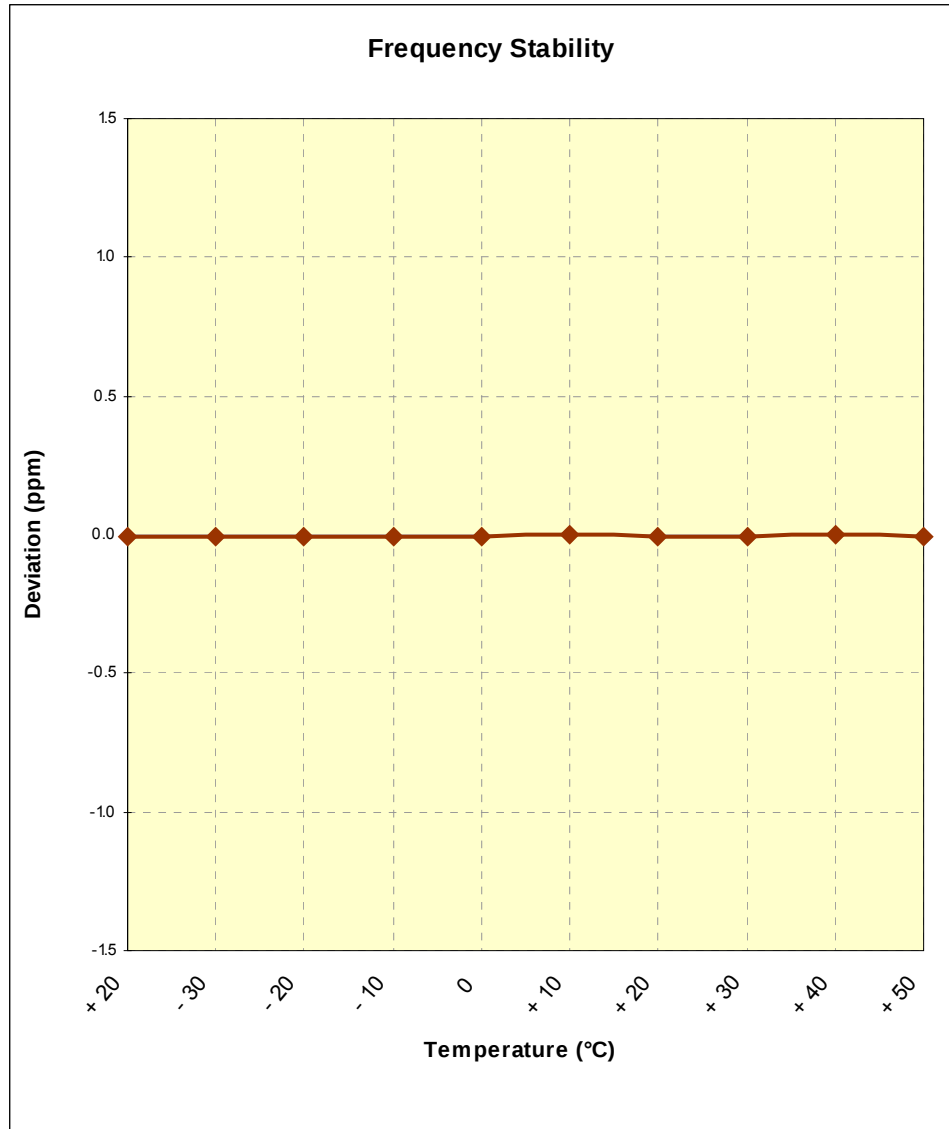
Figure 6-8. Frequency Stability Graph (PCS CDMA Mode – Ch. 600)
