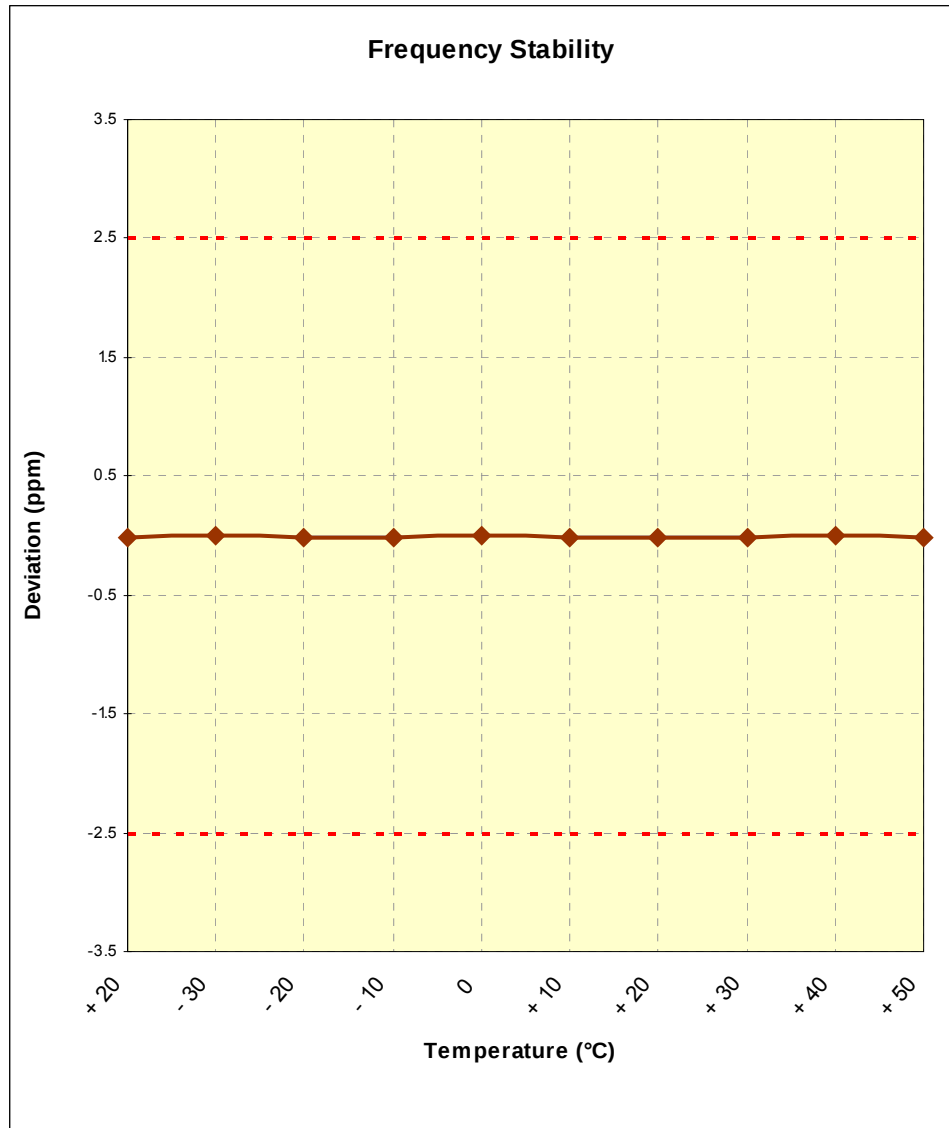
Figure 6-7. Frequency Stability Graph (Cellular CDMA Mode – Ch. 384)
