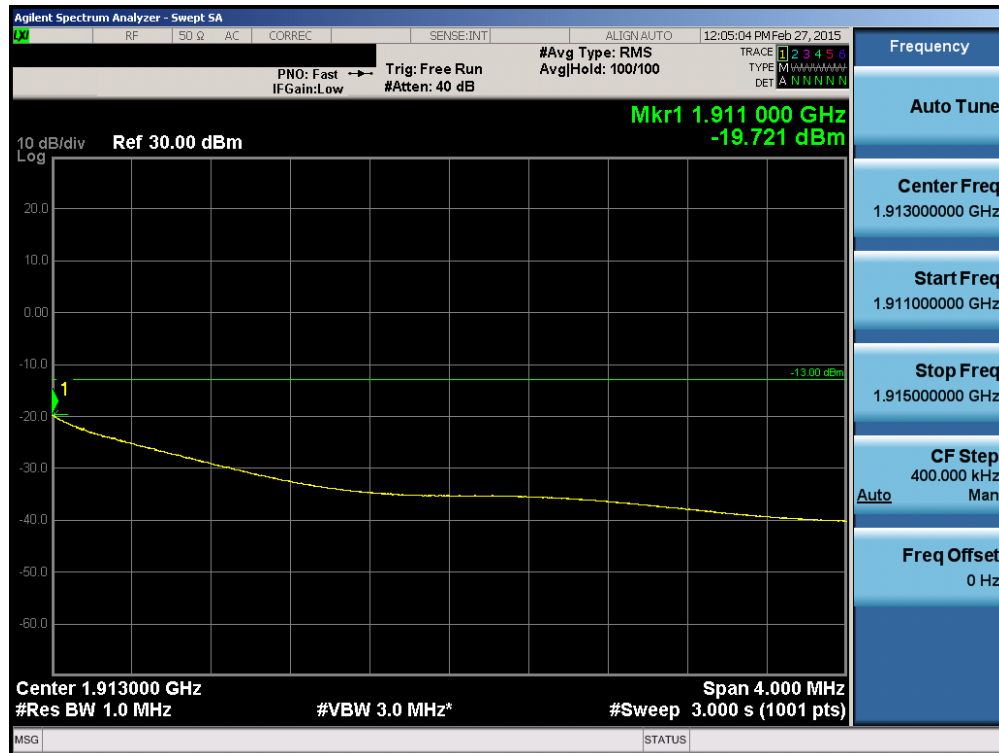
Plot 6-28. 4MHz Span Plot (PCS CDMA Mode – Ch. 1175)
