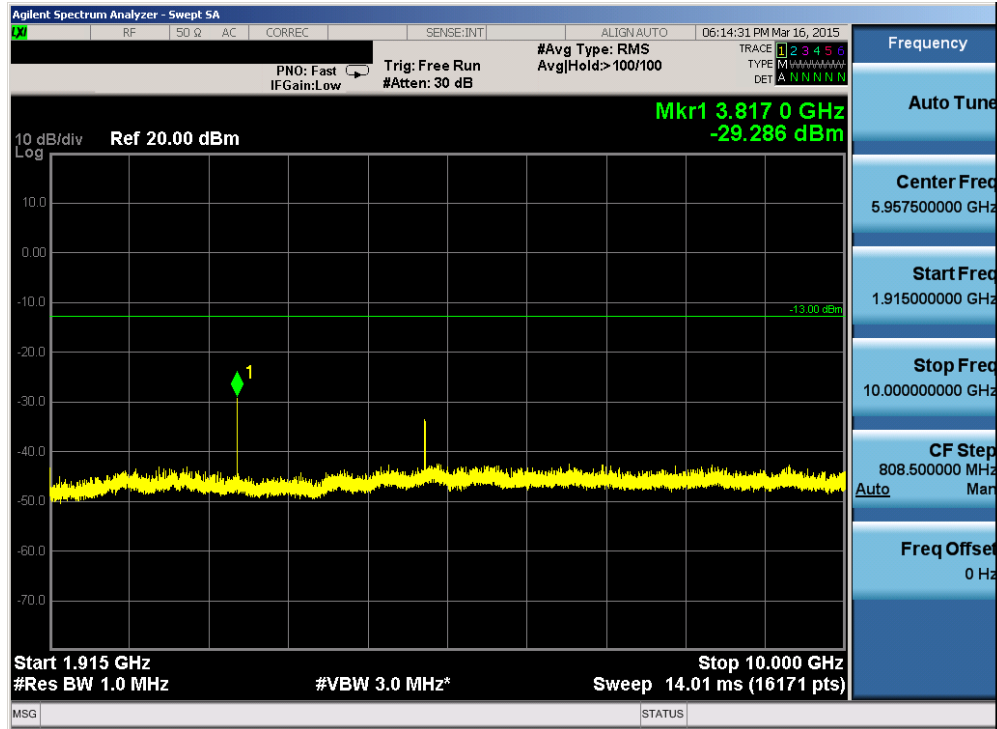
Plot 6-19. Conducted Spurious Plot (PCS CDMA Mode – Ch. 1175)
