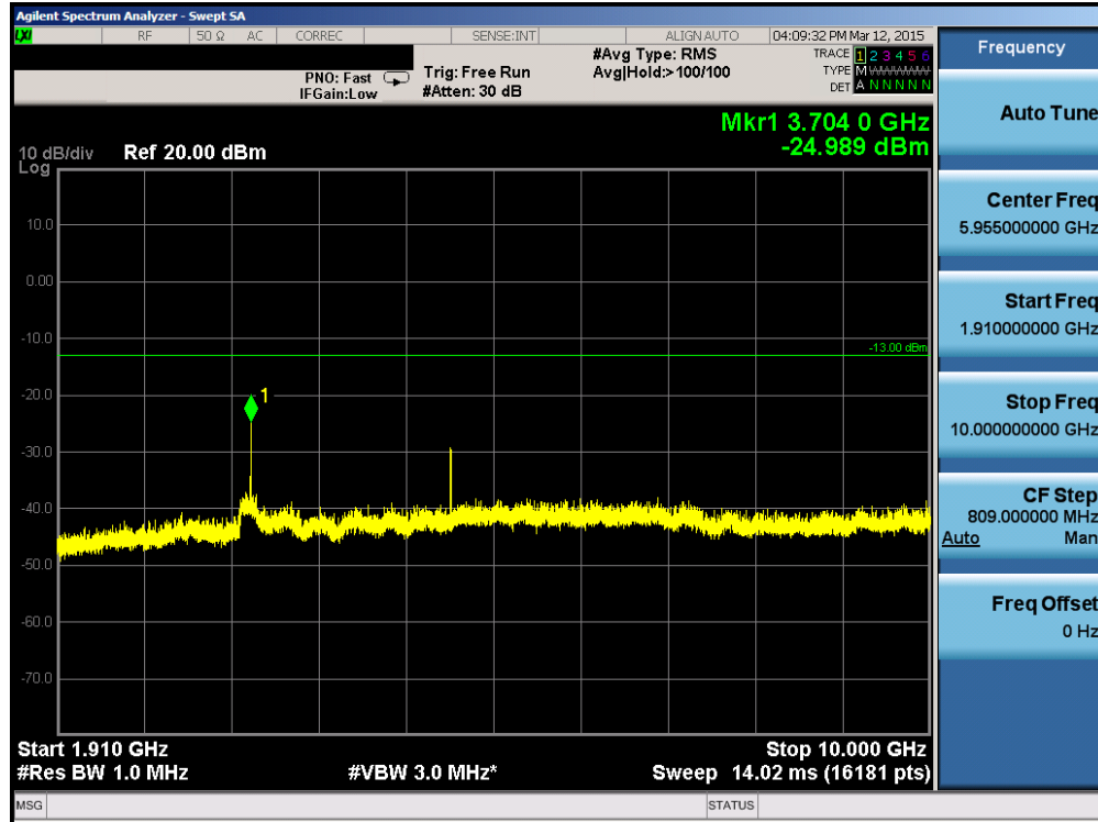
Plot 6-13. Conducted Spurious Plot (PCS CDMA Mode – Ch. 25)
