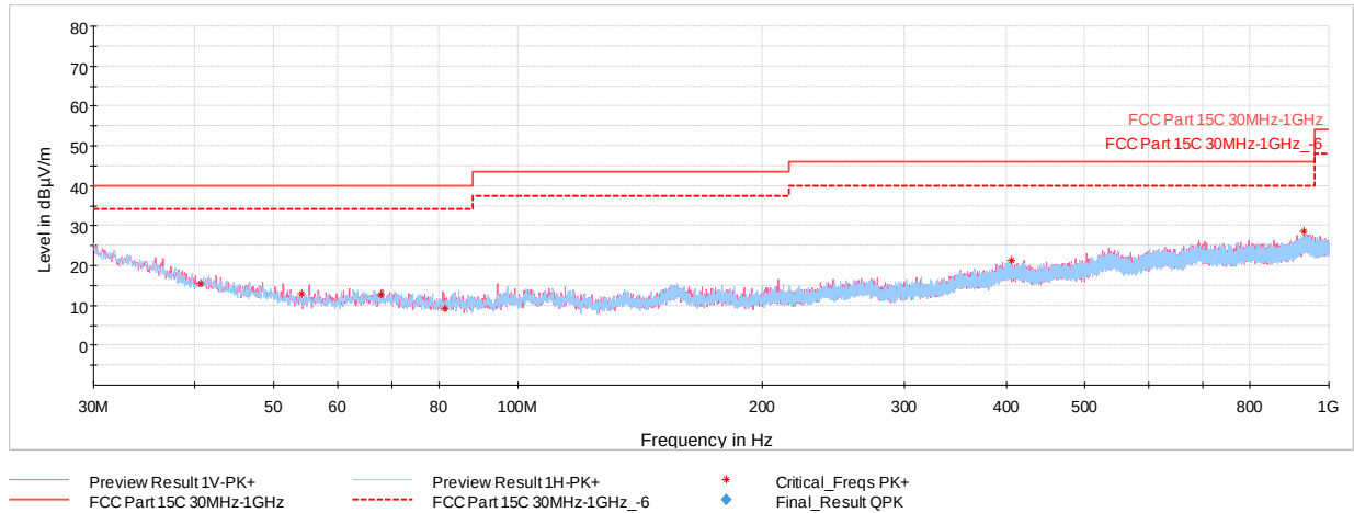
Plot 7-6. Radiated Spurious Emissions 30MHz – 1GHz
