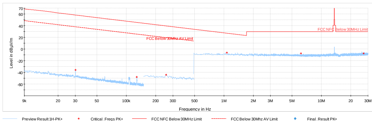
Plot 7-5. Radiated Spurious Emissions 9kHz – 30MHz (Pol. Z)
