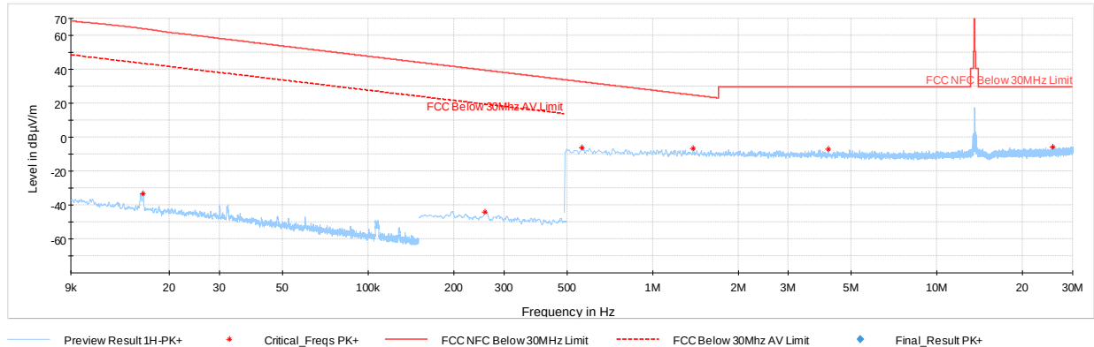
Plot 7-3. Radiated Spurious Emissions 9kHz – 30MHz (Pol. X)
