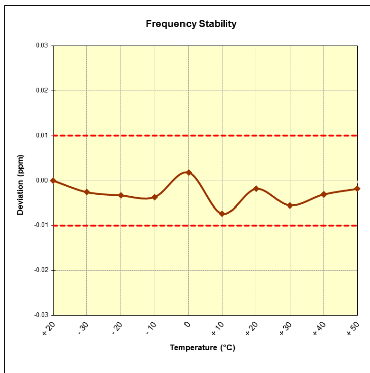
Figure 7-3. Frequency Stability Plot
