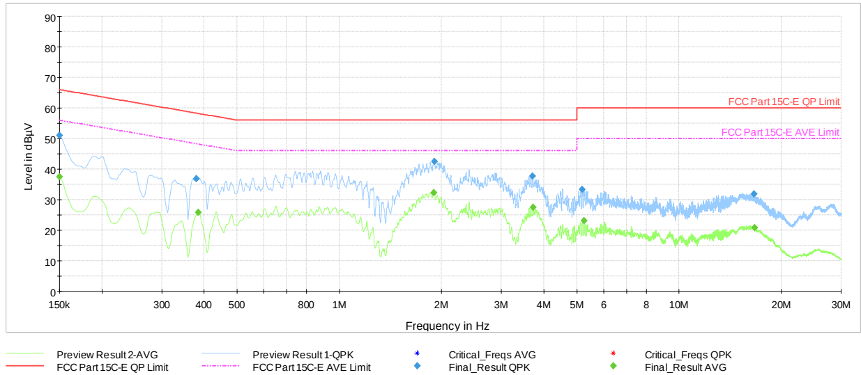
Plot 7-7. AC Line-Conducted Plot (L1)
