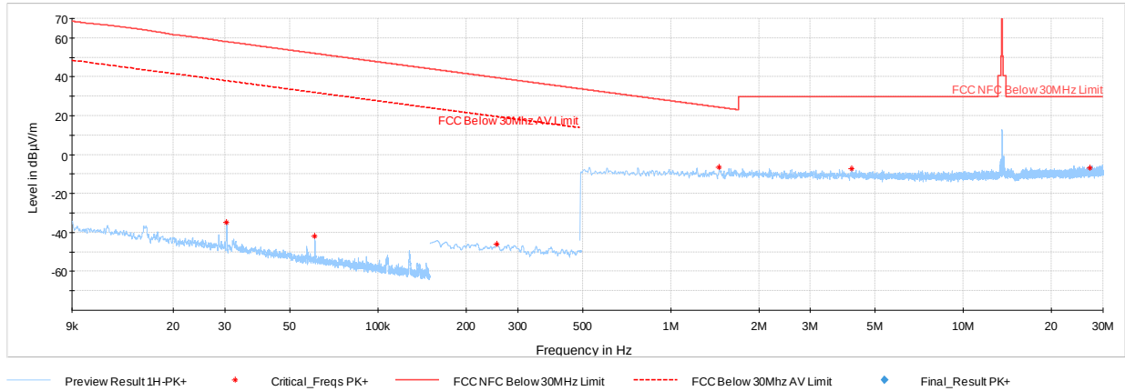
Plot 7-4. Radiated Spurious Emissions 9kHz – 30MHz (Pol. Y)
