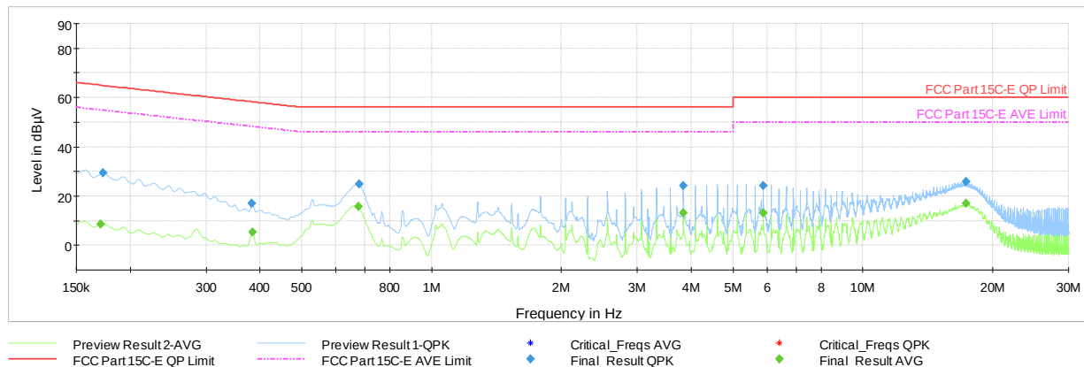
Plot 7-9. AC Line-Conducted Plot (L1) with WCP
