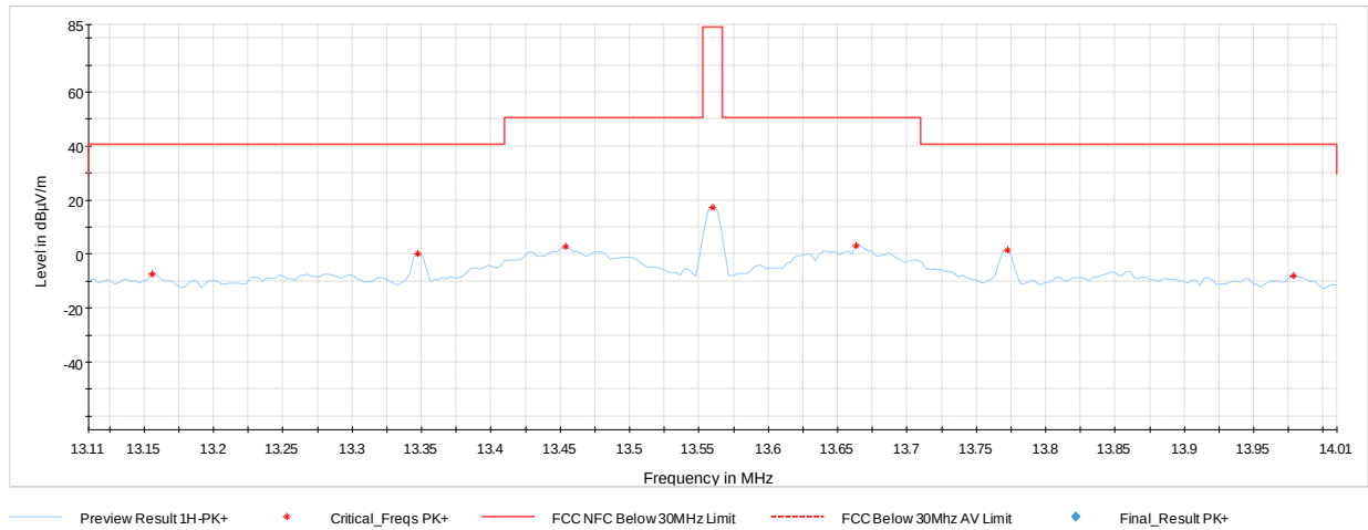
Plot 7-2. In Band Radiated Spurious Emissions
