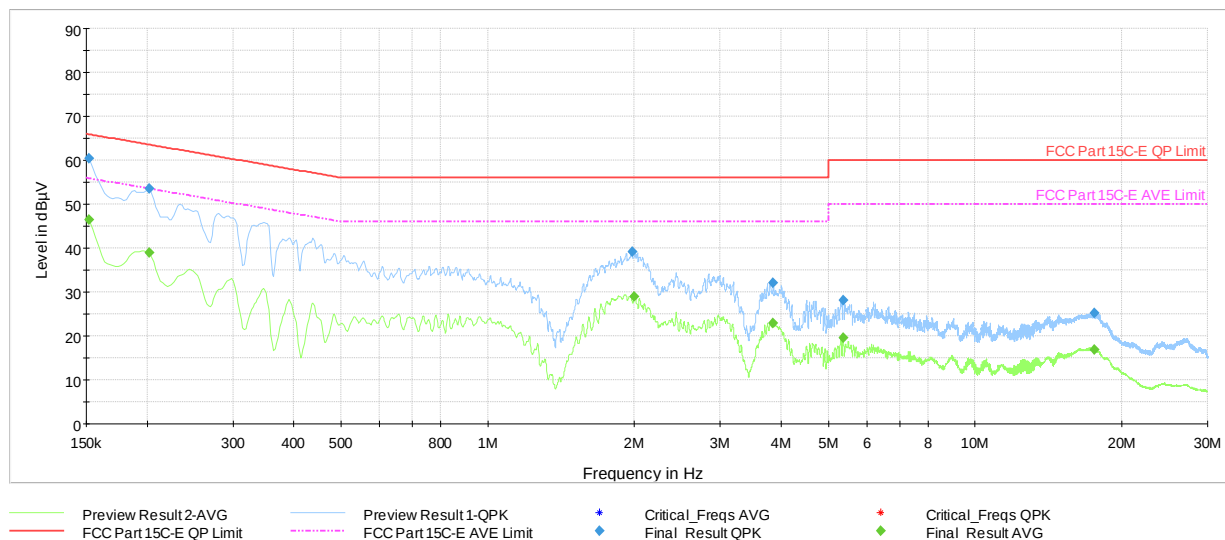
Plot 7-8. AC Line-Conducted Plot (N)
