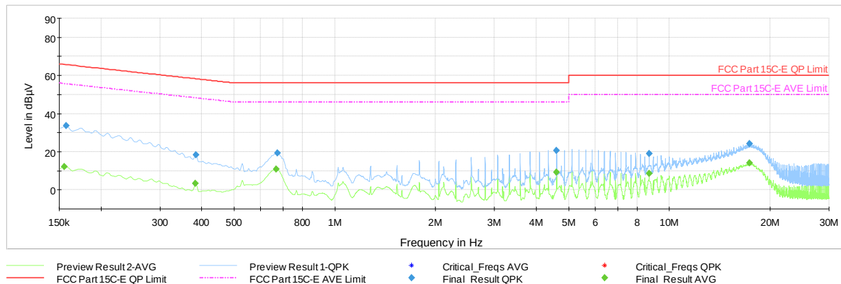
Plot 7-10. AC Line-Conducted Plot (N) with WCP
