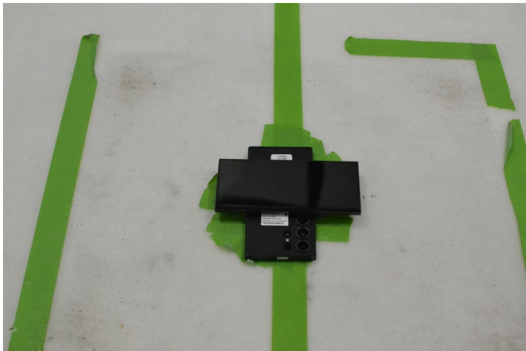
Figure 16. Test Setup – WPT Position – 30Hz-1GHz
