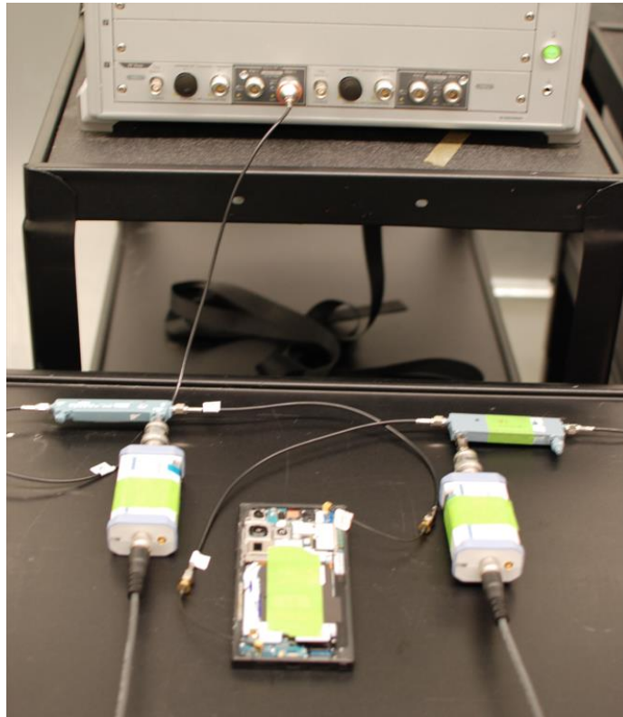
Test Setup Photo 3 – Conducted Test Setup (Figure 5-1c)
