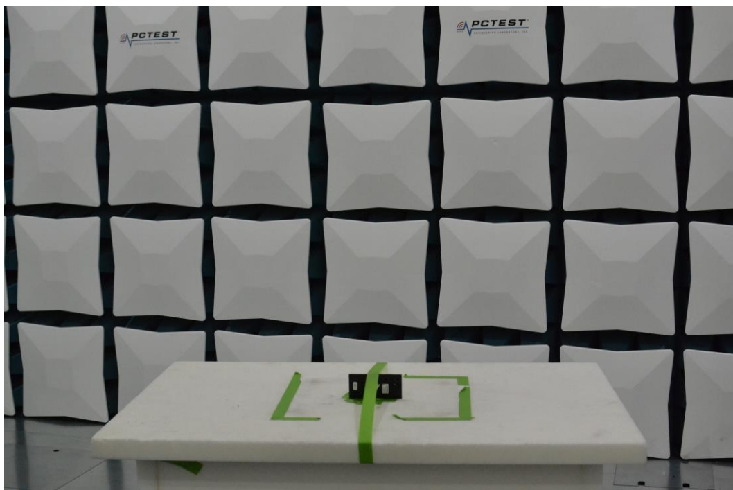
Figure 10. Test Setup – Y Position – 30MHz-1GHz
