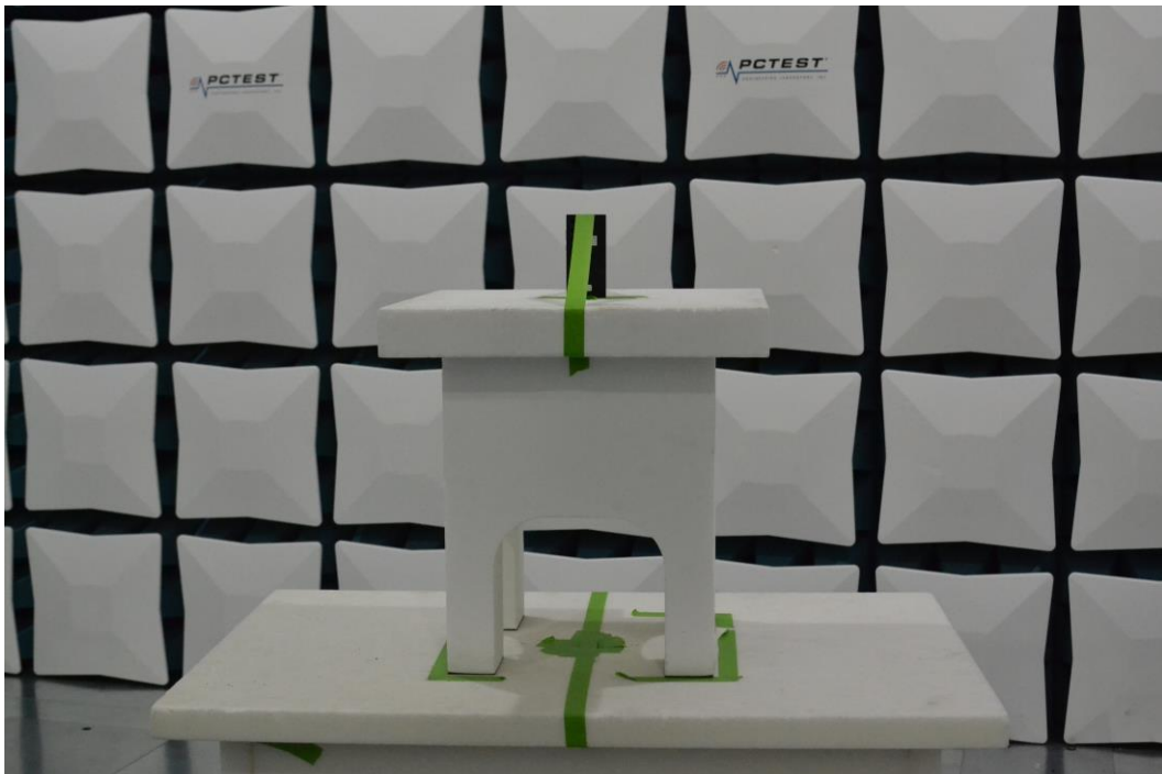
Figure 6. Test Setup – Z Position – 1GHz-18GHz
