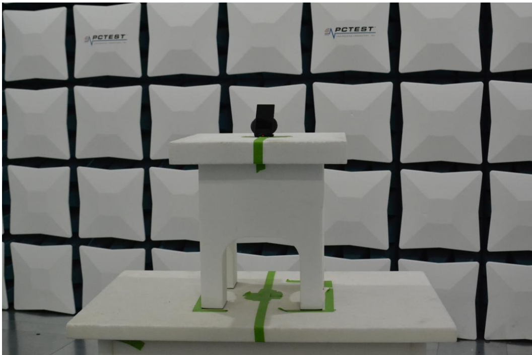
Figure 8. Test Setup – WCP Position – 1GHz-18GHz
