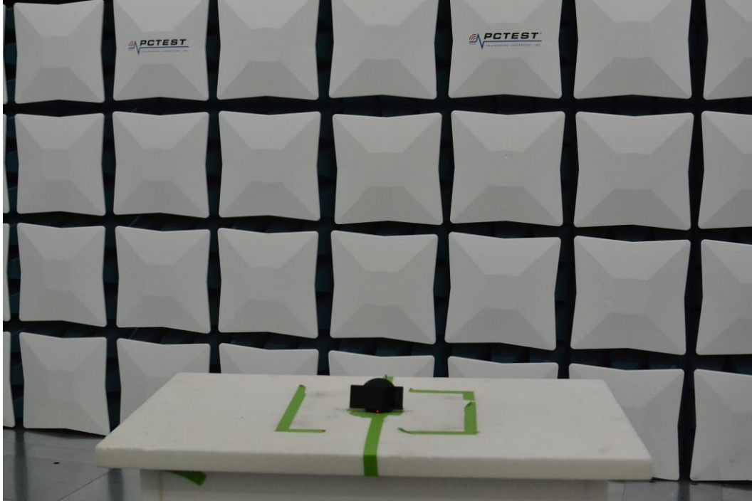
Figure 13. Test Setup – WCP Position – 30MHz-1GHz
