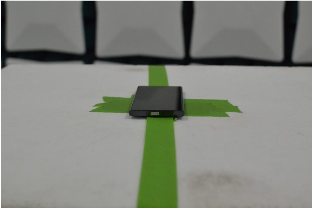
Figure 1. Test Setup – X Position – 1GHz-18GHz
