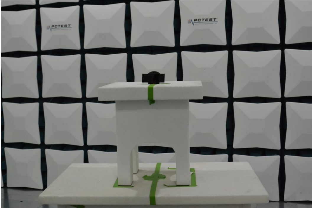
Figure 7. Test Setup – WCP Position – 1GHz-18GHz
