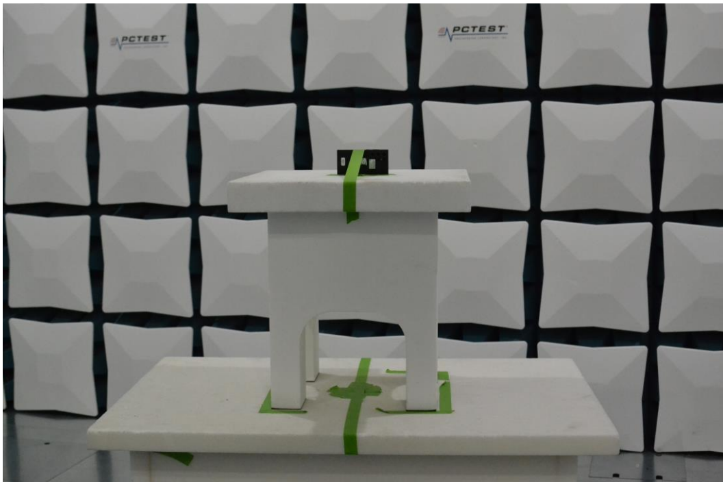
Figure 4. Test Setup – Y Position – 1GHz-18GHz
