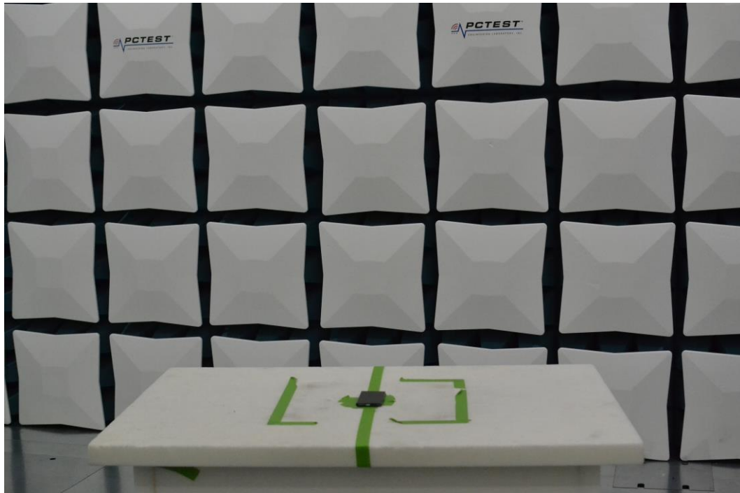
Figure 9. Test Setup – X Position – 30MHz-1GHz
