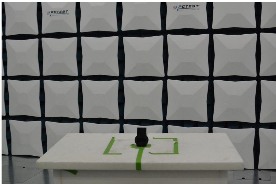
Figure 12. Test Setup – WCP Position – 30MHz-1GHz
