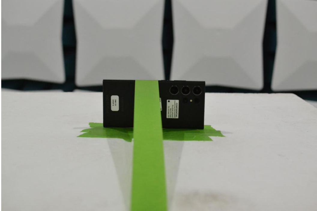
Figure 3. Test Setup – Y Position – 1GHz-18GHz
