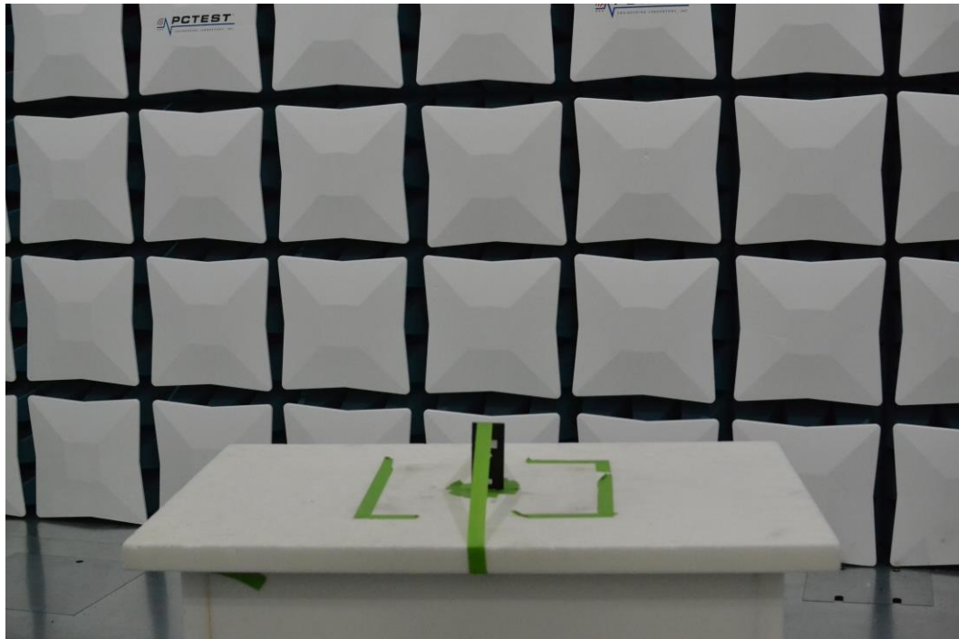
Figure 11. Test Setup – Z Position – 30MHz-1GHz
